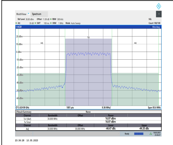
1-N48-PC3-30-30-M-CP-QPSK-Outer_Full-78@0-A nt1-1--PASS
