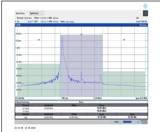
1-N48-PC3-30-20-H-DFT-PI2BPSK-Edge_1RB_Left -1@0-Ant1-1--PASS
