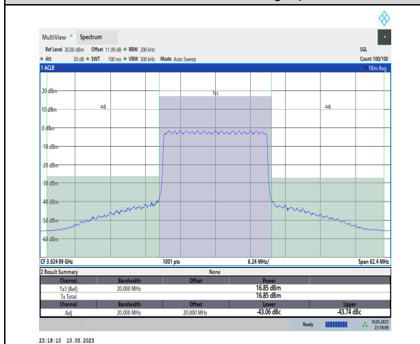
1-N48-PC3-30-20-M-CP-QPSK-Outer_Full-51@0-A nt1-1--PASS
