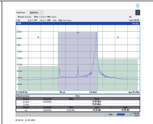
1-N48-PC3-30-30-M-DFT-PI2BPSK-Edge_1RB_Left-1@77-Ant1-1--PASS
