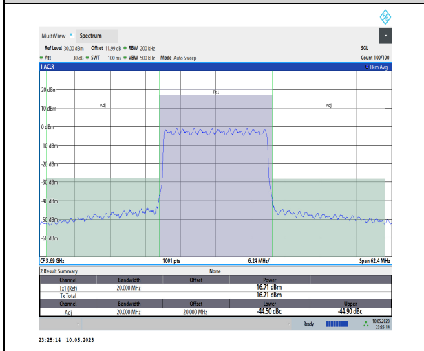
1-N48-PC3-30-20-H-CP-QPSK-Outer_Full-51@0-Ant t1-1--PASS
