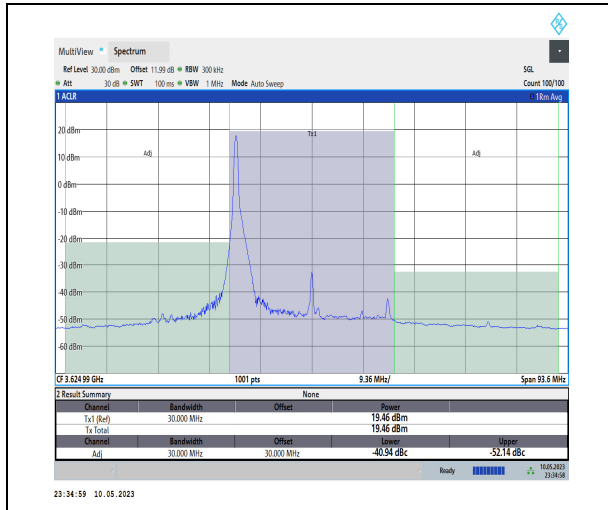
1-N48-PC3-30-30-M-DFT-PI2BPSK-Edge_1RB_Lef t-1@0-Ant1-1--PASS
