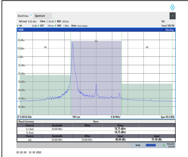
1-N48-PC3-30-30-L-DFT-PI2BPSK-Edge_1RB_Left -1@0-Ant1-1--PASS
