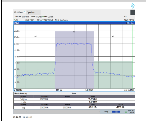
1-N48-PC3-30-20-H-DFT-PI2BPSK-Outer_Full-50@ 0-Ant1-1--PASS
