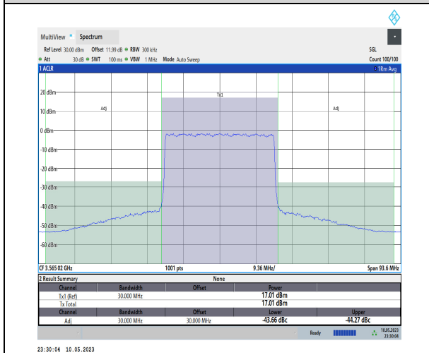
1-N48-PC3-30-30-L-CP-QPSK-Outer_Full-78@0-A nt1-1--PASS
