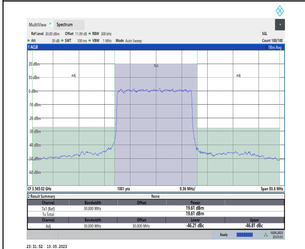
1-N48-PC3-30-30-L-DFT-PI2BPSK-Outer_Full-75@ 0-Ant1-1--PASS
