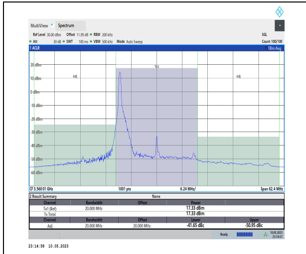
1-N48-PC3-30-20-L-CP-QPSK-Edge_1RB_Left-1@ 0-Ant1-1--PASS-see graph
