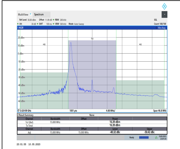
1-N48-PC3-30-15-M-CP-QPSK-Edge_1RB_Left-1@ 0-Ant1-1--PASS-see graph
