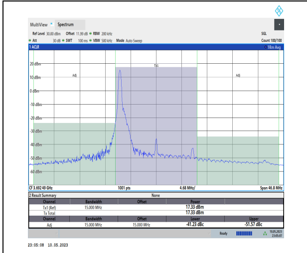
1-N48-PC3-30-15-H-CP-QPSK-Edge_1RB_Left-1@ 0-Ant1-1--PASS-see graph
