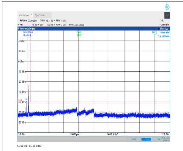
1-N48-PC3-30-40-H-1-DFT-PI2BPSK-Inner_1RB_Le ft-1@1-3000-12000-Ant1-3601.65--40.69--40-PASS
