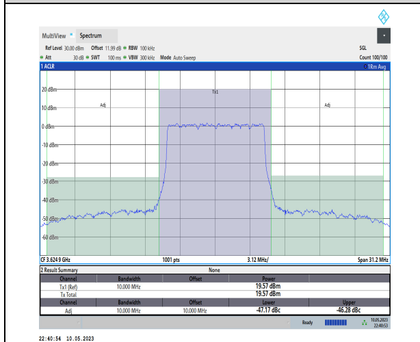
1-N48-PC3-30-10-M-DFT-PI2BPSK-Outer_Full-24@ 0-Ant1-1--PASS
