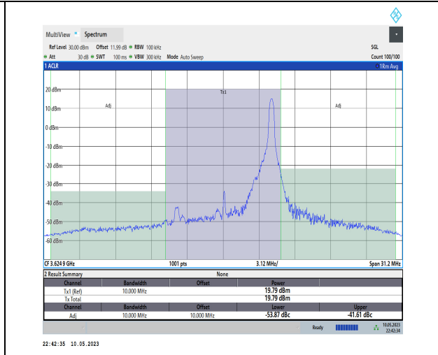
1-N48-PC3-30-10-M-DFT-PI2BPSK-Edge_1RB_Left -1@23-Ant1-1--PASS
