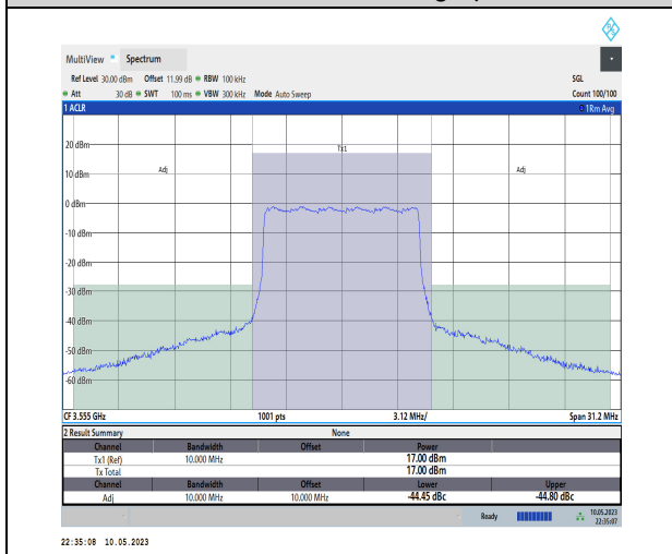
1-N48-PC3-30-10-L-CP-QPSK-Outer_Full-24@0-Ant t1-1--PASS
