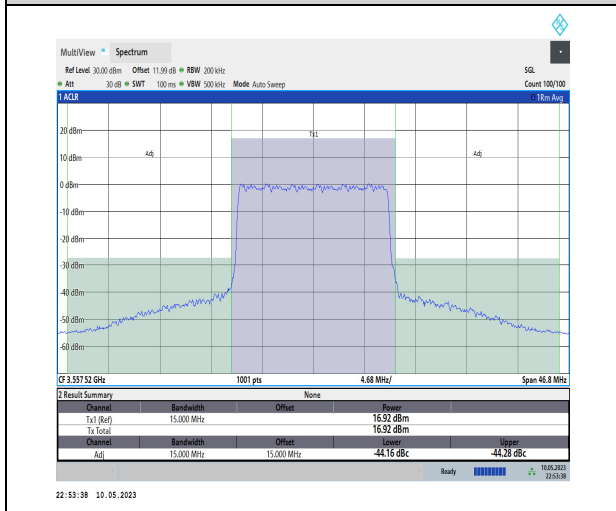
1-N48-PC3-30-15-L-CP-QPSK-Outer_Full-36@0-Ant t1-1--PASS
