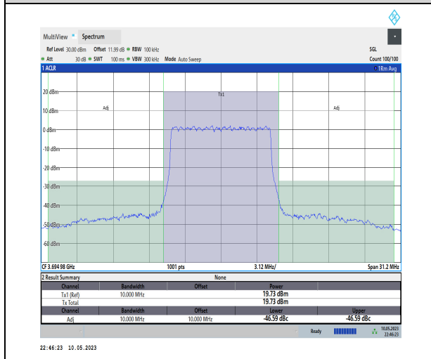
1-N48-PC3-30-10-H-DFT-PI2BPSK-Outer_Full-24@ 0-Ant1-1--PASS
