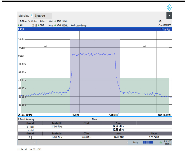
1-N48-PC3-30-15-L-DFT-PI2BPSK-Outer_Full-36@0-Ant1-1--PASS
