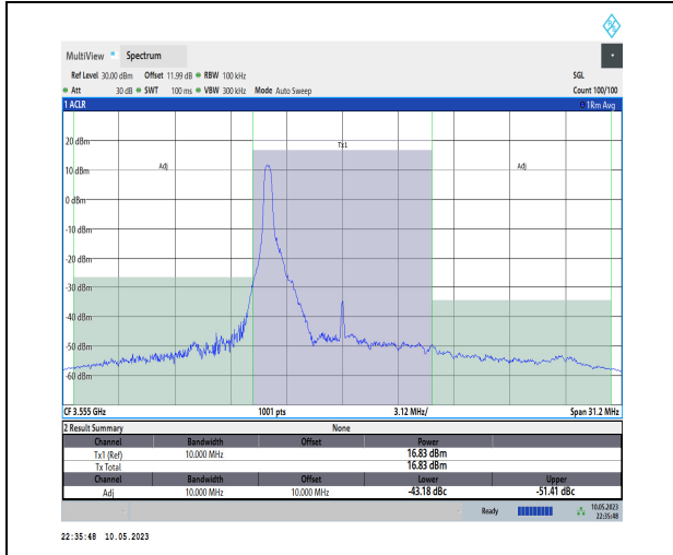
1-N48-PC3-30-10-L-CP-QPSK-Edge_1RB_Left-1@ 0-Ant1-1--PASS-see graph
