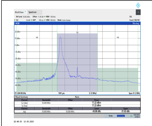
1-N48-PC3-30-10-H-CP-QPSK-Edge_1RB_Left-1@ 0-Ant1-1--PASS-see graph
