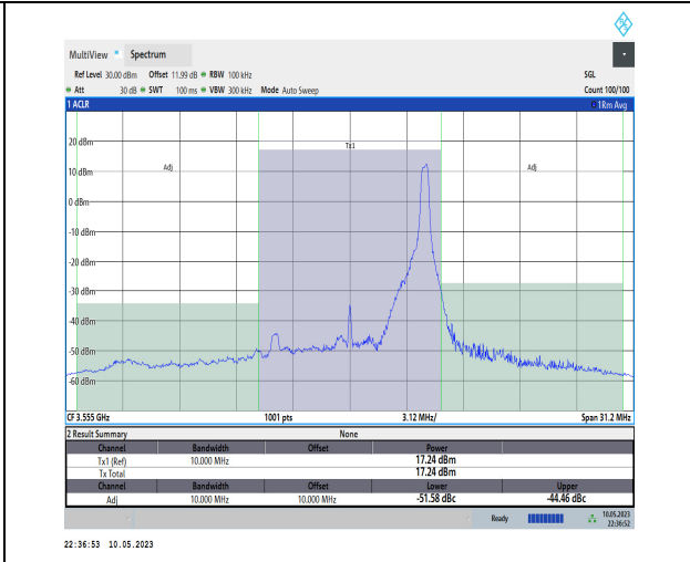
1-N48-PC3-30-10-L-CP-QPSK-Edge_1RB_Left-1@2 3-Ant1-1--PASS
