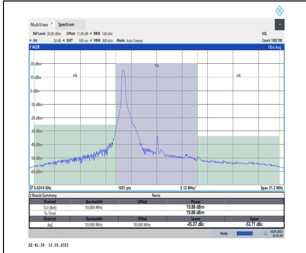
1-N48-PC3-30-10-M-DFT-PI2BPSK-Edge_1RB_Left -1@0-Ant1-1--PASS
