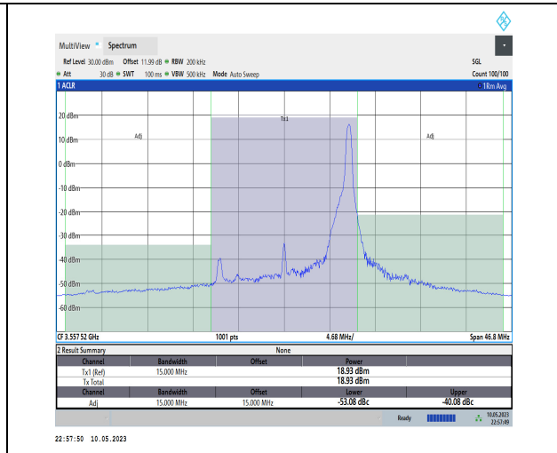
1-N48-PC3-30-15-L-DFT-PI2BPSK-Edge_1RB_Left-1@37-Ant1-1--PASS
