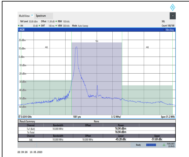
1-N48-PC3-30-10-M-CP-QPSK-Edge_1RB_Left-1@ 0-Ant1-1--PASS-see graph
