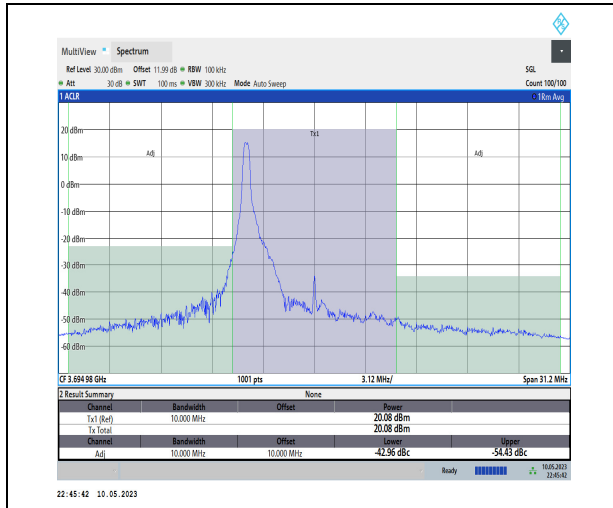
1-N48-PC3-30-10-H-DFT-PI2BPSK-Edge_1RB_Left -1@0-Ant1-1--PASS
