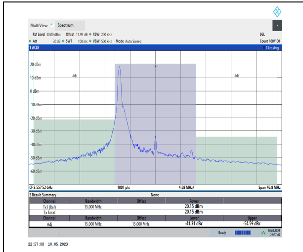
1-N48-PC3-30-15-L-DFT-PI2BPSK-Edge_1RB_Left-1@0-Ant1-1--PASS
