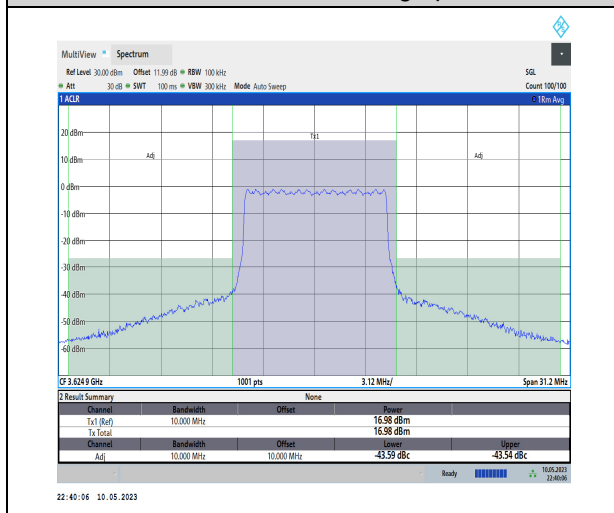
1-N48-PC3-30-10-M-CP-QPSK-Outer_Full-24@0-A nt1-1--PASS
