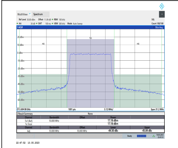
1-N48-PC3-30-10-H-CP-QPSK-Outer_Full-24@0-Ant t1-1--PASS
