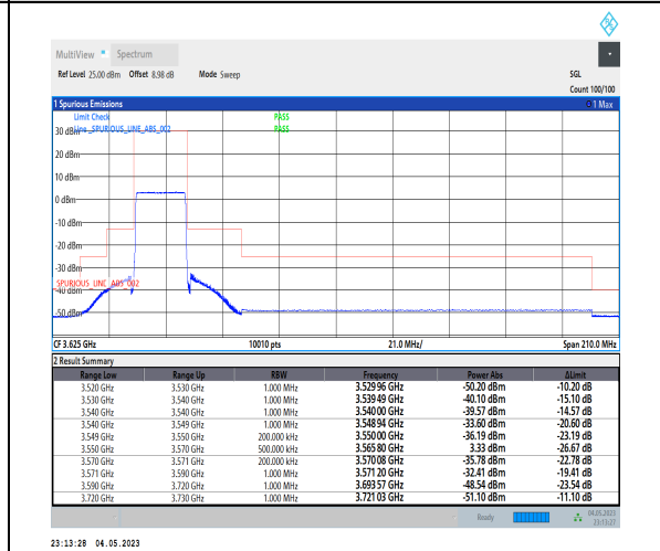
1-N48-PC3-30-20-L-6-CP-QPSK-Outer_Full-51@0-Ant1-1--PASS-see graph
