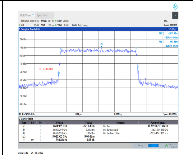
1-N48-PC3-30-40-M-7-CP-16QAM-Outer_Full-106@0 -Ant1-37.77-39.680-<math>\leq 40</math>-PASS
