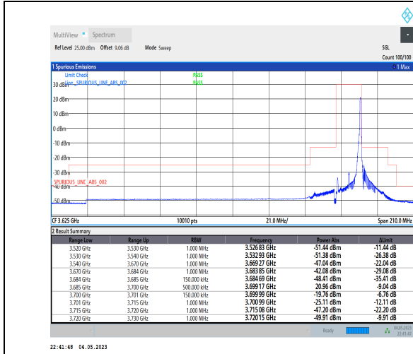
1-N48-PC3-30-15-H-2-DFT-PI2BPSK-Edge_1RB_Right-t_1@37-Ant1-1--PASS-see graph
