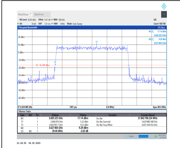
1-N48-PC3-30-40-M-8-CP-64QAM-Outer_Full-106@ 0-Ant1-37.843-39.440-≤40-PASS
