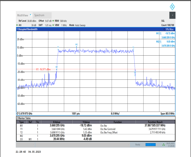
1-N48-PC3-30-40-H-8-CP-64QAM-Outer_Full-106@ 0-Ant1-37.868-39.440-≤40-PASS
