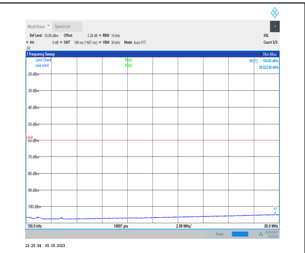
1-N48-PC3-30-40-M-1-DFT-PI2BPSK-Inner_1RB_Le ft-1@1-0.15-30-Ant1-29.74--104.65--60-PASS
