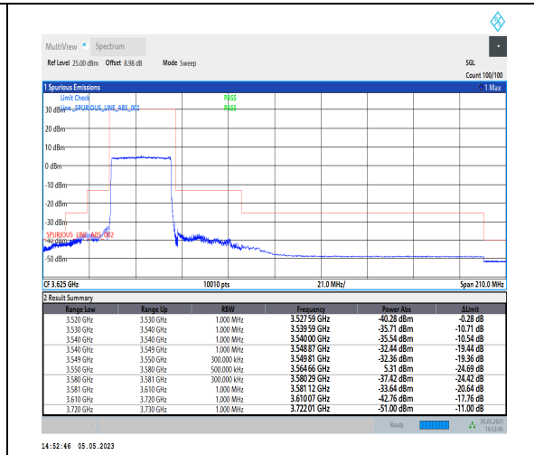
1-N48-PC3-30-30-L-3-DFT-PI2BPSK-Outer_Full-75@0-Ant1-1--PASS-see graph
