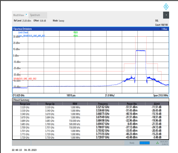
1-N48-PC3-30-15-H-3-DFT-PI2BPSK-Outer_Full-36@0-Ant1-1--PASS-see graph
