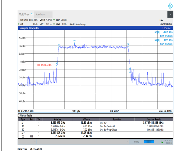
1-N48-PC3-30-40-H-1-DFT-QPSK-Outer_Full-100@ 0-Ant1-35.757-37.760-≤40-PASS
