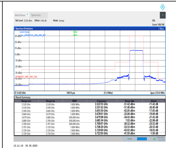
1-N48-PC3-30-20-H-3-DFT-PI2BPSK-Outer_Full-5 0@0-Ant1-1--PASS-see graph
