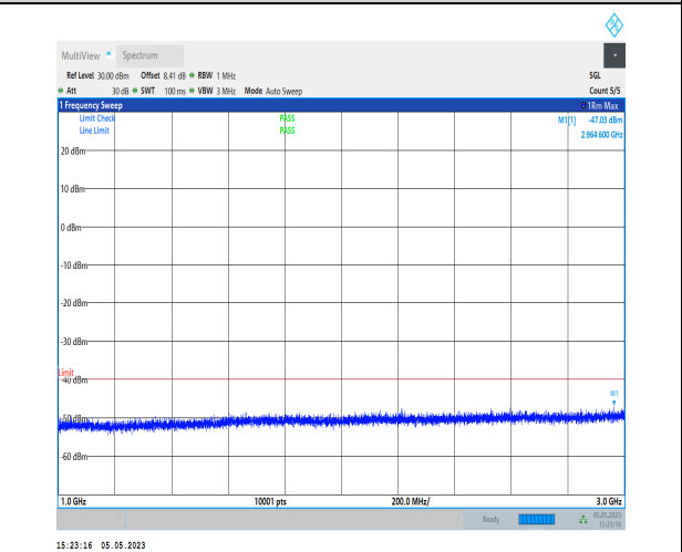
1-N48-PC3-30-40-H-1-DFT-PI2BPSK-Inner_1RB_Le ft-1@1-1000-3000-Ant1-2677.60--47.03--40-PASS
