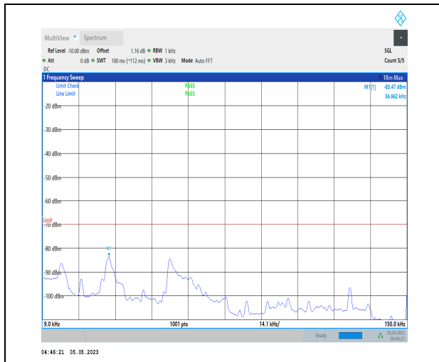
1-N48-PC3-30-40-M-1-DFT-PI2BPSK-Inner_1RB_Le ft-1@1-0.009-0.15-Ant1-0.01--112.00--70-PASS
