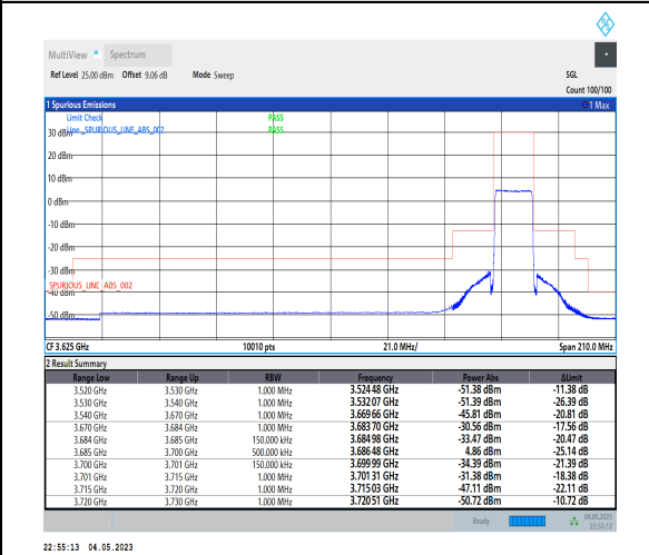
1-N48-PC3-30-15-H-6-CP-QPSK-Outer_Full-38@0-Ant1-1--PASS-see graph
