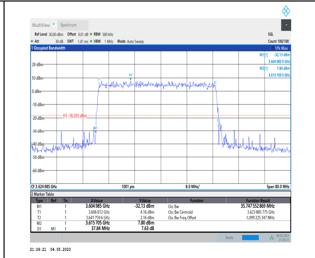
1-N48-PC3-30-40-M-5-DFT-256QAM-Outer_Full-100 @0-Ant1-35.748-37.840-<math>\leq 40</math>-PASS
