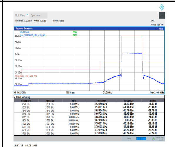
1-N48-PC3-30-30-H-6-CP-QPSK-Outer_Full-78@0-Ant1-1--PASS-see graph
