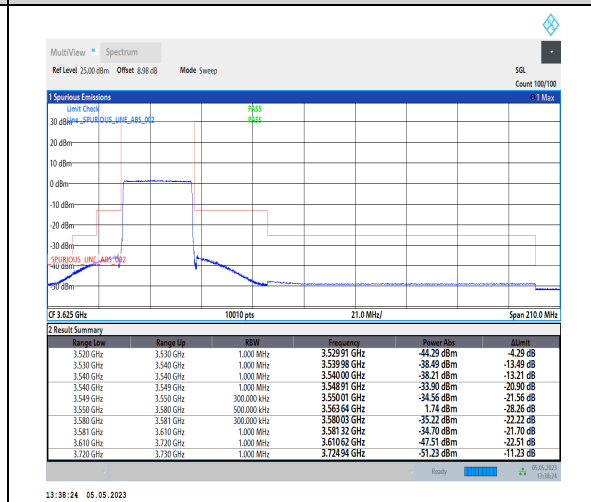
1-N48-PC3-30-30-L-6-CP-QPSK-Outer_Full-78@0-Ant1-1--PASS-see graph
