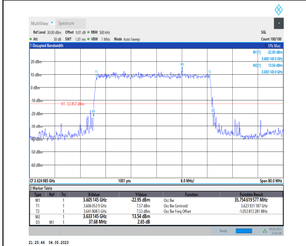
1-N48-PC3-30-40-M-2-DFT-PI2BPSK-Outer_Full-10 0@0-Ant1-35.755-37.680-≤40-PASS
