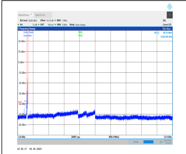
1-N48-PC3-30-40-L-1-DFT-PI2BPSK-Inner_1RB_Lef t-1@1-3000-12000-Ant1-3496.80--40.74--40-PASS
