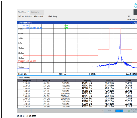
1-N48-PC3-30-20-H-2-DFT-PI2BPSK-Edge_1RB_Righ t_1@50-Ant1-1--PASS-see graph
