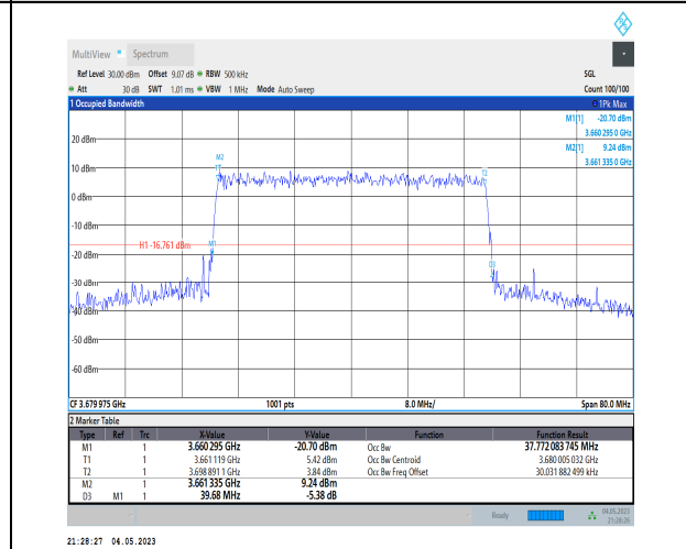
1-N48-PC3-30-40-H-6-CP-QPSK-Outer_Full-106@0 -Ant1-37.772-39.680-≤40-PASS
