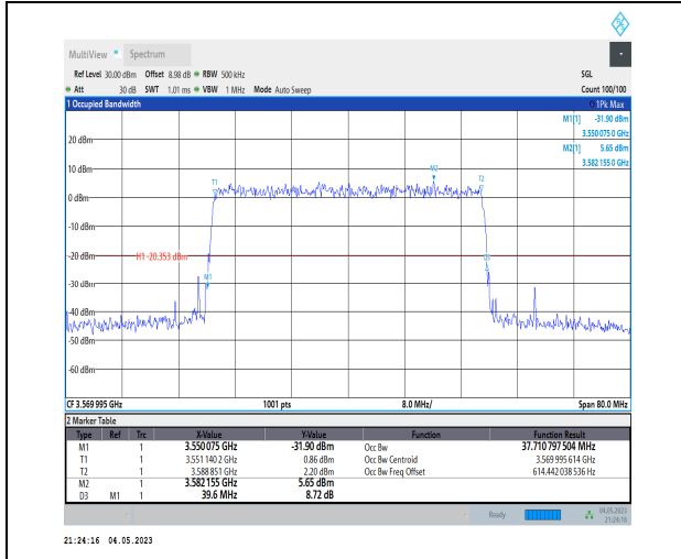
1-N48-PC3-30-40-L-9-CP-256QAM-Outer_Full-106 @0-Ant1-37.711-39.600-≤40-PASS
