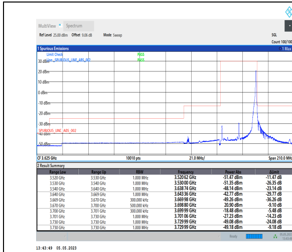
1-N48-PC3-30-30-H-2-DFT-PI2BPSK-Edge_1RB_Right-t1@77-Ant1-1--PASS-see graph
