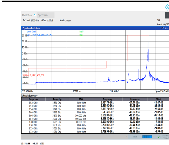
1-N48-PC3-30-30-H-5-CP-QPSK-Edge_1RB_Right-1@77-Ant1-1--PASS-see graph
