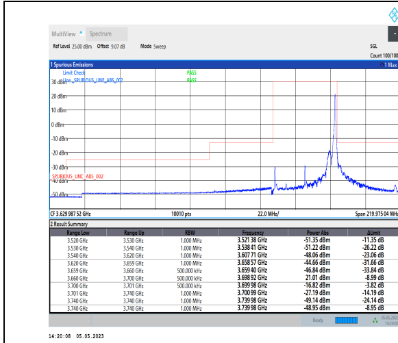
1-N48-PC3-30-40-H-2-DFT-PI2BPSK-Edge_1RB_Right t_1@105-Ant1-1--PASS-see graph
