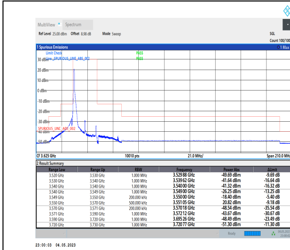
1-N48-PC3-30-20-L-1-DFT-PI2BPSK-Edge_1RB_Left-1@0-Ant1-1--PASS-see graph
