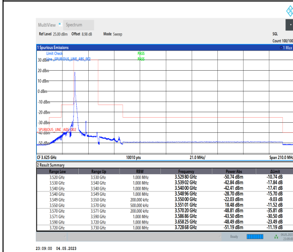
1-N48-PC3-30-20-L-4-CP-QPSK-Edge_1RB_Left-1@0-Ant1-1--PASS-see graph
