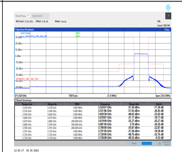
1-N48-PC3-30-20-H-6-CP-QPSK-Outer_Full-51@ 0-Ant1-1--PASS-see graph
