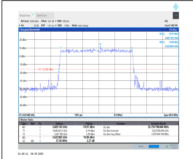
1-N48-PC3-30-40-M-4-DFT-64QAM-Outer_Full-100 @0-Ant1-35.76-37.360-<math>\leq 40</math>-PASS
