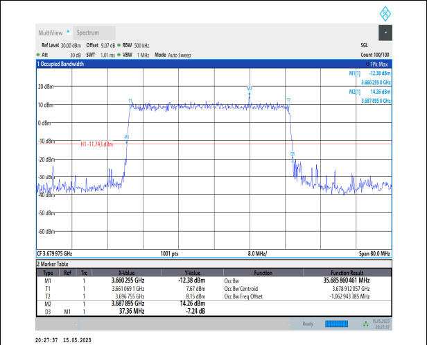
1-N48-PC3-30-40-H-2-DFT-PI2BPSK-Outer_Full-100@ 0-Ant1-35.686-37.360-≤40-PASS
