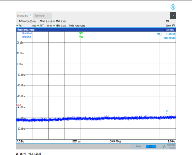
1-N48-PC3-30-40-M-1-DFT-PI2BPSK-Inner_1RB_Le ft-1@1-1000-3000-Ant1-2721.40--47.14--40-PASS
