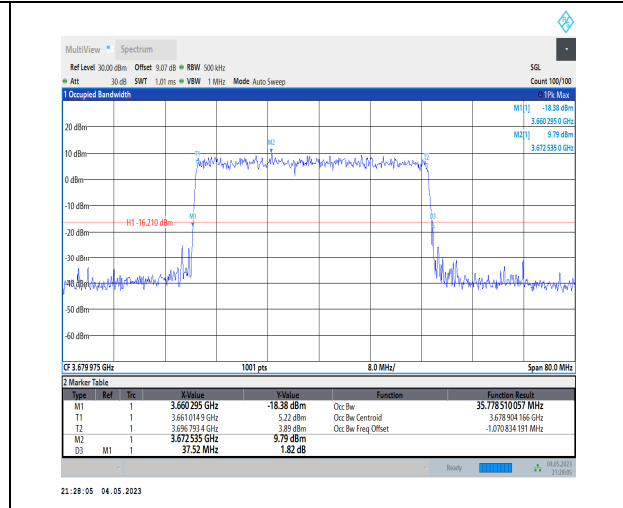
1-N48-PC3-30-40-H-4-DFT-64QAM-Outer_Full-100 @0-Ant1-35.779-37.520-≤40-PASS
