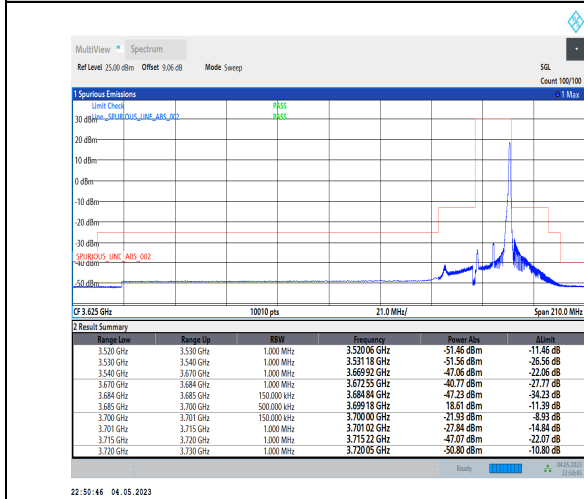
1-N48-PC3-30-15-H-5-CP-QPSK-Edge_1RB_Right-1@37-Ant1-1--PASS-see graph
