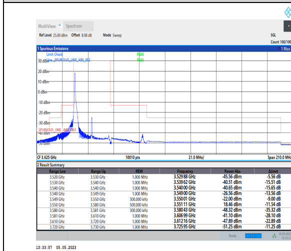
1-N48-PC3-30-30-L-4-CP-QPSK-Edge_1RB_Left-1@0-Ant1-1--PASS-see graph
