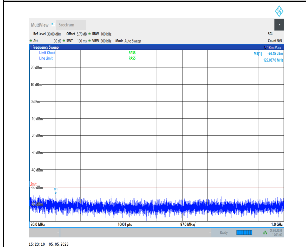
1-N48-PC3-30-40-H-1-DFT-PI2BPSK-Inner_1RB_Le ft-1@1-30-1000-Ant1-53.67--54.45--50-PASS
