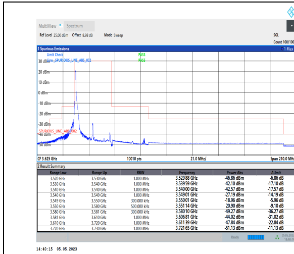
1-N48-PC3-30-30-L-1-DFT-PI2BPSK-Edge_1RB_Left-1@0-Ant1-1--PASS-see graph
