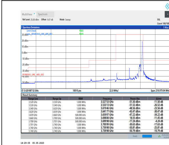
1-N48-PC3-30-40-H-5-CP-QPSK-Edge_1RB_Right-1 @105-Ant1-1--PASS-see graph
