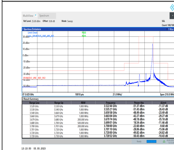
1-N48-PC3-30-20-H-5-CP-QPSK-Edge_1RB_Righ t_1@50-Ant1-1--PASS-see graph
