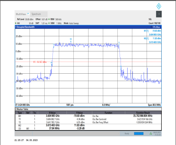
1-N48-PC3-30-40-M-1-DFT-QPSK-Outer_Full-100@ 0-Ant1-35.703-37.840-≤40-PASS
