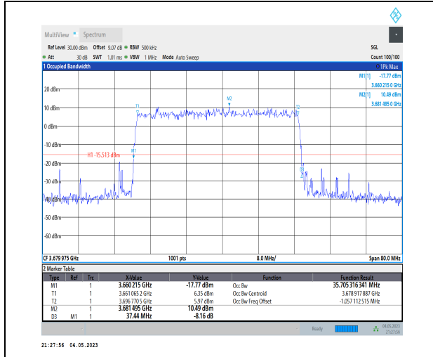
1-N48-PC3-30-40-H-3-DFT-16QAM-Outer_Full-100 @0-Ant1-35.705-37.440-≤40-PASS
