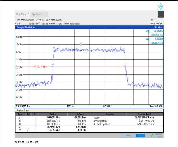
1-N48-PC3-30-40-M-9-CP-256QAM-Outer_Full-106 @0-Ant1-37.778-39.280-≤40-PASS
