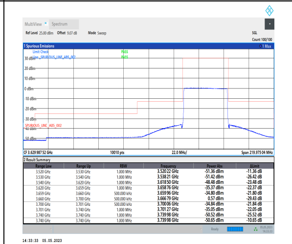
1-N48-PC3-30-40-H-6-CP-QPSK-Outer_Full-106 @0-Ant1-1--PASS-see graph
