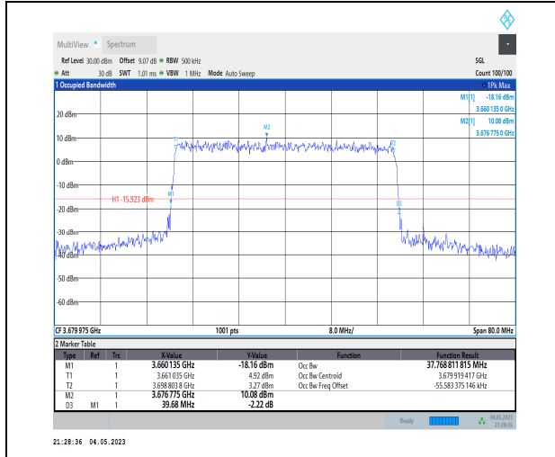
1-N48-PC3-30-40-H-7-CP-16QAM-Outer_Full-106@ 0-Ant1-37.769-39.680-≤40-PASS
