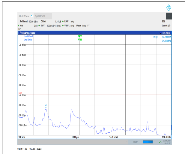
1-N48-PC3-30-40-H-1-DFT-PI2BPSK-Inner_1RB_Le ft-1@1-0.009-0.15-Ant1-0.01--112.02--70-PASS
