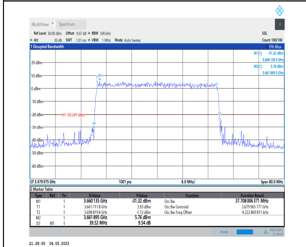
1-N48-PC3-30-40-H-9-CP-256QAM-Outer_Full-106@ @0-Ant1-37.708-39.520-≤40-PASS
