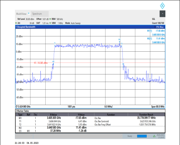
1-N48-PC3-30-40-M-3-DFT-16QAM-Outer_Full-100 @0-Ant1-35.778-37.280-≤40-PASS
