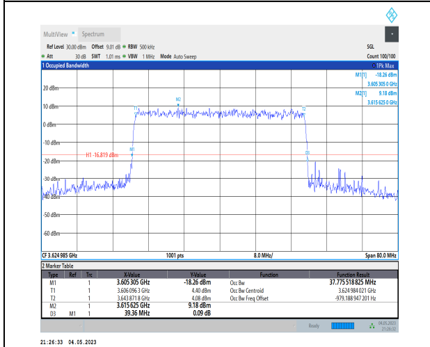
1-N48-PC3-30-40-M-6-CP-QPSK-Outer_Full-106@0 -Ant1-37.776-39.360-<math>\leq 40</math>-PASS
