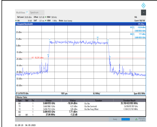
1-N48-PC3-30-40-H-5-DFT-256QAM-Outer_Full-100 @0-Ant1-35.769-37.840-≤40-PASS
