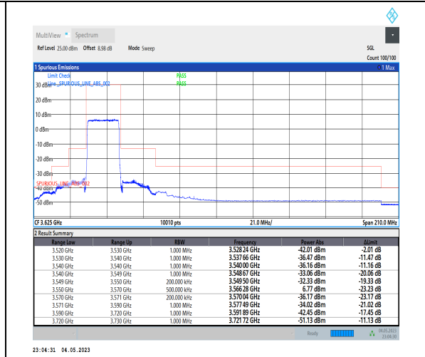
1-N48-PC3-30-20-L-3-DFT-PI2BPSK-Outer_Full-50@0-Ant1-1--PASS-see graph
