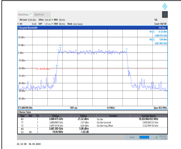
1-N48-PC3-30-20-H-9-CP-256QAM-Outer_Full-51@ @-Ant1-18.203-19.040-≤20-PASS
