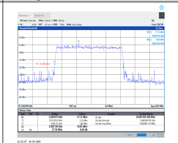
1-N48-PC3-30-40-L-4-DFT-64QAM-Outer_Full-100 @0-Ant1-35.698-37.760-≤40-PASS
