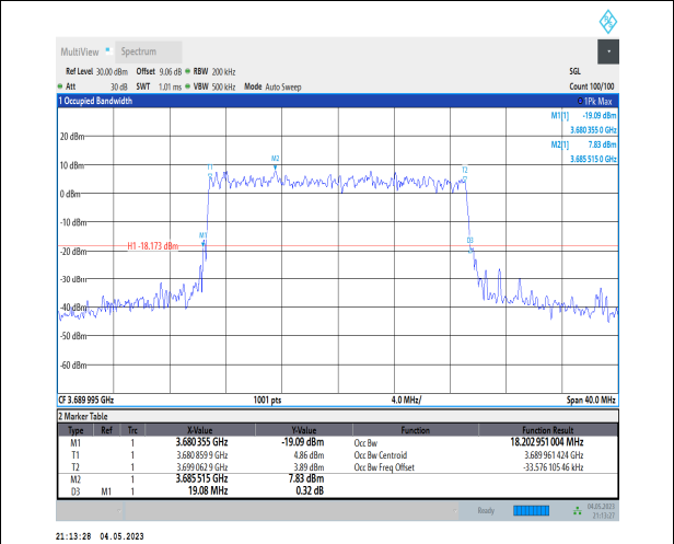
1-N48-PC3-30-20-H-8-CP-64QAM-Outer_Full-51@0 -Ant1-18.203-19.080-<=20-PASS
