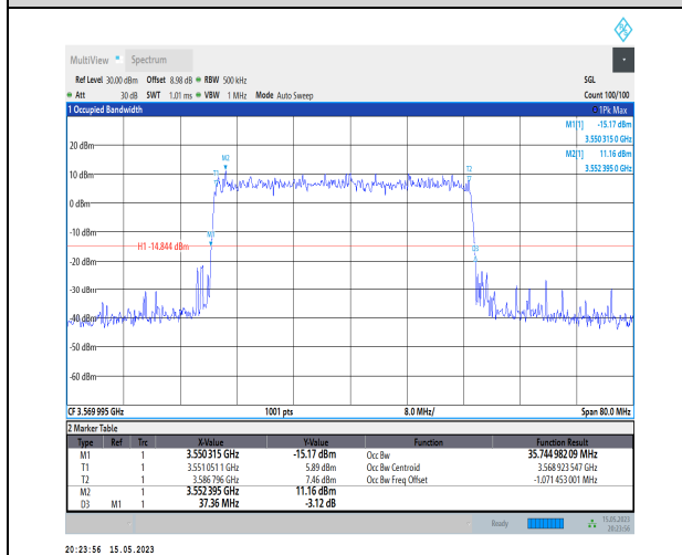
1-N48-PC3-30-40-L-3-DFT-16QAM-Outer_Full-100 @0-Ant1-35.745-37.360-≤40-PASS
