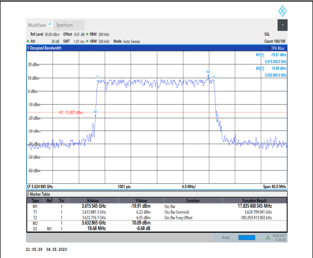
1-N48-PC3-30-20-M-3-DFT-16QAM-Outer_Full-50@ 0-Ant1-17.835-18.680-≤20-PASS
