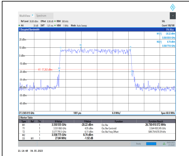
1-N48-PC3-30-30-L-4-DFT-64QAM-Outer_Full-75@ 0-Ant1-26.73-27.840-≤30-PASS
