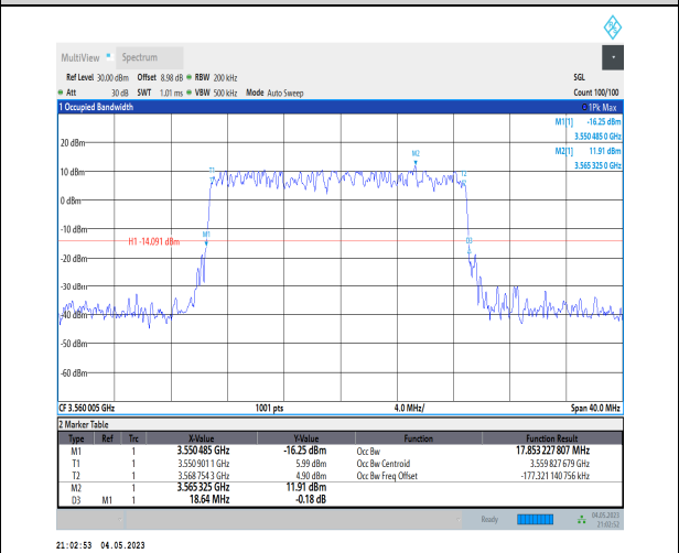
1-N48-PC3-30-20-L-2-DFT-PI2BPSK-Outer_Full-50@0 -Ant1-17.853-18.640-≤20-PASS
