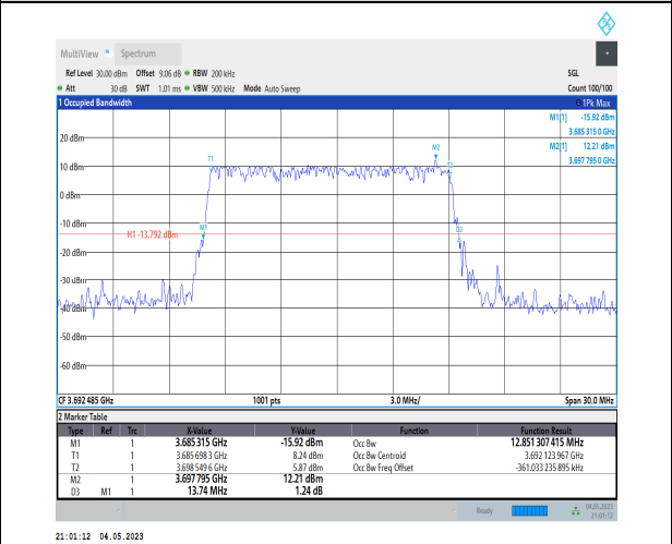
1-N48-PC3-30-15-H-3-DFT-16QAM-Outer_Full-36@ @-Ant1-12.851-13.740≤15-PASS
