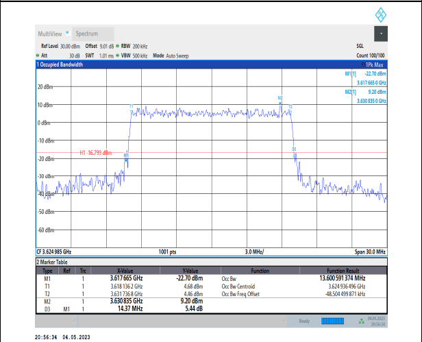
1-N48-PC3-30-15-M-8-CP-64QAM-Outer_Full-38@0 -Ant1-13.601-14.370-≤15-PASS
