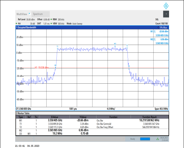
1-N48-PC3-30-20-L-6-CP-QPSK-Outer_Full-51@0- Ant1-18.22-19.200-≤20-PASS
