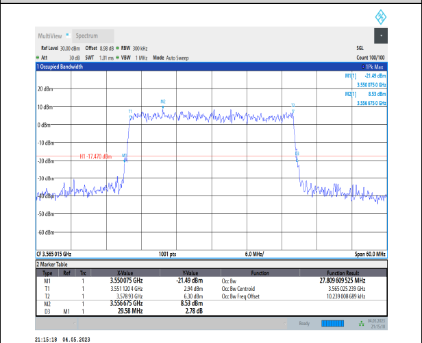
1-N48-PC3-30-30-L-7-CP-16QAM-Outer_Full-78@0- Ant1-27.81-29.580-≤30-PASS
