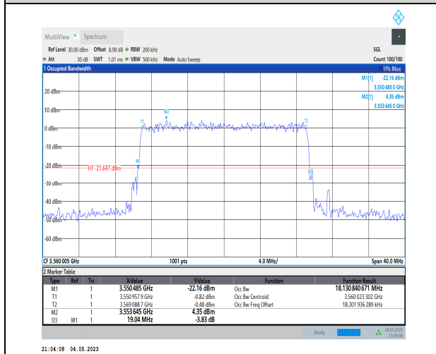
1-N48-PC3-30-20-L-9-CP-256QAM-Outer_Full-51@0- Ant1-18.131-19.040-≤20-PASS
