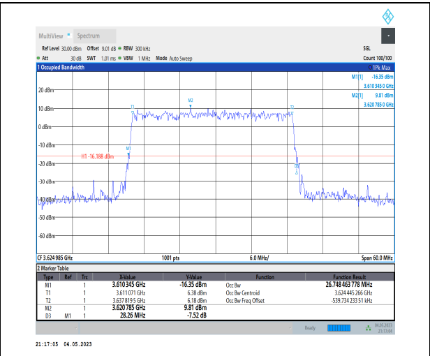
1-N48-PC3-30-30-M-4-DFT-64QAM-Outer_Full-75@ 0-Ant1-26.748-28.260-≤30-PASS
