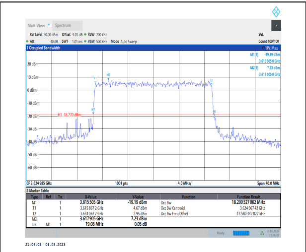
1-N48-PC3-30-20-M-7-CP-16QAM-Outer_Full-51@0- -Ant1-18.201-19.080-<20-PASS
