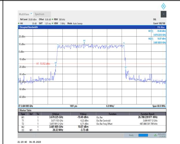
1-N48-PC3-30-30-H-1-DFT-QPSK-Outer_Full-75@0 -Ant1-26.788-28.320-≤30-PASS
