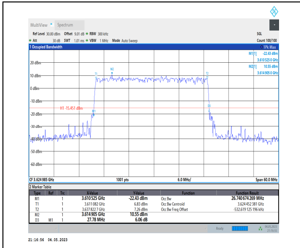
1-N48-PC3-30-30-M-3-DFT-16QAM-Outer_Full-75@ 0-Ant1-26.741-27.780-≤30-PASS
