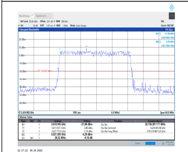
1-N48-PC3-30-30-M-5-DFT-256QAM-Outer_Full-75@ @0-Ant1-26.736-28.320-≤30-PASS
