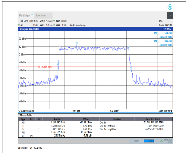
1-N48-PC3-30-30-H-2-DFT-PI2BPSK-Outer_Full-75 @0-Ant1-26.798-28.380-≤30-PASS
