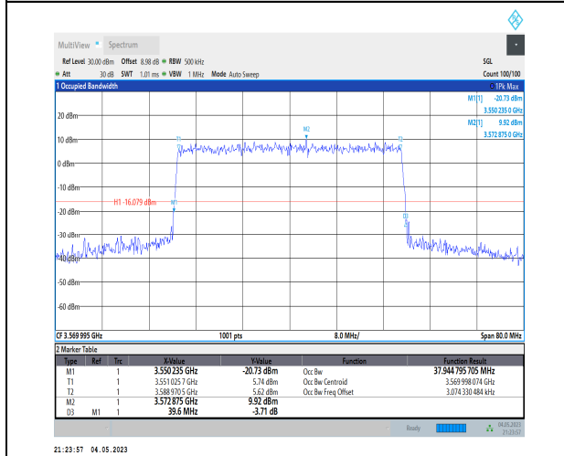
1-N48-PC3-30-40-L-7-CP-16QAM-Outer_Full-106@ 0-Ant1-37.945-39.600-<math>\leq 40</math>-PASS
