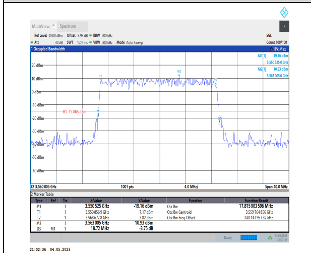
1-N48-PC3-30-20-L-1-DFT-QPSK-Outer_Full-50@0 Ant1-17.816-18.720-≤20-PASS
