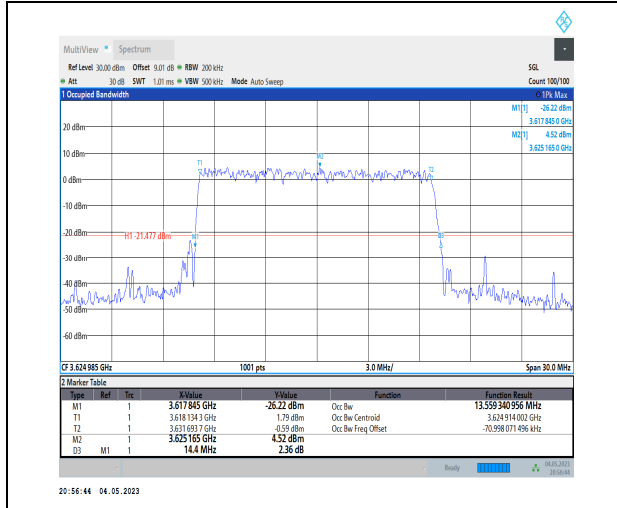
1-N48-PC3-30-15-M-9-CP-256QAM-Outer_Full-38@ @-Ant1-13.559-14.400≤15-PASS
