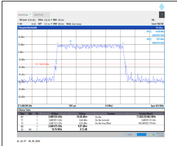
1-N48-PC3-30-20-H-1-DFT-QPSK-Outer_Full-50@0-Ant1-17.82-18.760-≤20-PASS
