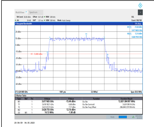
1-N48-PC3-30-15-M-1-DFT-QPSK-Outer_Full-36@0 -Ant1-12.831-14.130-≤15-PASS
