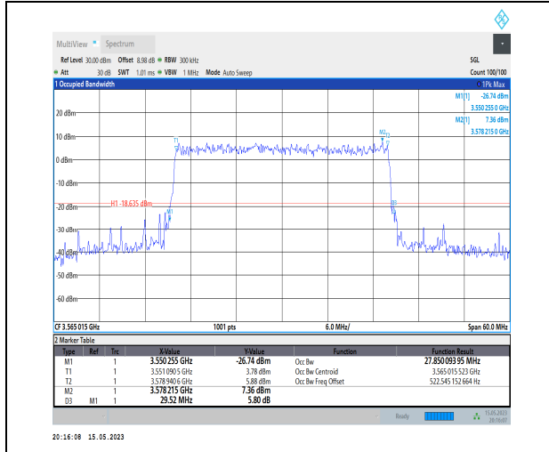
1-N48-PC3-30-30-L-8-CP-64QAM-Outer_Full-78@0-Ant1-27.850-29.520-≤30-PASS
