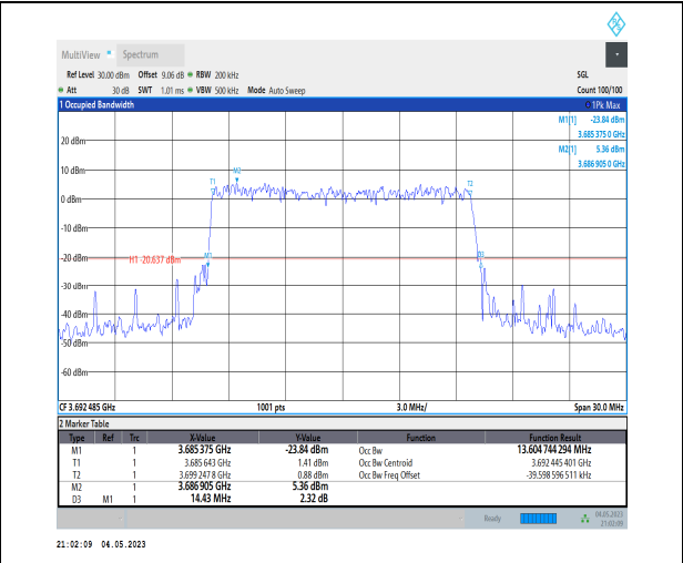
1-N48-PC3-30-15-H-9-CP-256QAM-Outer_Full-38@0 -Ant1-13.605-14.430-≤15-PASS
