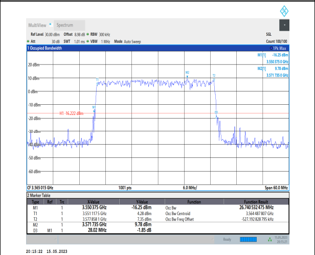
1-N48-PC3-30-30-L-3-DFT-16QAM-Outer_Full-75@ @-Ant1-26.740-28.020-≤30-PASS
