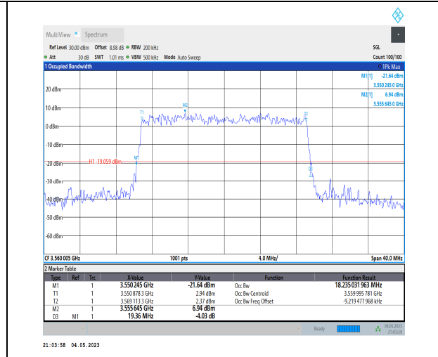
1-N48-PC3-30-20-L-8-CP-64QAM-Outer_Full-51@0- Ant1-18.235-19.360-≤20-PASS
