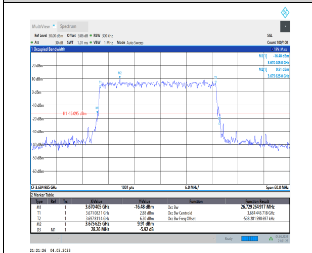
1-N48-PC3-30-30-H-4-DFT-64QAM-Outer_Full-75@ 0-Ant1-26.729-28.260-≤30-PASS
