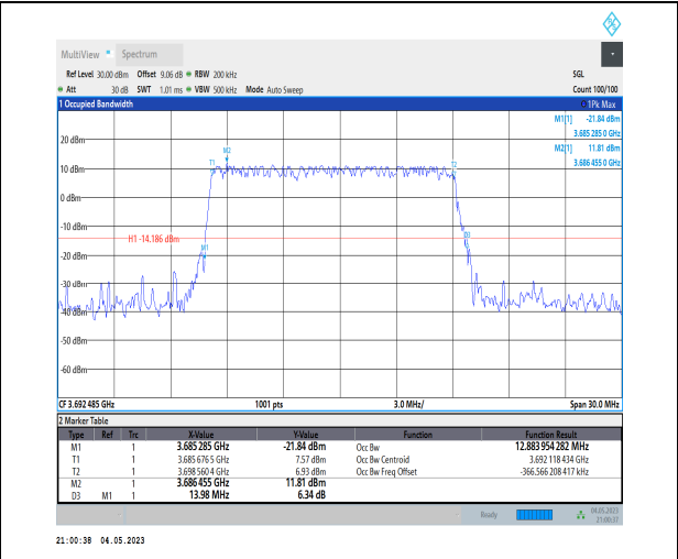
1-N48-PC3-30-15-H-1-DFT-QPSK-Outer_Full-36@ @-Ant1-12.884-13.980≤15-PASS
