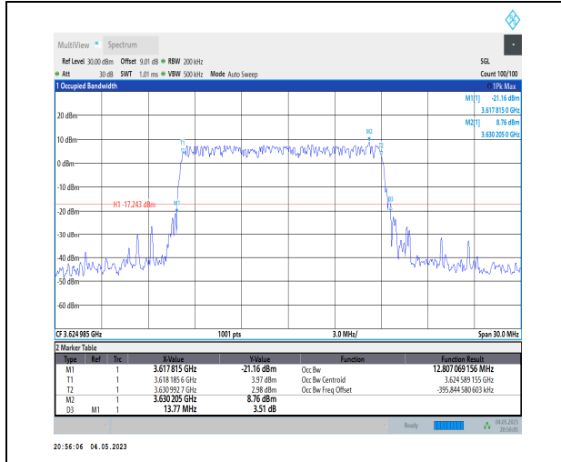
1-N48-PC3-30-15-M-5-DFT-256QAM-Outer_Full-36 @0-Ant1-12.807-13.770-≤15-PASS
