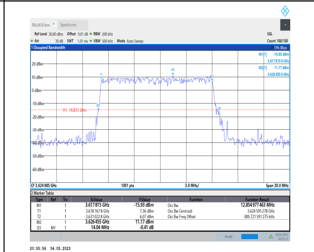
1-N48-PC3-30-15-M-4-DFT-64QAM-Outer_Full-36@0 0-Ant1-12.855-14.040-≤15-PASS
