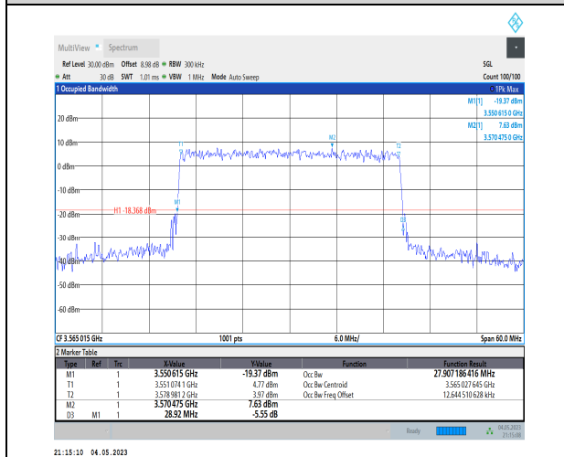
1-N48-PC3-30-30-L-6-CP-QPSK-Outer_Full-78@0-A nt1-27.907-28.920-≤30-PASS
