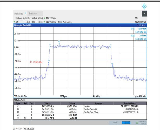
1-N48-PC3-30-20-M-9-CP-256QAM-Outer_Full-51@0- 0-Ant1-18.176-19.120-<20-PASS
