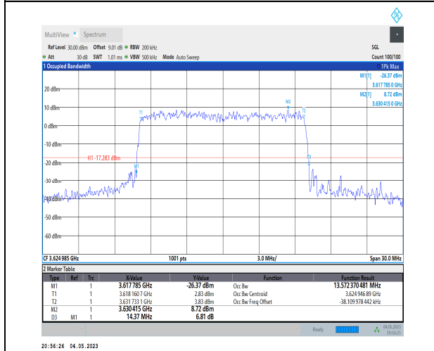
1-N48-PC3-30-15-M-7-CP-16QAM-Outer_Full-38@0 -Ant1-13.572-14.370-≤15-PASS
