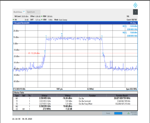
1-N48-PC3-30-30-L-1-DFT-QPSK-Outer_Full-75@0- Ant1-26.822-27.900-≤30-PASS
