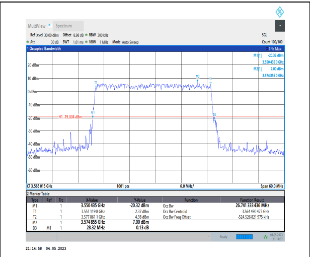
1-N48-PC3-30-30-L-5-DFT-256QAM-Outer_Full-75 @0-Ant1-26.741-28.320-≤30-PASS
