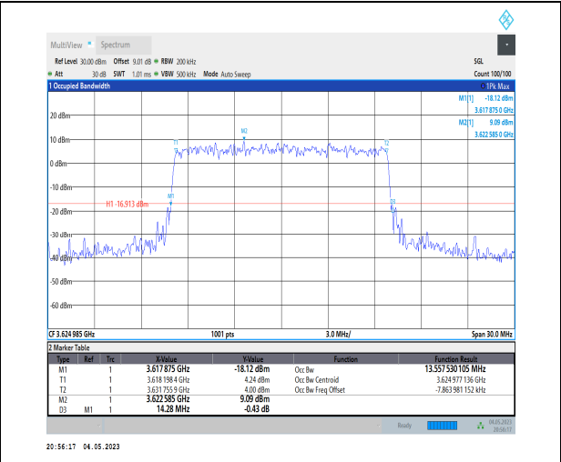
1-N48-PC3-30-15-M-6-CP-QPSK-Outer_Full-38@0- Ant1-13.558-14.280-≤15-PASS
