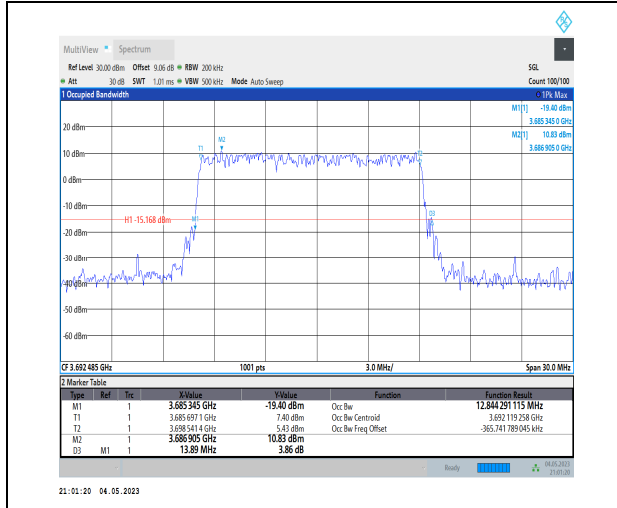
1-N48-PC3-30-15-H-4-DFT-64QAM-Outer_Full-36@ 0-Ant1-12.844-13.890≤15-PASS
