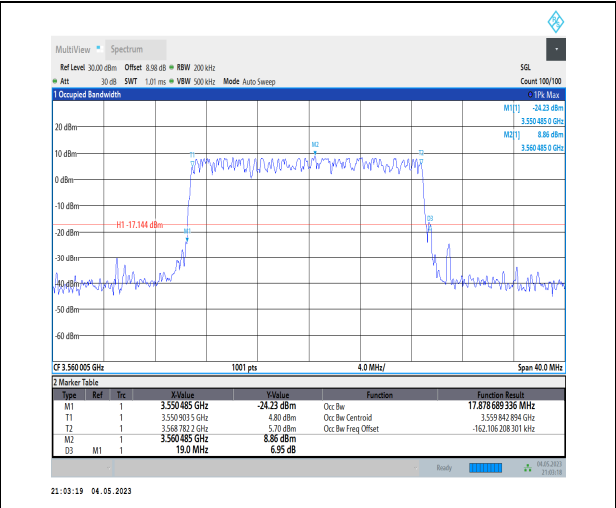
1-N48-PC3-30-20-L-4-DFT-64QAM-Outer_Full-50@ 0-Ant1-17.879-19.000-≤20-PASS
