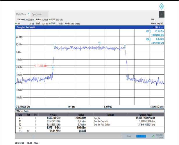
1-N48-PC3-30-40-L-8-CP-64QAM-Outer_Full-106@ 0-Ant1-37.852-39.840-<math>\leq 40</math>-PASS
