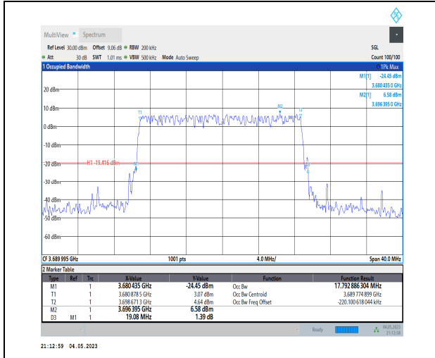
1-N48-PC3-30-20-H-5-DFT-256QAM-Outer_Full-50 @0-Ant1-17.793-19.080-<=20-PASS
