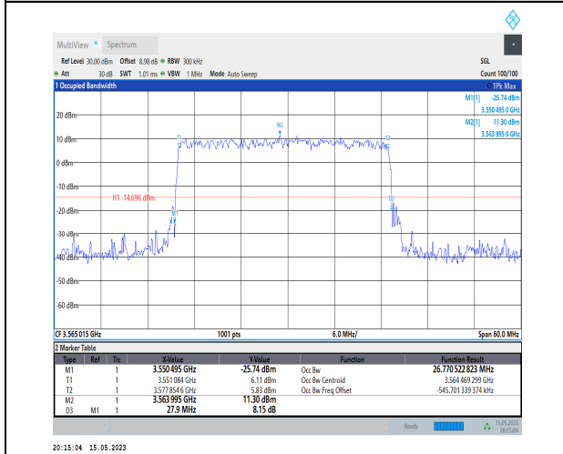
1-N48-PC3-30-30-L-2-DFT-PI2BPSK-Outer_Full-75 @-Ant1-26.770-27.900-≤30-PASS
