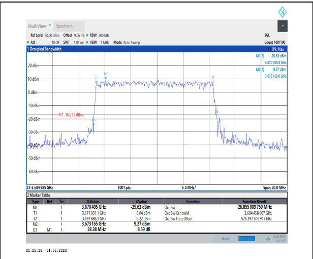
1-N48-PC3-30-30-H-3-DFT-16QAM-Outer_Full-75@ 0-Ant1-26.855-28.380-≤30-PASS
