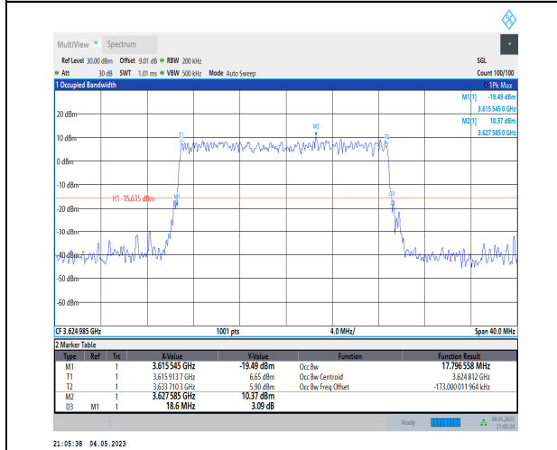
1-N48-PC3-30-20-M-4-DFT-64QAM-Outer_Full-50@ 0-Ant1-17.797-18.600-≤20-PASS
