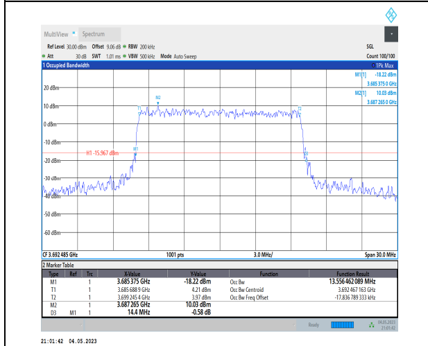
1-N48-PC3-30-15-H-6-CP-QPSK-Outer_Full-38@0- Ant1-13.556-14.400≤15-PASS
