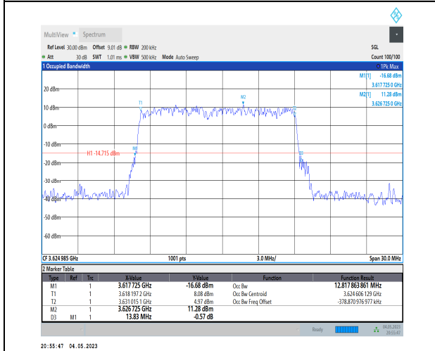
1-N48-PC3-30-15-M-3-DFT-16QAM-Outer_Full-36@0 0-Ant1-12.818-13.830-≤15-PASS
