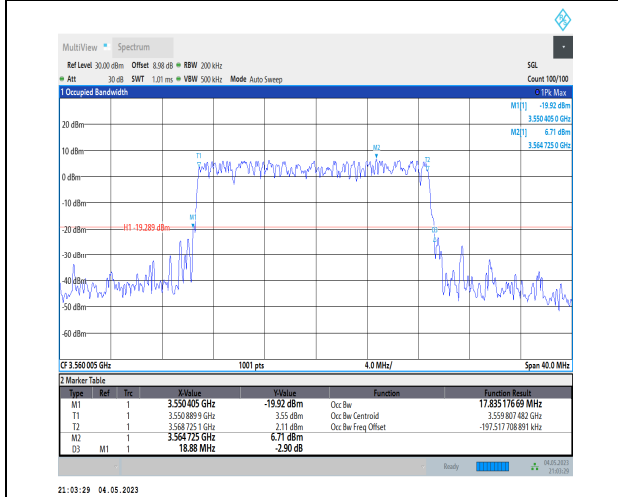
1-N48-PC3-30-20-L-5-DFT-256QAM-Outer_Full-50 @0-Ant1-17.835-18.880-≤20-PASS
