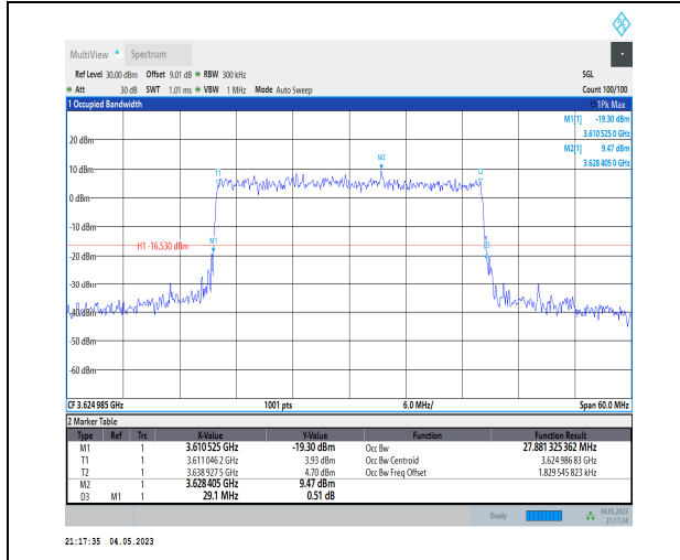
1-N48-PC3-30-30-M-7-CP-16QAM-Outer_Full-78@0 -Ant1-27.881-29.100-≤30-PASS
