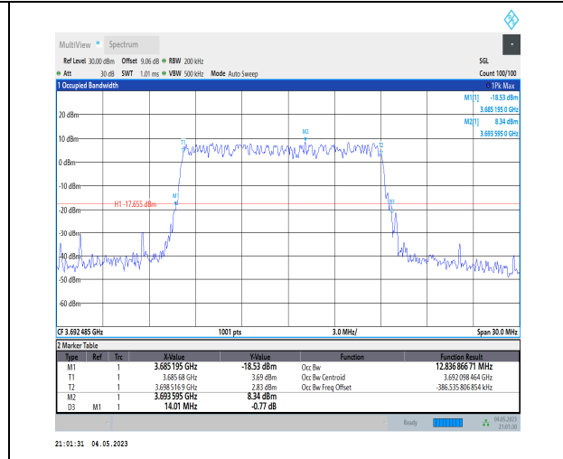
1-N48-PC3-30-15-H-5-DFT-256QAM-Outer_Full-36 @0-Ant1-12.837-14.010≤15-PASS
