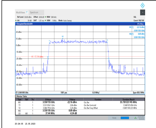
1-N48-PC3-30-40-L-5-DFT-256QAM-Outer_Full-100 @0-Ant1-35.74-37.440-<math>\leq 40</math>-PASS
