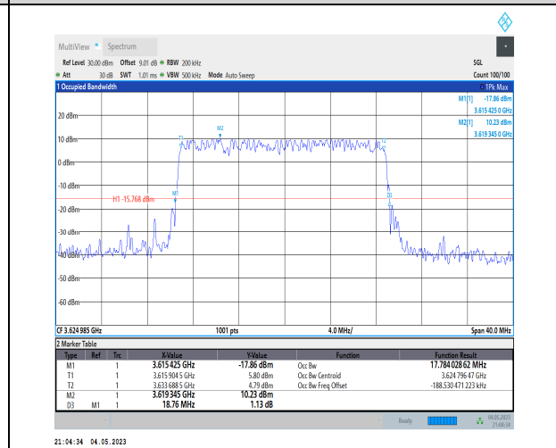
1-N48-PC3-30-20-M-1-DFT-QPSK-Outer_Full-50@0- Ant1-17.784-18.760-≤20-PASS
