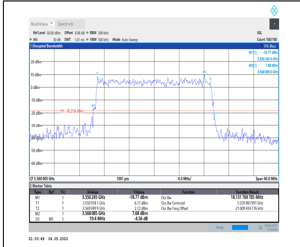
1-N48-PC3-30-20-L-7-CP-16QAM-Outer_Full-51@0- Ant1-18.132-19.400-≤20-PASS
