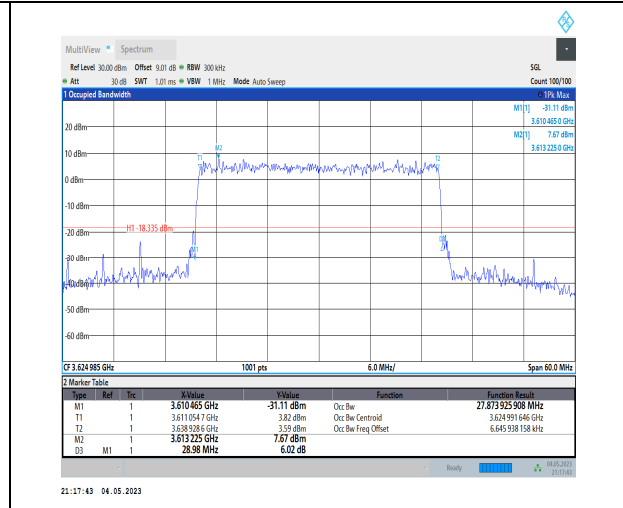
1-N48-PC3-30-30-M-8-CP-64QAM-Outer_Full-78@0 -Ant1-27.874-28.980-≤30-PASS
