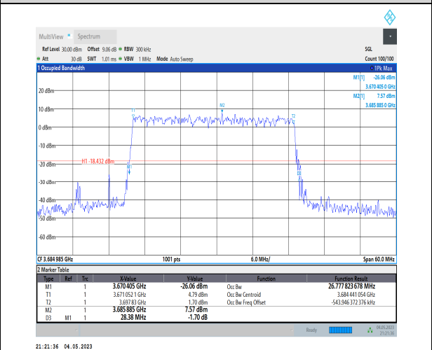
1-N48-PC3-30-30-H-5-DFT-256QAM-Outer_Full-75 @0-Ant1-26.778-28.380-≤30-PASS
