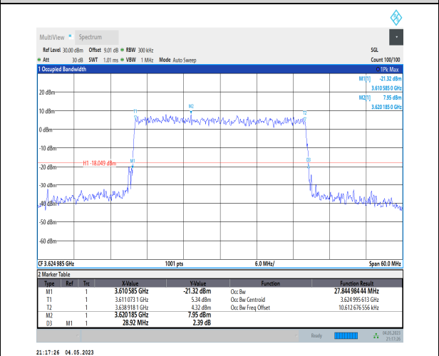
1-N48-PC3-30-30-M-6-CP-QPSK-Outer_Full-78@0- Ant1-27.845-28.920-≤30-PASS
