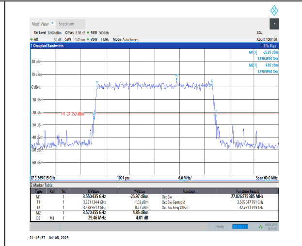
1-N48-PC3-30-30-L-9-CP-256QAM-Outer_Full-78@0-Ant1-27.827-29.460-≤30-PASS
