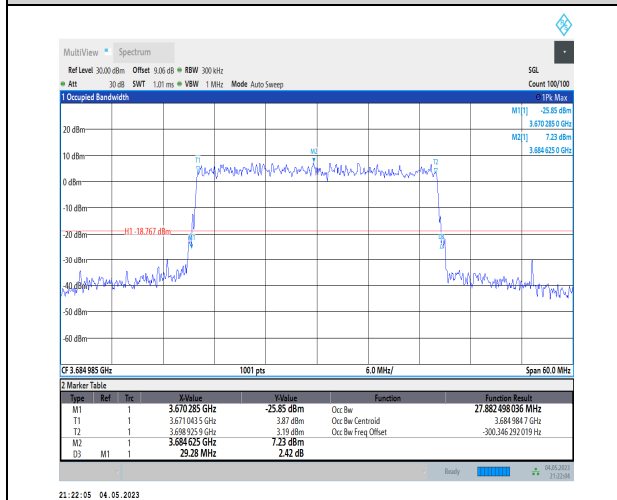
1-N48-PC3-30-30-H-8-CP-64QAM-Outer_Full-78@0- -Ant1-27.882-29.280-<math>\leq 30</math>-PASS
