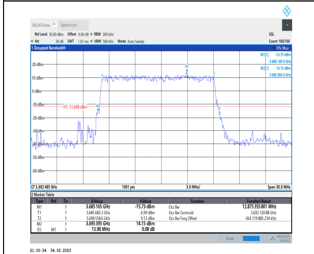
1-N48-PC3-30-15-H-2-DFT-PI2BPSK-Outer_Full-36@ @-Ant1-12.875-13.980≤15-PASS
