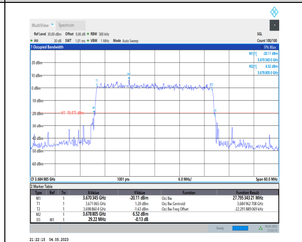
1-N48-PC3-30-30-H-9-CP-256QAM-Outer_Full-78@0- 0-Ant1-27.795-29.220-<math>\leq 30</math>-PASS
