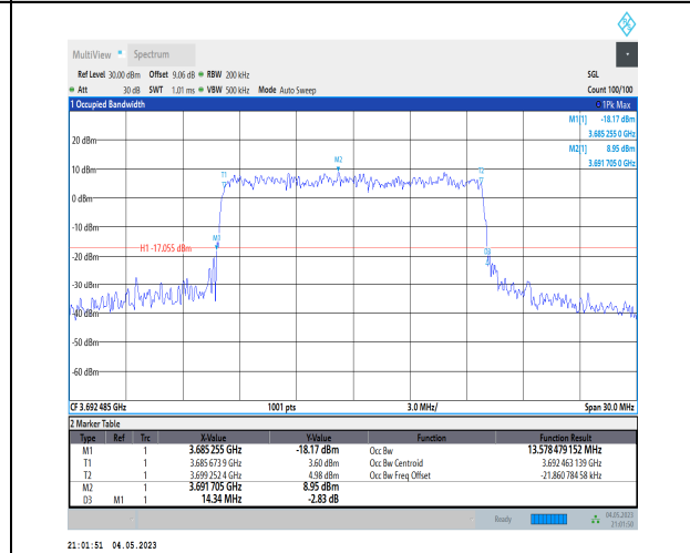
1-N48-PC3-30-15-H-7-CP-16QAM-Outer_Full-38@0 -Ant1-13.578-14.340≤15-PASS
