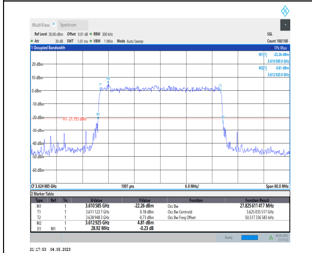
1-N48-PC3-30-30-M-9-CP-256QAM-Outer_Full-78@0 -Ant1-27.826-28.920-≤30-PASS
