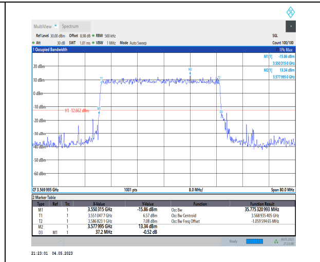
1-N48-PC3-30-40-L-2-DFT-PI2BPSK-Outer_Full-100 @0-Ant1-35.775-37.200-≤40-PASS
