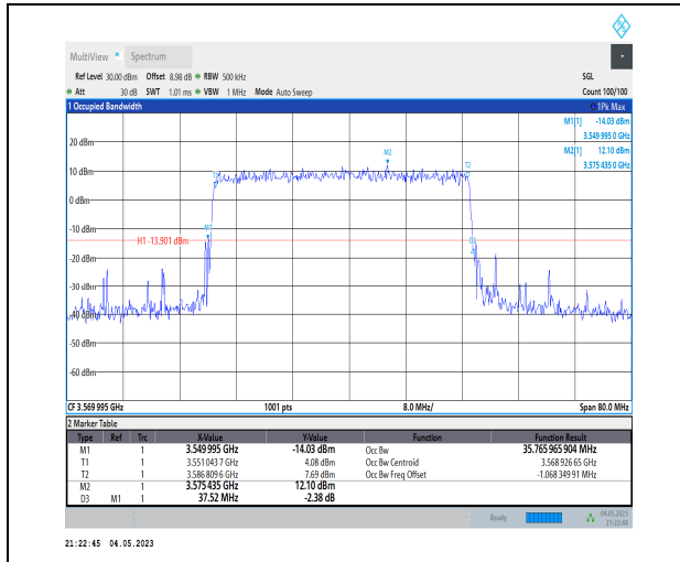
1-N48-PC3-30-40-L-1-DFT-QPSK-Outer_Full-100@0 -Ant1-35.766-37.520-≤40-PASS
