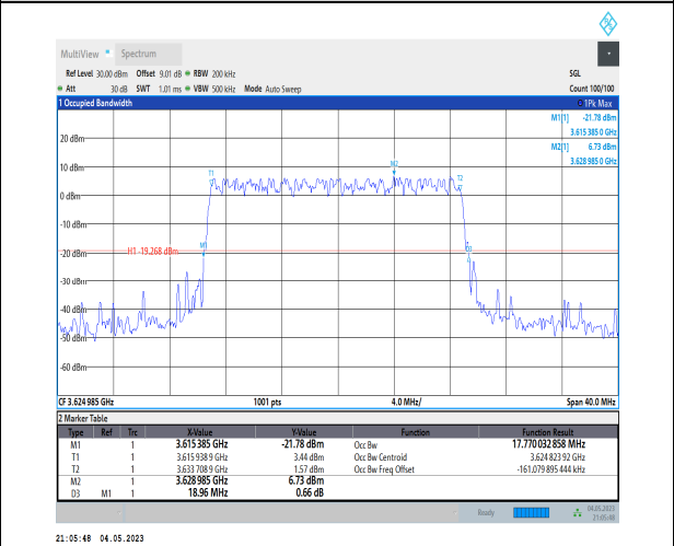
1-N48-PC3-30-20-M-5-DFT-256QAM-Outer_Full-50 @0-Ant1-17.77-18.960-≤20-PASS
