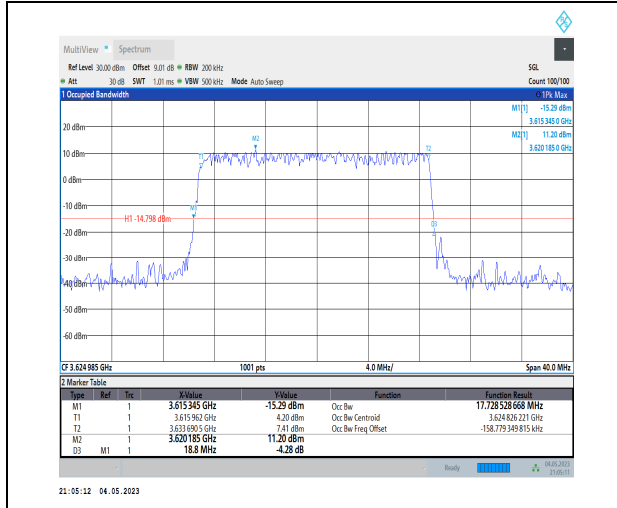
1-N48-PC3-30-20-M-2-DFT-PI2BPSK-Outer_Full-50 @0-Ant1-17.729-18.800-≤20-PASS
