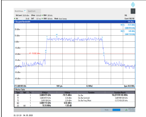
1-N48-PC3-30-20-H-7-CP-16QAM-Outer_Full-51@0 -Ant1-18.237-19.160-<=20-PASS
