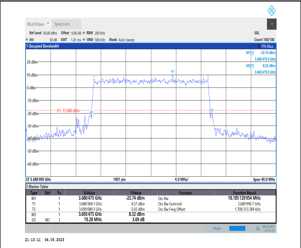
1-N48-PC3-30-20-H-6-CP-QPSK-Outer_Full-51@0- Ant1-18.185-19.280-<=20-PASS
