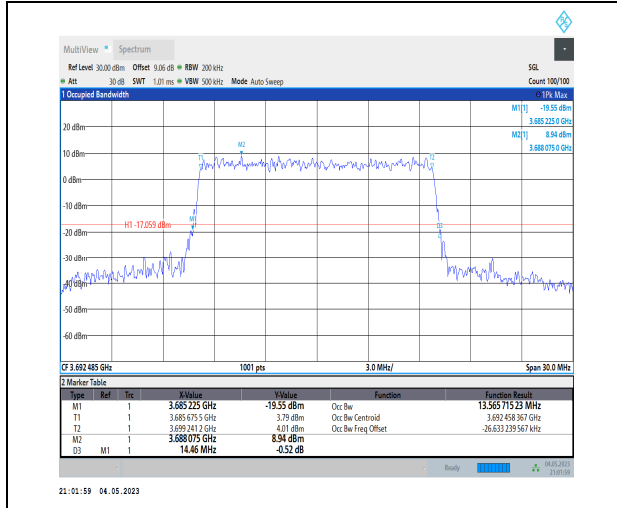
1-N48-PC3-30-15-H-8-CP-64QAM-Outer_Full-38@0 -Ant1-13.566-14.460-≤15-PASS
