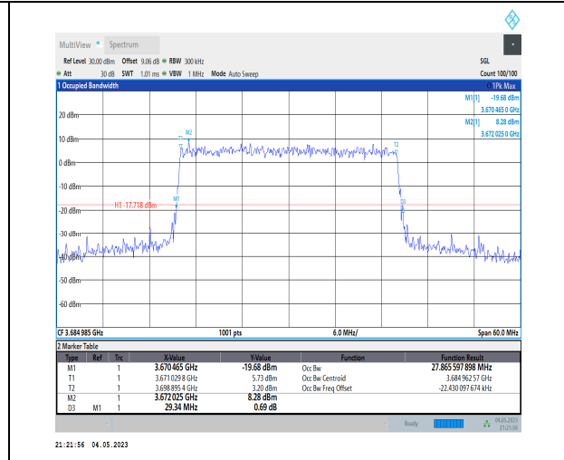
1-N48-PC3-30-30-H-7-CP-16QAM-Outer_Full-78@0- -Ant1-27.866-29.340-<math>\leq 30</math>-PASS
