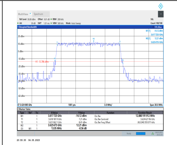
1-N48-PC3-30-15-M-2-DFT-PI2BPSK-Outer_Full-36 @0-Ant1-12.88-13.950-≤15-PASS
