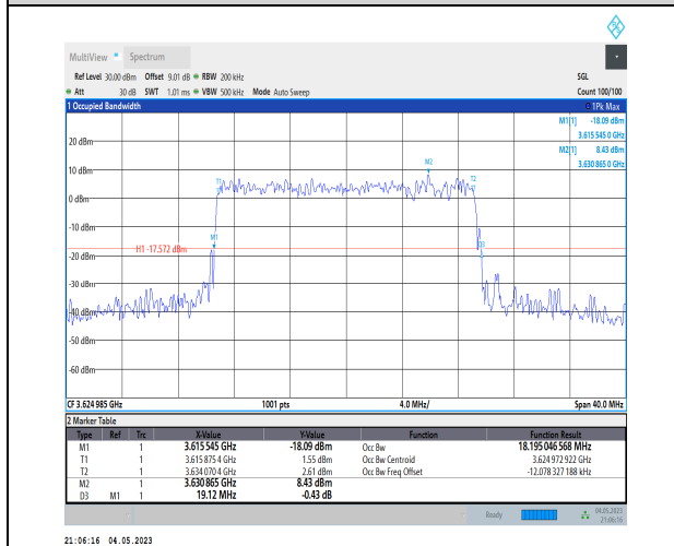
1-N48-PC3-30-20-M-8-CP-64QAM-Outer_Full-51@0- -Ant1-18.195-19.120-<20-PASS
