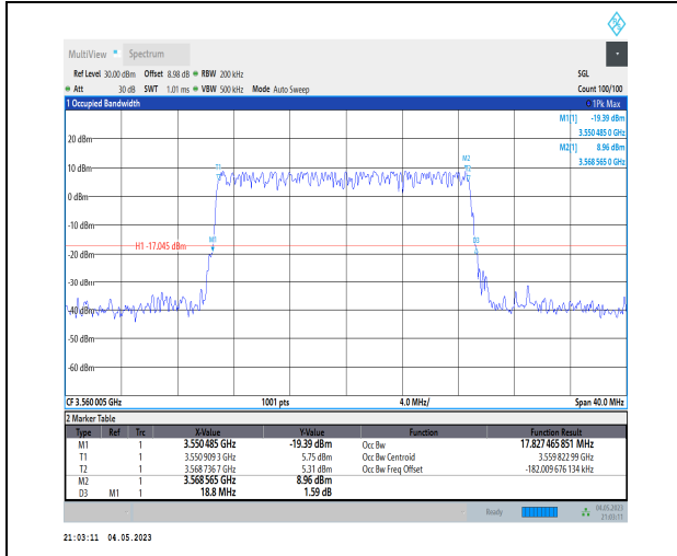
1-N48-PC3-30-20-L-3-DFT-16QAM-Outer_Full-50@ 0-Ant1-17.827-18.800-≤20-PASS
