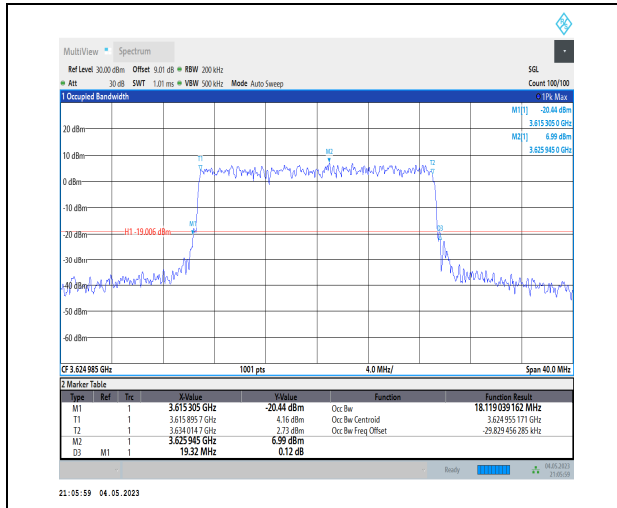
1-N48-PC3-30-20-M-6-CP-QPSK-Outer_Full-51@0- Ant1-18.119-19.320-<20-PASS
