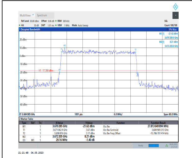
1-N48-PC3-30-30-H-6-CP-QPSK-Outer_Full-78@0- Ant1-27.814-29.160-<math>\leq 30</math>-PASS
