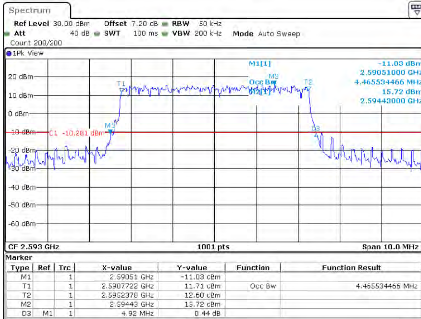
Band41-5MHz-QPSK-40620-25RB#0-4.466
