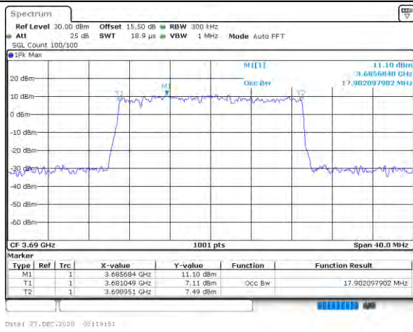
Highest Channel / 20MHz / QPSK
