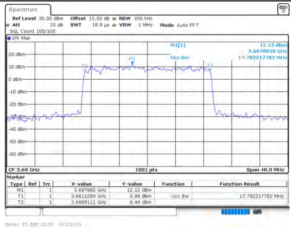
Highest Channel / 20MHz / 16QAM
