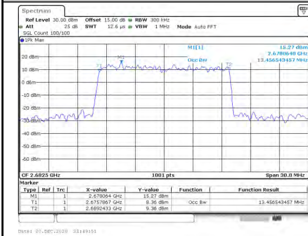
Middle Channel / 15MHz / 64QAM
