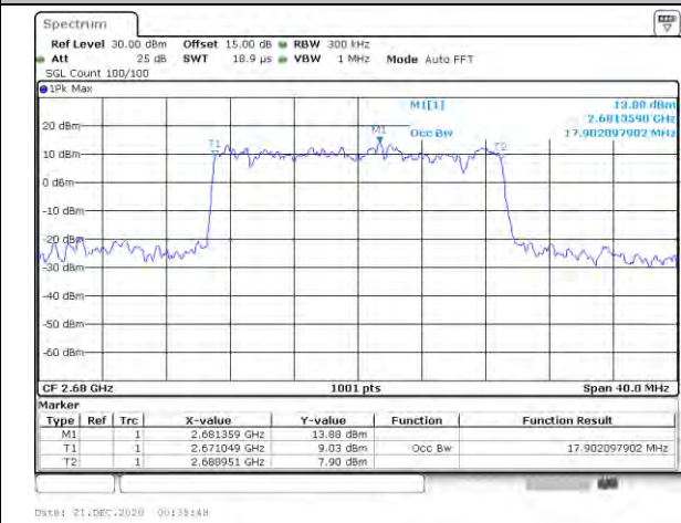
Middle Channel / 20MHz / 64QAM
