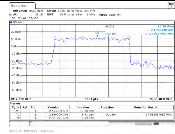
Highest Channel / 20MHz / 64QAM
