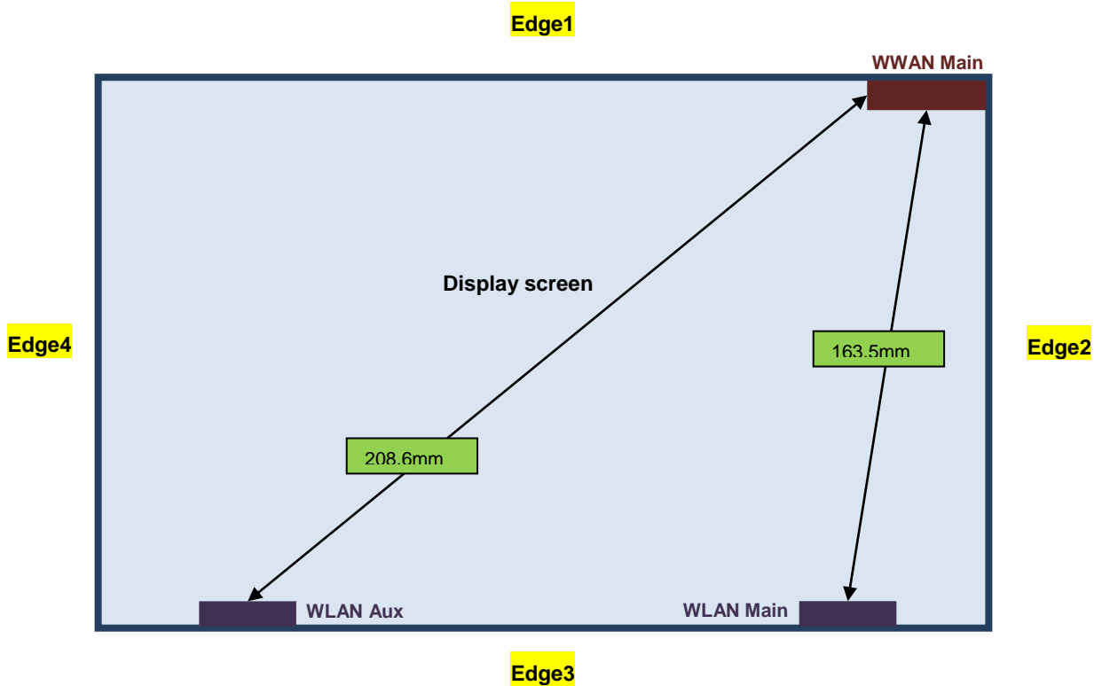
Front View
