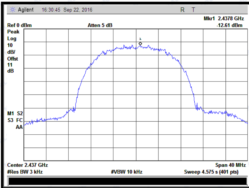
(Channel = 6 @ 802.11b)
