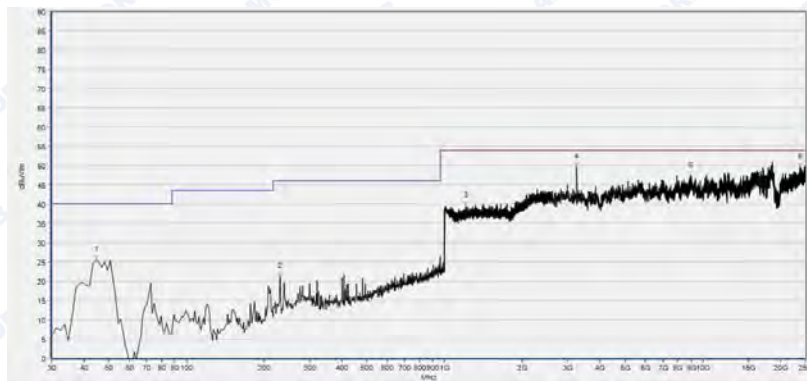
(Antenna Horizontal, 30MHz to 25GHz)
