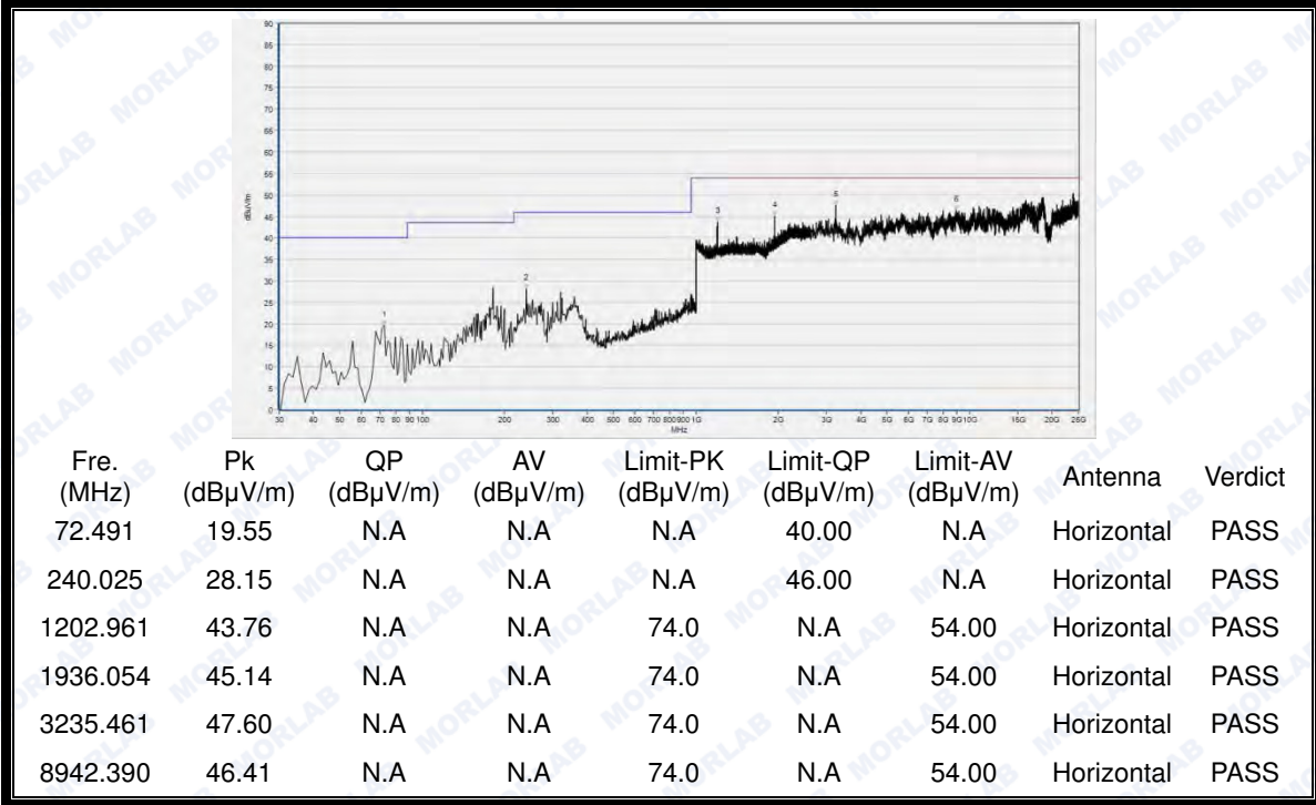
(30MHz to 25GHz, Antenna Horizontal @8-DPSK, channel 0)
