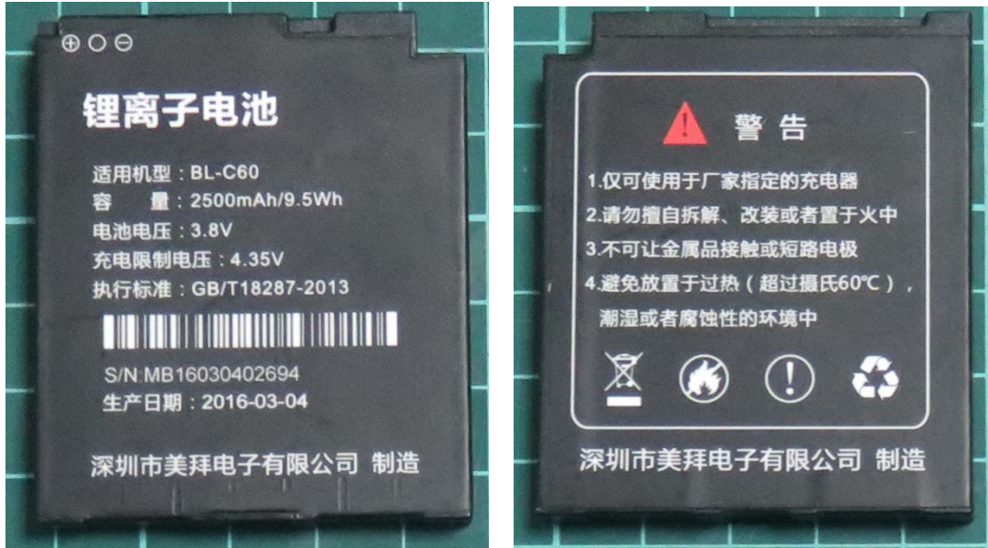
b: Battery
