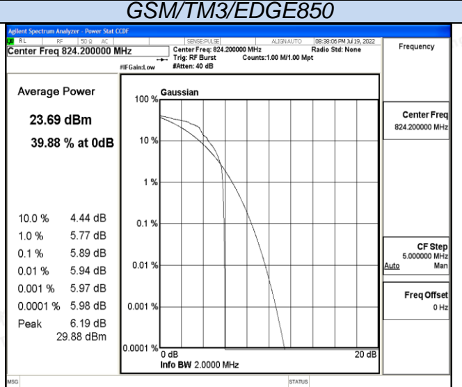
Channel 128 / 824.2 MHz
