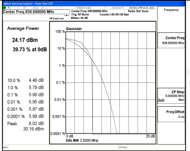
Channel 190 / 836.6 MHz
