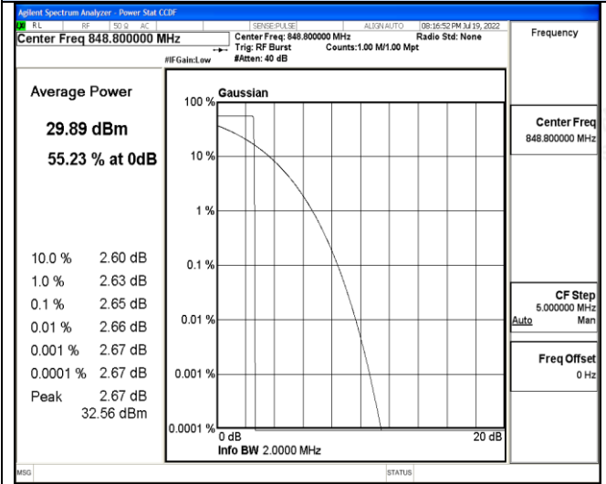
Channel 251 / 848.8 MHz
