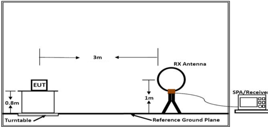
Below 30MHz
