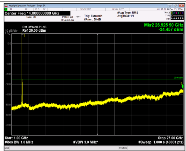
38-38-20MHz-20MHz-16QAM-16QAM-37850-38048-1RB#0-0RB#0-1000~27000MHz-PASS
