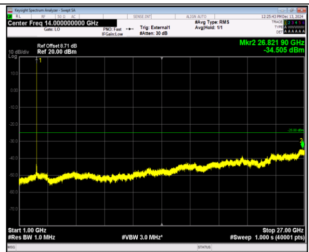
38-38-15MHz-15MHz-16QAM-16QAM-38025-38175-1RB# 74-0RB#0-1000~27000MHz-PASS
