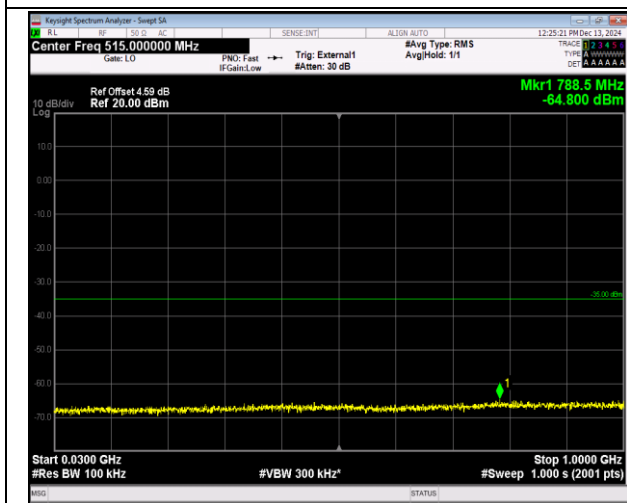
38-38-15MHz-15MHz-16QAM-16QAM-38025-38175-1RB #74-0RB#0-30~1000MHz-PASS
