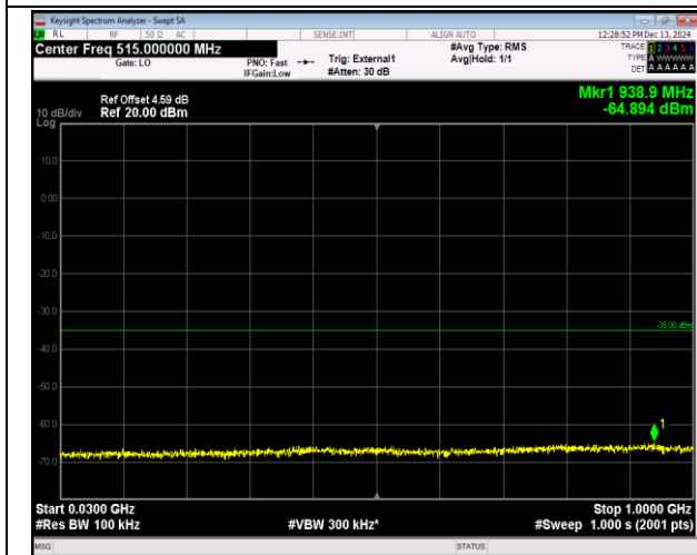
38-38-15MHz-15MHz-16QAM-16QAM-38025-38175-75R B#0-75RB#0-30~1000MHz-PASS
