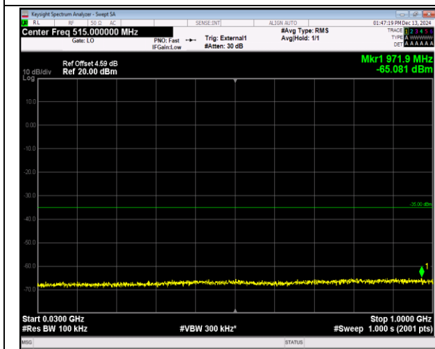
38-38-20MHz-20MHz-16QAM-16QAM-37901-38099-1RB #0-1RB#99-30~1000MHz-PASS
