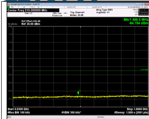
38-38-20MHz-20MHz-16QAM-16QAM-37901-38099-1RB #0-ORB#0-30~1000MHz-PASS
