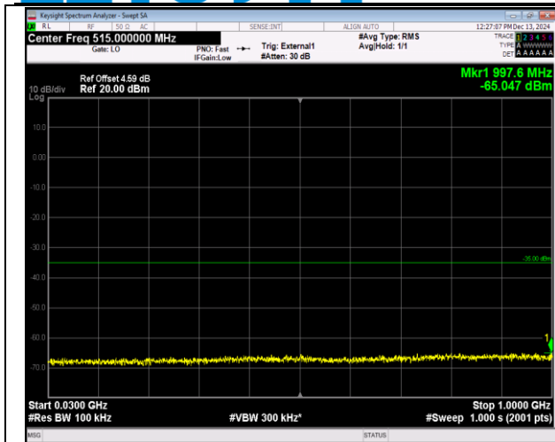
38-38-15MHz-15MHz-16QAM-16QAM-38025-38175-1RB #0-1RB#74-30~1000MHz-PASS
