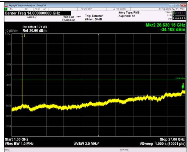
38-38-20MHz-20MHz-16QAM-16QAM-37850-38048-1RB# 99-0RB#0-1000~27000MHz-PASS
