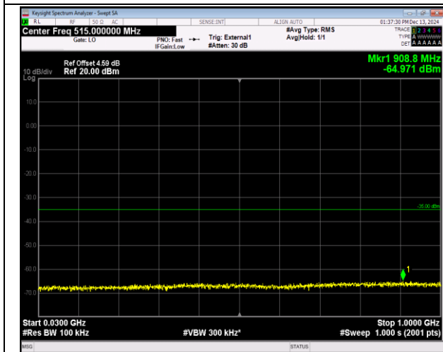
38-38-20MHz-20MHz-QPSK-QPSK-37850-38048-1RB#9 9-ORB#0-30~1000MHz-PASS
