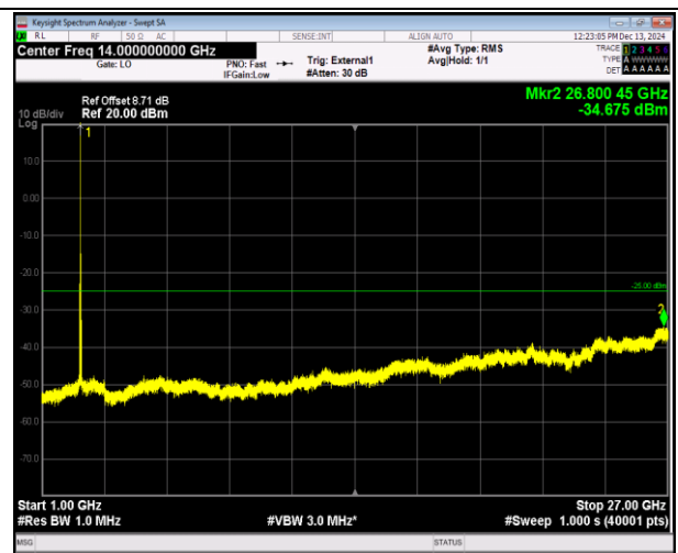
38-38-15MHz-15MHz-QPSK-QPSK-38025-38175-1RB#0-0 RB#0-1000~27000MHz-PASS
