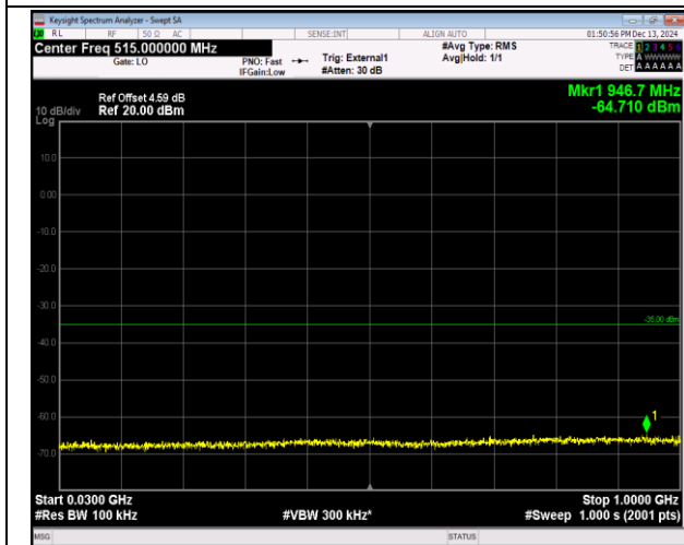
38-38-20MHz-20MHz-16QAM-16QAM-37952-38150-1RB #0-ORB#0-30~1000MHz-PASS
