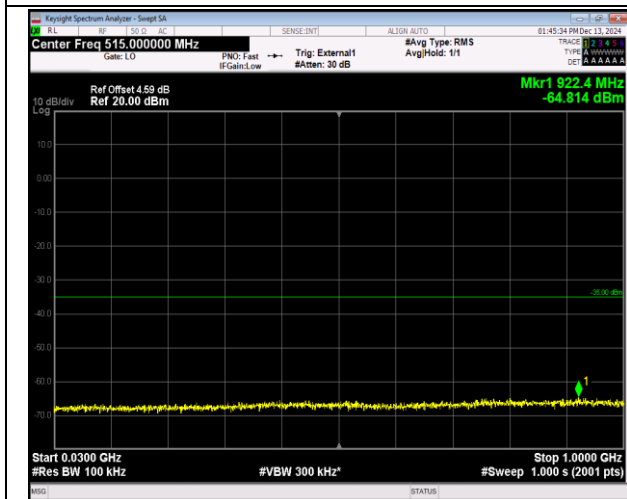
38-38-20MHz-20MHz-16QAM-16QAM-37901-38099-1RB #99-ORB#0-30~1000MHz-PASS
