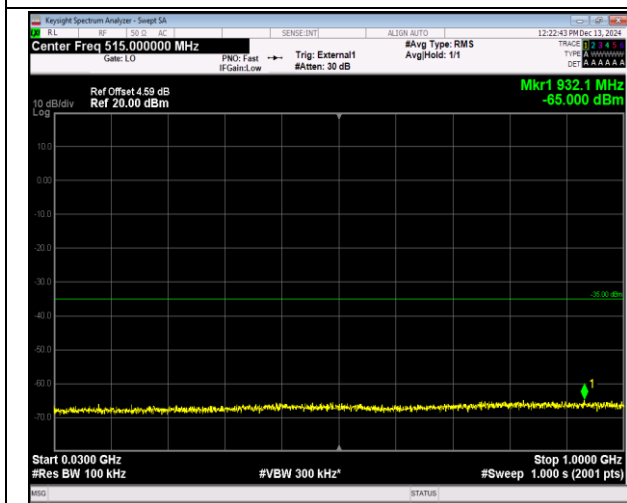
38-38-15MHz-15MHz-QPSK-QPSK-38025-38175-1RB#0- ORB#0-30~1000MHz-PASS
