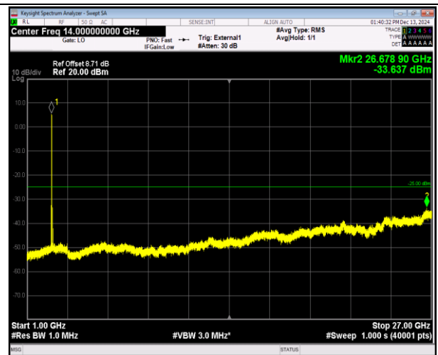
38-38-20MHz-20MHz-16QAM-16QAM-37850-38048-1RB#0-1RB#99-1000~27000MHz-PASS
