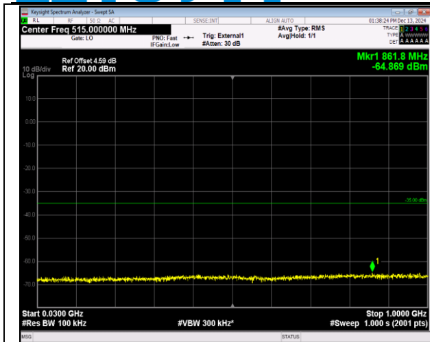
38-38-20MHz-20MHz-16QAM-16QAM-37850-38048-1RB #99-0RB#0-30~1000MHz-PASS
