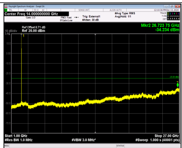
38-38-15MHz-15MHz-QPSK-QPSK-37825-37975-1RB#74- ORB#0-1000~27000MHz-PASS
