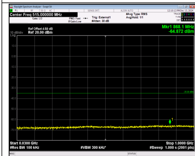
38-38-15MHz-15MHz-QPSK-QPSK-37825-37975-1RB#7 4-ORB#0-30~1000MHz-PASS
