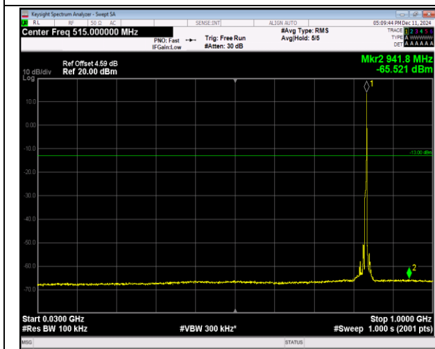
5-5-5MHz-3MHz-QPSK-QPSK-20510-20549-1RB#24-0RB B#0-30~1000MHz-PASS
