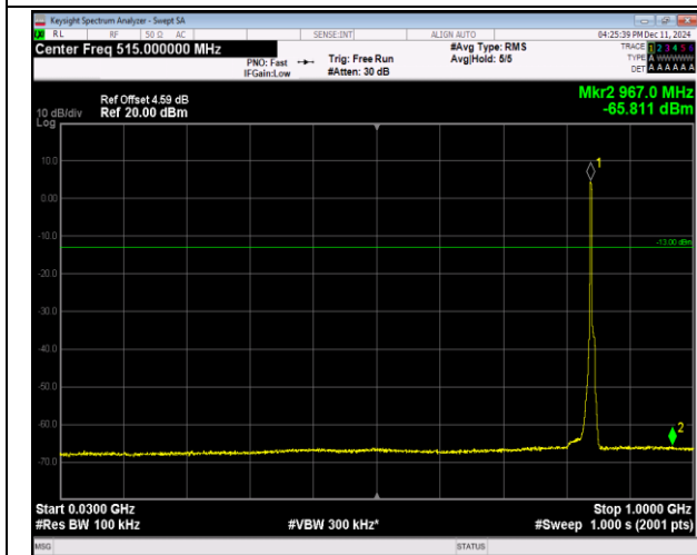
5-5-3MHz-5MHz-16QAM-16QAM-20586-20625-15RB#0- 25RB#0-30~1000MHz-PASS
