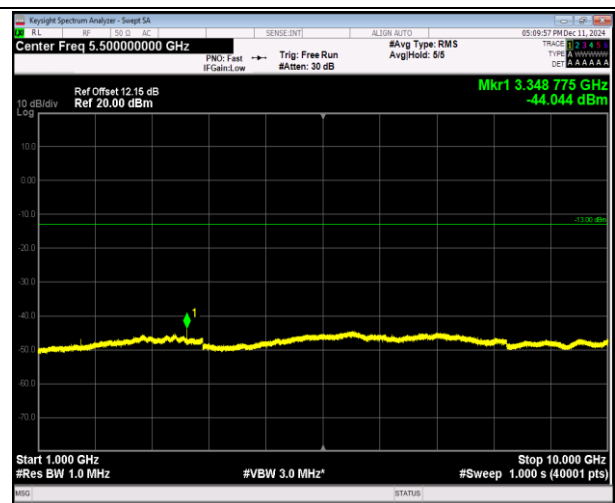
5-5-5MHz-3MHz-QPSK-QPSK-20510-20549-1RB#24-0RB#1 0-1000~10000MHz-PASS
