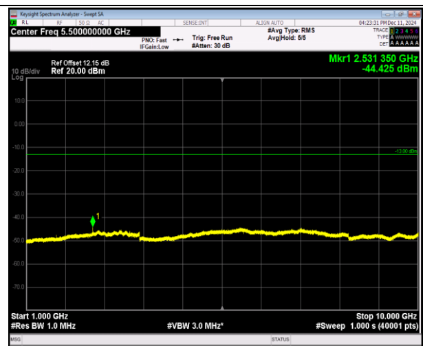
5-5-3MHz-5MHz-16QAM-16QAM-20586-20625-1RB#14-0R B#0-1000~10000MHz-PASS
