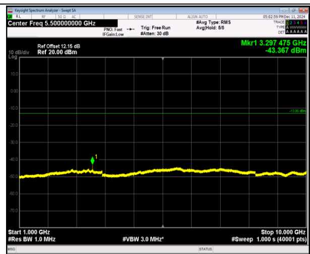
5-5-5MHz-3MHz-16QAM-16QAM-20425-20464-1RB#0-0R B#0-1000~10000MHz-PASS
