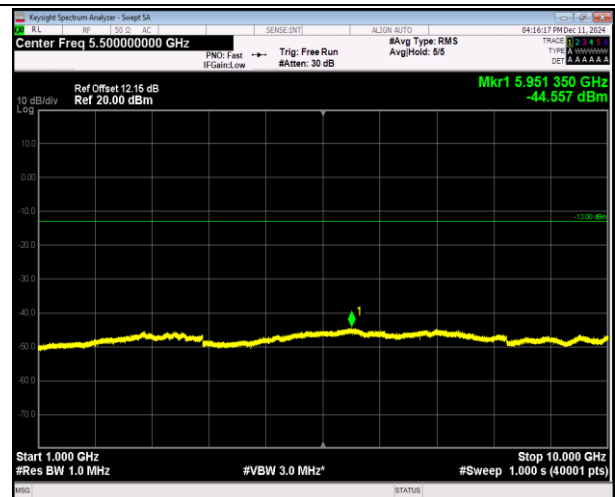
5-5-3MHz-5MHz-16QAM-16QAM-20416-20455-15RB#0-25RB#0-1000~10000MHz-PASS
