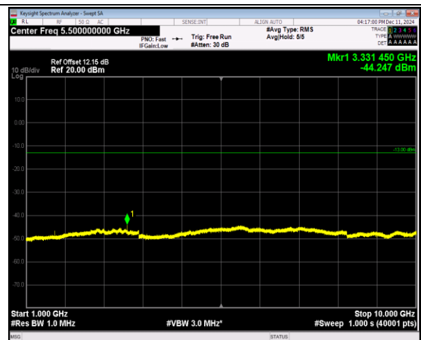
5-5-3MHz-5MHz-QPSK-QPSK-20501-20540-1RB#0-ORB#0-1000~10000MHz-PASS
