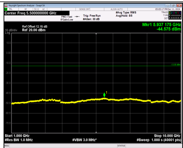
5-5-5MHz-3MHz-16QAM-16QAM-20425-20464-1RB#0-1R B#15-1000~10000MHz-PASS
