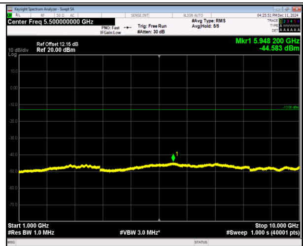
5-5-3MHz-5MHz-16QAM-16QAM-20586-20625-15RB#0-25 RB#0-1000~10000MHz-PASS
