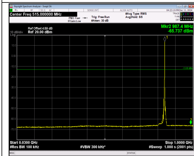
5-5-3MHz-5MHz-16QAM-16QAM-20586-20625-1RB#14- ORB#0-30~1000MHz-PASS
