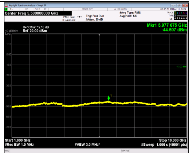
5-5-5MHz-3MHz-QPSK-QPSK-20425-20464-25RB#0-15RB #0-1000~10000MHz-PASS
