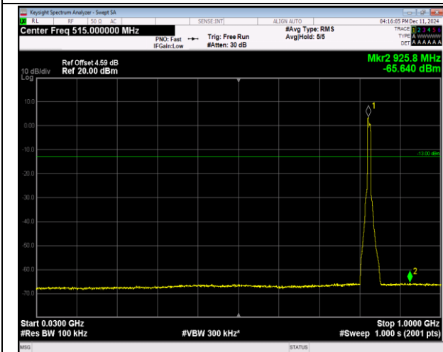
5-5-3MHz-5MHz-16QAM-16QAM-20416-20455-15RB#0-25RB#0-30~1000MHz-PASS
