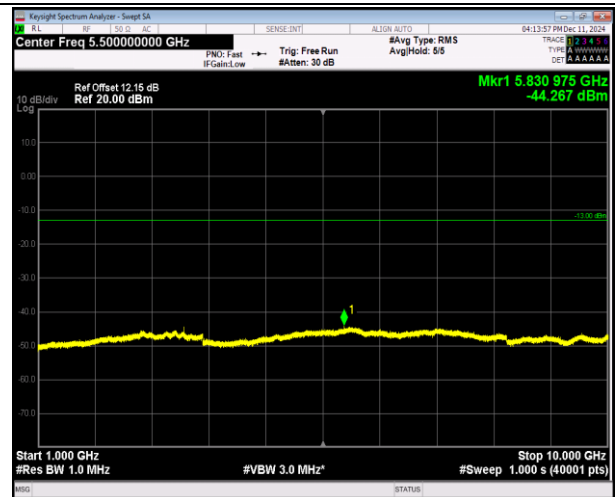
5-5-3MHz-5MHz-16QAM-16QAM-20416-20455-1RB#14-ORB#0-1000~10000MHz-PASS
