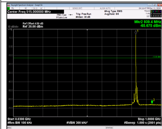
5-5-3MHz-5MHz-QPSK-QPSK-20501-20540-1RB#0-ORB#0-30~1000MHz-PASS
