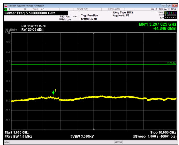
5-5-3MHz-5MHz-QPSK-QPSK-20416-20455-1RB#0-0RB#0 -1000~10000MHz-PASS
