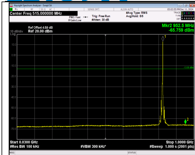
5-5-5MHz-3MHz-16QAM-16QAM-20425-20464-1RB#24- ORB#0-30~1000MHz-PASS
