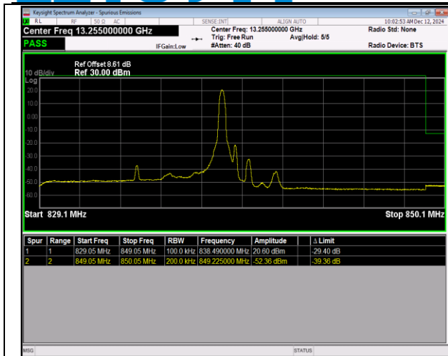
5-5-10MHz-10MHz-QPSK@QPSK-QPSK@QPSK-20501-20600-1RB#49@50RB#0-0RB#0@50RB#0-PASS
