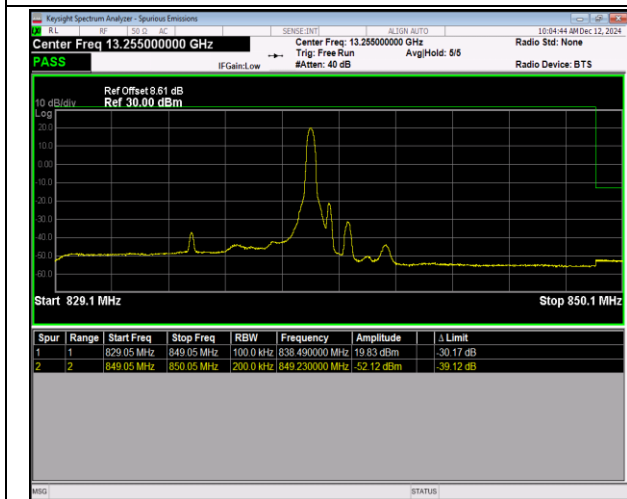
5-5-10MHz-10MHz-16QAM@16QAM-16QAM@16QAM-20501-20600-1RB#49@50RB#0-0RB#0@50RB#0-PASS
