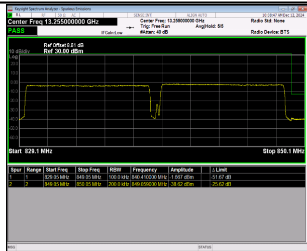
5-5-10MHz-10MHz-QPSK@QPSK-QPSK@QPSK-20501-20600-50RB#0@50RB#0-50RB#0@50RB#0-PASS
