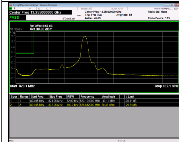
5-5-3MHz-5MHz-QPSK@QPSK-QPSK-20416-20 455-1RB#14@15RB#0-0RB#0@25RB#0-PASS
