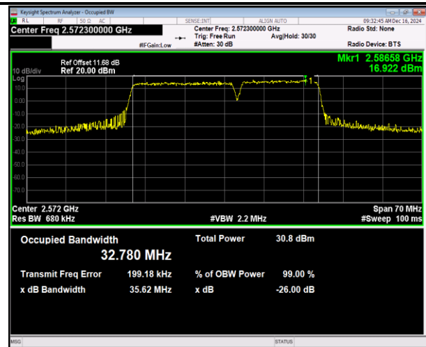
41(2555-2655)-41(2555-2655)-20MHz-15MHz-16QAM-16Q AM-40340-40511-100RB#0-75RB#0-PASS
