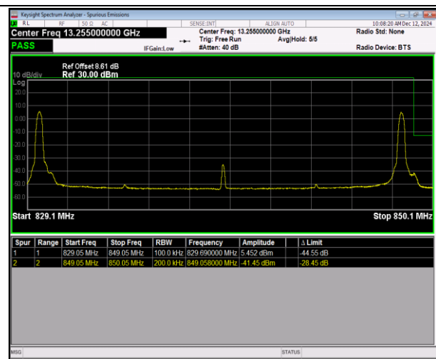
5-5-10MHz-10MHz-16QAM@16QAM-16QAM@16QAM-20501-20600-1RB#0@50RB#0-1RB#49@50RB#0-PASS
