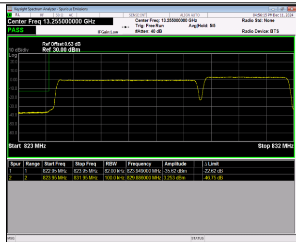
5-5-5MHz-3MHz-16QAM@16QAM-16QAM@16QAM-2042 5-20464-25RB#0@25RB#0-15RB#0@15RB#0-PASS
