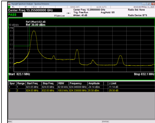
5-5-3MHz-5MHz-QPSK@QPSK-QPSK-20416-20 455-1RB#0@15RB#0-0RB#0@25RB#0-PASS
