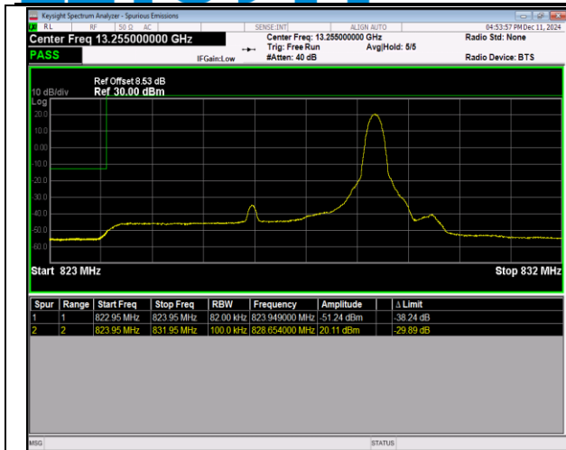
5-5-5MHz-3MHz-QPSK@QPSK-QPSK@QPSK-20425-20 464-1RB#24@25RB#0-0RB#0@15RB#0-PASS
