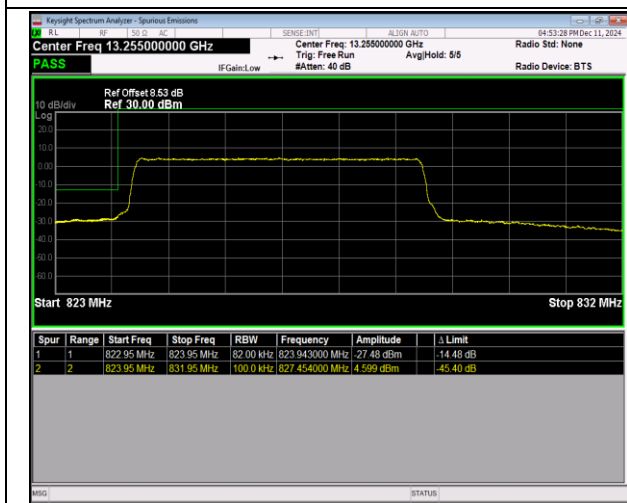
5-5-5MHz-3MHz-16QAM@16QAM-16QAM@16QAM-204 25-20464-1RB#0@25RB#0-0RB#0@15RB#0-PASS
