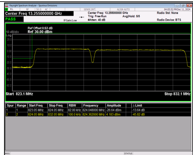
5-5-3MHz-5MHz-QPSK@QPSK-QPSK-20416-204 55-15RB#0@15RB#0-25RB#0@25RB#0-PASS
