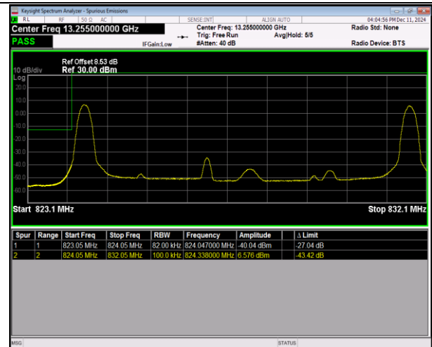
5-5-3MHz-5MHz-QPSK@QPSK-QPSK-20416-204 55-1RB#0@15RB#0-1RB#24@25RB#0-PASS
