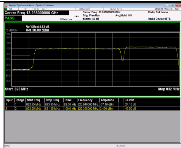
5-5-5MHz-3MHz-QPSK@QPSK-QPSK@QPSK-20425-204 64-25RB#0@25RB#0-15RB#0@15RB#0-PASS
