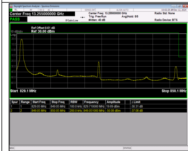
5-5-10MHz-10MHz-16QAM@16QAM-16QAM@16QAM-20501-20600-1RB#0@50RB#0-0RB#0@50RB#0-PASS
