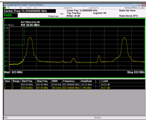
5-5-5MHz-3MHz-16QAM@16QAM-16QAM@16QAM-2042 5-20464-1RB#0@25RB#0-1RB#15@15RB#0-PASS
