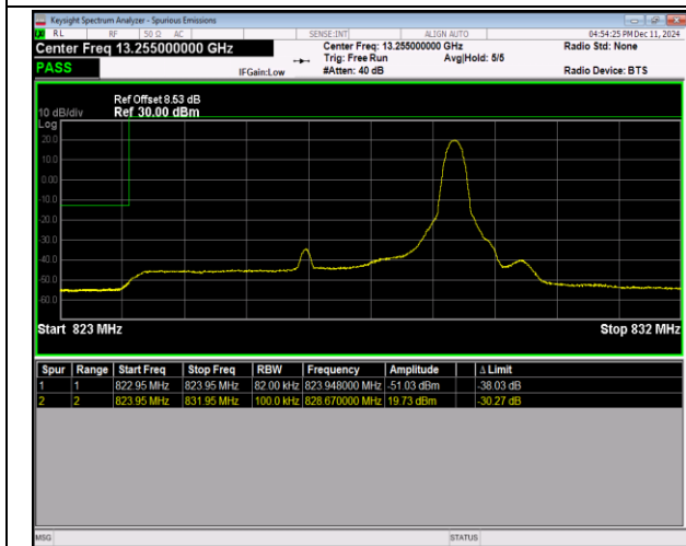
5-5-5MHz-3MHz-16QAM@16QAM-16QAM@16QAM-204 25-20464-1RB#24@25RB#0-0RB#0@15RB#0-PASS
