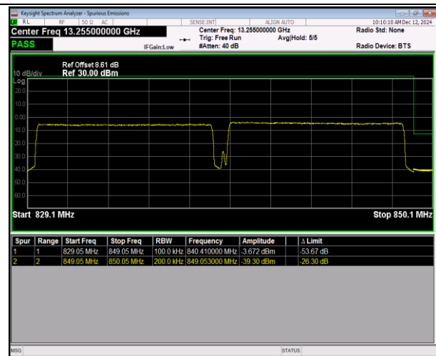
5-5-10MHz-10MHz-16QAM@16QAM-16QAM@16QAM-20501-20600-50RB#0@50RB#0-50RB#0@50RB#0-PASS
