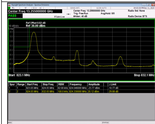
5-5-3MHz-5MHz-16QAM@16QAM-16QAM-204
