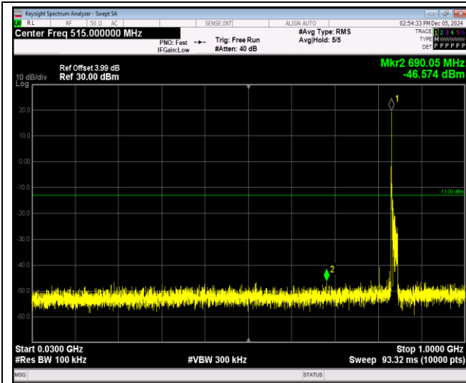
Band38-5MHz-QPSK-37775-1RB#0-Range1:30~100 0MHz
