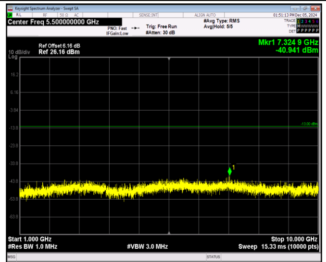
Band26-1.4MHz-16QAM-26697-1RB#0-Range2:1000~10000MHz
