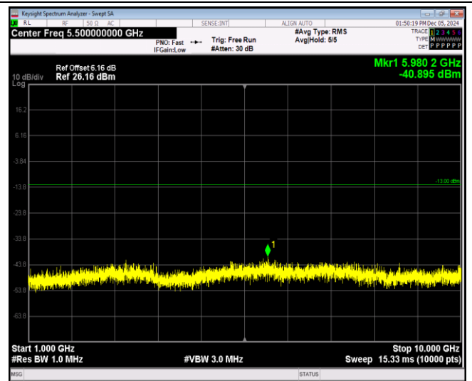
Band26-1.4MHz-QPSK-27033-1RB#0-Range2:1000~10000MHz
