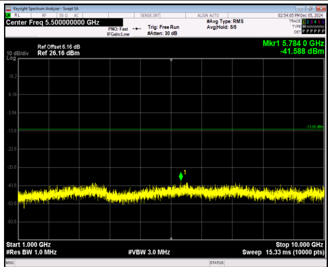
Band26-15MHz-16QAM-26865-1RB#0-Range2:1000~10000MHz
