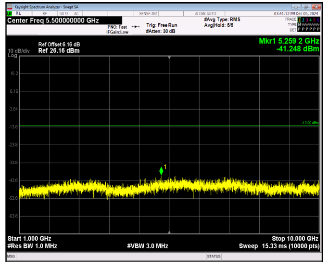
Band26-1.4MHz-64QAM-26740-1RB#0-Range2:1000 ~10000MHz
