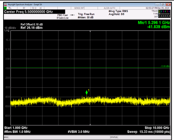
Band26-15MHz-16QAM-26965-1RB#0-Range2:1000 ~10000MHz
