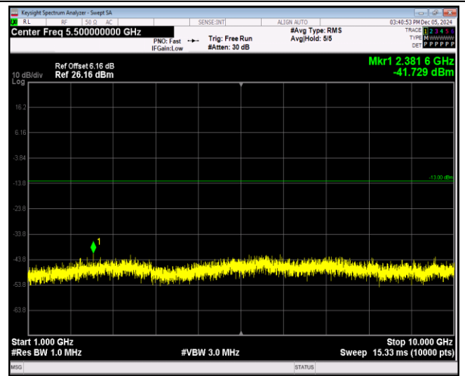
Band26-1.4MHz-16QAM-26697-1RB#0-Range2:1000~10000MHz
