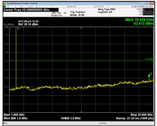
Band2-1.4MHz-64QAM-18607-1RB#0-Range2:1000~20000MHz
