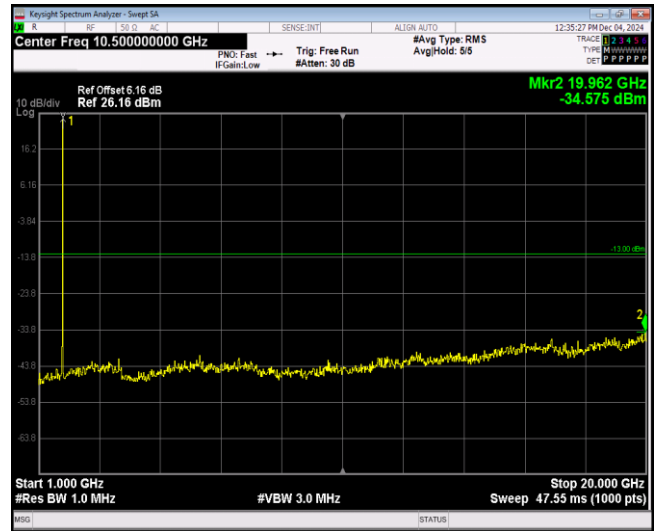
Band4-1.4MHz-16QAM-19957-1RB#0-Range2:1000~ 20000MHz
