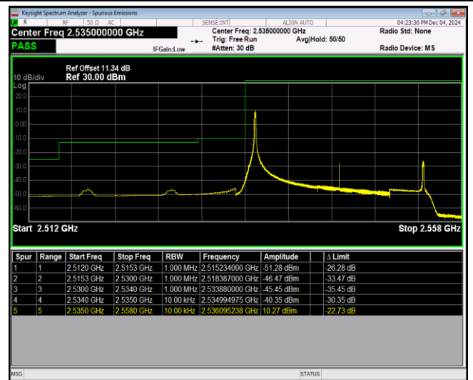
Band41-20MHz-QPSK-40140-100RB#0
