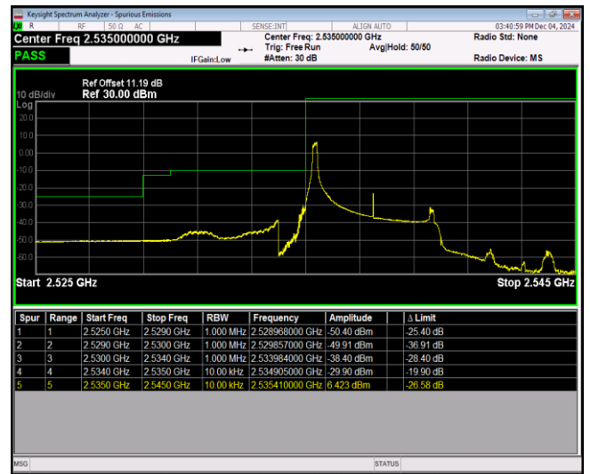
Band41-5MHz-64QAM-40065-25RB#0
