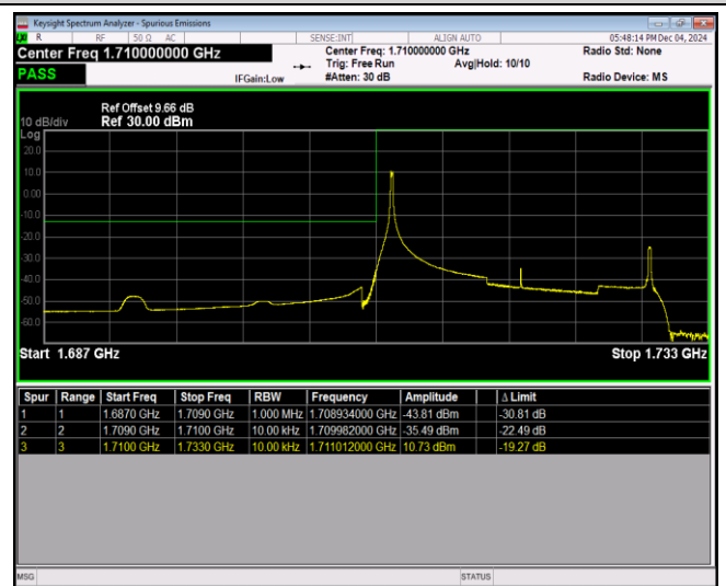
Band66-20MHz-64QAM-132072-100RB#0
