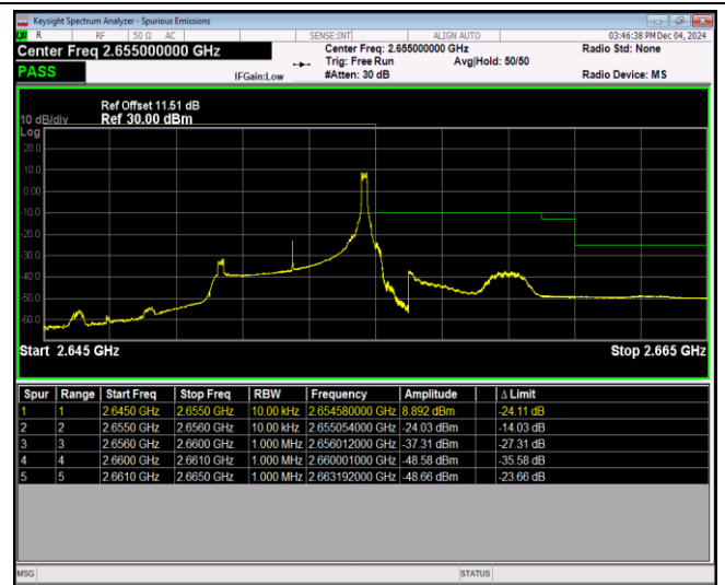
Band41-5MHz-64QAM-40065-1RB#0
