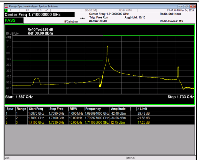
Band66-20MHz-QPSK-132072-100RB#0
