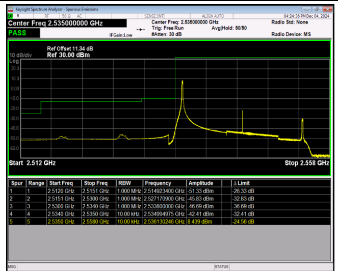
Band41-20MHz-64QAM-40140-100RB#0
