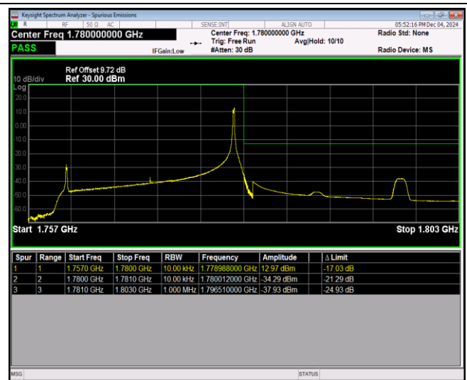
Band66-20MHz-16QAM-132072-1RB#0
