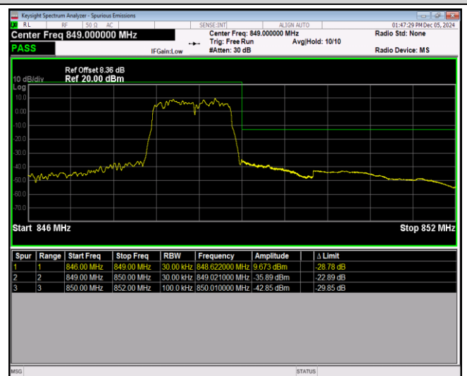
Band26-1.4MHz-16QAM-26697-1RB#5
