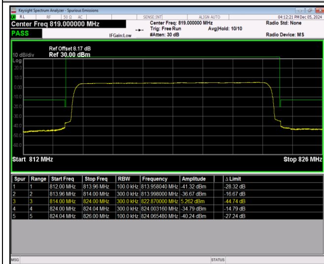
Band26-10MHz-16QAM-26740-1RB#49
