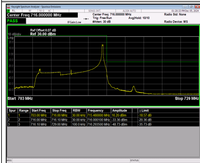
Band17-10MHz-16QAM-23780-1RB#0
