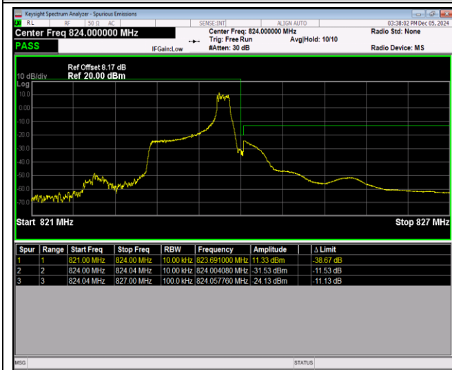
Band26-1.4MHz-64QAM-26797-1RB#0
