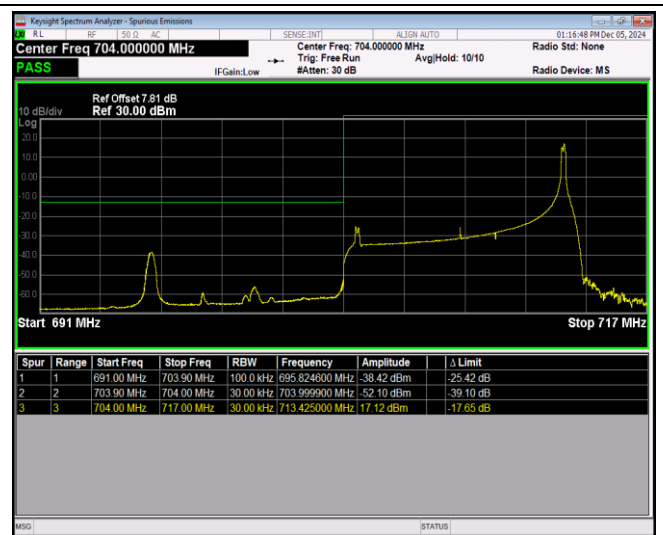
Band17-10MHz-16QAM-23800-1RB#0
