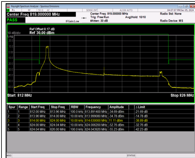
Band26-10MHz-QPSK-26740-50RB#0
