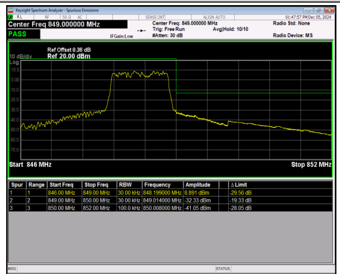
Band26-1.4MHz-64QAM-26697-1RB#5
