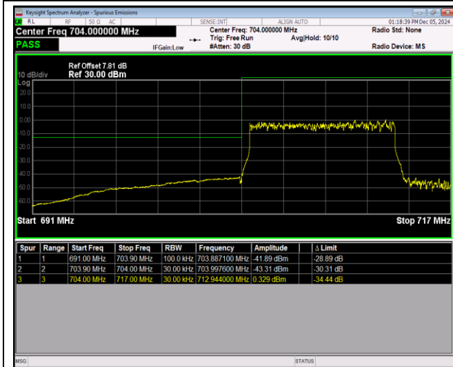
Band17-10MHz-64QAM-23800-1RB#49
