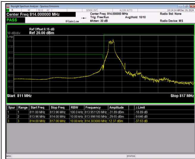
Band26-1.4MHz-64QAM-26697-6RB#0
