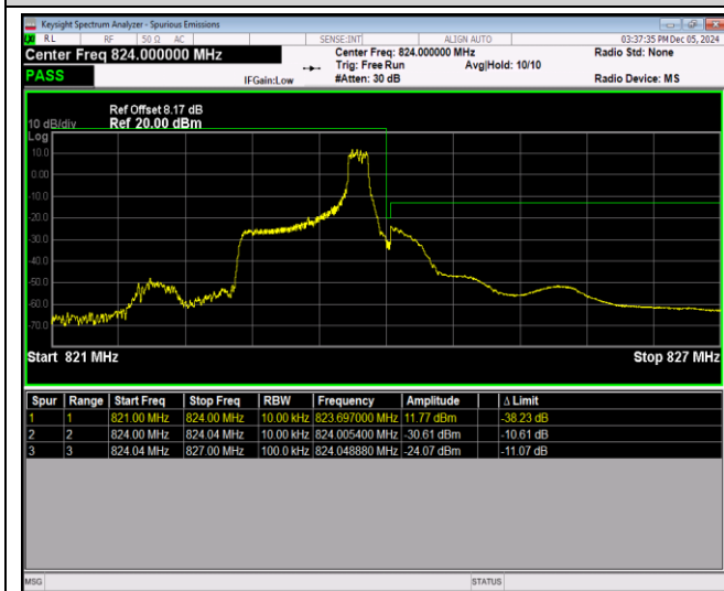
Band26-1.4MHz-16QAM-26797-1RB#0
