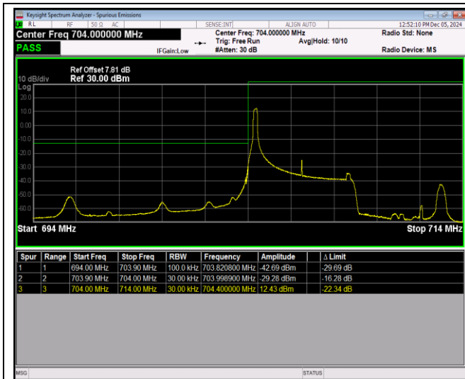
Band17-5MHz-16QAM-23755-25RB#0
