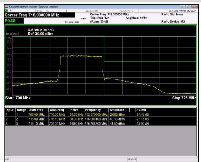
Band17-5MHz-64QAM-23755-1RB#24
