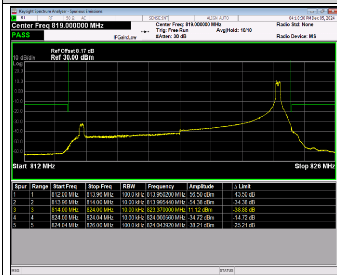
Band26-10MHz-64QAM-26740-1RB#0
