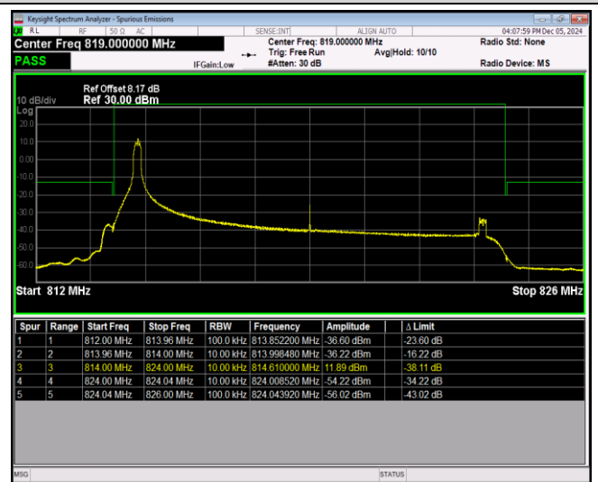
Band26-10MHz-16QAM-26740-50RB#0
