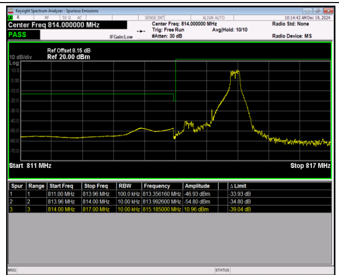
Band26-1.4MHz-64QAM-26783-1RB#0
