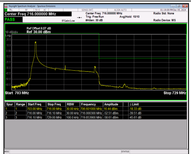
Band17-10MHz-QPSK-23800-50RB#0
