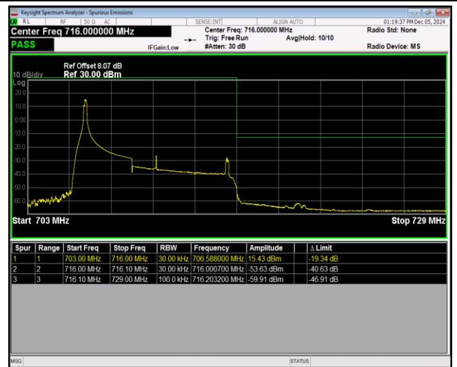
Band17-10MHz-16QAM-23800-50RB#0
