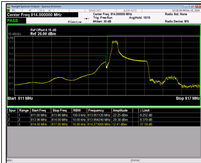
Band26-1.4MHz-16QAM-26697-6RB#0
