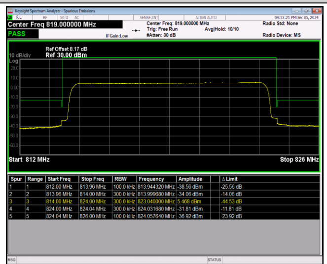
Band26-10MHz-64QAM-26740-1RB#49
