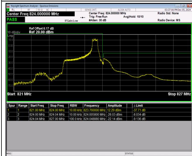
Band26-1.4MHz-QPSK-26797-1RB#0
