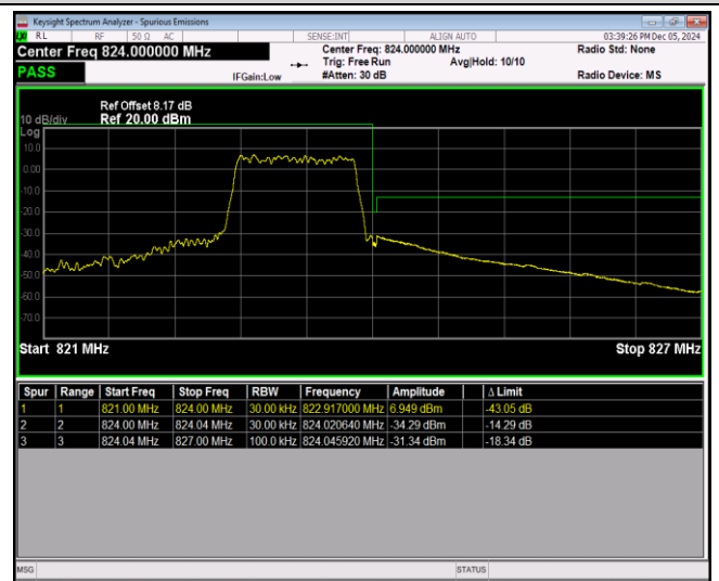
Band26-1.4MHz-64QAM-26797-1RB#5
