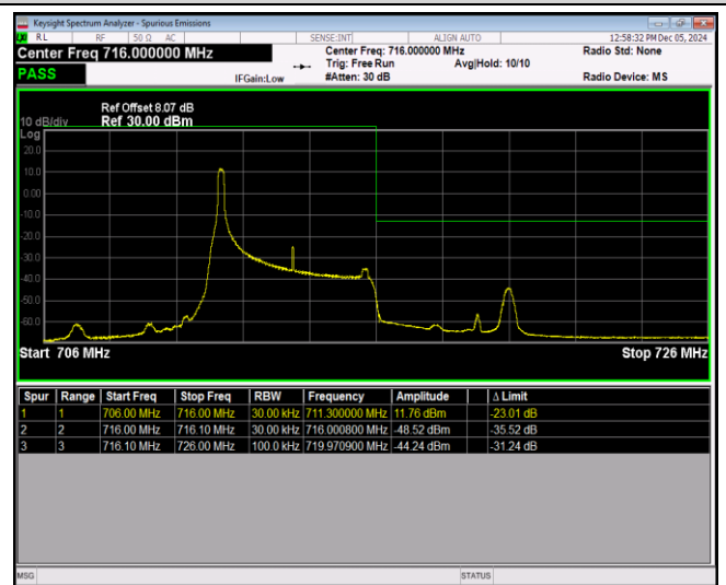
Band17-5MHz-64QAM-23825-25RB#0
