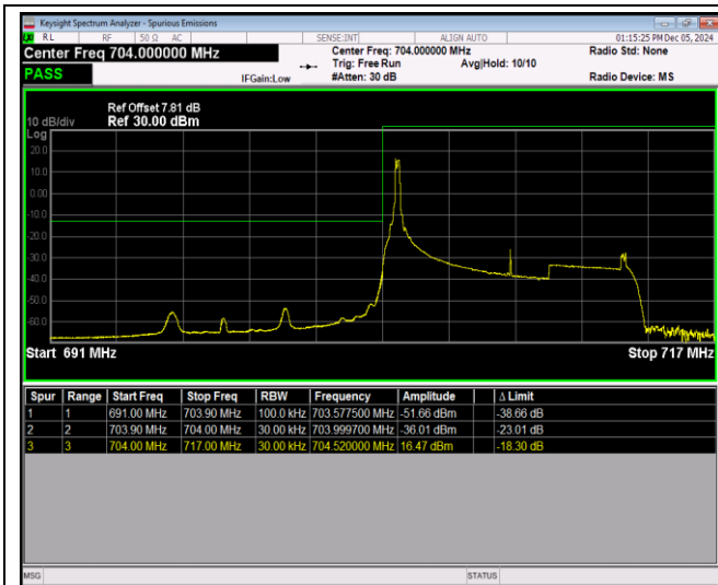
Band17-10MHz-16QAM-23780-50RB#0
