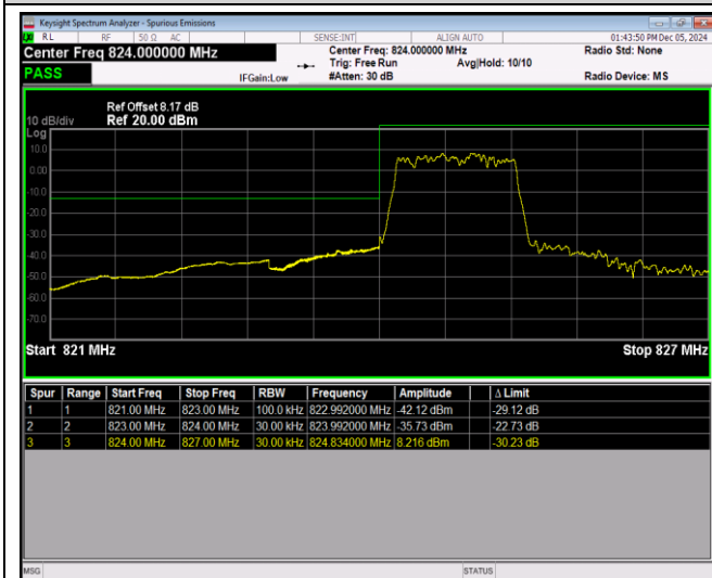
Band26-1.4MHz-QPSK-27033-1RB#5
