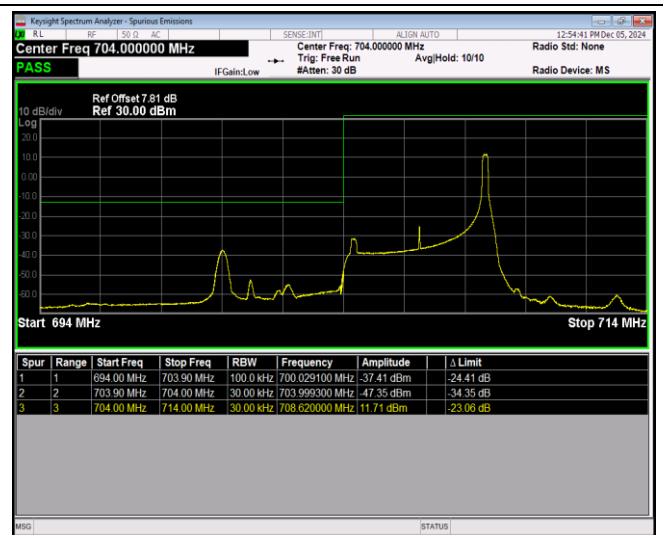
Band17-5MHz-64QAM-23825-1RB#0
