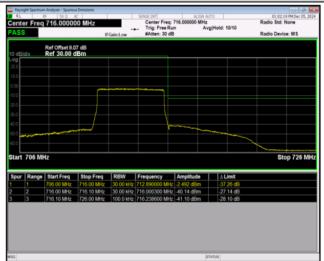
Band17-10MHz-QPSK-23780-1RB#49
