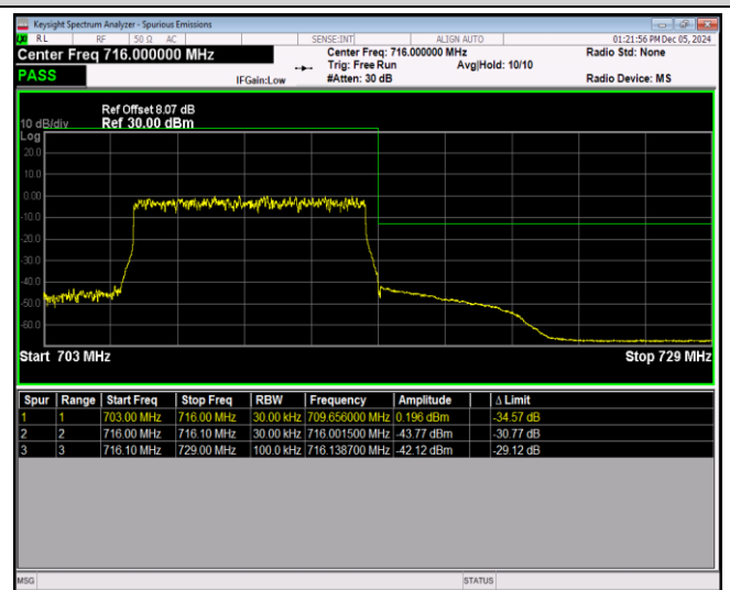
Band17-10MHz-16QAM-23780-1RB#49
