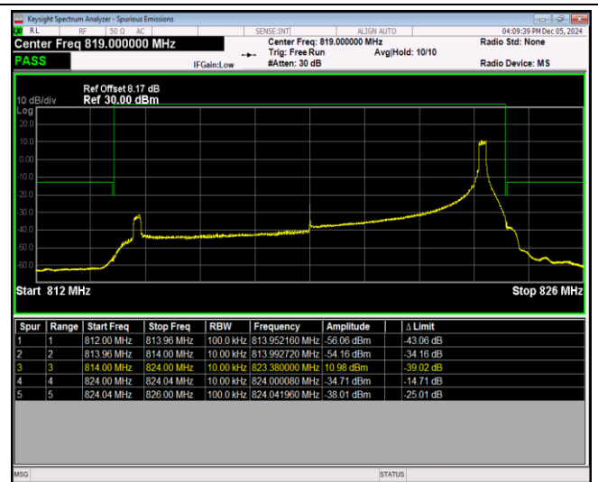
Band26-10MHz-16QAM-26740-1RB#0
