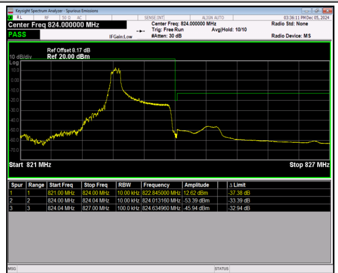
Band26-1.4MHz-16QAM-26783-6RB#0
