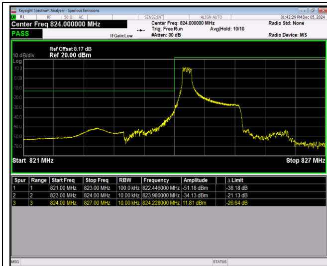
Band26-1.4MHz-64QAM-26797-6RB#0
