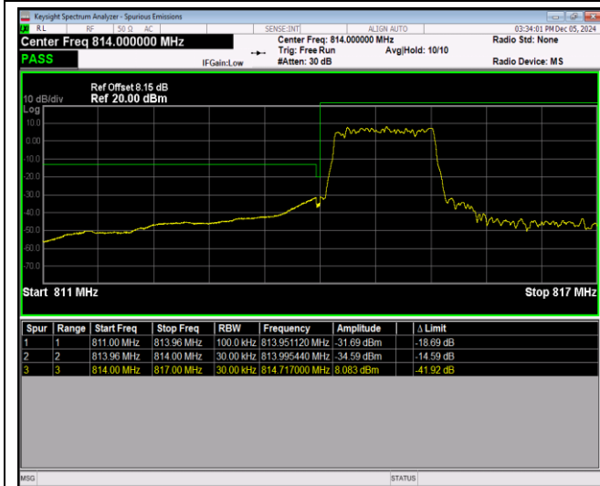
Band26-1.4MHz-QPSK-26783-1RB#5
