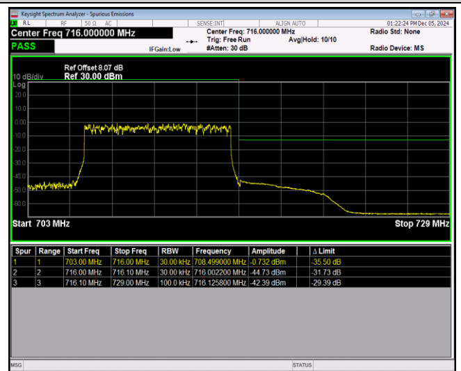
Band17-10MHz-64QAM-23780-1RB#49
