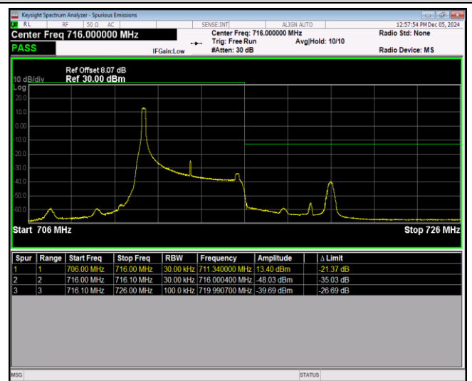
Band17-5MHz-16QAM-23825-25RB#0
