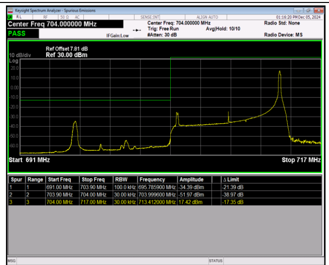
Band17-10MHz-QPSK-23800-1RB#0
