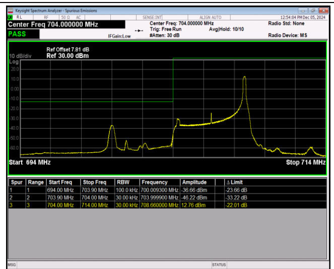
Band17-5MHz-16QAM-23825-1RB#0
