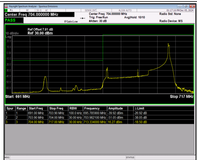
Band17-10MHz-64QAM-23800-1RB#0
