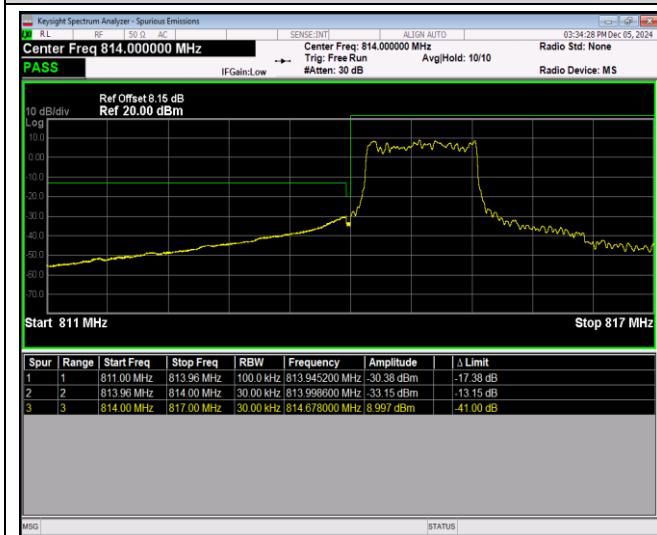
Band26-1.4MHz-16QAM-26783-1RB#5
