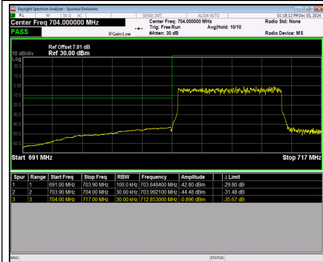
Band17-10MHz-16QAM-23800-1RB#49
