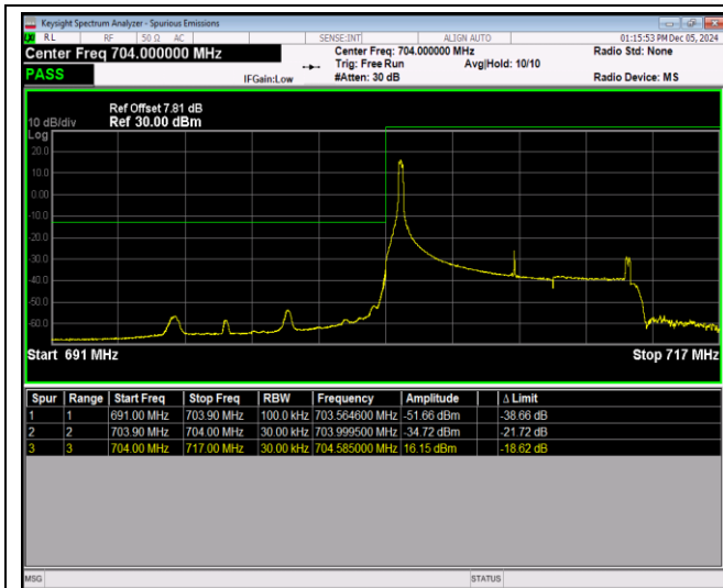
Band17-10MHz-64QAM-23780-50RB#0
