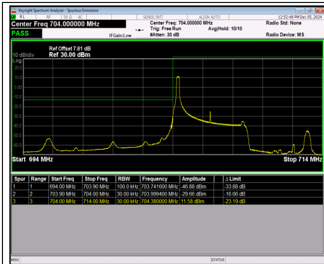
Band17-5MHz-64QAM-23755-25RB#0
