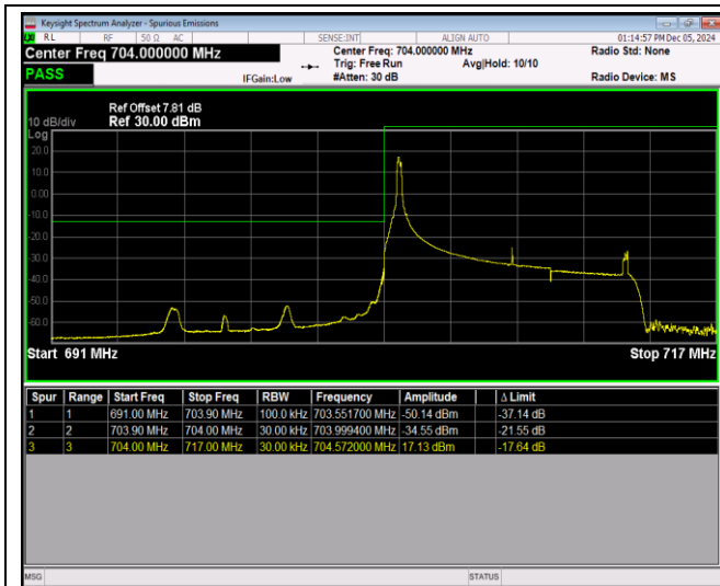
Band17-10MHz-QPSK-23780-50RB#0
