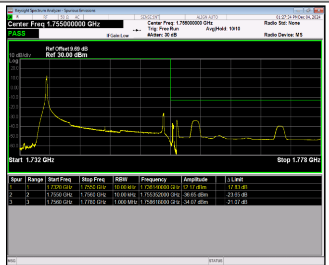
Band4-20MHz-64QAM-20300-100RB#0
