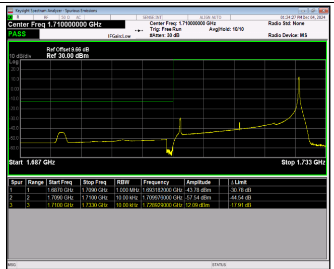
Band4-20MHz-16QAM-20300-1RB#0
