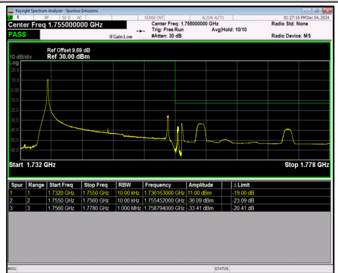
Band4-20MHz-16QAM-20300-100RB#0
