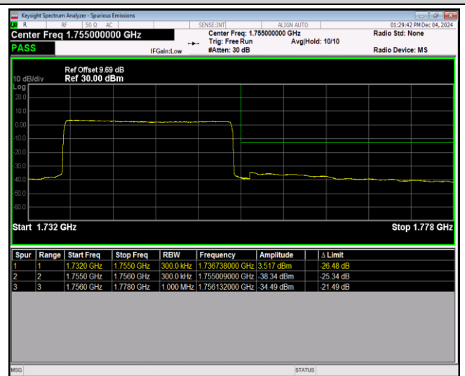
Band4-20MHz-64QAM-20050-1RB#99
