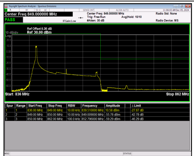
Band5-10MHz-16QAM-20600-50RB#0
