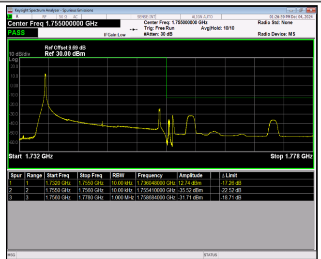
Band4-20MHz-QPSK-20300-100RB#0
