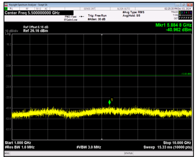
Band26-15MHz-16QAM-26965-1RB#0-Range2:1000~10000MHz
