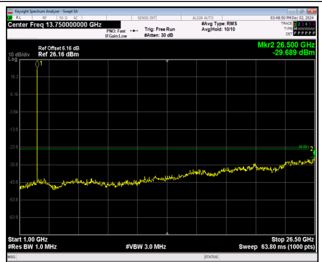
Band41-5MHz-64QAM-40640-1RB#0-Range2:1000~26500MHz
