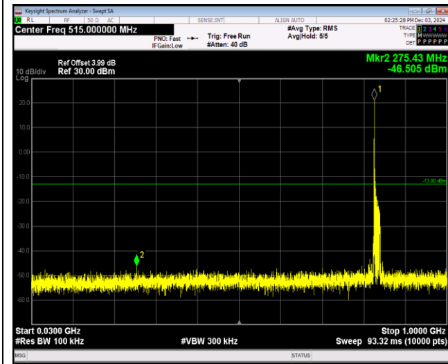
Band26-15MHz-16QAM-26965-1RB#0-Range1:30~1000MHz
