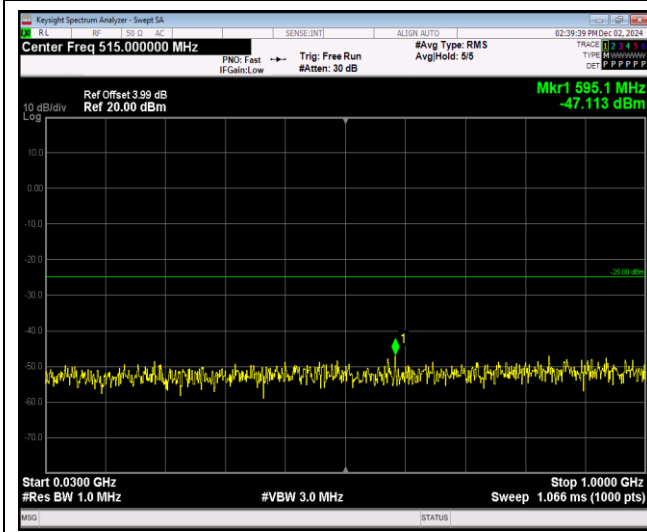
Band38-5MHz-64QAM-37775-1RB#0-Range1:30~1000MHz
