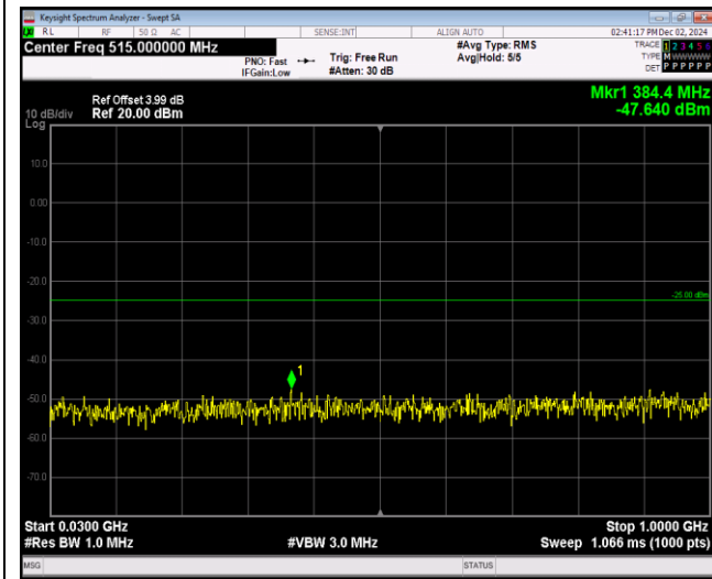
Band38-5MHz-64QAM-37775-1RB#0-Range1:30~1000MHz
