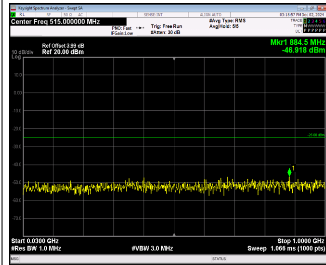
Band38-20MHz-QPSK-38150-1RB#0-Range1:30~1000MHz
