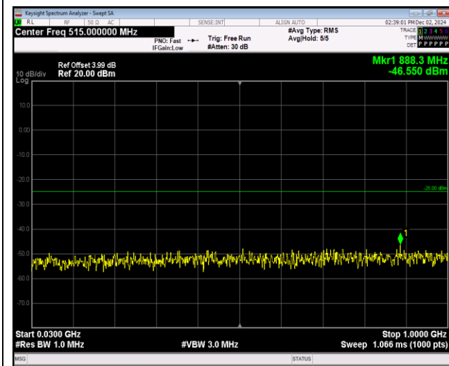
Band38-5MHz-QPSK-38000-1RB#0-Range1:30~100 OMHz
