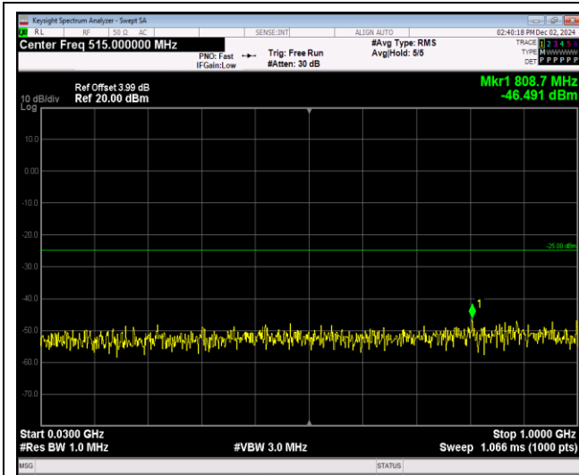
Band38-5MHz-16QAM-38225-1RB#0-Range1:30~1000MHz
