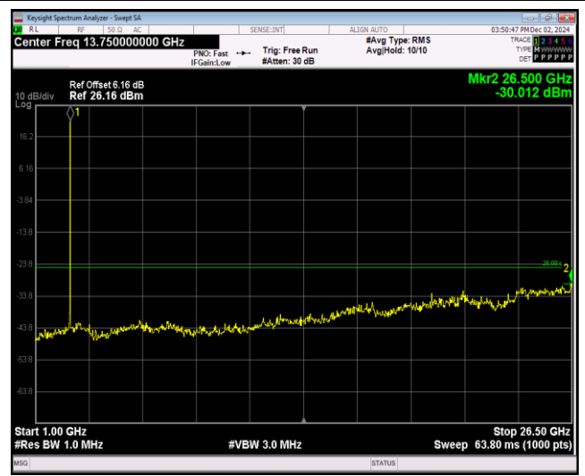
Band41-5MHz-64QAM-41215-1RB#0-Range2:1000~26500MHz
