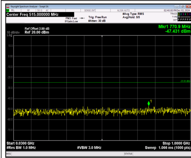
Band38-5MHz-QPSK-38000-1RB#0-Range1:30~100 OMHz
