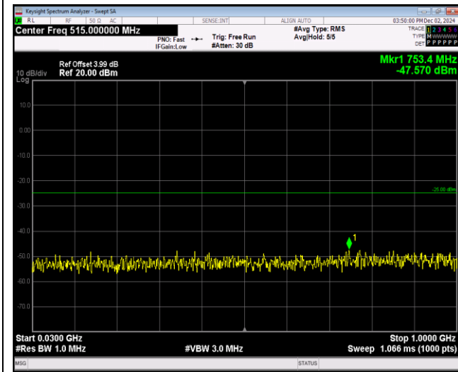
Band41-5MHz-16QAM-40065-1RB#0-Range1:30~10 00MHz
