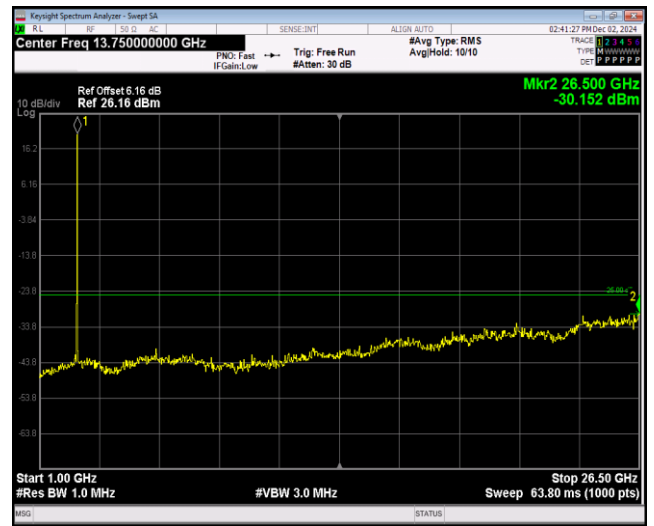
Band38-5MHz-64QAM-37775-1RB#0-Range2:1000~26500MHz
