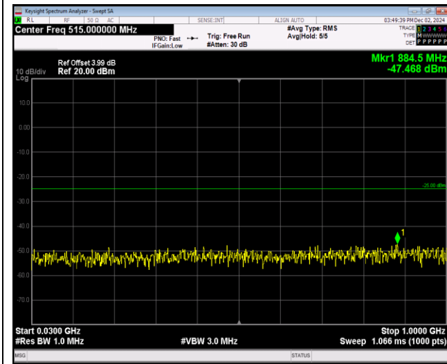
Band41-5MHz-64QAM-41215-1RB#0-Range1:30~1000MHz
