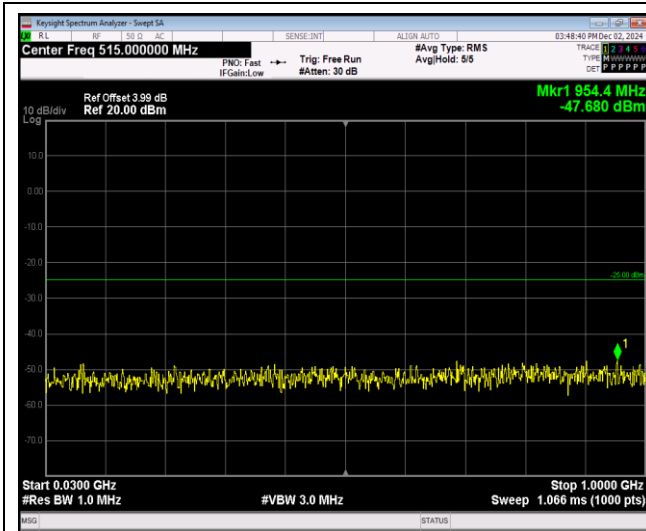
Band41-5MHz-64QAM-40640-1RB#0-Range1:30~1000MHz
