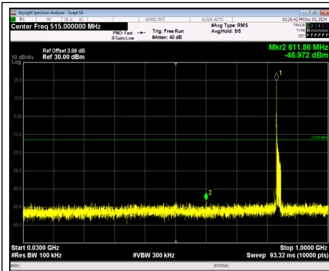
Band38-5MHz-QPSK-37775-1RB#0-Range1:30~100 OMHz
