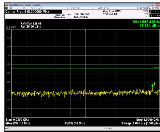
Band41-5MHz-16QAM-40065-1RB#0-Range1:30~10 00MHz
