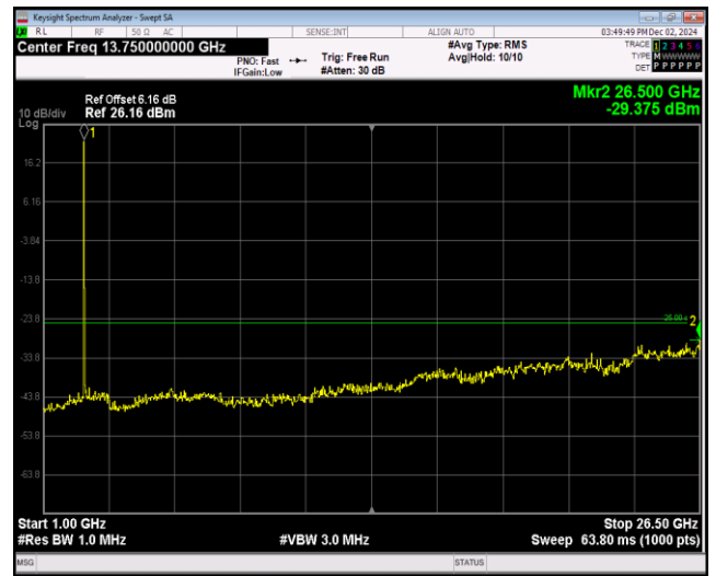
Band41-5MHz-64QAM-41215-1RB#0-Range2:1000~26500MHz
