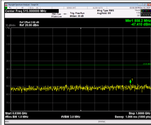
Band41-5MHz-64QAM-41215-1RB#0-Range1:30~1000MHz
