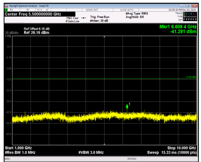
Band26-1.4MHz-QPSK-26740-1RB#0-Range2:1000~10000MHz
