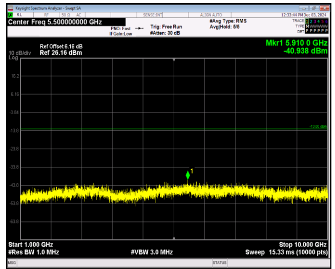
Band17-5MHz-16QAM-23790-1RB#0-Range2:1000~10000MHz
