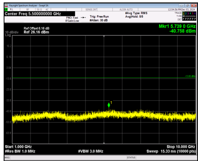
Band17-10MHz-QPSK-23800-1RB#0-Range2:1000~10000MHz
