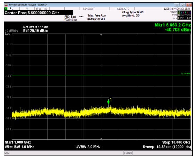
Band17-10MHz-QPSK-23780-1RB#0-Range2:1000~10000MHz
