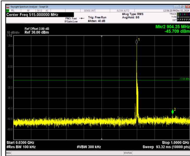
Band26-1.4MHz-QPSK-26697-1RB#0-Range1:30~1000MHz
