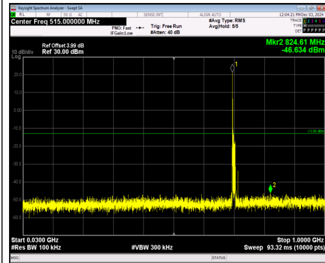
Band12-10MHz-64QAM-23130-1RB#0-Range1:30~1000MHz
