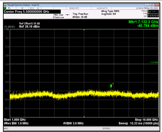
Band17-5MHz-16QAM-23790-1RB#0-Range2:1000~10000MHz
