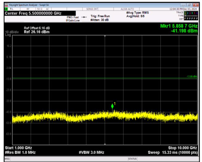
Band12-10MHz-64QAM-23130-1RB#0-Range2:1000~10000MHz
