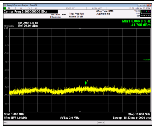
Band17-10MHz-16QAM-23800-1RB#0-Range2:1000~10000MHz
