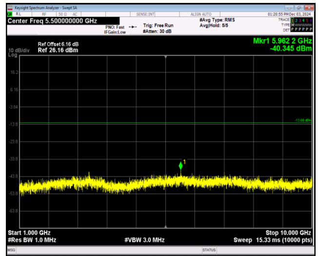
Band26-1.4MHz-16QAM-27033-1RB#0-Range2:1000~10000MHz
