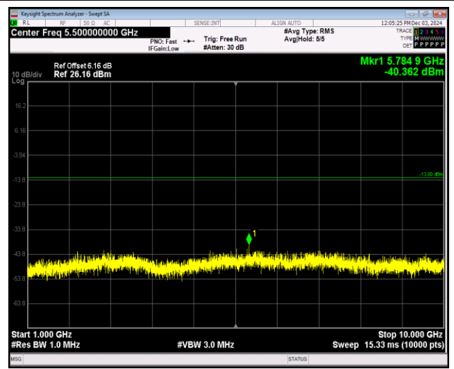
Band12-10MHz-64QAM-23130-1RB#0-Range2:1000~10000MHz
