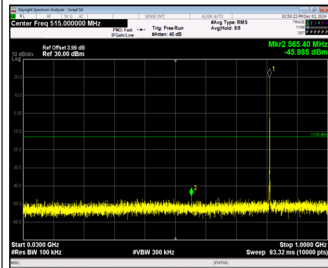
Band26-1.4MHz-QPSK-26740-1RB#0-Range1:30~1000MHz
