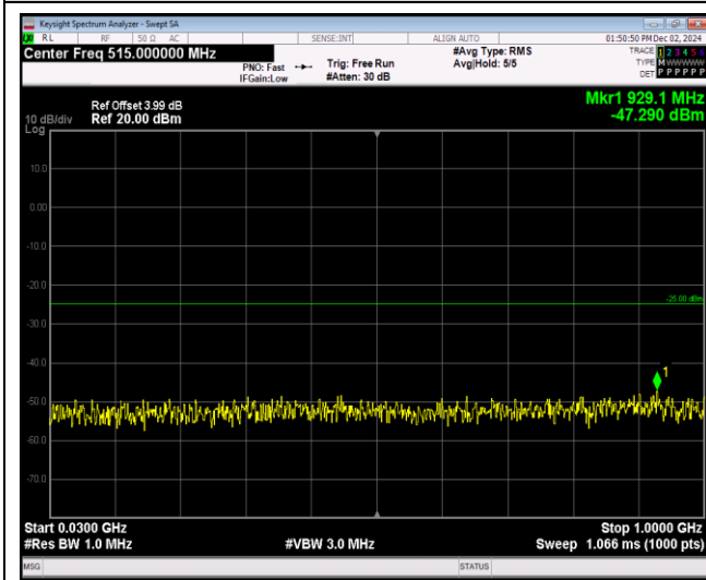
Band7-20MHz-64QAM-20850-1RB#0-Range1:30~1000MHz
