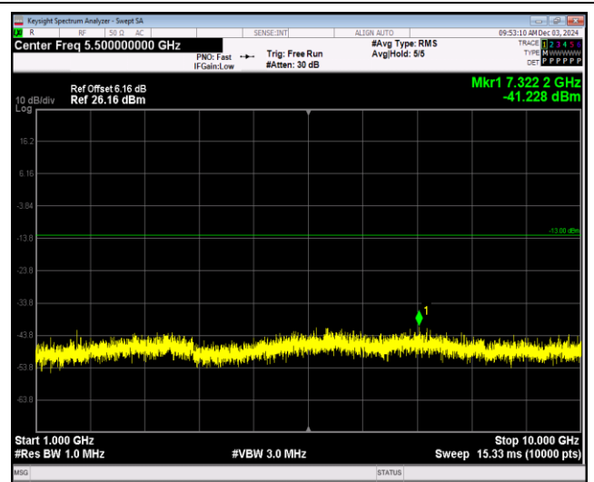
Band5-10MHz-16QAM-20450-1RB#0-Range2:1000~10000MHz
