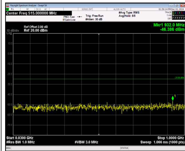
Band7-20MHz-QPSK-21100-1RB#0-Range1:30~100 OMHz
