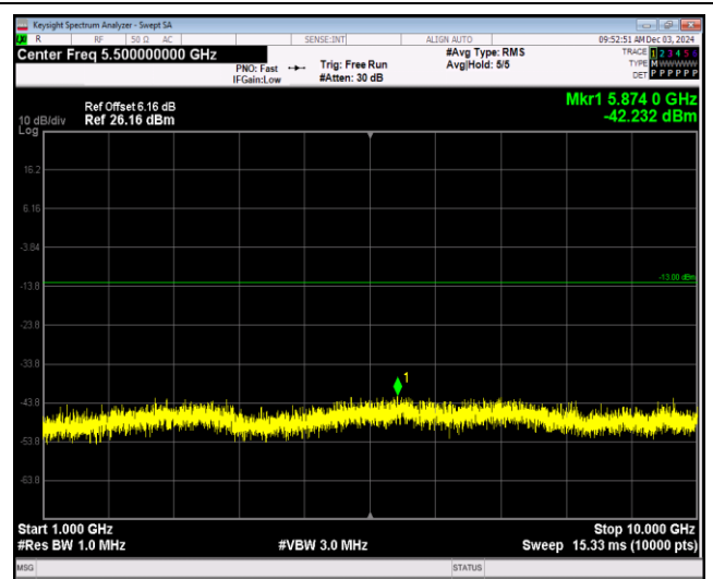
Band5-10MHz-64QAM-20600-1RB#0-Range2:1000~10000MHz
