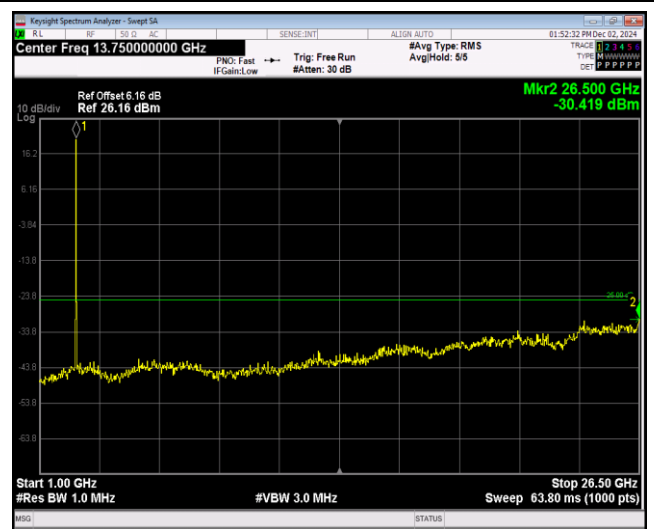
Band7-20MHz-64QAM-20850-1RB#0-Range2:1000~26500MHz
