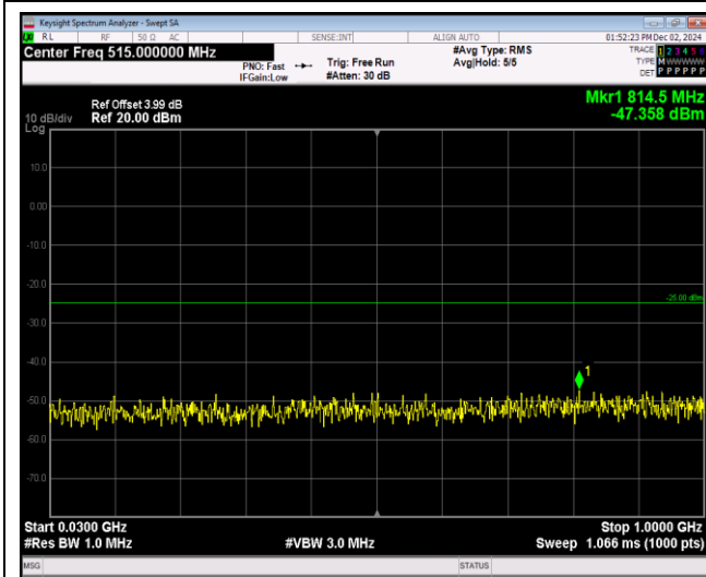
Band7-20MHz-64QAM-20850-1RB#0-Range1:30~1000MHz
