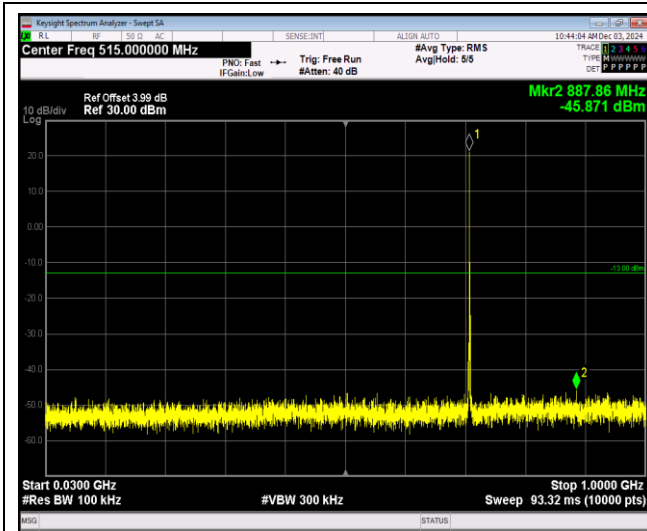
Band12-1.4MHz-64QAM-23017-1RB#0-Range1:30~1000MHz
