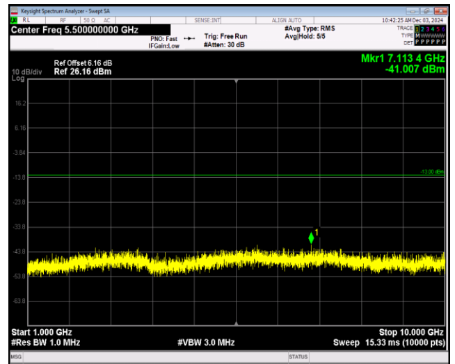
Band12-1.4MHz-QPSK-23173-1RB#0-Range2:1000~10000MHz
