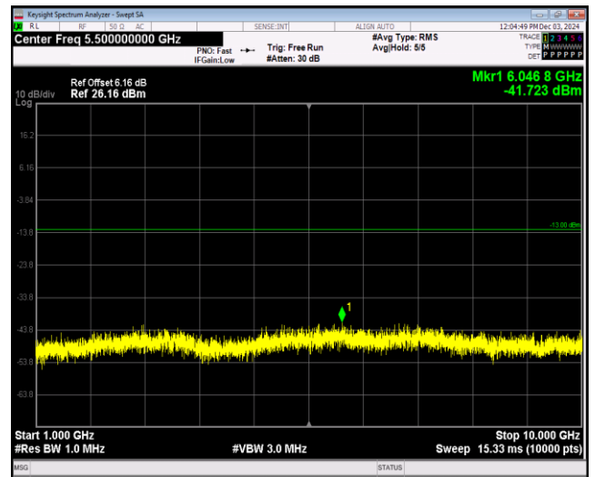
Band12-10MHz-16QAM-23060-1RB#0-Range2:1000~10000MHz
