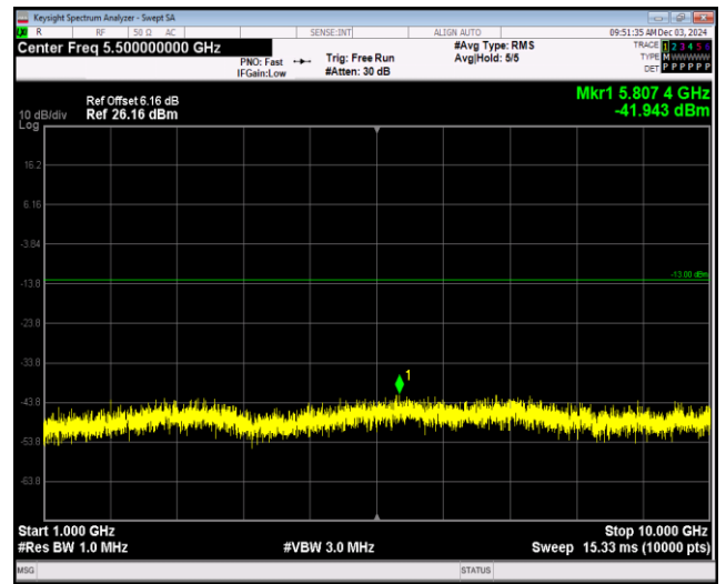
Band5-10MHz-16QAM-20525-1RB#0-Range2:1000~10000MHz
