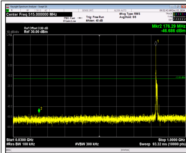
Band5-10MHz-64QAM-20600-1RB#0-Range1:30~1000MHz
