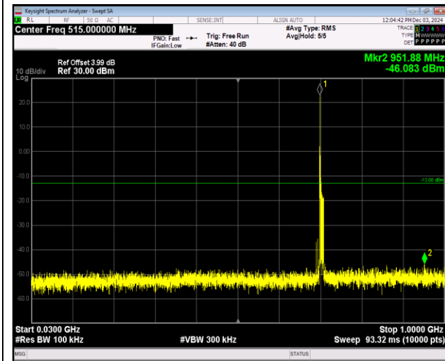
Band12-10MHz-16QAM-23060-1RB#0-Range1:30~1000MHz
