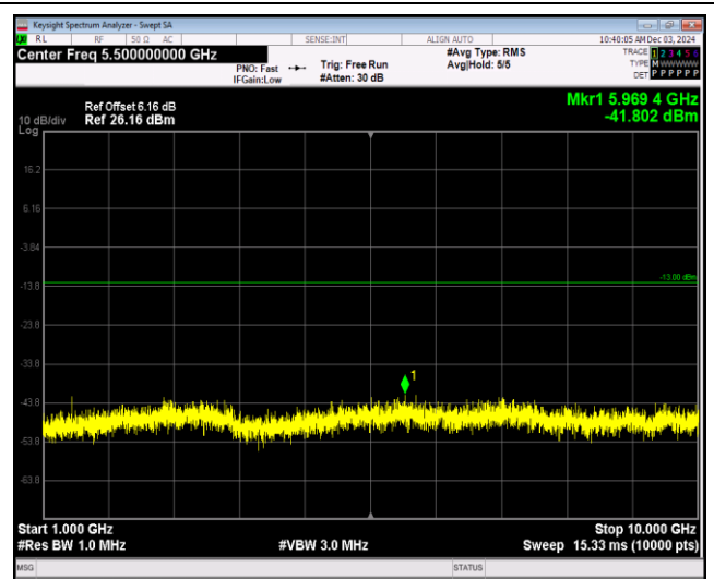
Band12-1.4MHz-QPSK-23095-1RB#0-Range2:1000~10000MHz
