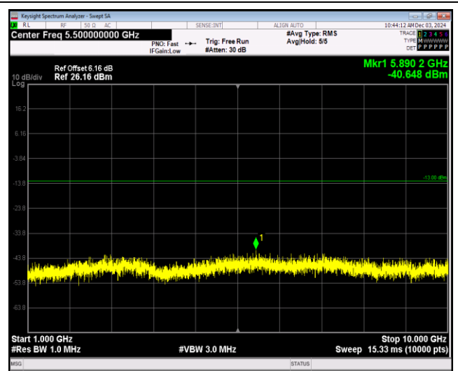
Band12-1.4MHz-64QAM-23017-1RB#0-Range2:1000~10000MHz
