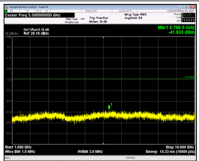
Band12-10MHz-QPSK-23130-1RB#0-Range2:1000~10000MHz
