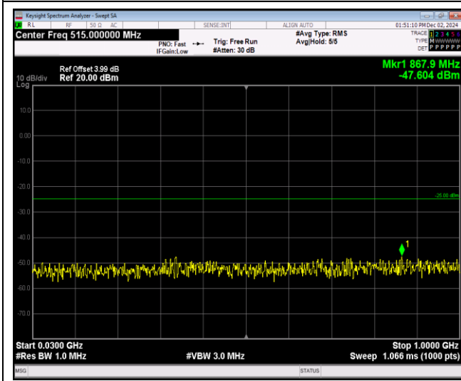
Band7-20MHz-QPSK-21100-1RB#0-Range1:30~100 OMHz
