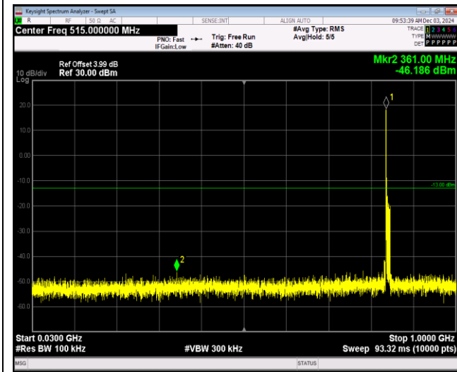
Band7-5MHz-QPSK-20775-1RB#0-Range1:30~1000MHz
