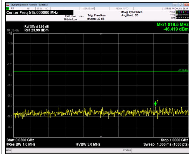
Band4-1.4MHz-QPSK-20175-1RB#0-Range1:30~1000MHz
