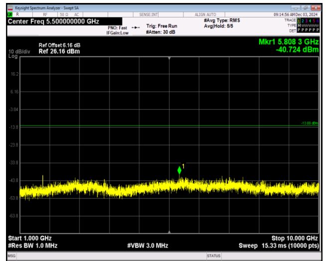
Band5-1.4MHz-16QAM-20407-1RB#0-Range2:1000~10000MHz
