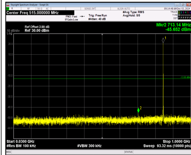
Band5-1.4MHz-16QAM-20407-1RB#0-Range1:30~1000MHz
