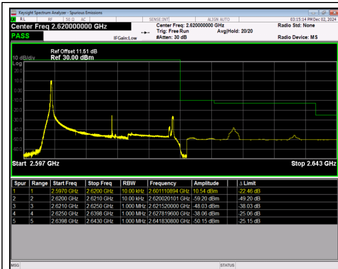
Band38-20MHz-16QAM-38150-100RB#0
