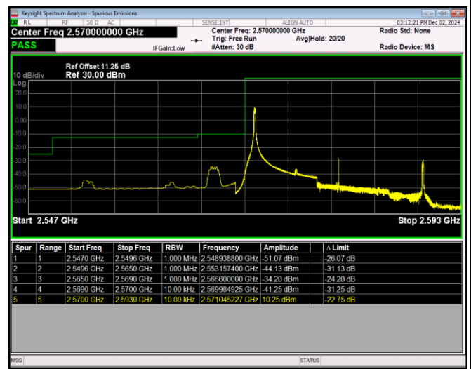
Band38-20MHz-16QAM-37850-100RB#0
