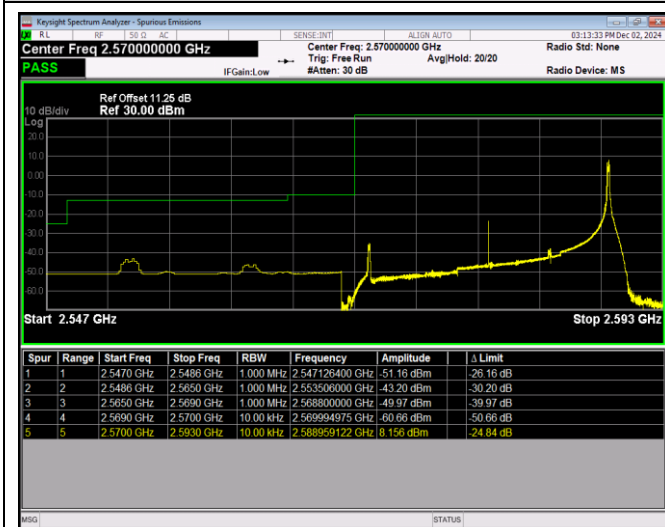
Band38-20MHz-64QAM-38150-1RB#0
