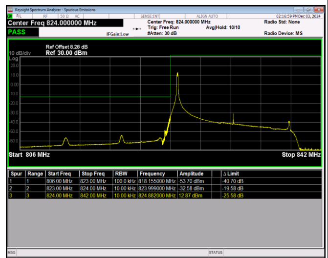
Band26-15MHz-16QAM-26865-75RB#0
