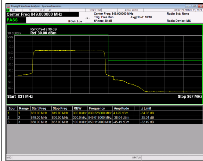
Band26-15MHz-16QAM-26865-1RB#74
