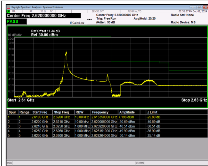
Band38-5MHz-64QAM-38225-25RB#0
