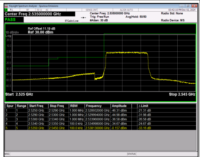
Band41-5MHz-16QAM-41215-1RB#24
