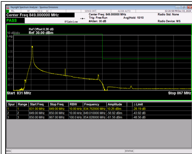
Band26-15MHz-64QAM-26965-75RB#0
