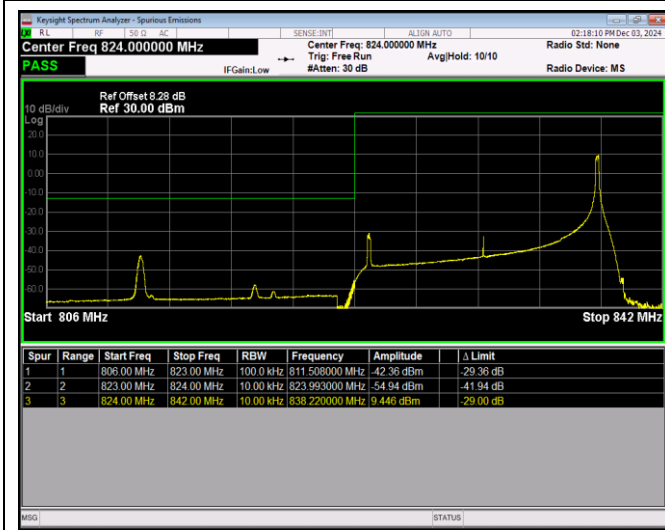
Band26-15MHz-64QAM-26965-1RB#0
