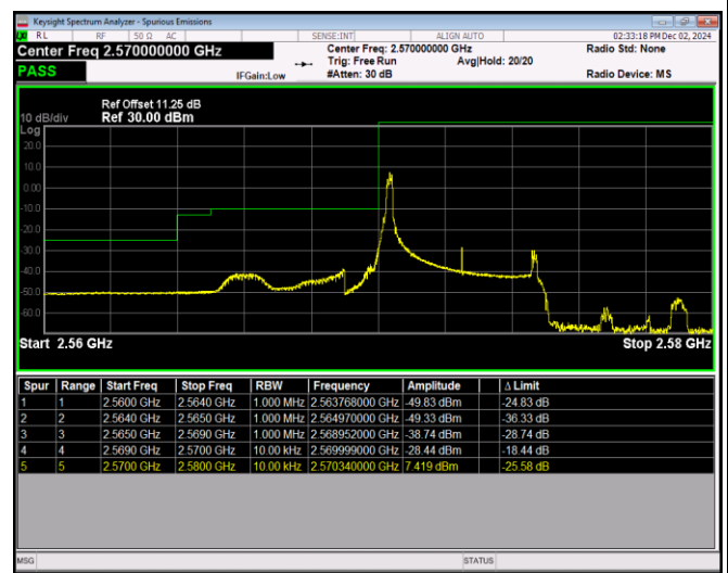
Band38-5MHz-QPSK-37775-25RB#0
