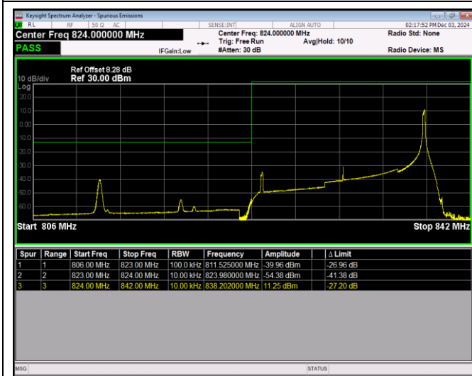
Band26-15MHz-16QAM-26965-1RB#0
