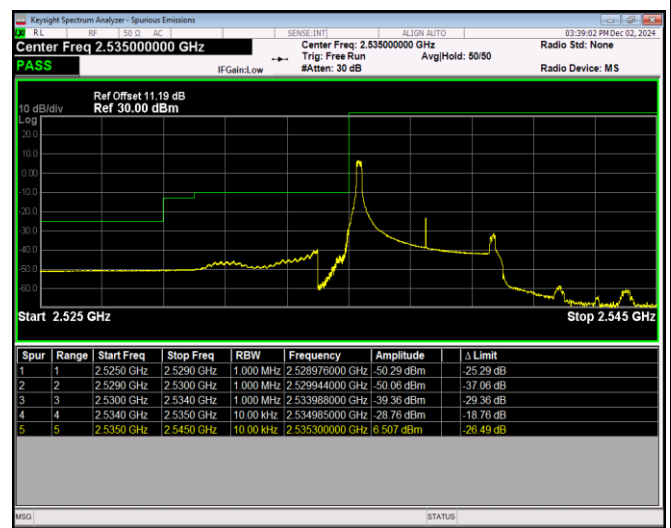
Band41-5MHz-16QAM-40065-25RB#0
