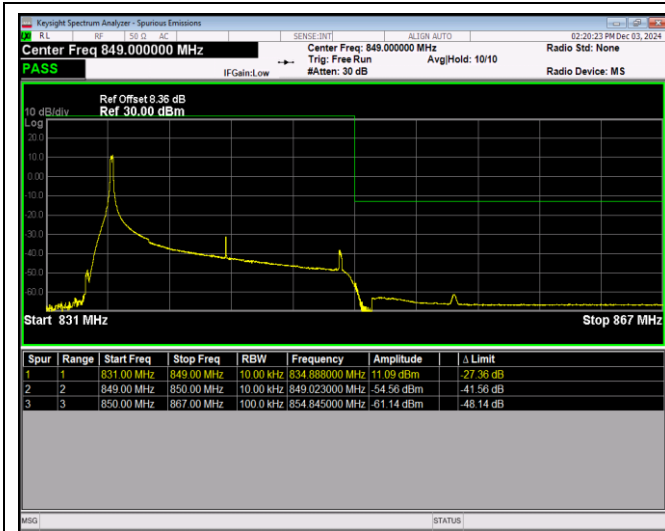
Band26-15MHz-QPSK-26965-75RB#0
