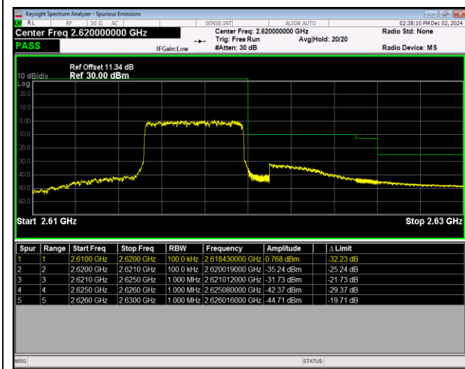
Band38-5MHz-64QAM-37775-1RB#24
