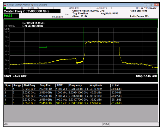
Band41-5MHz-QPSK-41215-1RB#24
