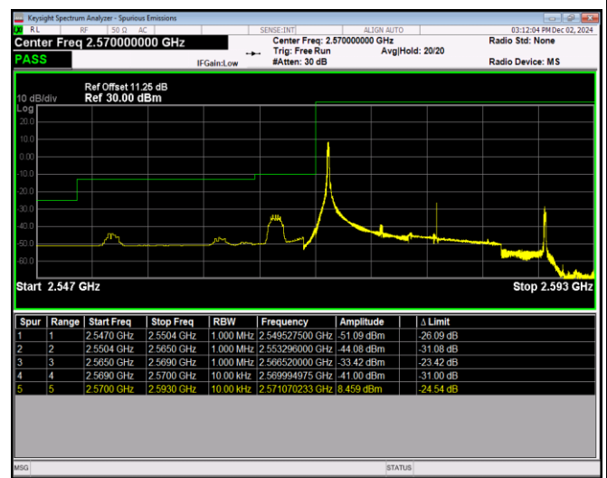
Band38-20MHz-QPSK-37850-100RB#0
