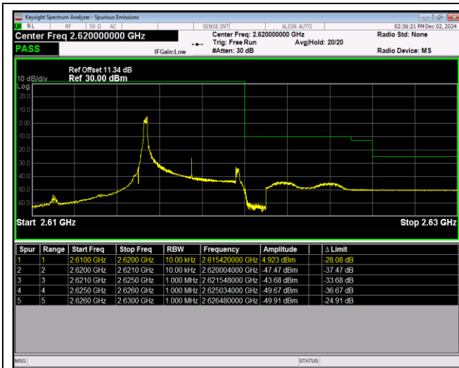
Band38-5MHz-16QAM-38225-25RB#0
