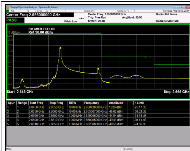
Band41-5MHz-QPSK-41215-25RB#0
