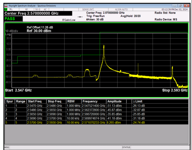
Band38-20MHz-64QAM-37850-100RB#0
