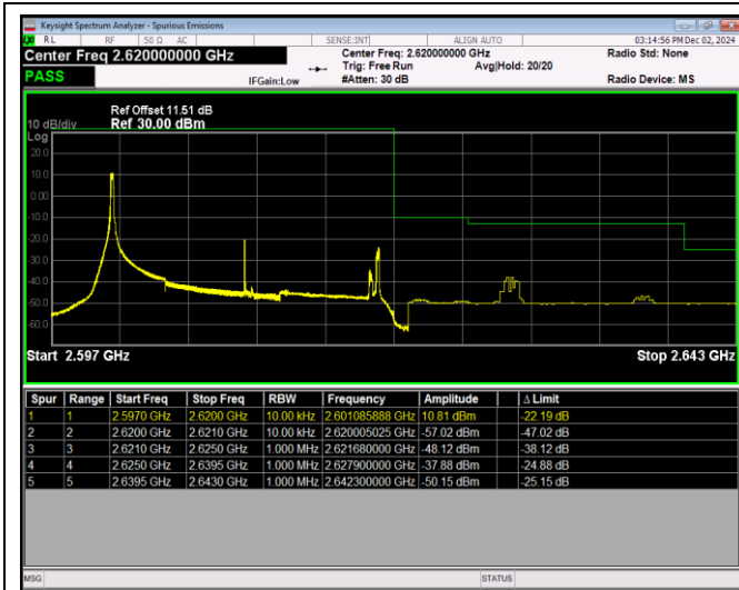
Band38-20MHz-QPSK-38150-100RB#0
