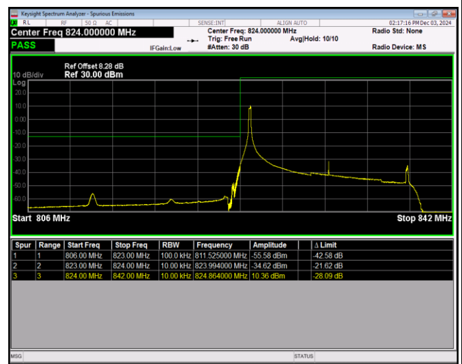
Band26-15MHz-64QAM-26865-75RB#0
