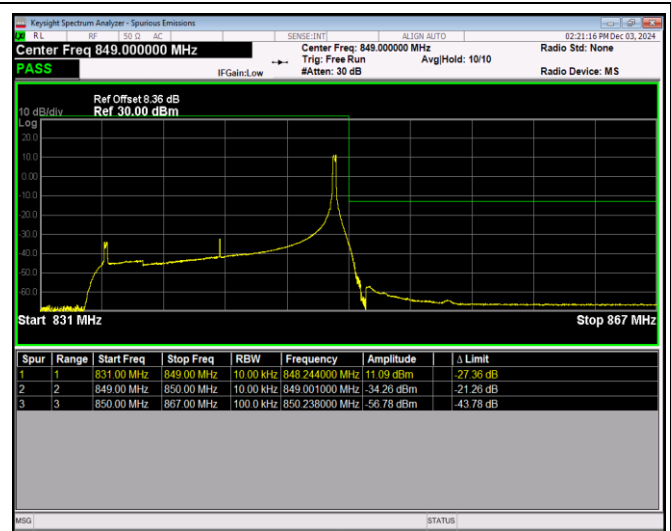
Band26-15MHz-16QAM-26865-1RB#0
