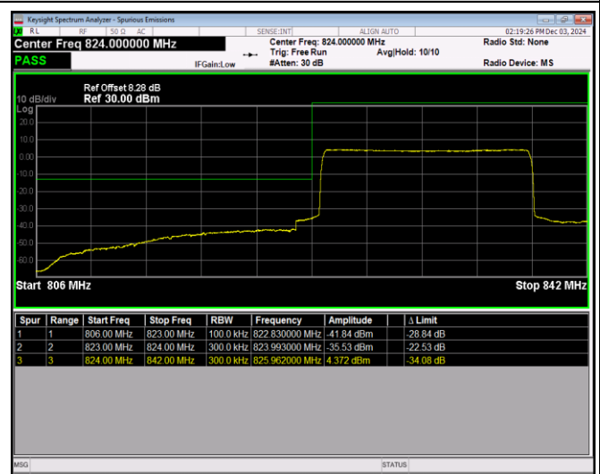
Band26-15MHz-16QAM-26965-1RB#74
