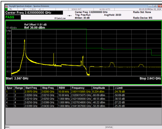
Band38-20MHz-64QAM-38150-100RB#0
