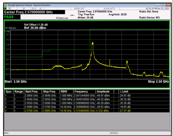
Band38-5MHz-16QAM-37775-25RB#0
