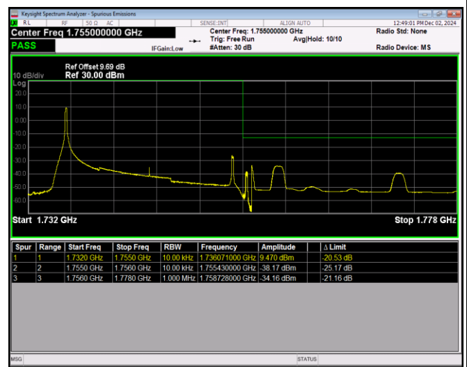
Band4-20MHz-64QAM-20300-100RB#0
