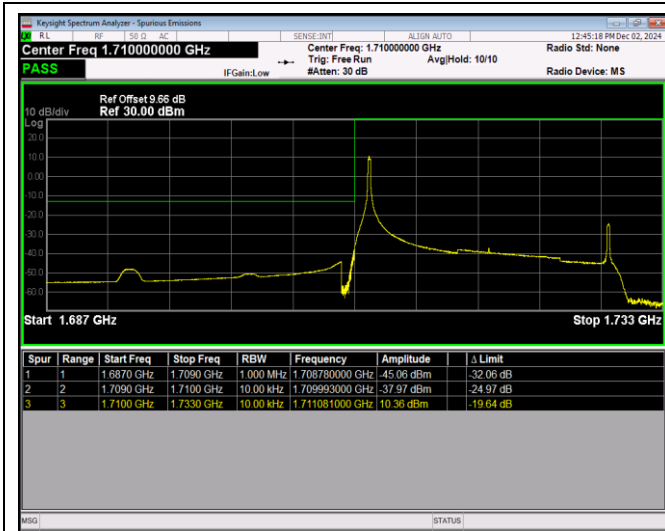
Band4-20MHz-64QAM-20050-100RB#0
