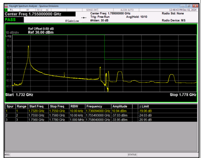
Band4-20MHz-16QAM-20300-100RB#0
