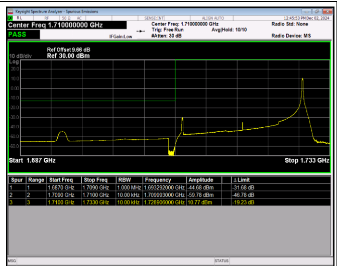
Band4-20MHz-16QAM-20300-1RB#0
