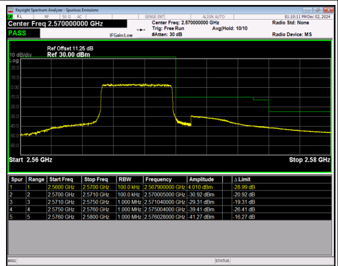
Band7-5MHz-64QAM-20775-1RB#24
