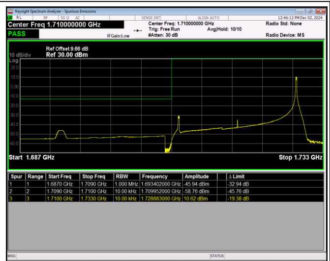
Band4-20MHz-64QAM-20300-1RB#0
