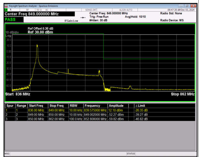
Band5-10MHz-16QAM-20600-50RB#0
