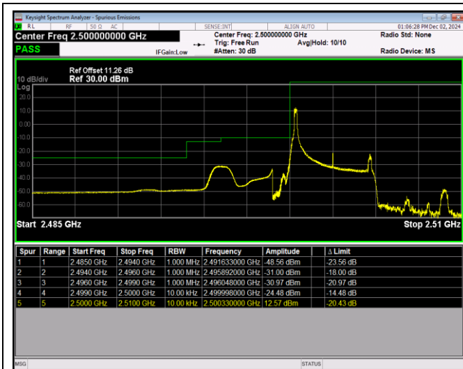
Band7-5MHz-QPSK-20775-25RB#0
