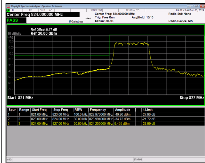
Band5-1.4MHz-QPSK-20643-1RB#5
