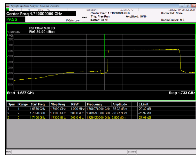
Band4-20MHz-16QAM-20300-1RB#99
