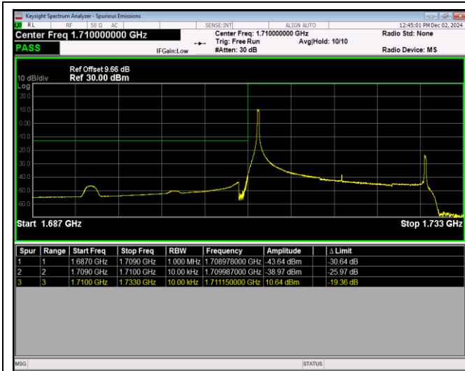
Band4-20MHz-16QAM-20050-100RB#0
