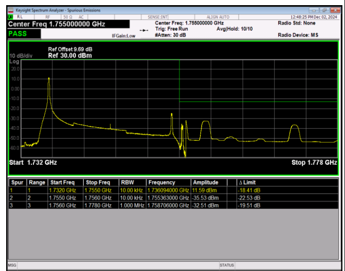
Band4-20MHz-QPSK-20300-100RB#0
