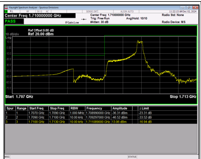
Band4-1.4MHz-64QAM-20393-1RB#0
