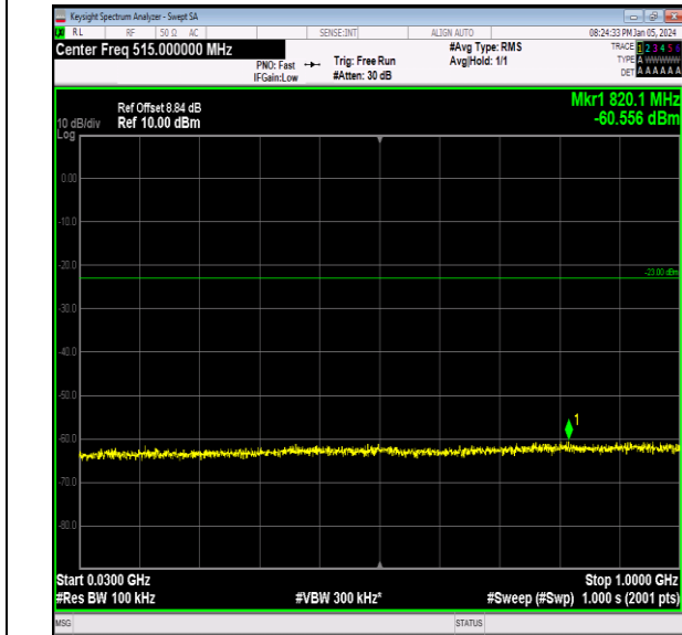
Band66_20MHz_16QAM_132322_1RB#0_30~1000_30~1 000
