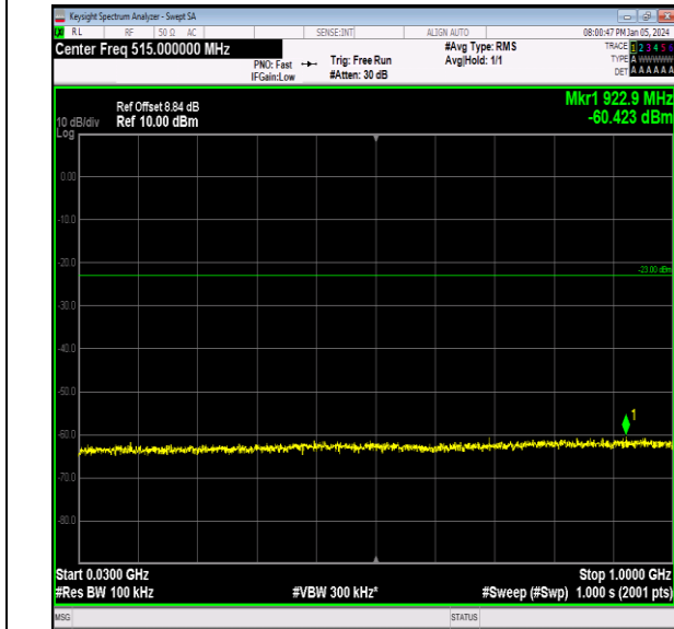
Band66_15MHz_16QAM_132597_1RB#0_30~1000_30~1 000
