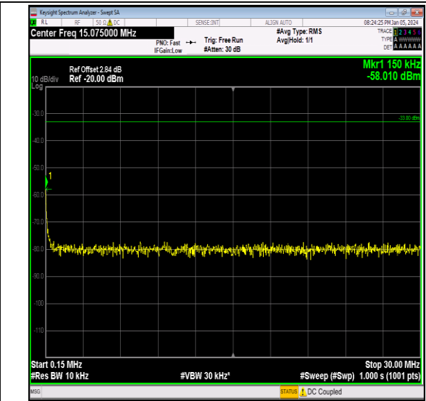
Band66_20MHz_16QAM_132322_1RB#0_0.15~30_0.15~ 30
