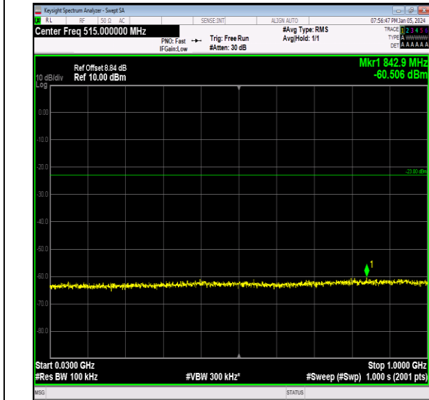
Band66_15MHz_QPSK_132322_1RB#0_30-1000_30-1000 00
