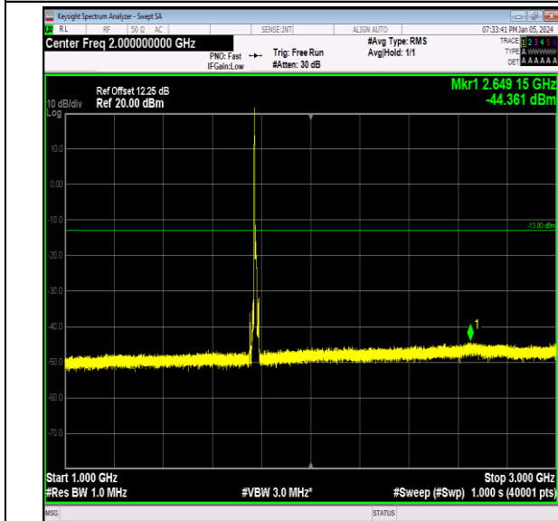
Band66_10MHz_16QAM_132622_1RB#0_1000~3000_1000~3000
