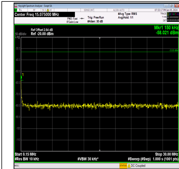
Band66_10MHz_16QAM_132622_1RB#0_0.15~30_0.15~30
