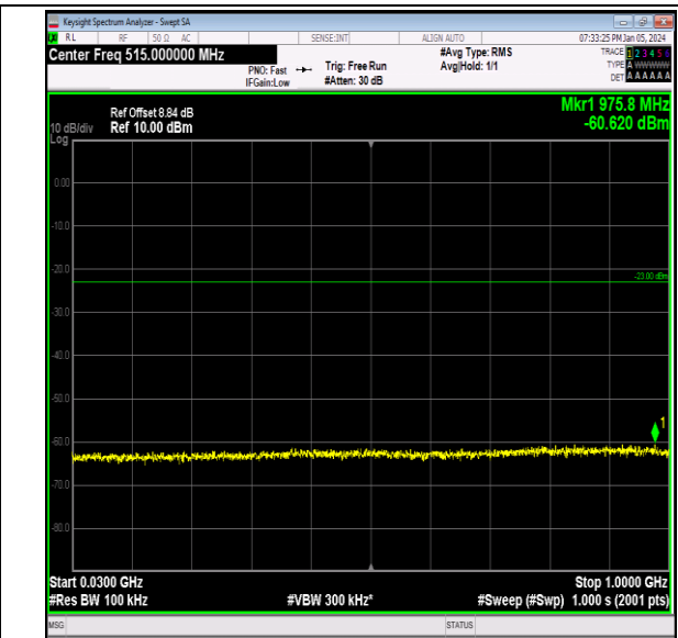
Band66_10MHz_16QAM_132622_1RB#0_30~1000_30~1000
