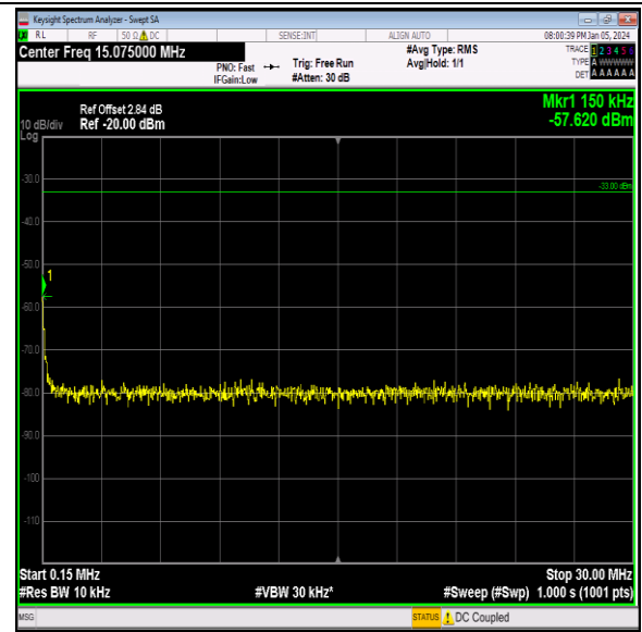
Band66_15MHz_16QAM_132597_1RB#0_0.15~30_0.15~ 30
