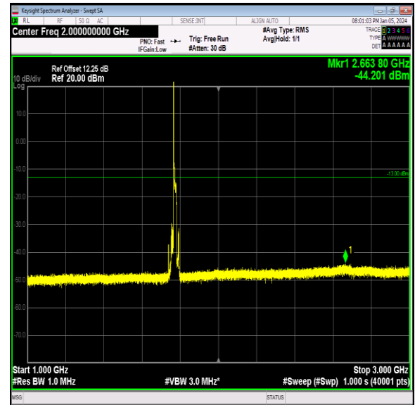
Band66_15MHz_16QAM_132597_1RB#0_1000~3000_10 00~3000
