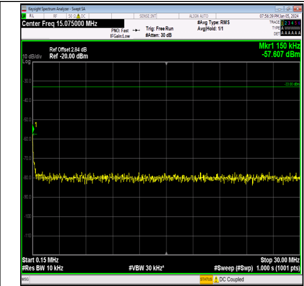
Band66_15MHz_QPSK_132322_1RB#0_0.15-30_0.15-30 0
