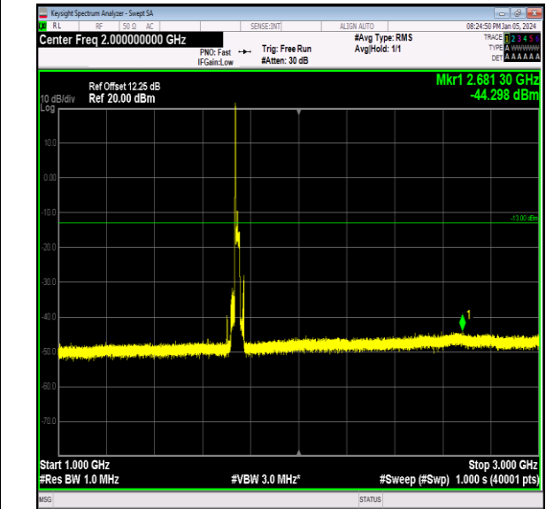
Band66_20MHz_16QAM_132322_1RB#0_1000~3000_10 00~3000
