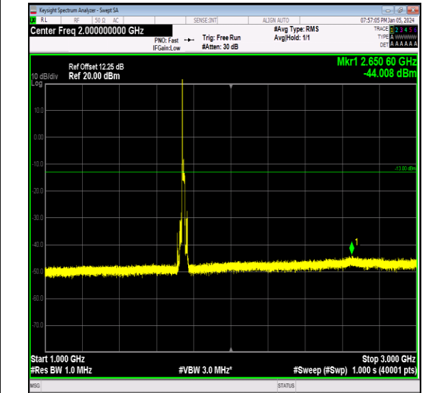
Band66_15MHz_QPSK_132322_1RB#0_1000-3000_1000-3000 0~3000
