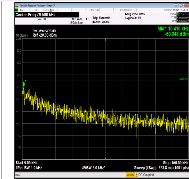
Band41_20MHz_64QAM_40140_1RB#0_0.009~0.15_0.00 9~0.15
