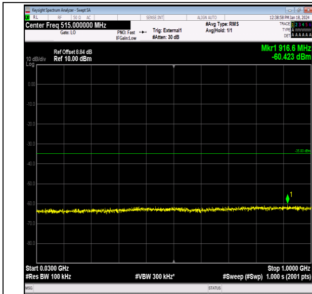
Band41_20MHz_64QAM_41140_1RB#0_30~1000_30~10 00
