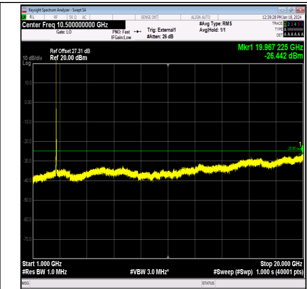
Band41_20MHz_64QAM_41140_1RB#0_1000~20000_10 00~20000
