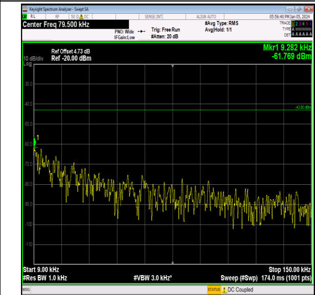
Band66_1.4MHz_16QAM_132322_1RB#0_0.009~0.15_0.009~0.15
