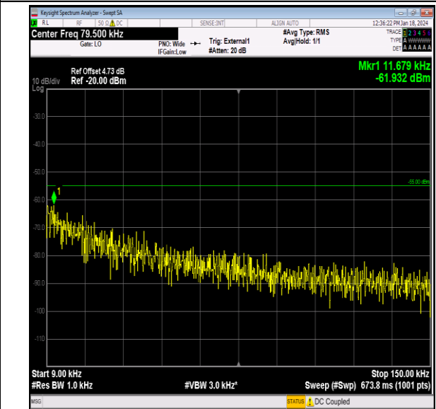
Band41_20MHz_16QAM_41140_1RB#0_0.009~0.15_0.00 9~0.15
