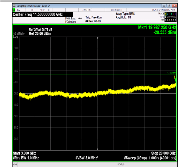
Band66_1.4MHz_QPSK_131979_1RB#0_3000~20000_30
