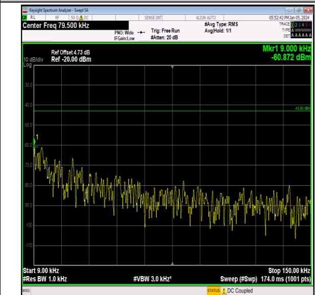
Band66_1.4MHz_QPSK_131979_1RB#0_0.009~0.15_0.0 09~0.15
