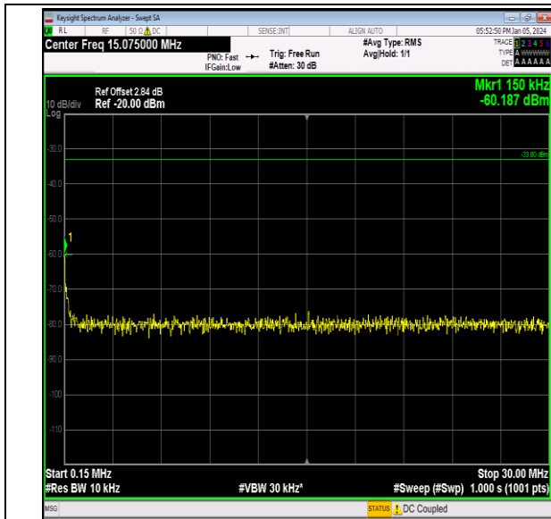
Band66_1.4MHz_QPSK_131979_1RB#0_0.15~30_0.15~3
