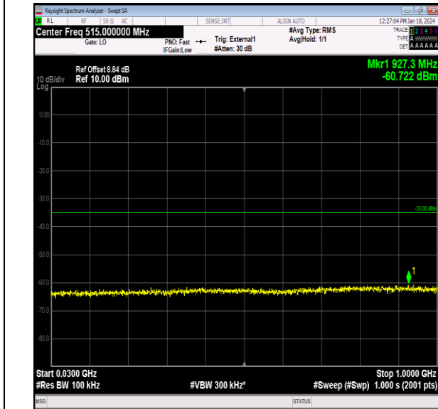
Band41_20MHz_64QAM_40140_1RB#0_30~1000_30~10 00
