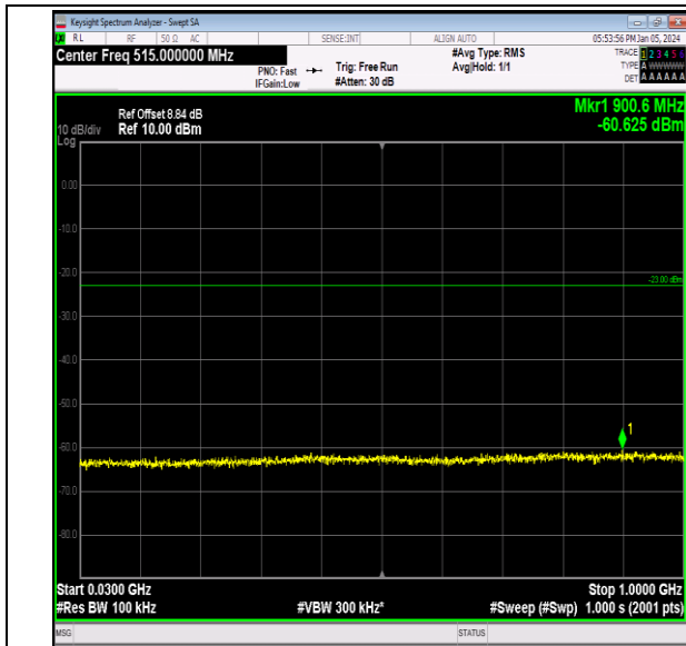
Band66_1.4MHz_16QAM_131979_1RB#0_30~1000_30~1000
