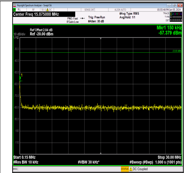
Band66_1.4MHz_QPSK_132322_1RB#0_0.15~30_0.15~3 0
