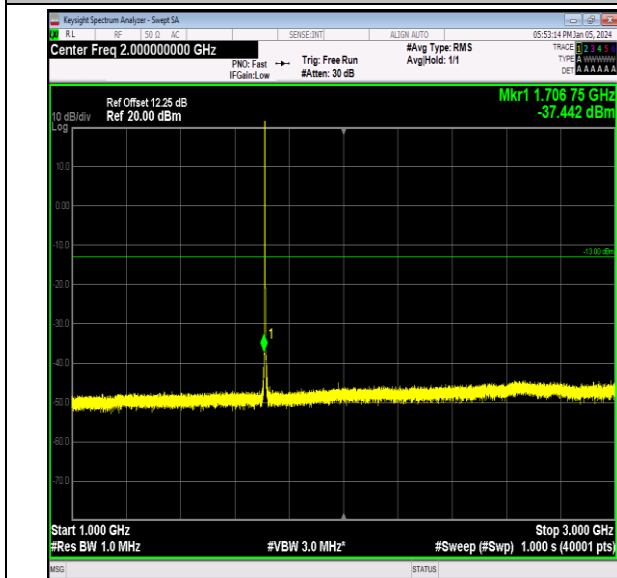
Band66_1.4MHz_QPSK_131979_1RB#0_1000~3000_100
