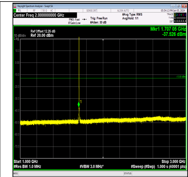
Band66_1.4MHz_16QAM_131979_1RB#0_1000~3000_1000~3000
