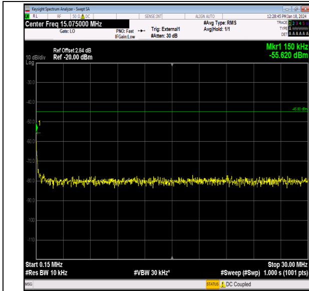
Band41_20MHz_QPSK_40640_1RB#0_0.15~30_0.15~30
