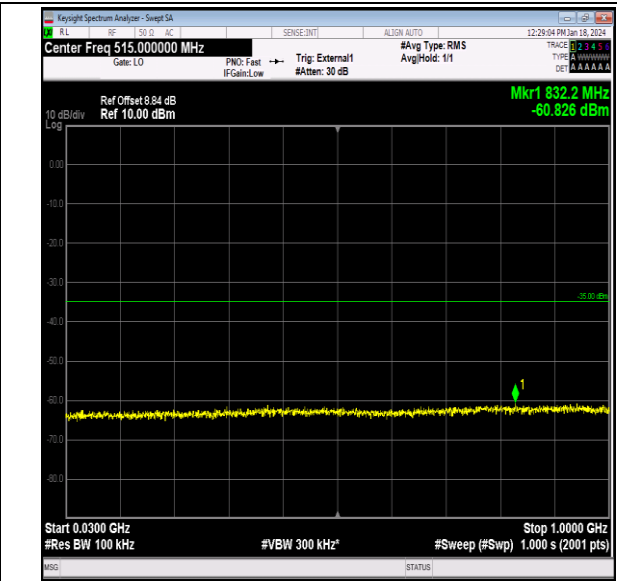
Band41_20MHz_QPSK_40640_1RB#0_30~1000_30~1000 0
