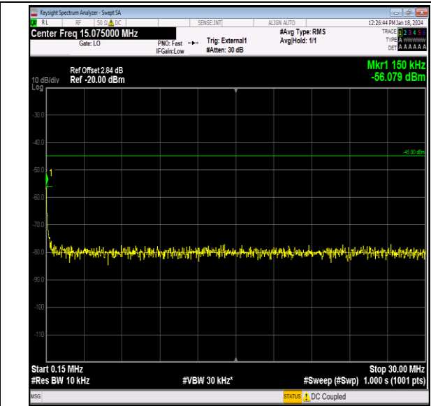
Band41_20MHz_64QAM_40140_1RB#0_0.15~30_0.15~3 0
