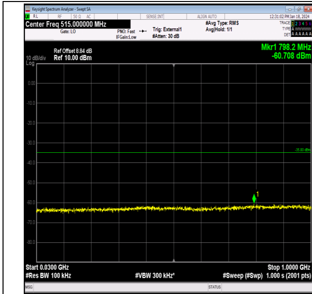
Band41_20MHz_16QAM_40640_1RB#0_30~1000_30~10 00
