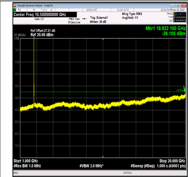
Band41_20MHz_16QAM_40640_1RB#0_1000~20000_10 00~20000
