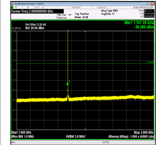
Band66_1.4MHz_QPSK_132322_1RB#0_1000~3000_100 0~3000
