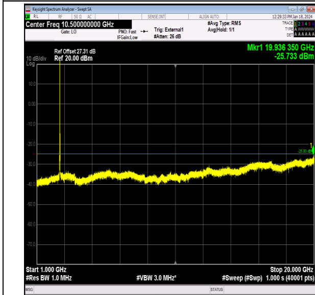
Band41_20MHz_QPSK_40640_1RB#0_1000~20000_1000~20000 0~20000
