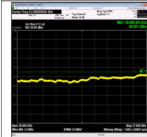
Band41_20MHz_64QAM_41140_1RB#0_20000~27000_2 0000~27000
