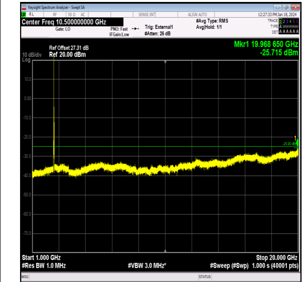
Band41_20MHz_64QAM_40140_1RB#0_1000~20000_10 00~20000
