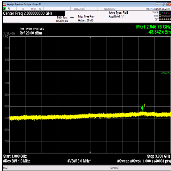
Band26_15MHz_16QAM_26865_1RB#0_1000~3000_100
