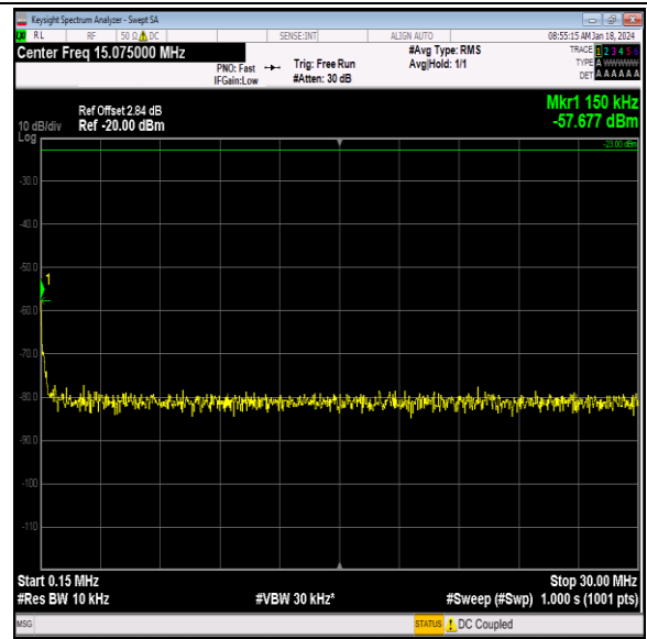
Band26_15MHz_QPSK_26865_1RB#0_0.15~30_0.15~30
