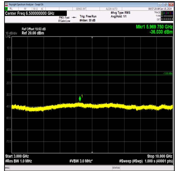
Band26_15MHz_16QAM_26865_1RB#0_3000~10000_30
