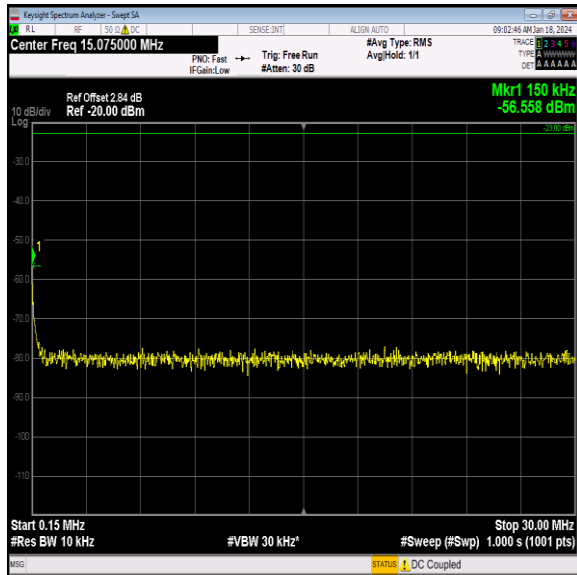
Band26_15MHz_16QAM_26965_1RB#0_0.15~30_0.15~3 0
