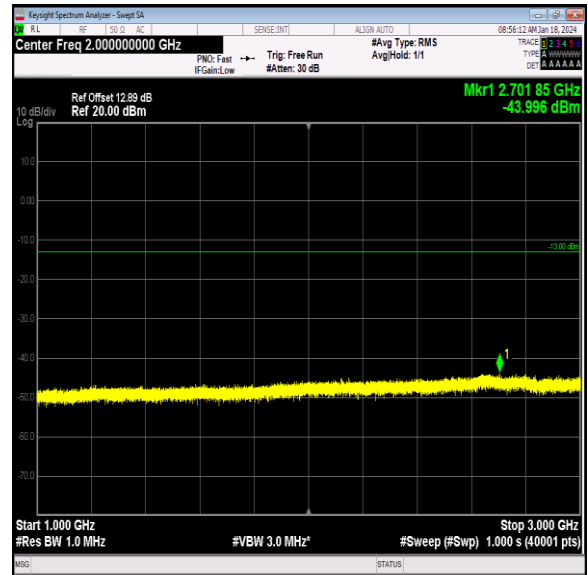
Band26_15MHz_QPSK_26865_1RB#0_1000~3000_1000 ~3000
