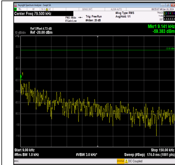
Band26_15MHz_QPSK_26865_1RB#0_0.009~0.15_0.009 ~0.15
