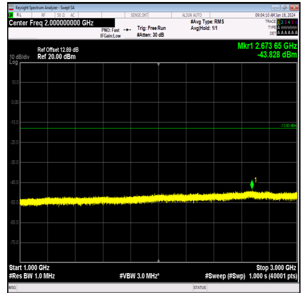
Band26_15MHz_64QAM_26965_1RB#0_1000-3000_1000-3000 0~3000
