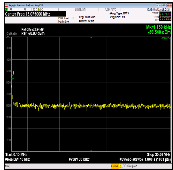
Band26_15MHz_64QAM_26965_1RB#0_0.15-30_0.15-30 0
