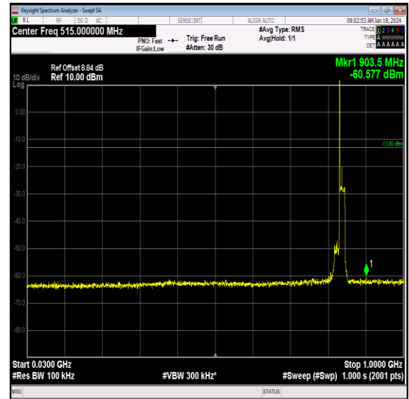
Band26_15MHz_16QAM_26965_1RB#0_30~1000_30~10 00
