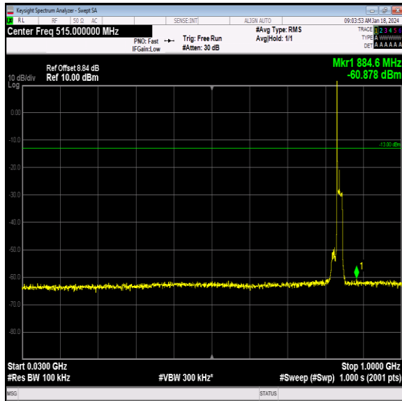
Band26_15MHz_64QAM_26965_1RB#0_30-1000_30-1000 00
