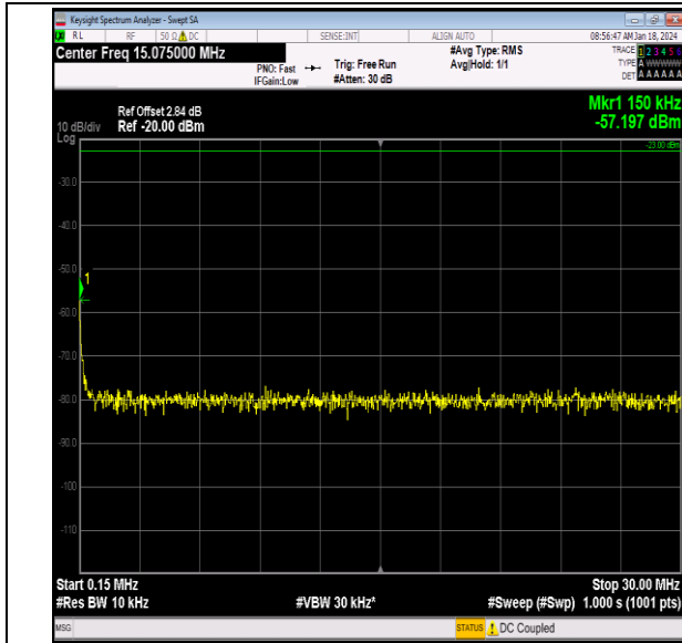
Band26_15MHz_16QAM_26865_1RB#0_0.15~30_0.15~3
