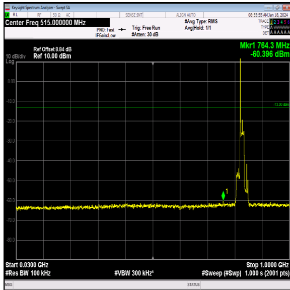
Band26_15MHz_QPSK_26865_1RB#0_30~1000_30~100 0
