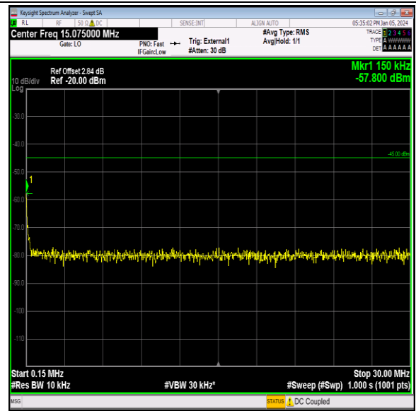
Band41_5MHz_64QAM_41215_1RB#0_0.15~30_0.15~30
