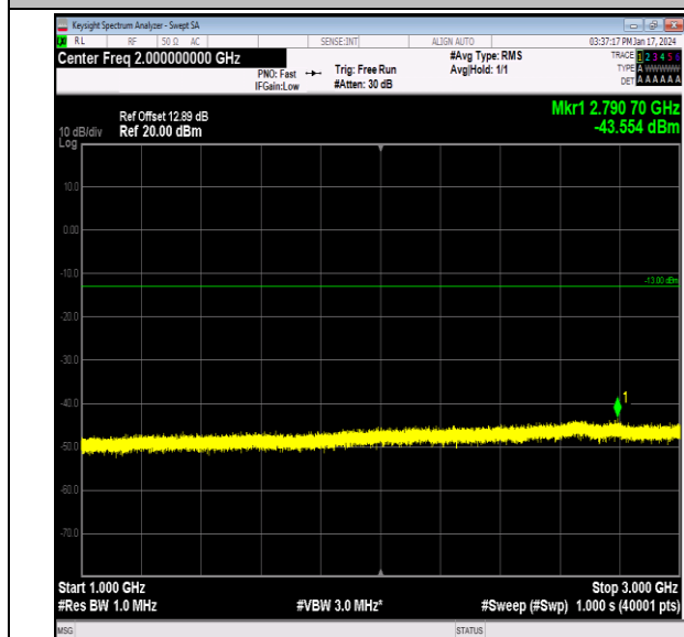
Band26_5MHz_QPSK_26915_1RB#0_1000~3000_1000~3000
