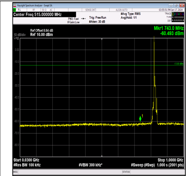
Band26_10MHz_QPSK_26840_1RB#0_30~1000_30~1000 0
