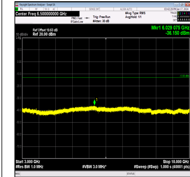
Band26_5MHz_64QAM_27015_1RB#0_3000~10000_300 0~10000
