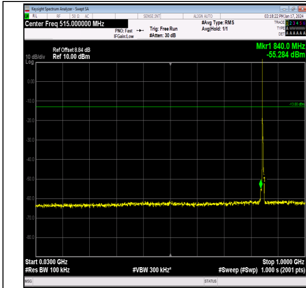
Band26_3MHz_16QAM_27025_1RB#0_30~1000_30~100 0
