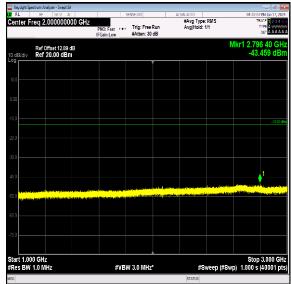
Band26_10MHz_16QAM_26990_1RB#0_1000~3000_100 0~3000
