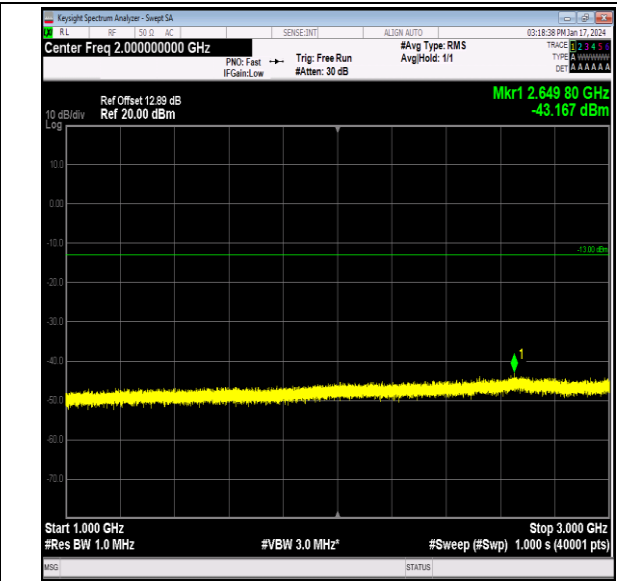
Band26_3MHz_16QAM_27025_1RB#0_1000~3000_1000 ~3000
