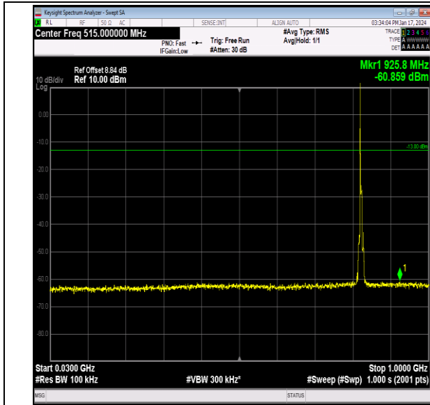
Band26_5MHz_QPSK_26815_1RB#0_30~1000_30~1000
