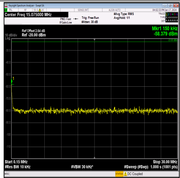
Band26_10MHz_16QAM_26990_1RB#0_0.15~30_0.15~3 0
