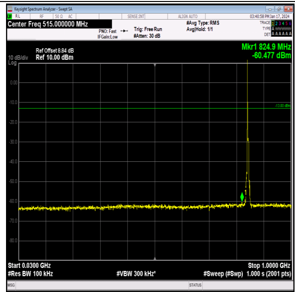
Band26_5MHz_16QAM_27015_1RB#0_30~1000_30~1000 0
