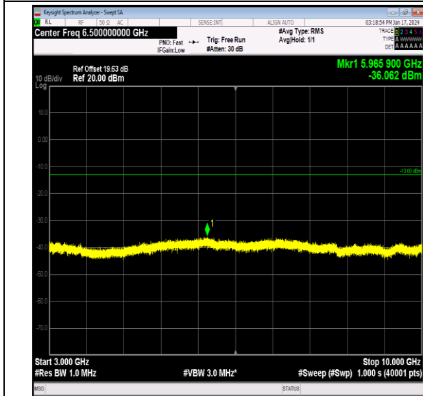
Band26_3MHz_16QAM_27025_1RB#0_3000~10000_300 0~10000
