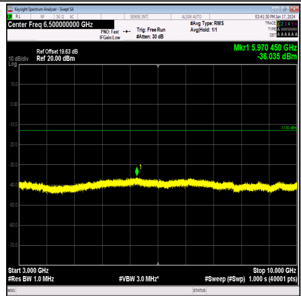
Band26_5MHz_16QAM_27015_1RB#0_3000~10000_3000 0~10000
