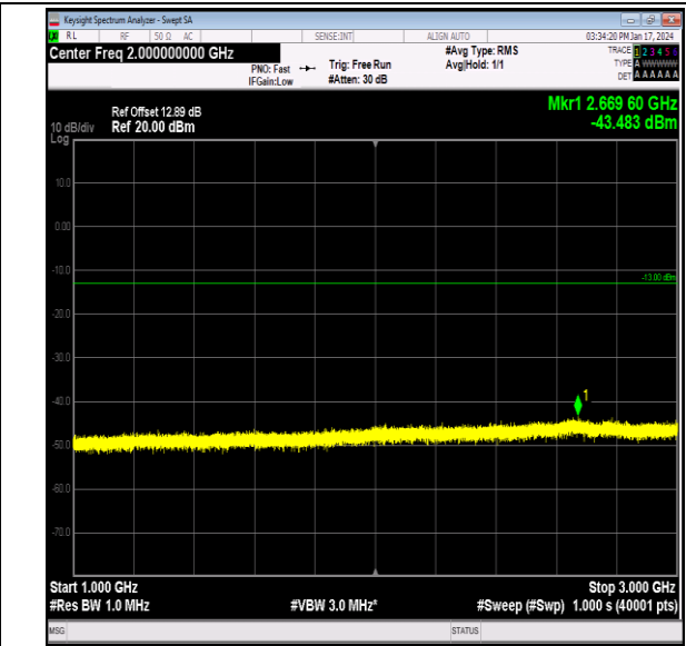
Band26_5MHz_QPSK_26815_1RB#0_1000~3000_1000~3000
