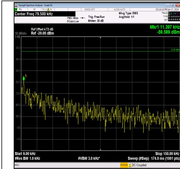
Band26_3MHz_64QAM_26915_1RB#0_0.009~0.15_0.009 ~0.15
