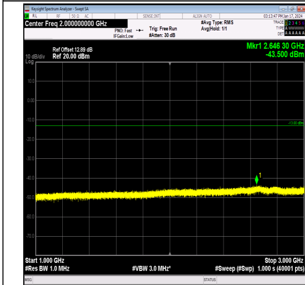
Band26_3MHz_64QAM_26805_1RB#0_1000~3000_1000 ~3000
