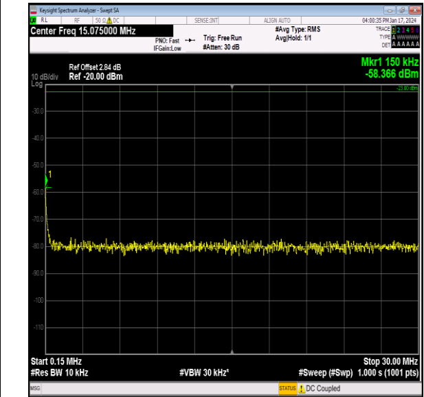
Band26_10MHz_64QAM_26915_1RB#0_0.15~30_0.15~3 0
