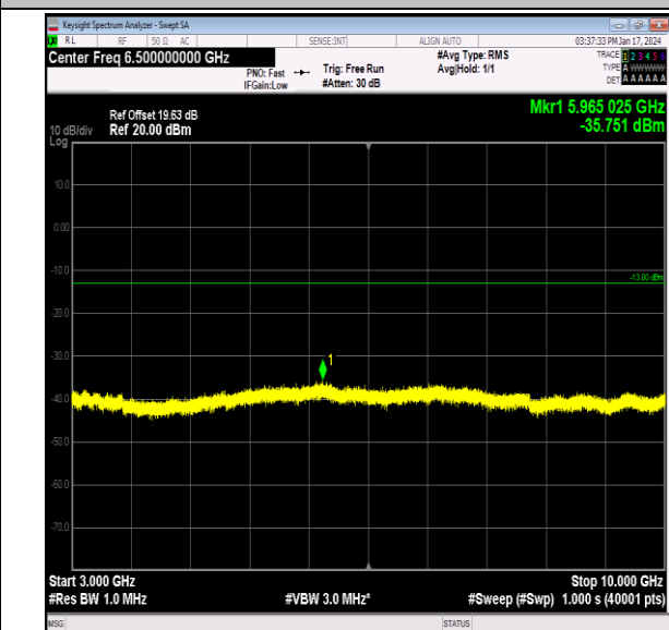
Band26_5MHz_QPSK_26915_1RB#0_3000~10000_3000~10000
