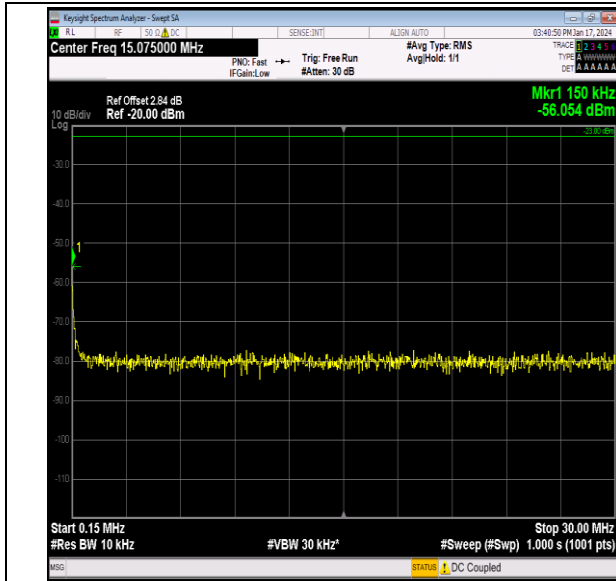
Band26_5MHz_16QAM_27015_1RB#0_0.15~30_0.15~30
