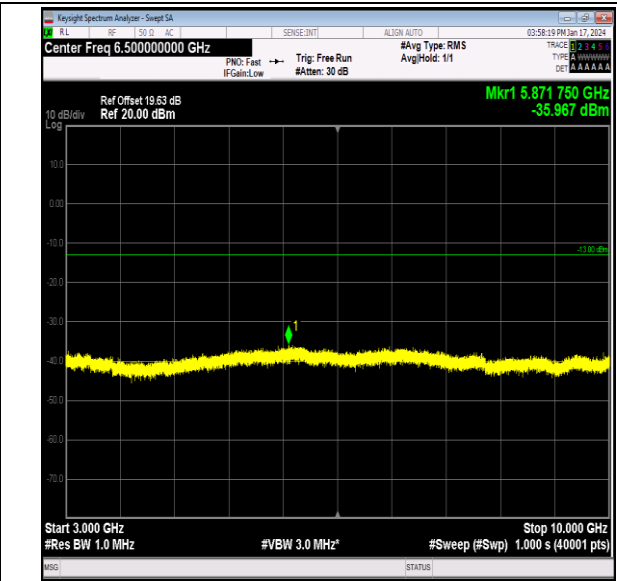
Band26_10MHz_64QAM_26840_1RB#0_3000~10000_30 00~10000
