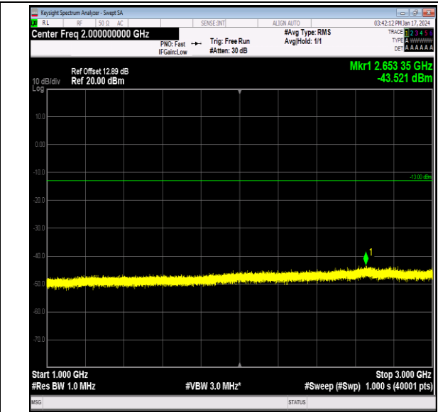
Band26_5MHz_64QAM_27015_1RB#0_1000~3000_1000 ~3000
