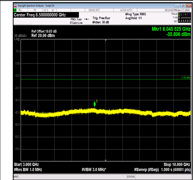
Band26_3MHz_64QAM_26805_1RB#0_3000~10000_3000 0~10000
