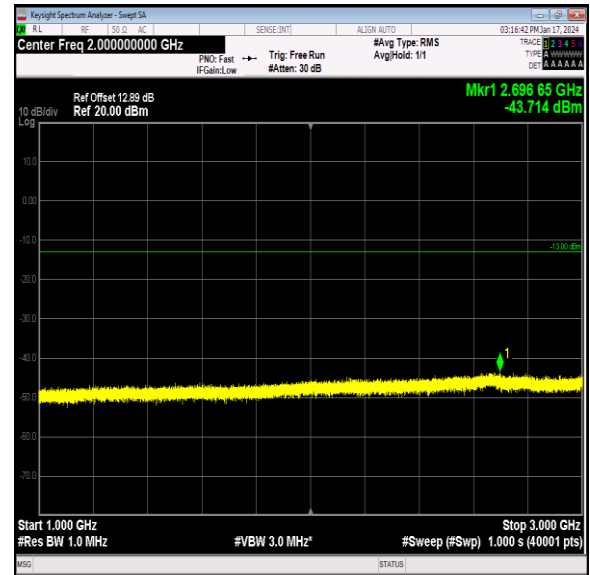
Band26_3MHz_64QAM_26915_1RB#0_1000~3000_1000 ~3000
