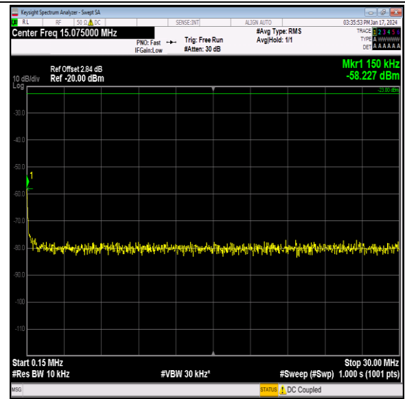
Band26_5MHz_64QAM_26815_1RB#0_0.15~30_0.15~30
