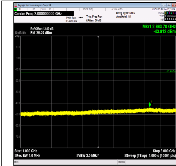
Band26_10MHz_64QAM_26840_1RB#0_1000~3000_100 0~3000
