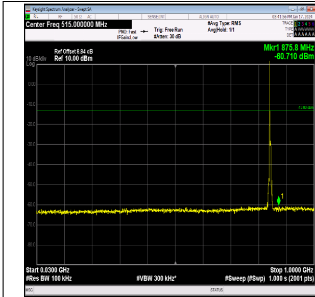
Band26_5MHz_64QAM_27015_1RB#0_30~1000_30~100 0
