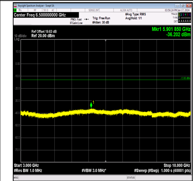
Band26_10MHz_QPSK_26840_1RB#0_3000~10000_3000 0~10000
