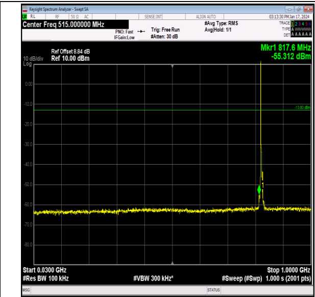
Band26_3MHz_64QAM_26805_1RB#0_30~1000_30~1000 0
