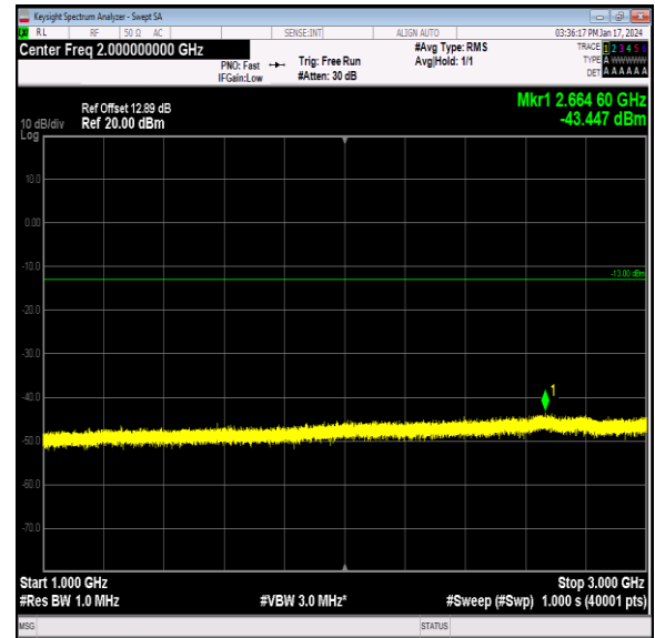
Band26_5MHz_64QAM_26815_1RB#0_1000~3000_1000 ~3000
