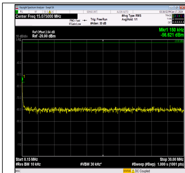
Band26_5MHz_QPSK_26915_1RB#0_0.15~30_0.15~30
