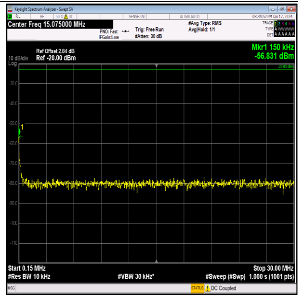
Band26_5MHz_QPSK_27015_1RB#0_0.15~30_0.15~30
