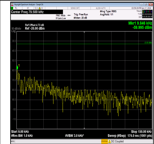
Band26_10MHz_16QAM_26915_1RB#0_0.009~0.15_0.00 9~0.15
