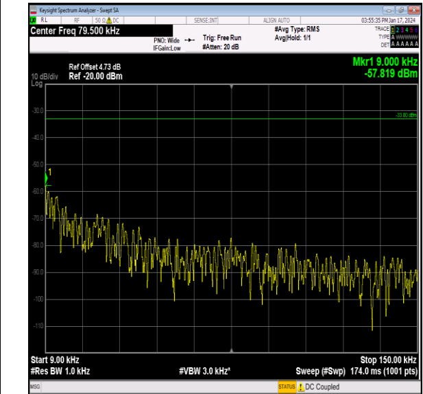
Band26_10MHz_QPSK_26840_1RB#0_0.009~0.15_0.009 ~0.15
