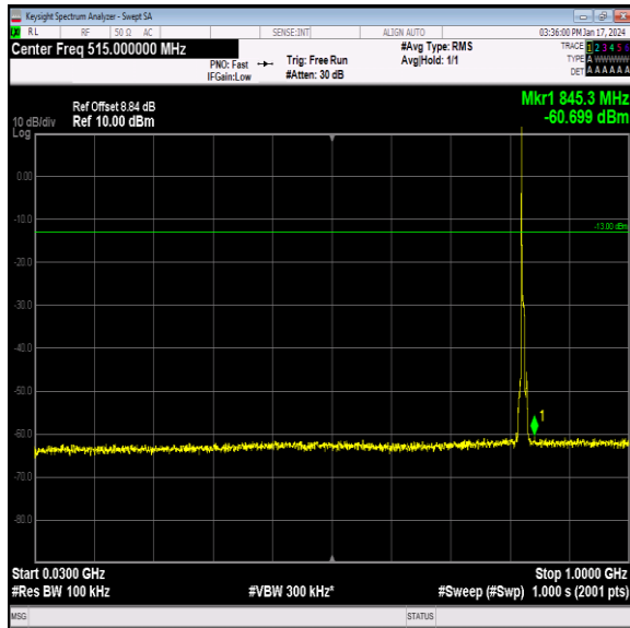
Band26_5MHz_64QAM_26815_1RB#0_30~1000_30~100 0
