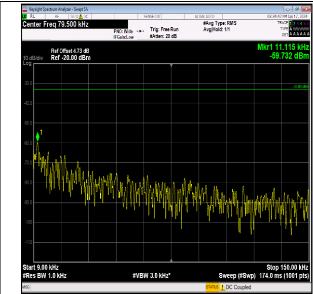
Band26_5MHz_16QAM_26815_1RB#0_0.009~0.15_0.009 ~0.15
