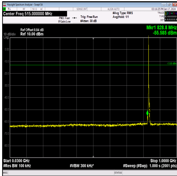
Band26_3MHz_64QAM_26915_1RB#0_30~1000_30~100 0
