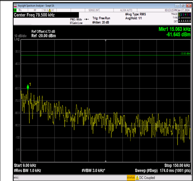
Band26_3MHz_64QAM_26805_1RB#0_0.009~0.15_0.009 ~0.15
