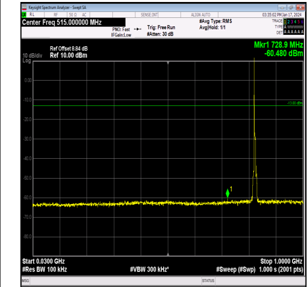
Band26_5MHz_16QAM_26815_1RB#0_30~1000_30~100 0
