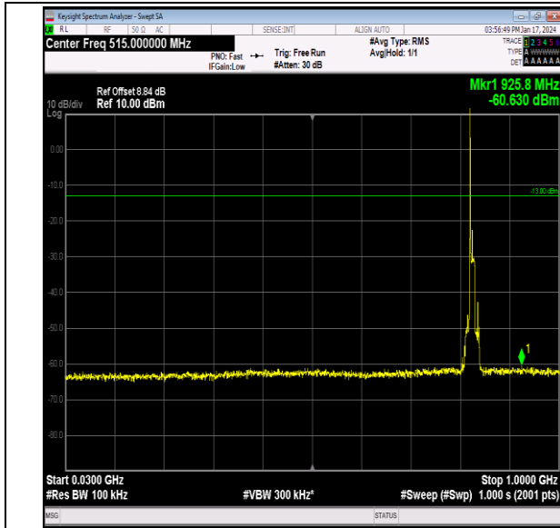
Band26_10MHz_16QAM_26840_1RB#0_30~1000_30~10 00
