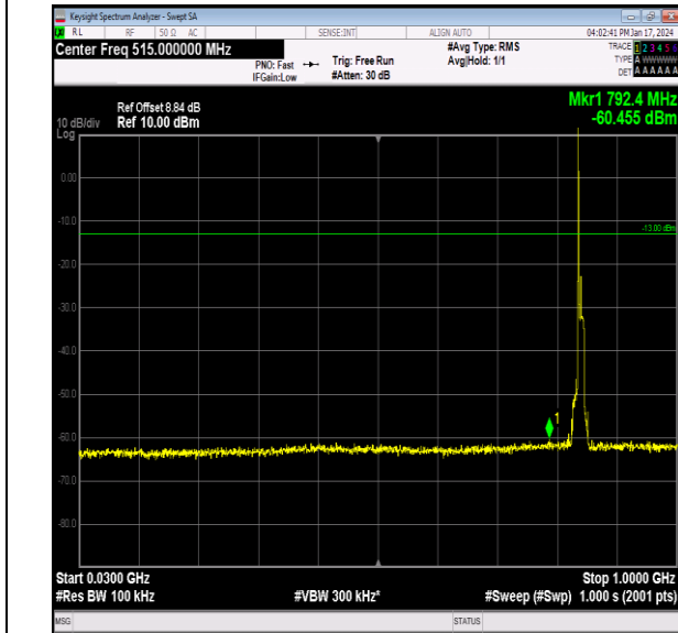
Band26_10MHz_16QAM_26990_1RB#0_30~1000_30~10 00
