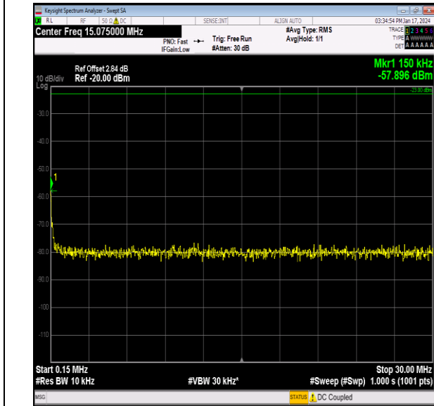
Band26_5MHz_16QAM_26815_1RB#0_0.15~30_0.15~30
