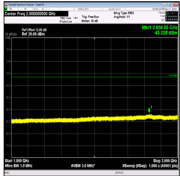
Band26_5MHz_QPSK_27015_1RB#0_1000~3000_1000~3000
