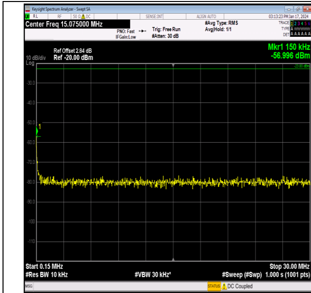
Band26_3MHz_64QAM_26805_1RB#0_0.15~30_0.15~30
