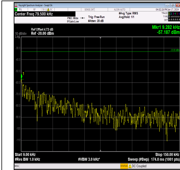
Band26_10MHz_16QAM_26990_1RB#0_0.009~0.15_0.00 9~0.15
