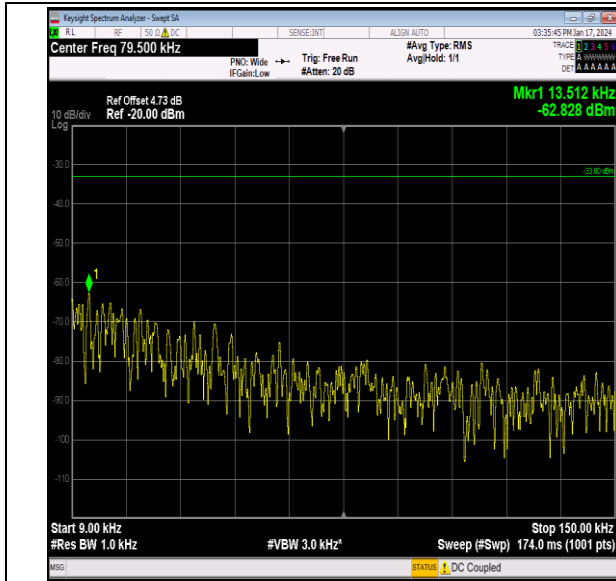
Band26_5MHz_64QAM_26815_1RB#0_0.009~0.15_0.009 ~0.15
