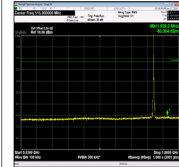
Band26_5MHz_QPSK_27015_1RB#0_30~1000_30~1000
