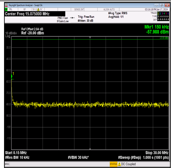
Band26_3MHz_64QAM_26915_1RB#0_0.15~30_0.15~30
