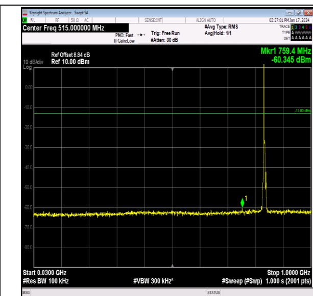
Band26_5MHz_QPSK_26915_1RB#0_30~1000_30~1000
