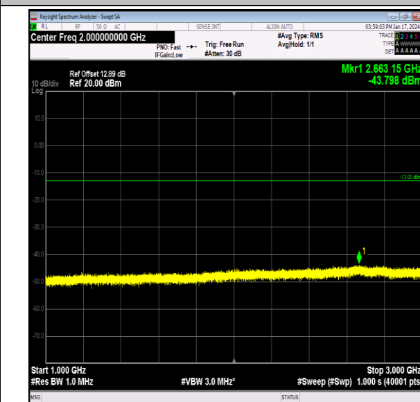
Band26_10MHz_QPSK_26915_1RB#0_1000~3000_1000 ~3000
