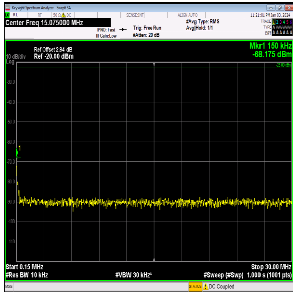
Band26_10MHz_QPSK_26740_1RB#0_0.15~30_0.15~30
