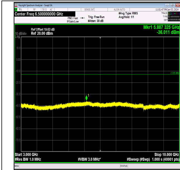
Band26_5MHz_64QAM_26765_1RB#0_3000~10000_300 0~10000
