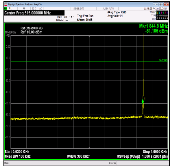
Band26_1.4MHz_16QAM_27033_1RB#0_30~1000_30~1 000
