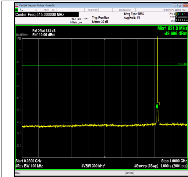
Band26_1.4MHz_64QAM_26797_1RB#0_30~1000_30~1 000
