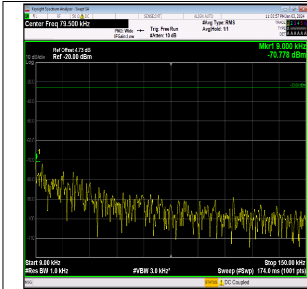
Band26_5MHz_64QAM_26765_1RB#0_0.009~0.15_0.009 ~0.15
