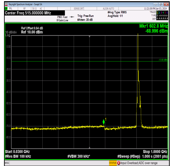
Band26_10MHz_QPSK_26740_1RB#0_30~1000_30~100 0
