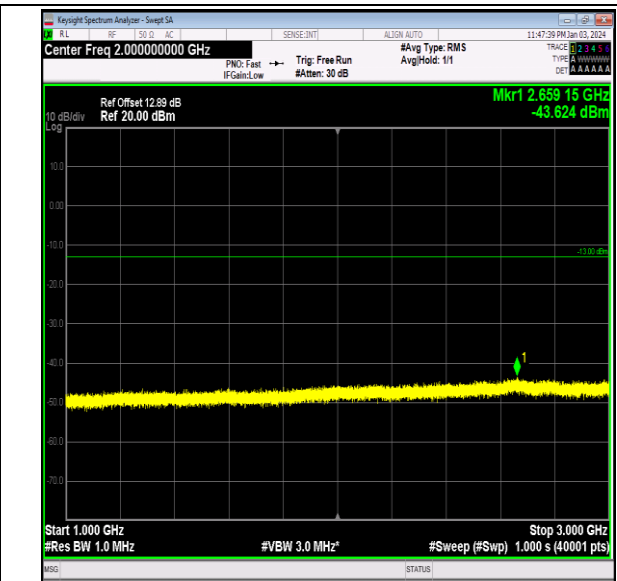
Band26_1.4MHz_QPSK_27033_1RB#0_1000~3000_1000 ~3000
