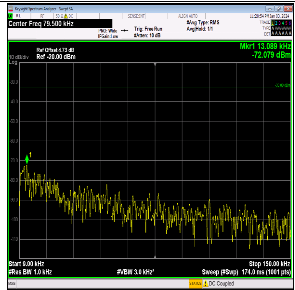
Band26_10MHz_QPSK_26740_1RB#0_0.009~0.15_0.009 ~0.15
