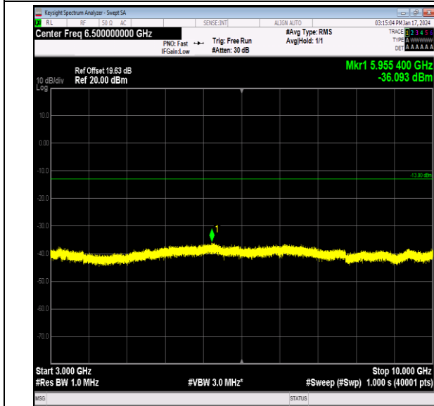
Band26_3MHz_QPSK_26915_1RB#0_3000~10000_3000~10000
