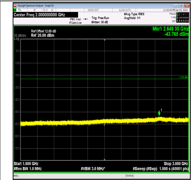
Band26_1.4MHz_64QAM_26797_1RB#0_1000~3000_100 0~3000
