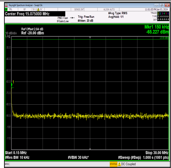
Band26_5MHz_64QAM_26765_1RB#0_0.15~30_0.15~30
