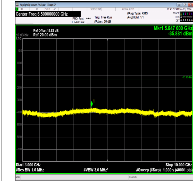
Band26_1.4MHz_64QAM_26797_1RB#0_3000~10000_30 00~10000
