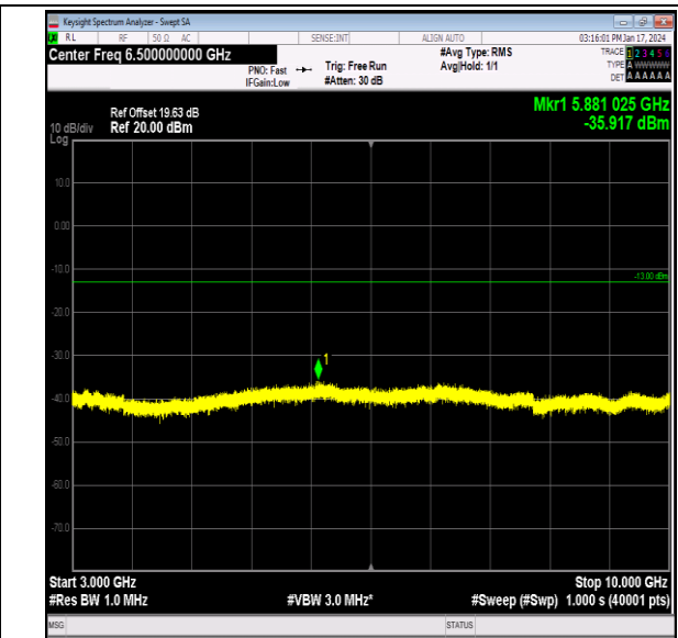
Band26_3MHz_16QAM_26915_1RB#0_3000~10000_300 0~10000
