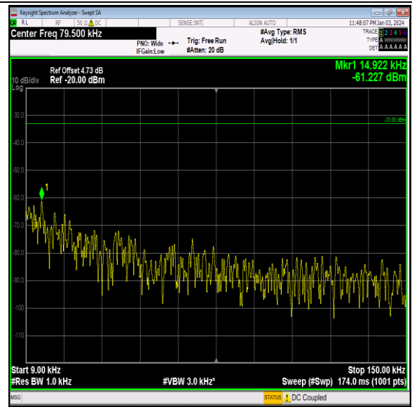
Band26_1.4MHz_16QAM_27033_1RB#0_0.009~0.15_0.0 09~0.15
