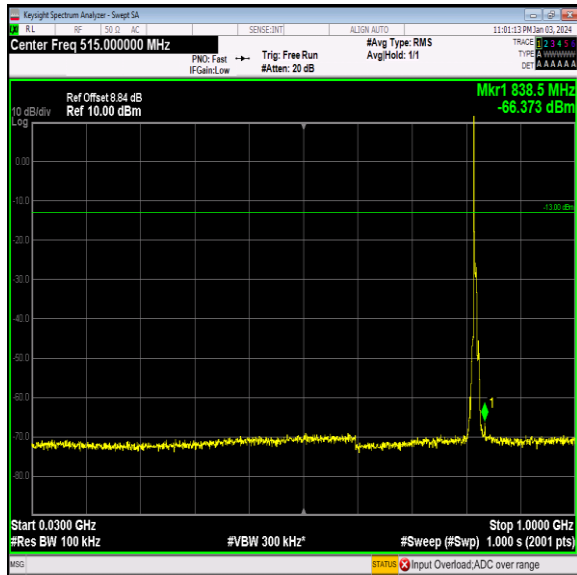
Band26_5MHz_64QAM_26765_1RB#0_30~1000_30~100 0
