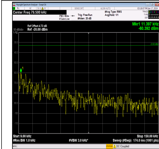
Band26_3MHz_16QAM_27025_1RB#0_0.009~0.15_0.009 ~0.15
