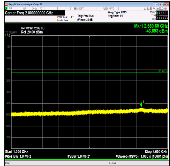
Band26_5MHz_64QAM_26765_1RB#0_1000~3000_1000 ~3000
