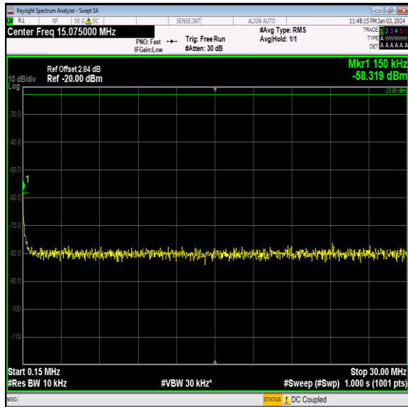
Band26_1.4MHz_16QAM_27033_1RB#0_0.15~30_0.15~ 30
