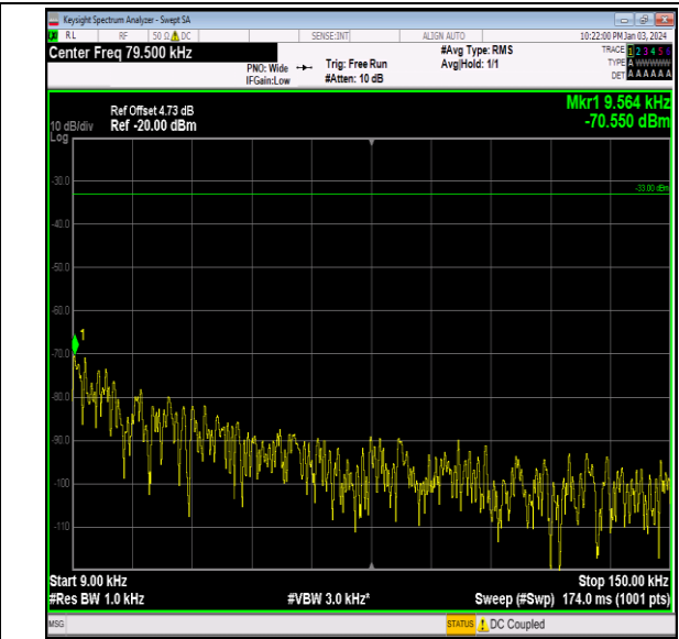
Band26_3MHz_QPSK_26775_1RB#0_0.009~0.15_0.009~ 0.15
