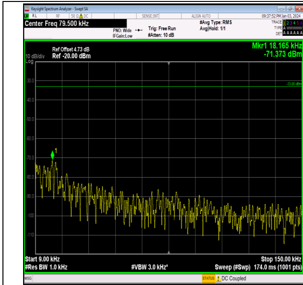
Band26_1.4MHz_64QAM_26697_1RB#0_0.009~0.15_0.0 09~0.15
