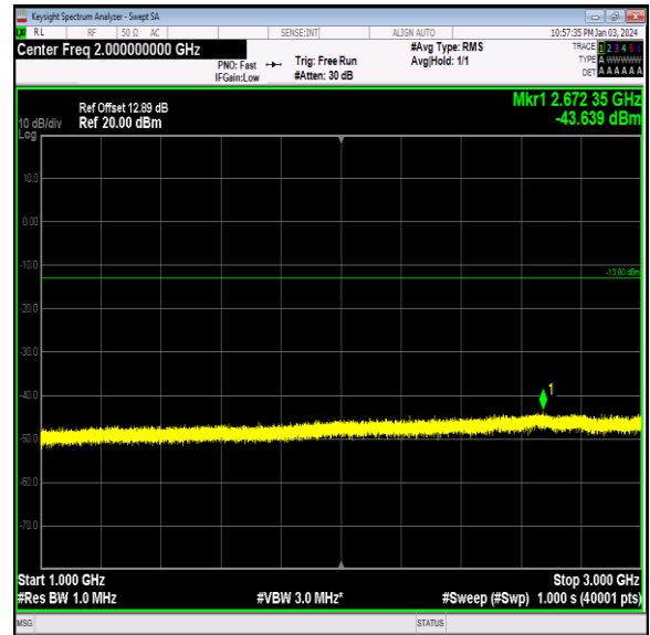
Band26_5MHz_16QAM_26740_1RB#0_1000~3000_1000 ~3000
