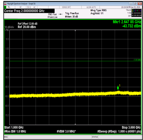
Band26_3MHz_QPSK_26740_1RB#0_1000~3000_1000~3000
