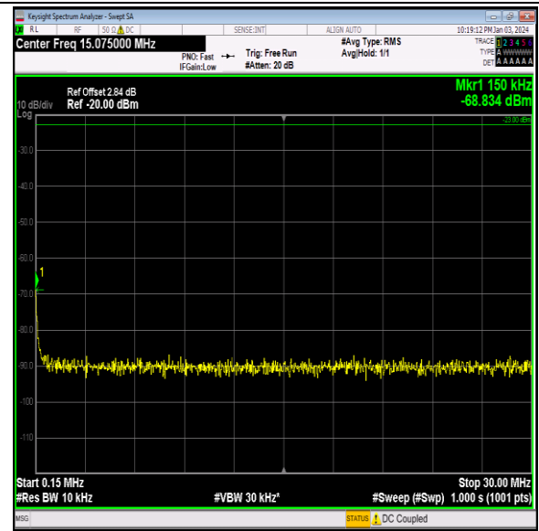
Band26_3MHz_QPSK_26740_1RB#0_0.15~30_0.15~30
