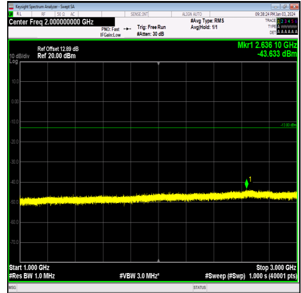
Band26_1.4MHz_64QAM_26697_1RB#0_1000~3000_100 0~3000
