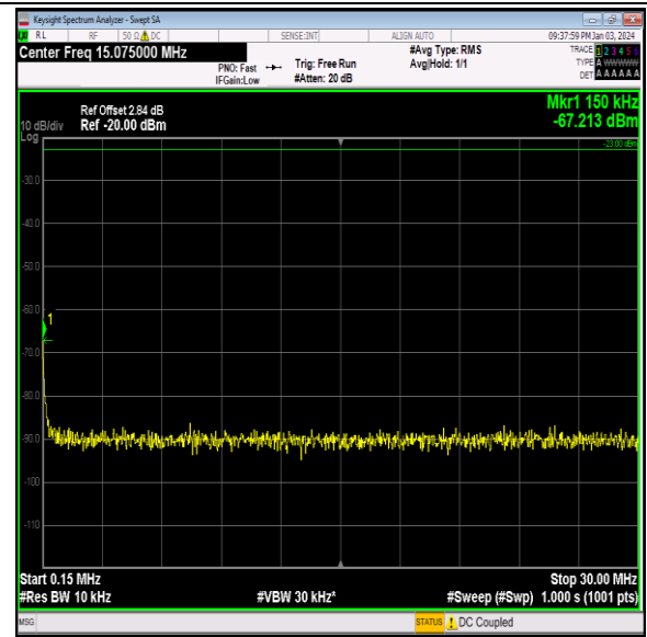
Band26_1.4MHz_64QAM_26697_1RB#0_0.15~30_0.15~ 30
