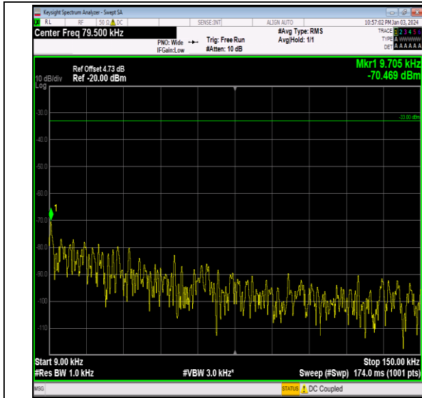
Band26_5MHz_16QAM_26740_1RB#0_0.009~0.15_0.009 ~0.15
