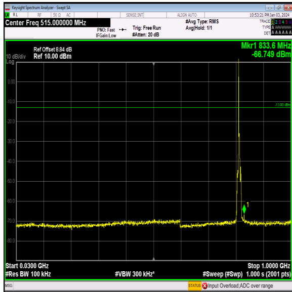
Band26_5MHz_QPSK_26715_1RB#0_30~1000_30~1000
