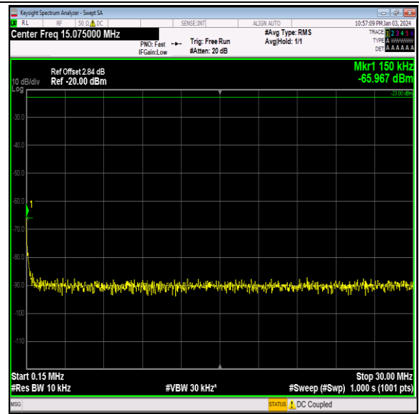
Band26_5MHz_16QAM_26740_1RB#0_0.15~30_0.15~30
