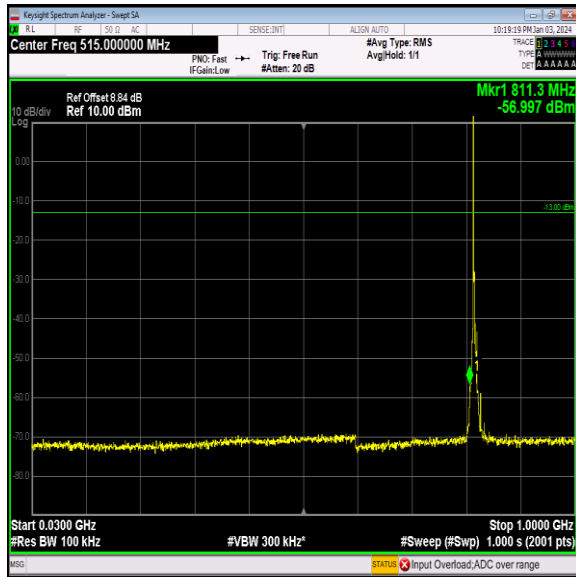
Band26_3MHz_QPSK_26740_1RB#0_30~1000_30~1000
