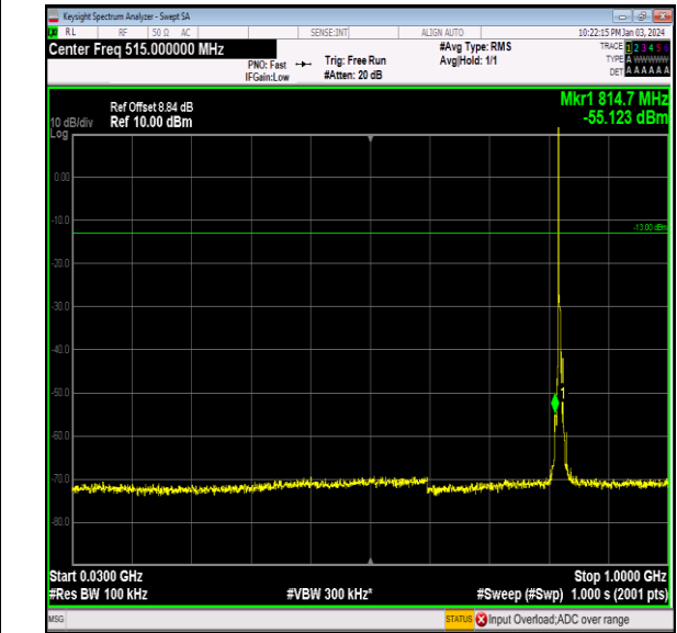
Band26_3MHz_QPSK_26775_1RB#0_30~1000_30~1000
