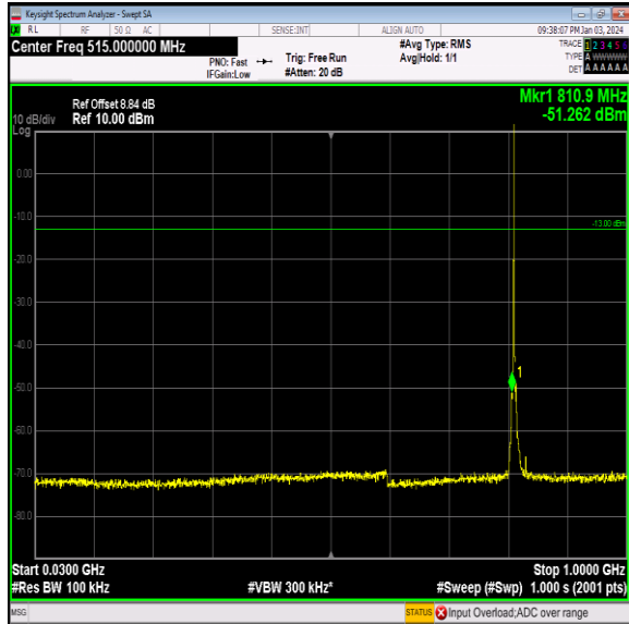
Band26_1.4MHz_64QAM_26697_1RB#0_30~1000_30~1 000
