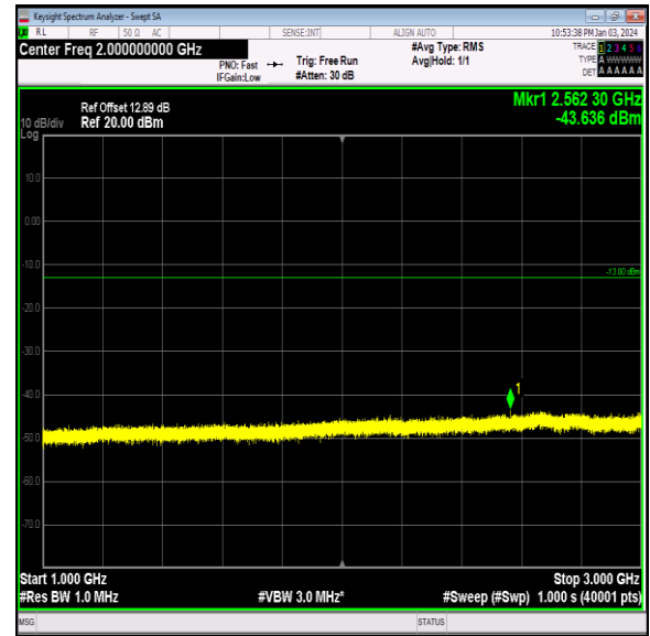
Band26_5MHz_QPSK_26715_1RB#0_1000~3000_1000~3000
