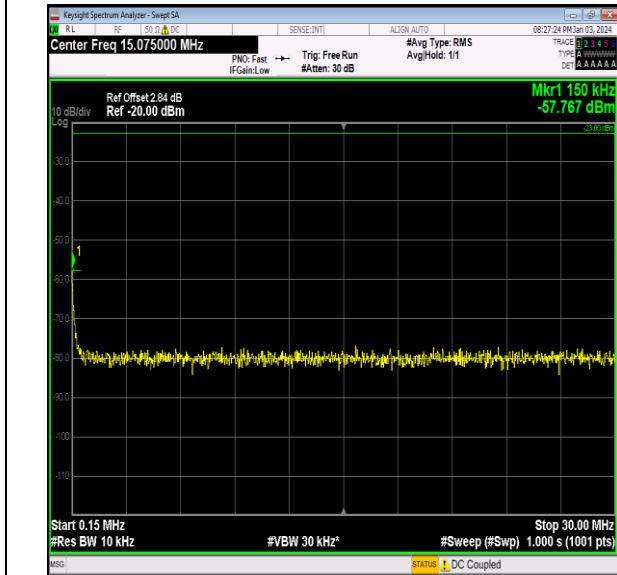
Band12_5MHz_QPSK_23095_1RB#0_0.15~30_0.15~30
