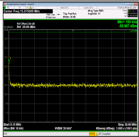
Band12_3MHz_16QAM_23165_1RB#0_0.15~30_0.15~30
