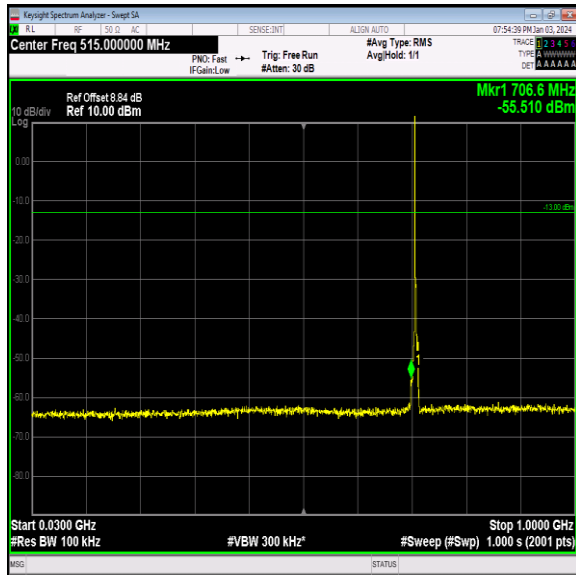
Band12_3MHz_16QAM_23165_1RB#0_30~1000_30~100 0
