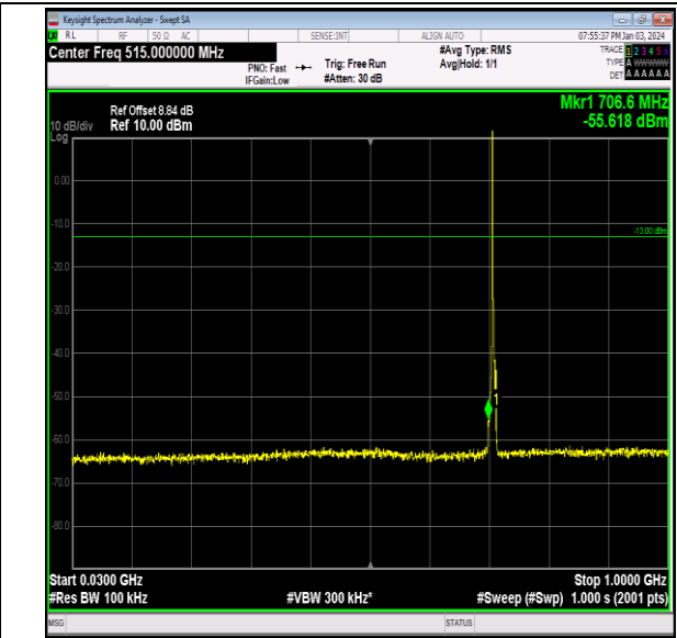
Band12_3MHz_64QAM_23165_1RB#0_30~1000_30~1000 0
