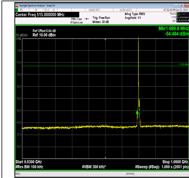
Band12_3MHz_64QAM_23095_1RB#0_30~1000_30~100 0
