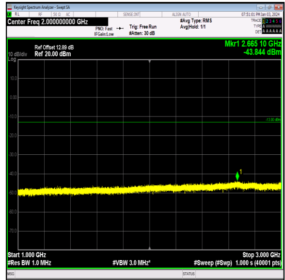
Band12_3MHz_QPSK_23095_1RB#0_1000~3000_1000~3000
