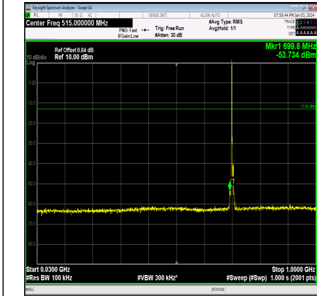
Band12_3MHz_QPSK_23095_1RB#0_30~1000_30~1000
