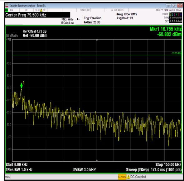
Band12_5MHz_QPSK_23095_1RB#0_0.009~0.15_0.009~ 0.15
