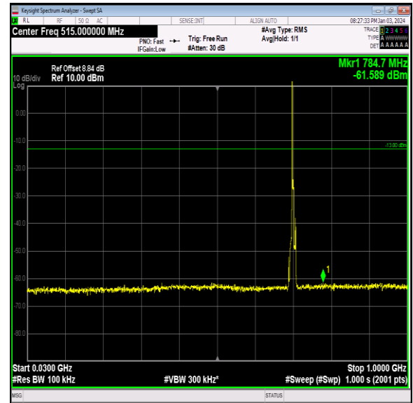
Band12_5MHz_QPSK_23095_1RB#0_30~1000_30~1000
