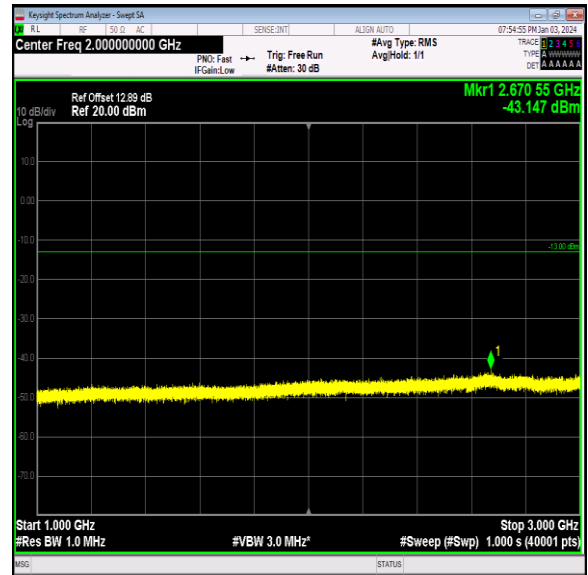
Band12_3MHz_16QAM_23165_1RB#0_1000~3000_1000 ~3000
