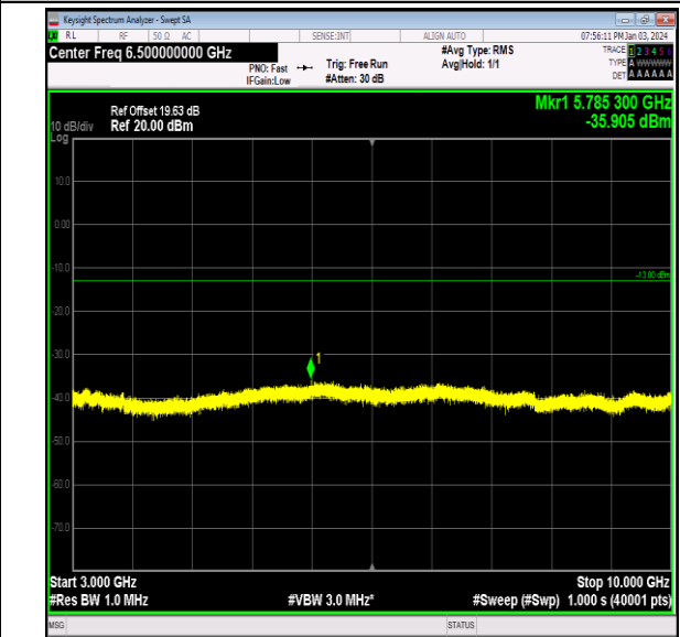
Band12_3MHz_64QAM_23165_1RB#0_3000~10000_3000 0~10000
