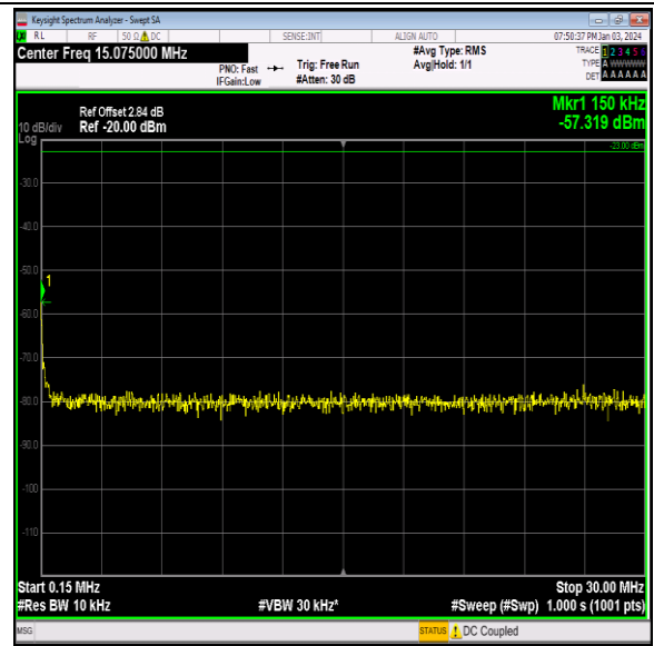
Band12_3MHz_QPSK_23095_1RB#0_0.15~30_0.15~30
