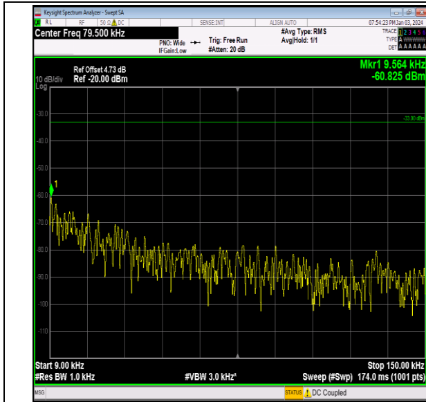
Band12_3MHz_16QAM_23165_1RB#0_0.009~0.15_0.009 ~0.15
