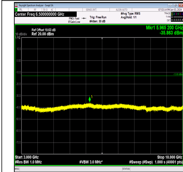
Band12_3MHz_64QAM_23095_1RB#0_3000~10000_300 0~10000
