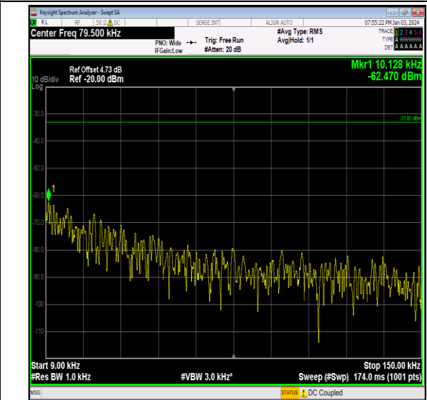
Band12_3MHz_64QAM_23165_1RB#0_0.009~0.15_0.009 ~0.15
