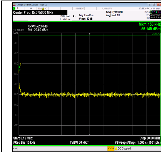
Band12_3MHz_64QAM_23165_1RB#0_0.15~30_0.15~30
