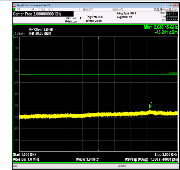
Band12_3MHz_64QAM_23095_1RB#0_1000~3000_1000 ~3000
