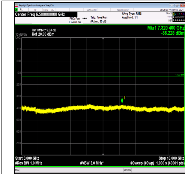
Band12_5MHz_QPSK_23035_1RB#0_3000~10000_3000 ~10000
