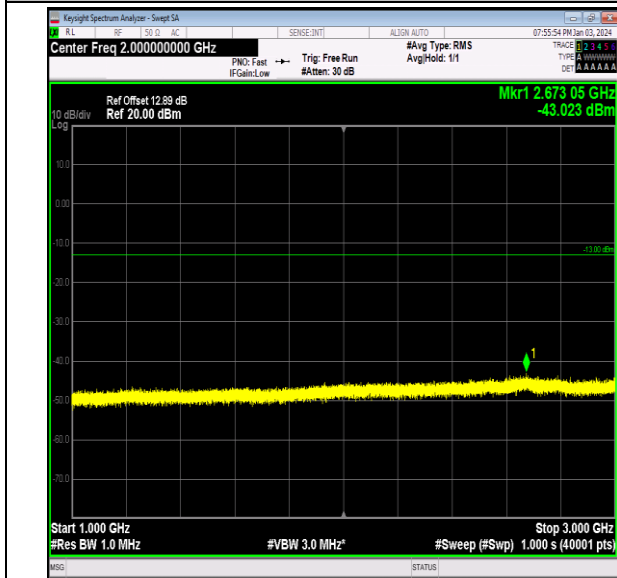
Band12_3MHz_64QAM_23165_1RB#0_1000~3000_1000 ~3000
