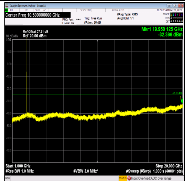
Band7_10MHz_16QAM_21400_1RB#0_1000~20000_100 0~20000
