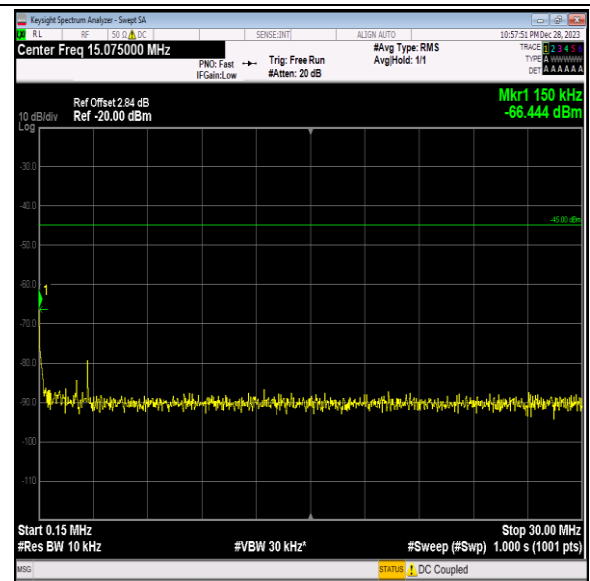
Band7_10MHz_16QAM_21400_1RB#0_0.15~30_0.15~30
