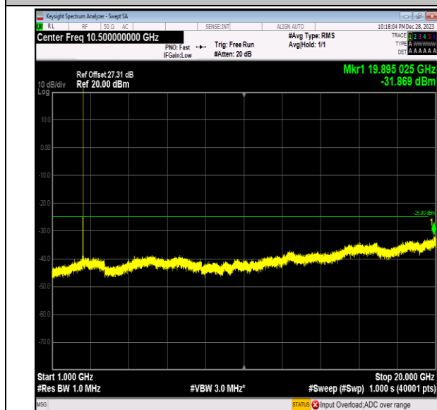
Band7_5MHz_QPSK_21100_1RB#0_1000~20000_1000~20000
