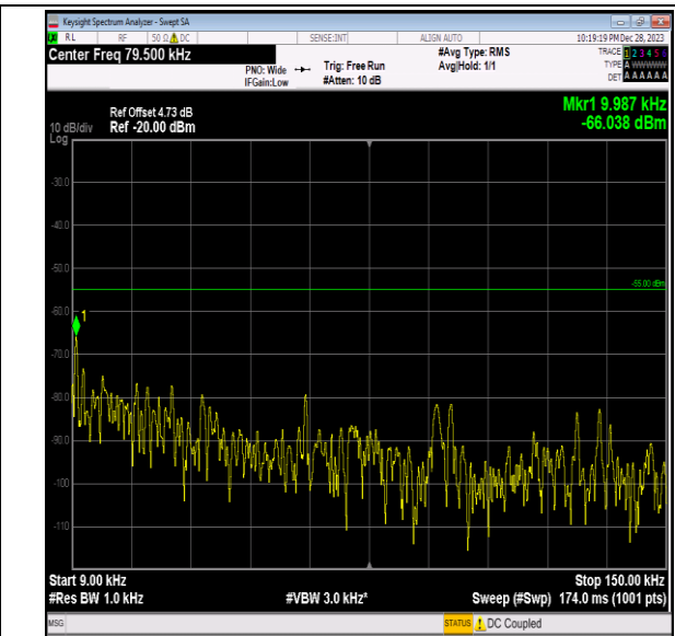
Band7_5MHz_64QAM_21100_1RB#0_0.009~0.15_0.009~ 0.15
