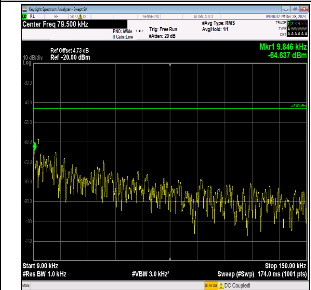
Band2_20MHz_64QAM_18700_1RB#0_0.009~0.15_0.009 ~0.15
