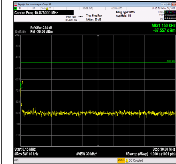
Band7_5MHz_16QAM_20775_1RB#0_0.15~30_0.15~30
