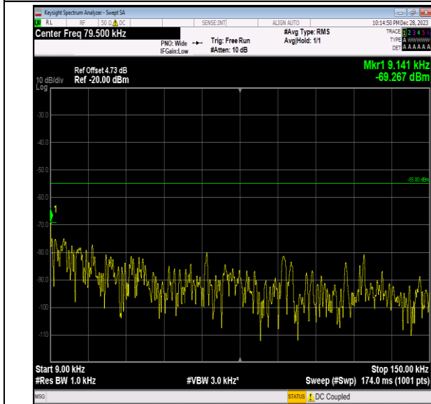
Band7_5MHz_QPSK_20775_1RB#0_0.009~0.15_0.009~0.15
