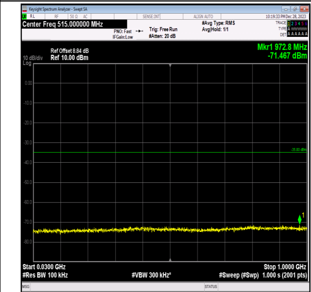
Band7_5MHz_64QAM_21100_1RB#0_30~1000_30~1000
