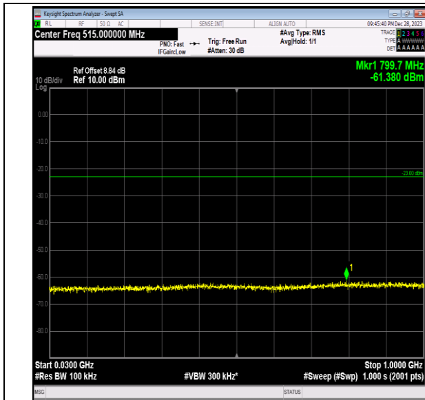
Band2_20MHz_16QAM_19100_1RB#0_30~1000_30~100 0
