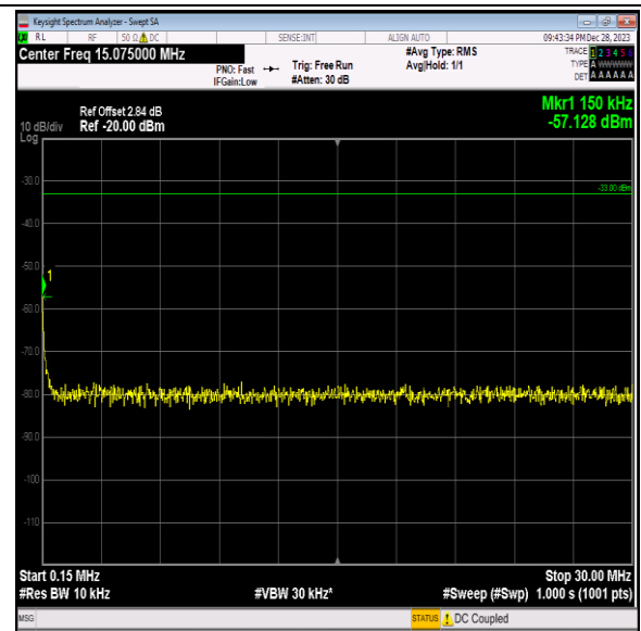
Band2_20MHz_64QAM_18900_1RB#0_0.15~30_0.15~30
