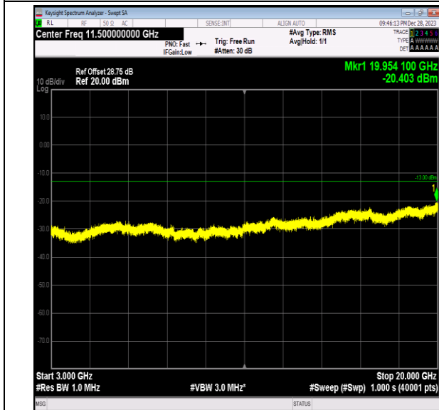
Band2_20MHz_16QAM_19100_1RB#0_3000~20000_300 0~20000
