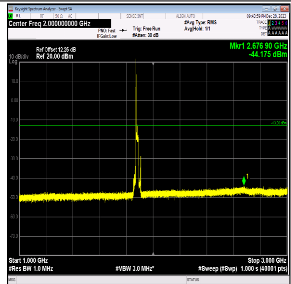
Band2_20MHz_64QAM_18900_1RB#0_1000~3000_1000 ~3000
