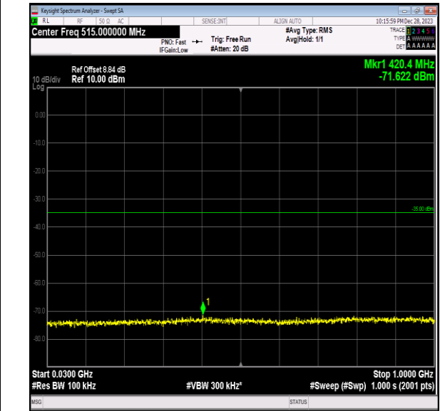
Band7_5MHz_16QAM_20775_1RB#0_30~1000_30~1000
