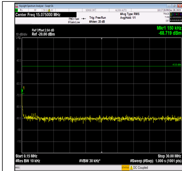
Band7_5MHz_QPSK_21100_1RB#0_0.15~30_0.15~30
