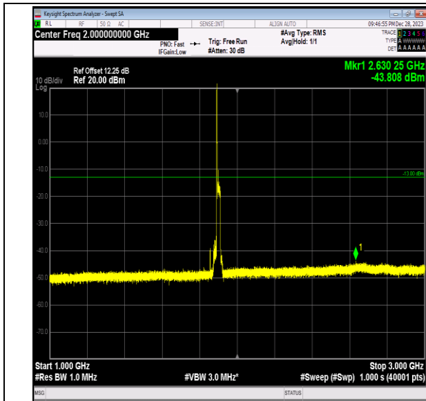
Band2_20MHz_64QAM_19100_1RB#0_1000~3000_1000 ~3000
