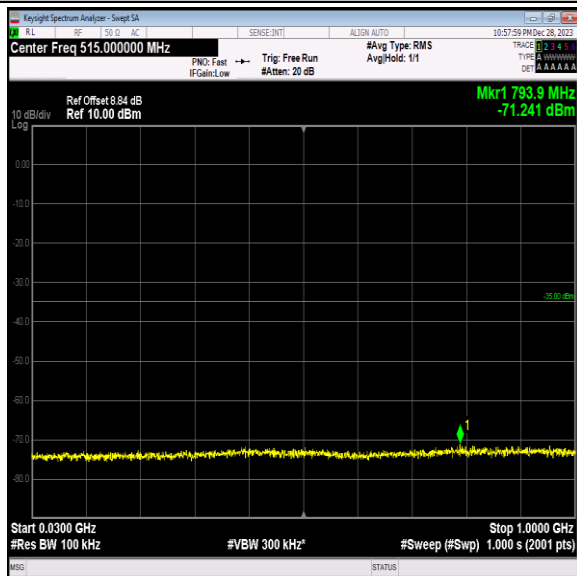
Band7_10MHz_16QAM_21400_1RB#0_30~1000_30~100 0
