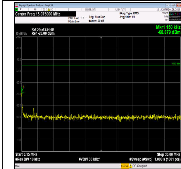
Band7_5MHz_64QAM_21100_1RB#0_0.15~30_0.15~30
