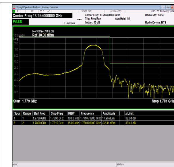
Band66_1.4MHz_64QAM_132665_1RB#5
