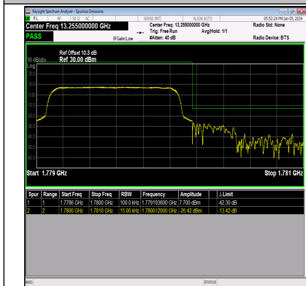
Band66_1.4MHz_64QAM_132665_6RB#0
