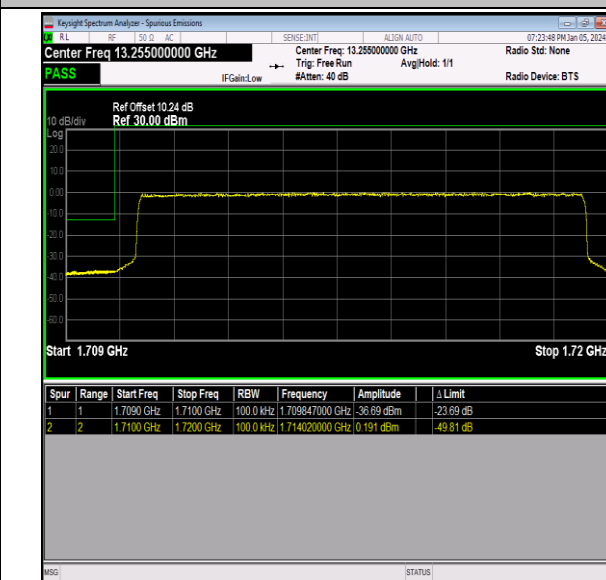
Band66_10MHz_16QAM_132022_50RB#0
