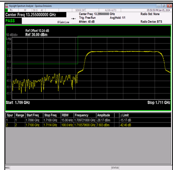
Band66_1.4MHz_64QAM_131979_6RB#0
