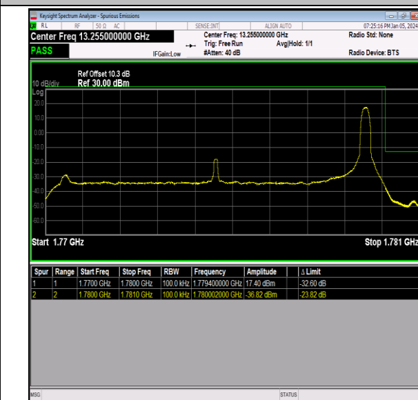
Band66_10MHz_64QAM_132622_1RB#49
