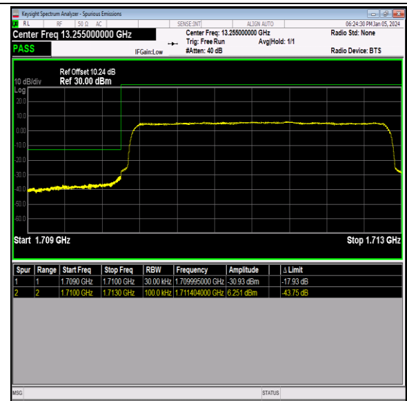
Band66_3MHz_QPSK_131987_15RB#0
