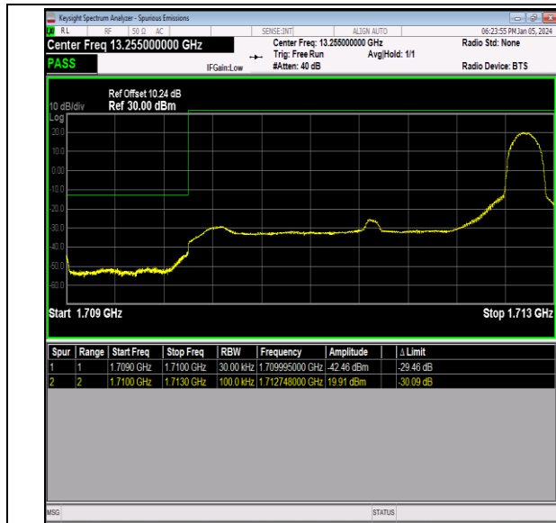
Band66_3MHz_QPSK_131987_1RB#14
