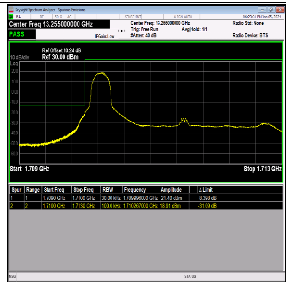
Band66_3MHz_16QAM_131987_1RB#0
