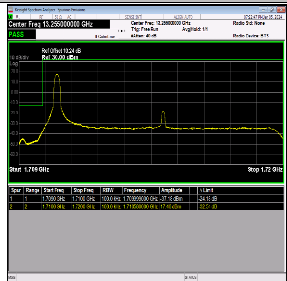
Band66_10MHz_64QAM_132022_1RB#0
