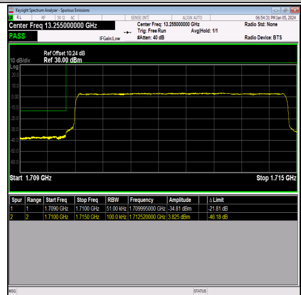
Band66_5MHz_QPSK_131997_25RB#0
