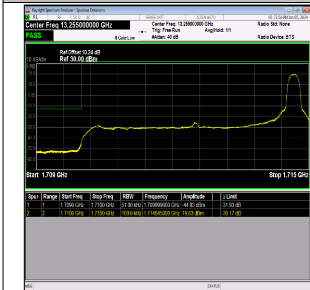
Band66_5MHz_QPSK_131997_1RB#24
