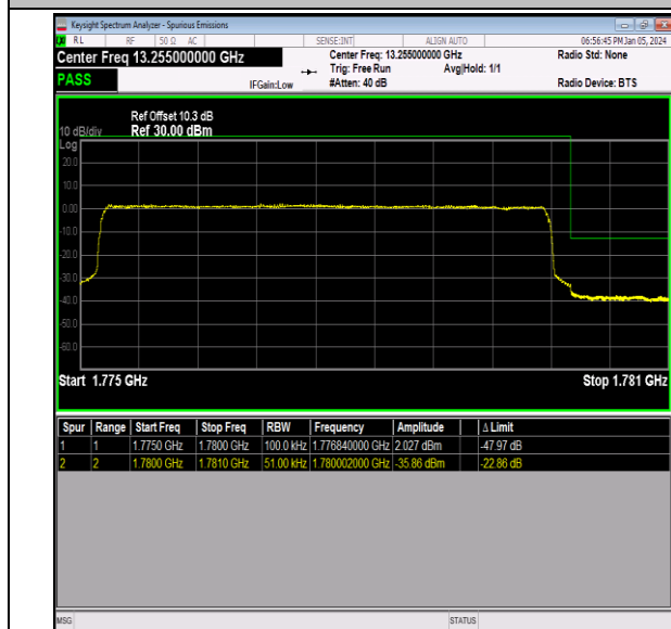
Band66_5MHz_64QAM_132647_25RB#0
