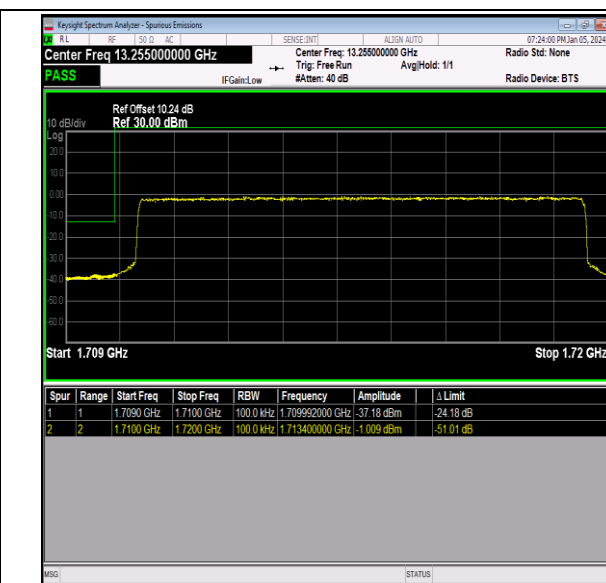
Band66_10MHz_64QAM_132022_50RB#0
