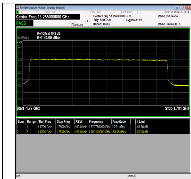
Band66_10MHz_QPSK_132622_50RB#0
