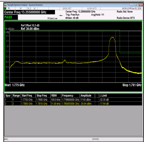
Band66_5MHz_64QAM_132647_1RB#24
