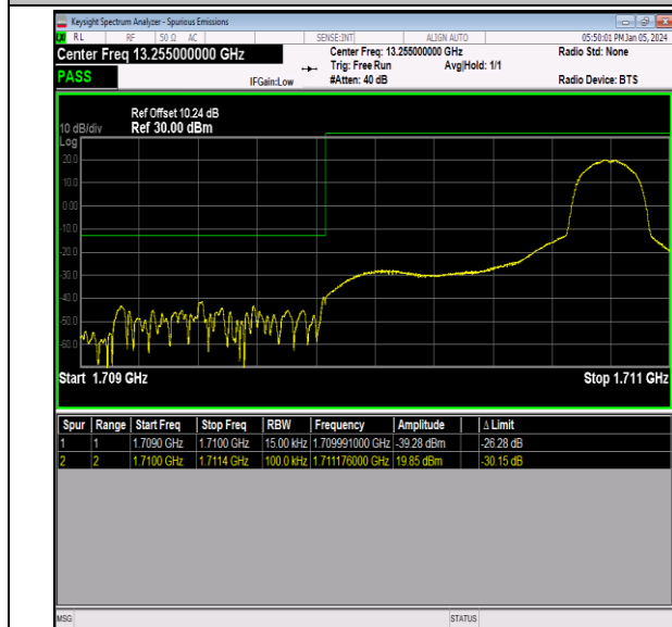
Band66_1.4MHz_QPSK_131979_1RB#5
