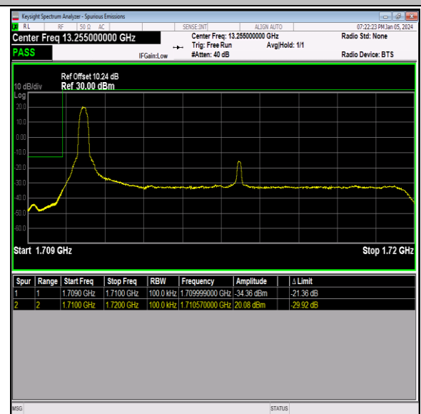
Band66_10MHz_QPSK_132022_1RB#0
