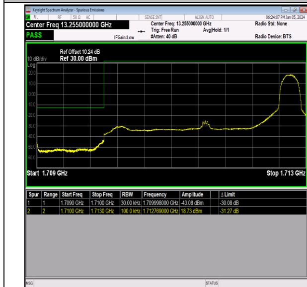
Band66_3MHz_16QAM_131987_1RB#14
