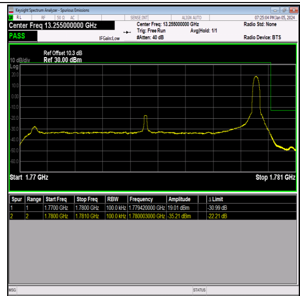
Band66_10MHz_16QAM_132622_1RB#49
