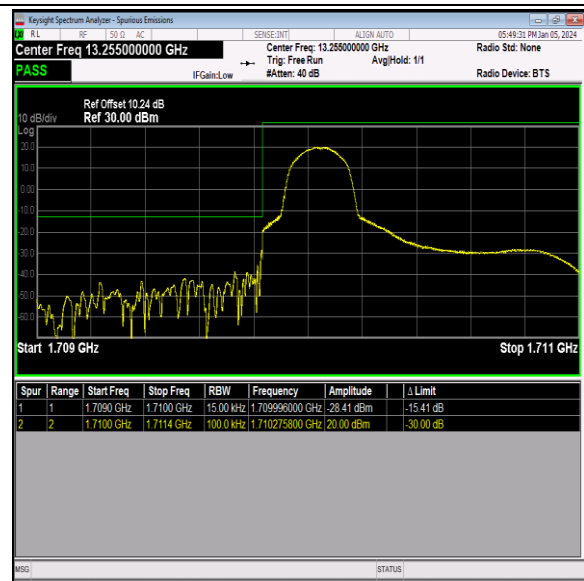
Band66_1.4MHz_QPSK_131979_1RB#0
