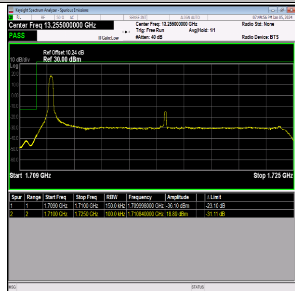
Band66_15MHz_16QAM_132047_1RB#0
