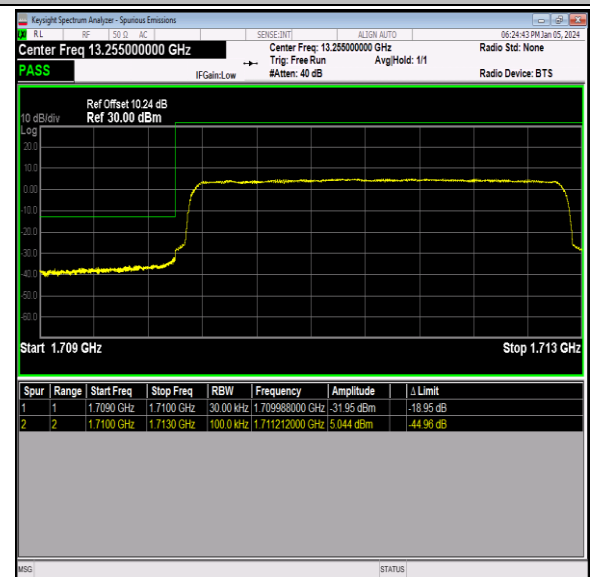
Band66_3MHz_16QAM_131987_15RB#0
