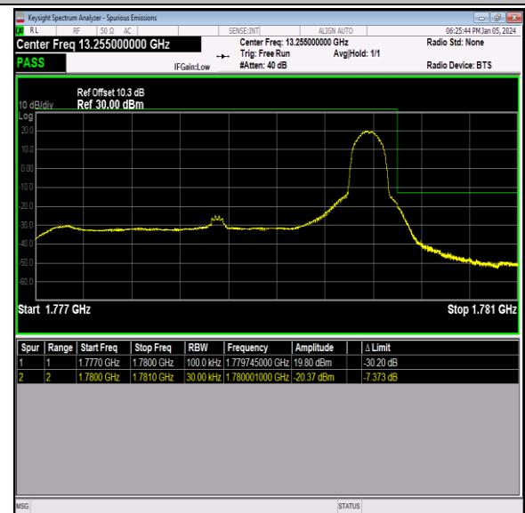
Band66_3MHz_QPSK_132657_1RB#14
