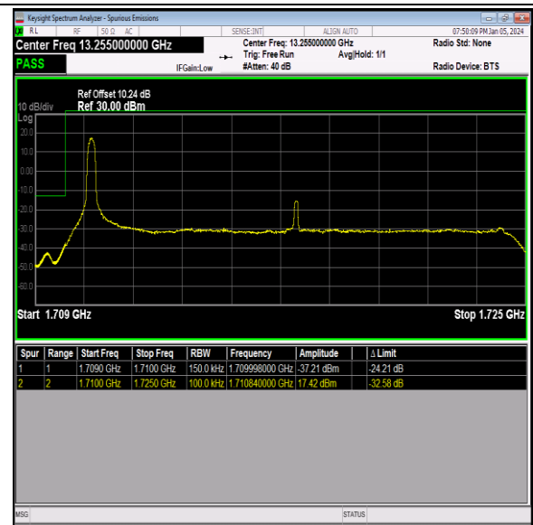
Band66_15MHz_64QAM_132047_1RB#0
