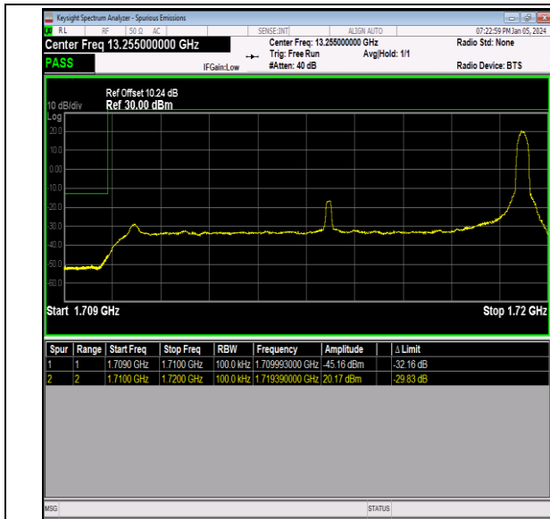
Band66_10MHz_QPSK_132022_1RB#49
