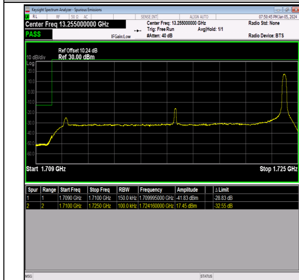
Band66_15MHz_64QAM_132047_1RB#74
