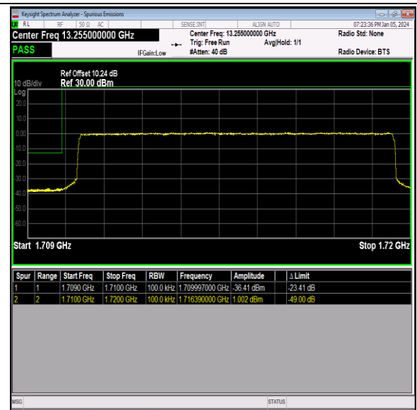
Band66_10MHz_QPSK_132022_50RB#0
