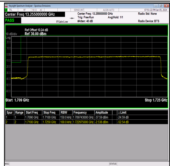
Band66_15MHz_64QAM_132047_75RB#0
