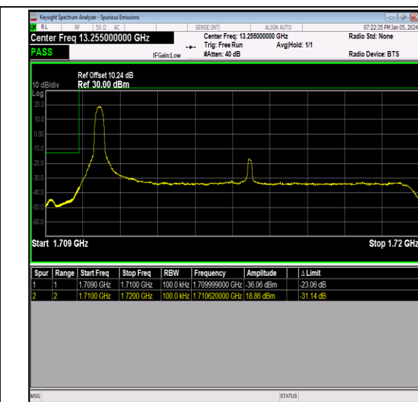
Band66_10MHz_16QAM_132022_1RB#0
