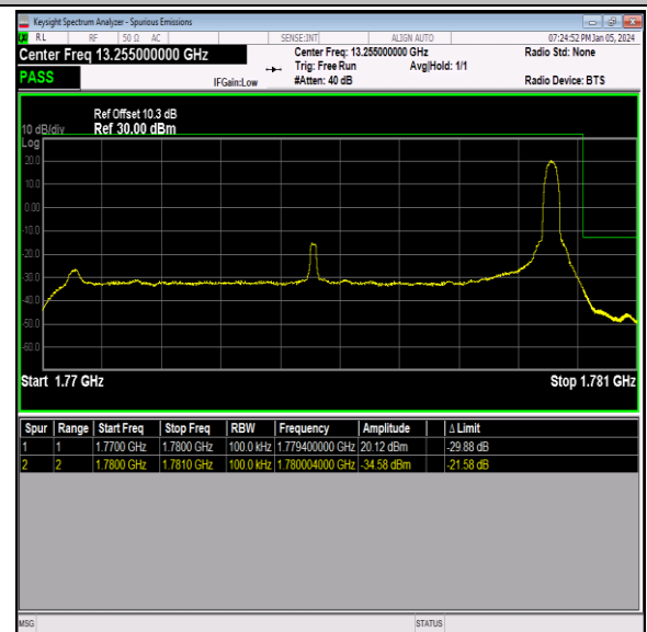
Band66_10MHz_QPSK_132622_1RB#49
