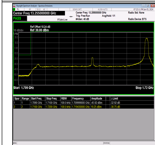
Band66_10MHz_16QAM_132022_1RB#49
