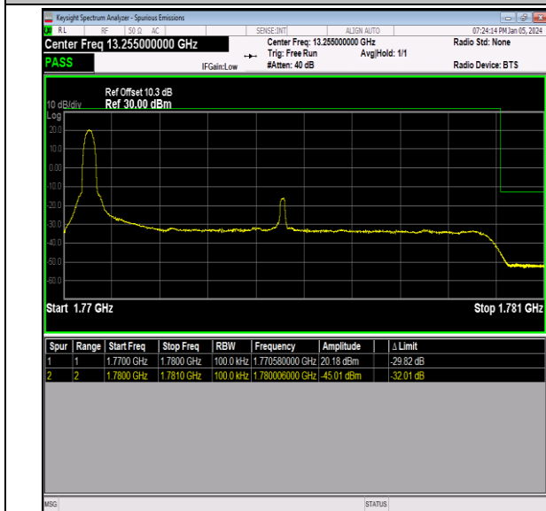
Band66_10MHz_QPSK_132622_1RB#0
