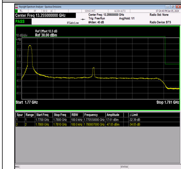
Band66_10MHz_64QAM_132622_1RB#0
