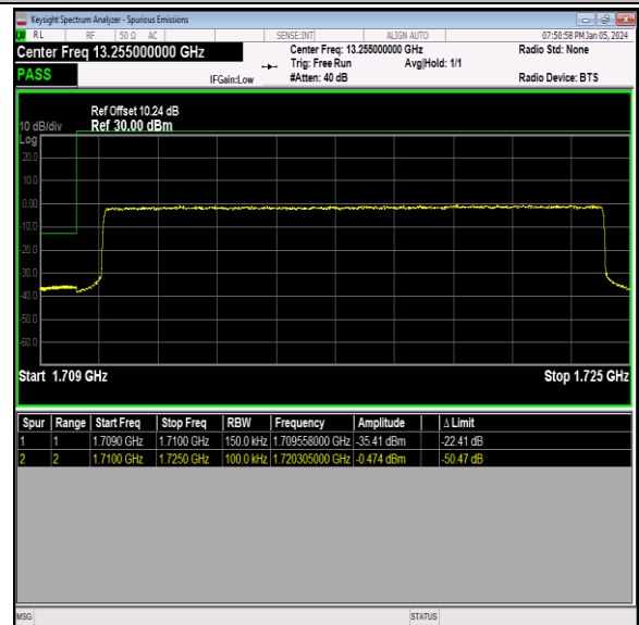
Band66_15MHz_QPSK_132047_75RB#0
