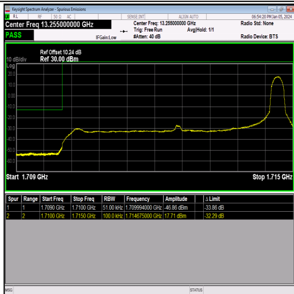
Band66_5MHz_64QAM_131997_1RB#24
