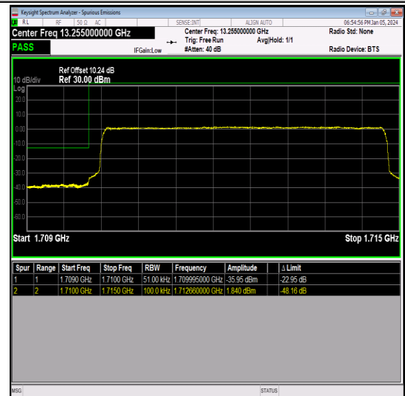
Band66_5MHz_64QAM_131997_25RB#0
