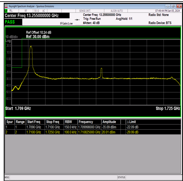
Band66_15MHz_QPSK_132047_1RB#0
