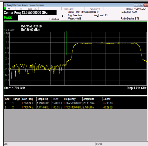
Band66_1.4MHz_QPSK_131979_6RB#0
