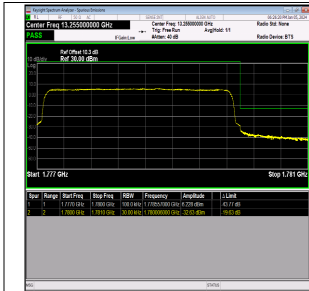
Band66_3MHz_QPSK_132657_15RB#0
