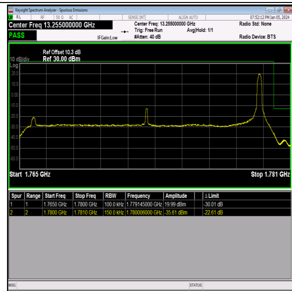
Band66_15MHz_QPSK_132597_1RB#74
