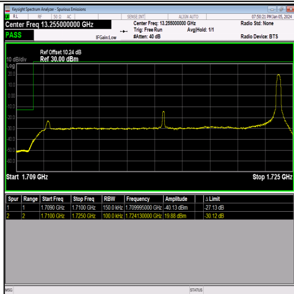
Band66_15MHz_QPSK_132047_1RB#74
