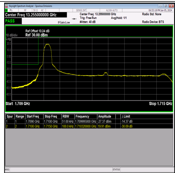
Band66_5MHz_QPSK_131997_1RB#0
