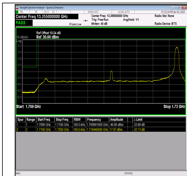
Band66_10MHz_64QAM_132022_1RB#49
