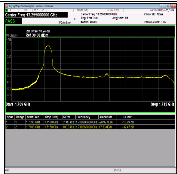
Band66_5MHz_64QAM_131997_1RB#0
