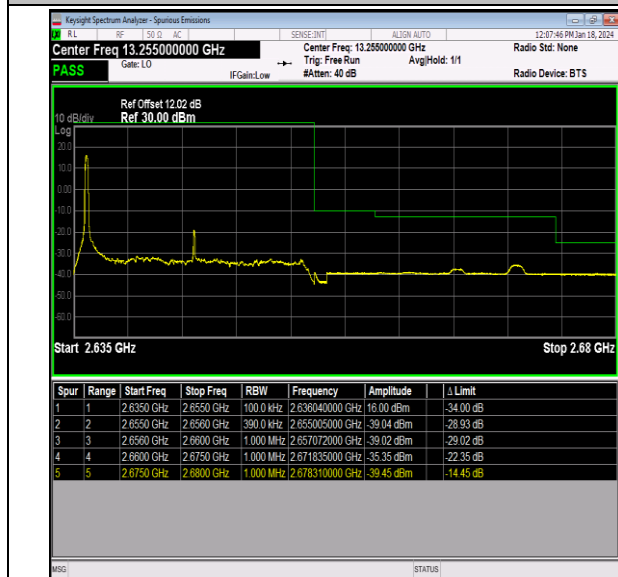
Band41_20MHz_64QAM_41140_1RB#0
