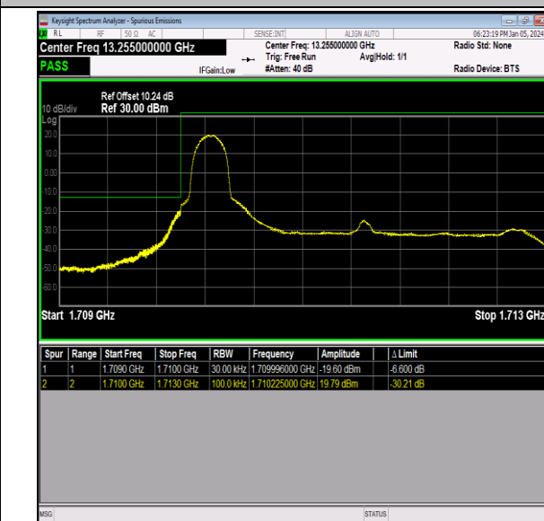
Band66_3MHz_QPSK_131987_1RB#0
