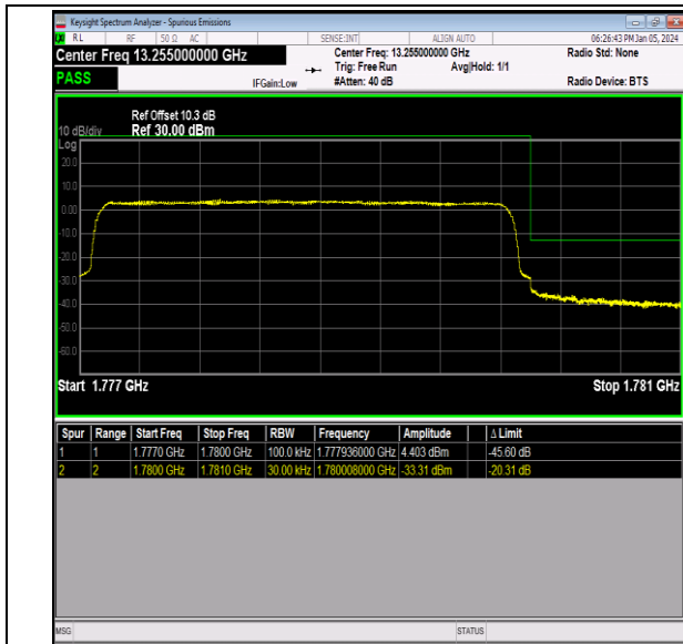
Band66_3MHz_64QAM_132657_15RB#0
