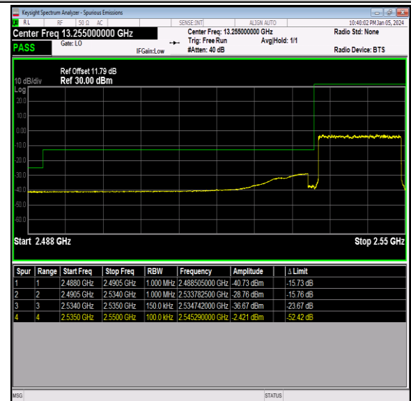
Band41_15MHz_64QAM_40115_75RB#0
