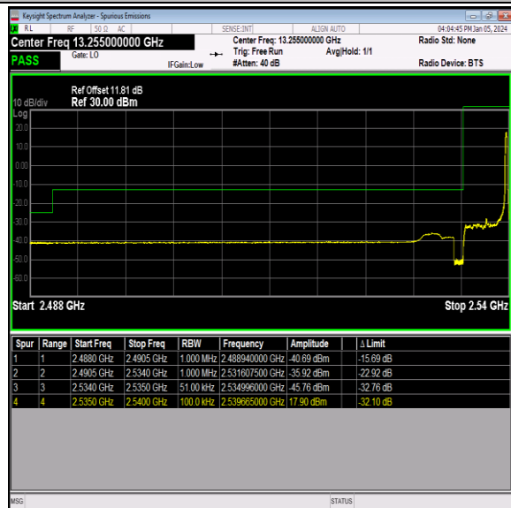
Band41_5MHz_64QAM_40065_1RB#24
