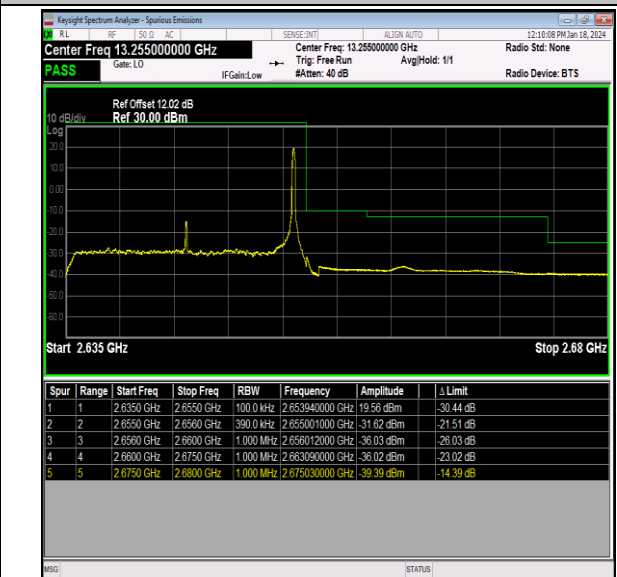
Band41_20MHz_QPSK_41140_1RB#99
