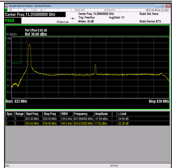
Band26_15MHz_64QAM_26865_1RB#0
