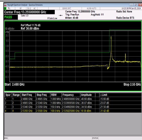
Band41_15MHz_16QAM_40115_1RB#0
