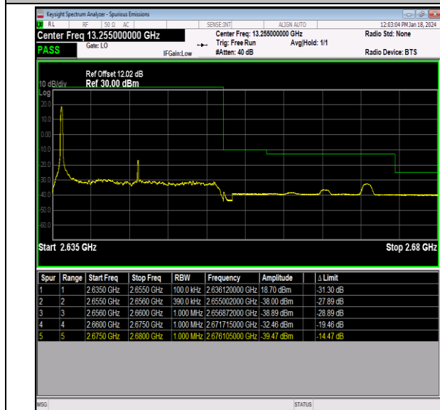
Band41_20MHz_QPSK_41140_1RB#0
