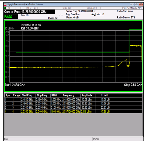
Band41_5MHz_64QAM_40065_25RB#0
