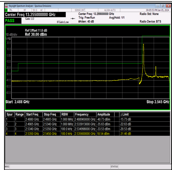
Band41_10MHz_16QAM_40090_1RB#0
