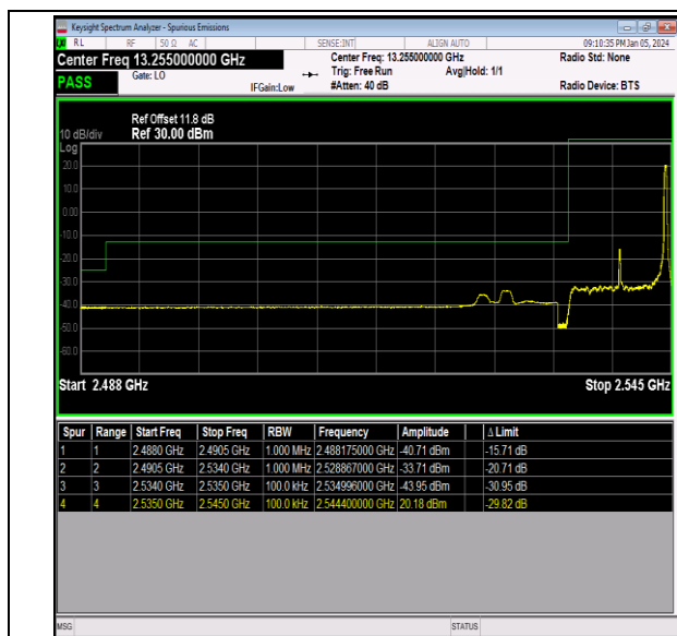
Band41_10MHz_QPSK_40090_1RB#49
