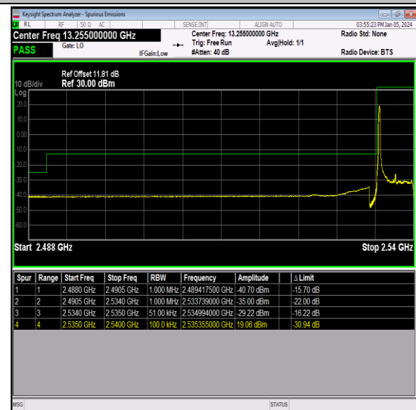
Band41_5MHz_16QAM_40065_1RB#0
