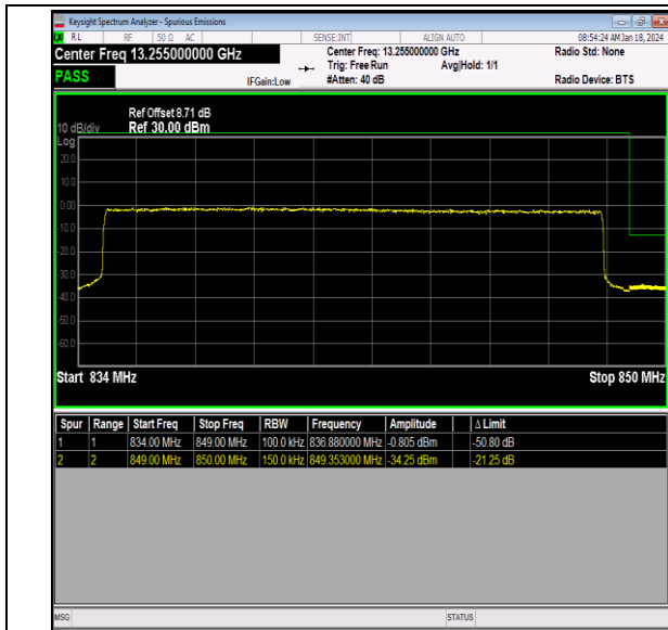
Band26_15MHz_QPSK_26965_75RB#0
