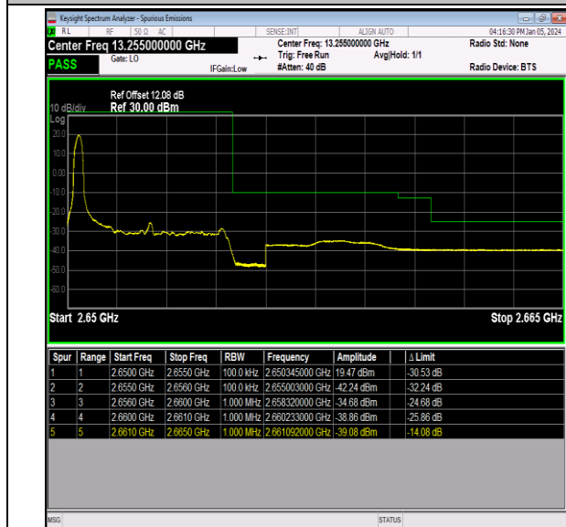
Band41_5MHz_16QAM_41215_1RB#0
