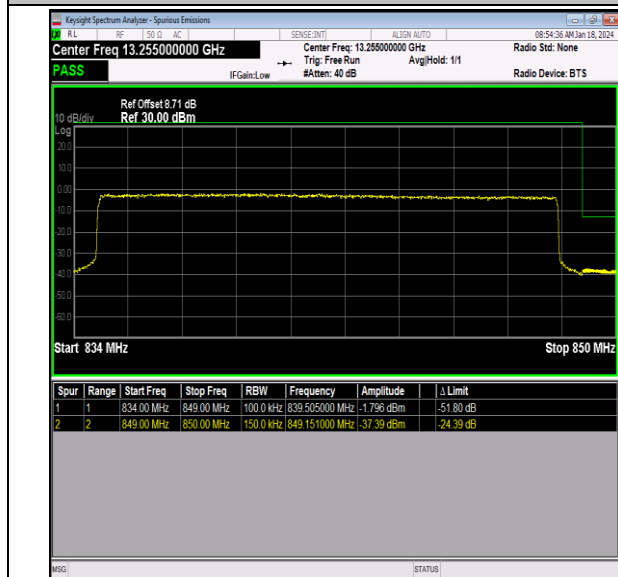
Band26_15MHz_16QAM_26965_75RB#0
