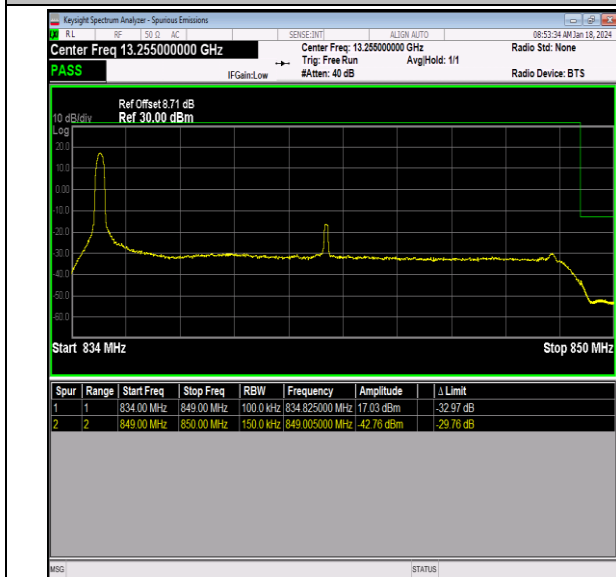
Band26_15MHz_64QAM_26965_1RB#0
