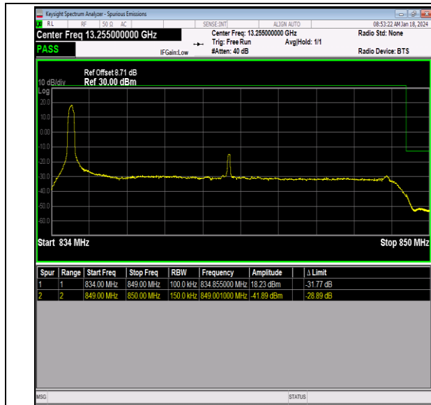
Band26_15MHz_16QAM_26965_1RB#0
