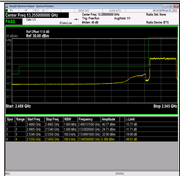
Band41_10MHz_16QAM_40090_50RB#0
