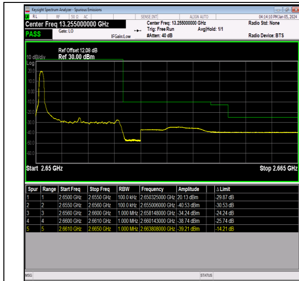
Band41_5MHz_QPSK_41215_1RB#0
