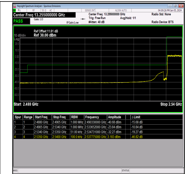
Band41_5MHz_16QAM_40065_25RB#0
