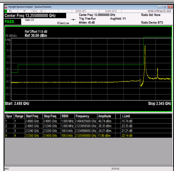
Band41_10MHz_64QAM_40090_1RB#0
