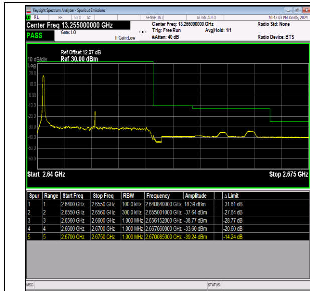
Band41_15MHz_64QAM_41165_1RB#0
