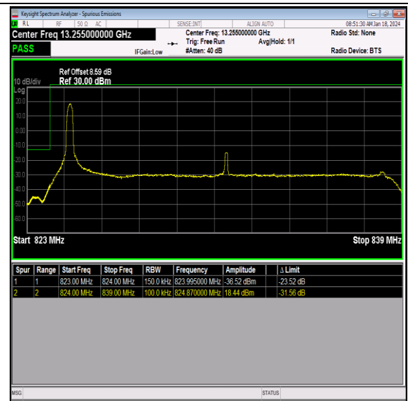
Band26_15MHz_16QAM_26865_1RB#0
