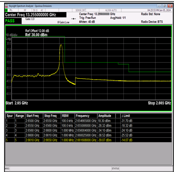
Band41_5MHz_64QAM_41215_1RB#24
