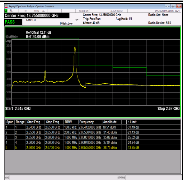
Band41_10MHz_64QAM_41190_1RB#49
