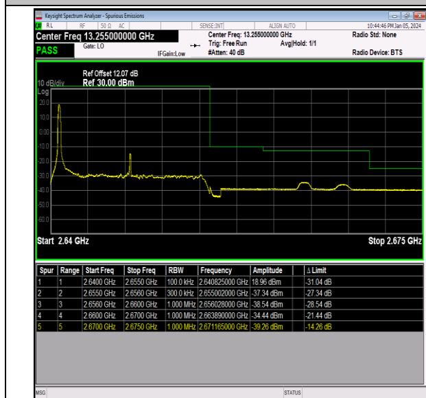
Band41_15MHz_16QAM_41165_1RB#0
