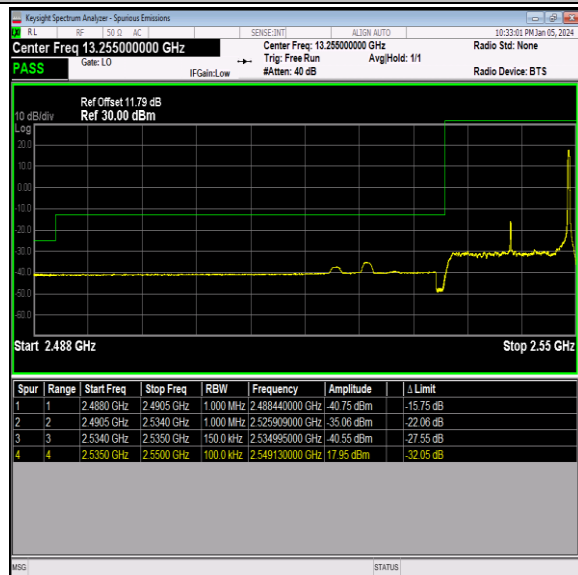
Band41_15MHz_64QAM_40115_1RB#74
