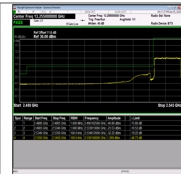
Band41_10MHz_QPSK_40090_50RB#0
