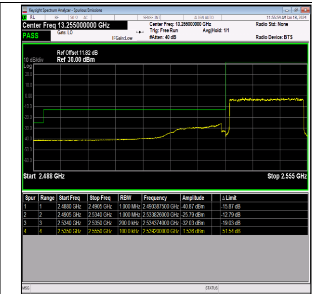
Band41_20MHz_QPSK_40140_100RB#0
