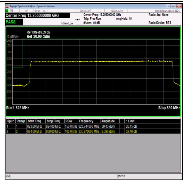
Band26_15MHz_64QAM_26865_75RB#0
