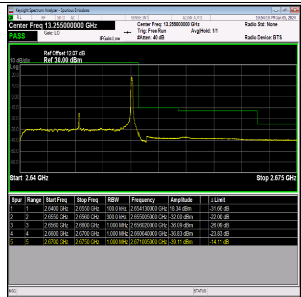
Band41_15MHz_64QAM_41165_1RB#74
