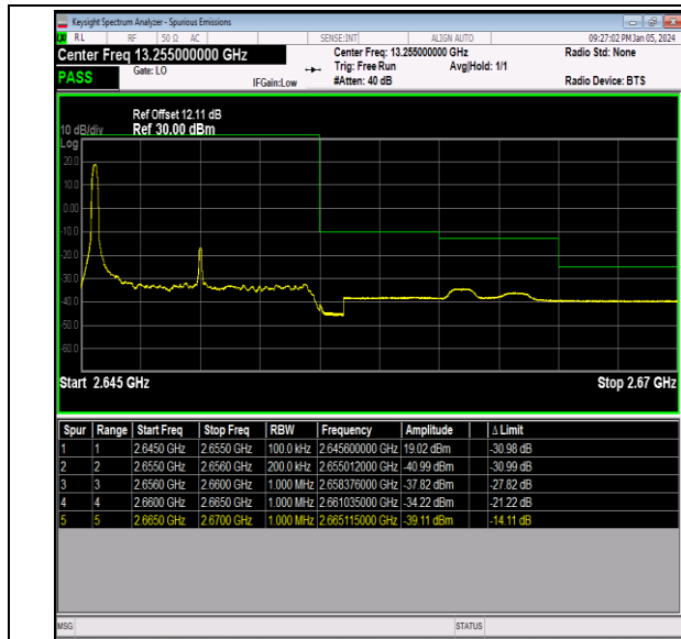
Band41_10MHz_16QAM_41190_1RB#0
