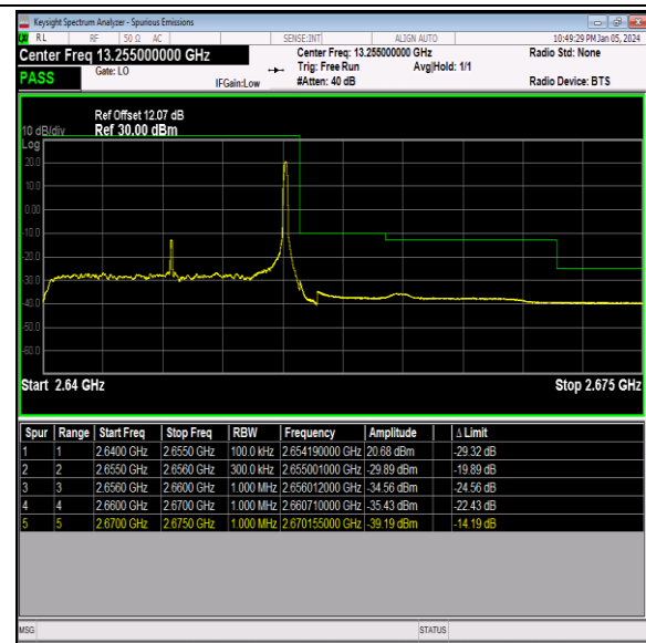
Band41_15MHz_QPSK_41165_1RB#74
