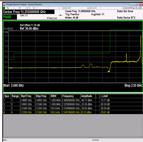
Band41_15MHz_QPSK_40115_1RB#74
