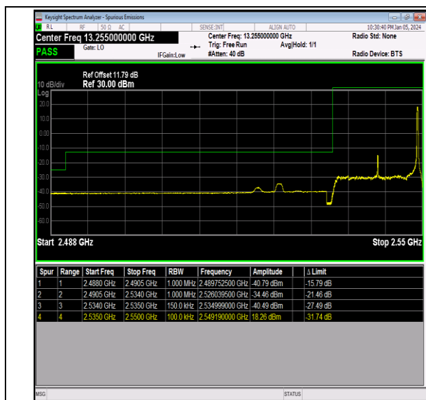
Band41_15MHz_16QAM_40115_1RB#74
