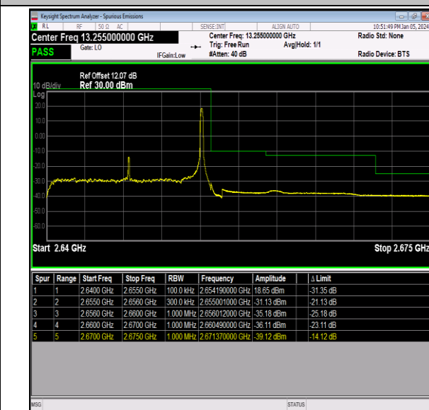
Band41_15MHz_16QAM_41165_1RB#74
