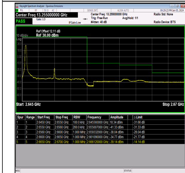
Band41_10MHz_64QAM_41190_1RB#0
