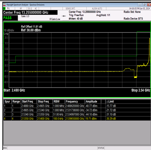
Band41_5MHz_QPSK_40065_1RB#24
