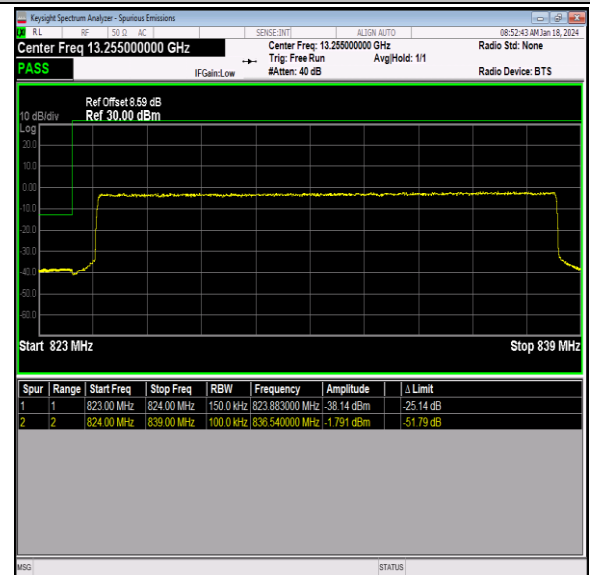
Band26_15MHz_16QAM_26865_75RB#0
