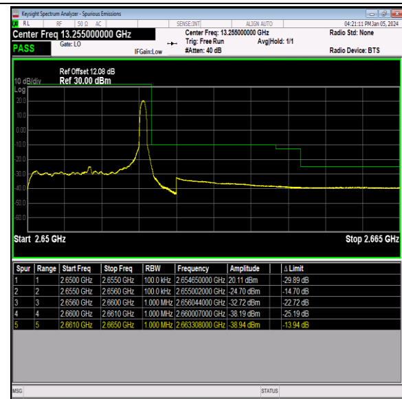
Band41_5MHz_QPSK_41215_1RB#24
