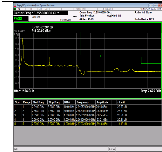
Band41_15MHz_QPSK_41165_1RB#0
