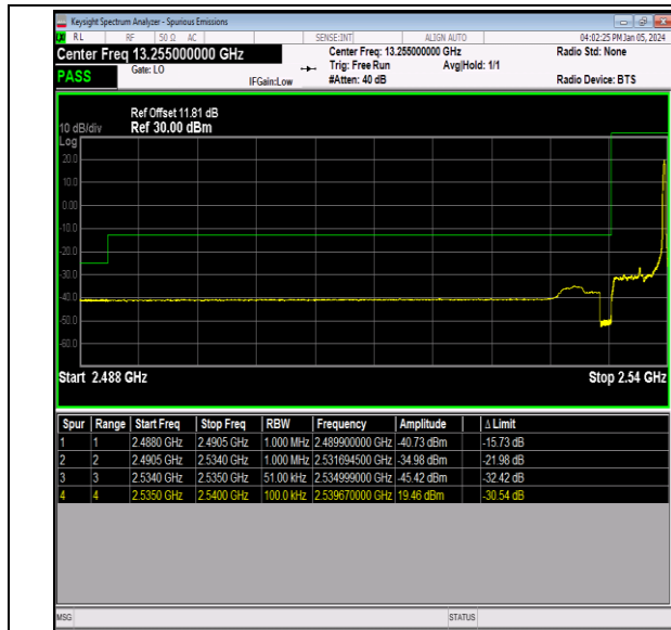
Band41_5MHz_16QAM_40065_1RB#24
