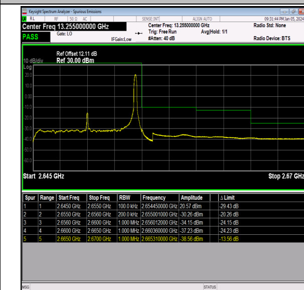
Band41_10MHz_QPSK_41190_1RB#49
