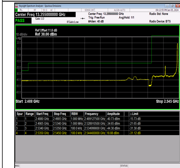
Band41_10MHz_16QAM_40090_1RB#49
