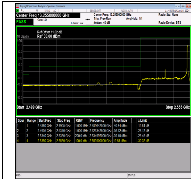
Band41_20MHz_QPSK_40140_1RB#99
