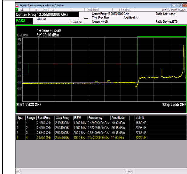
Band41_20MHz_16QAM_40140_1RB#99
