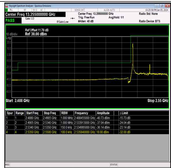
Band41_15MHz_64QAM_40115_1RB#0
