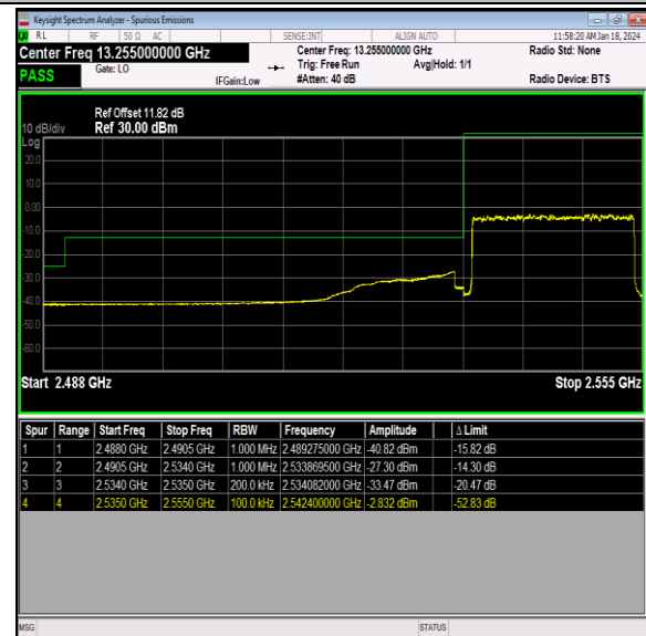
Band41_20MHz_16QAM_40140_100RB#0
