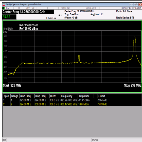
Band26_15MHz_16QAM_26865_1RB#74
