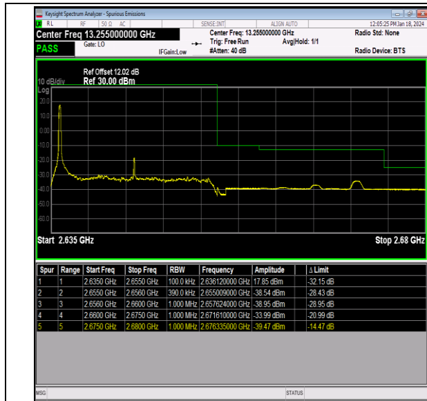
Band41_20MHz_16QAM_41140_1RB#0
