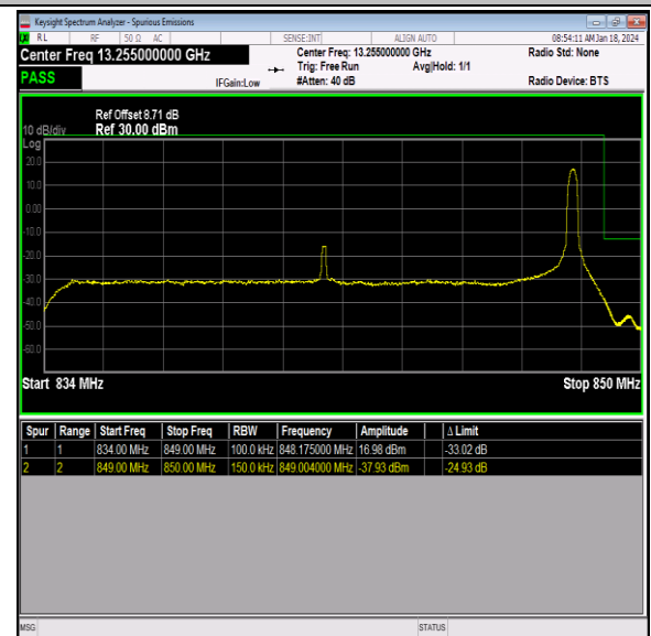
Band26_15MHz_64QAM_26965_1RB#74
