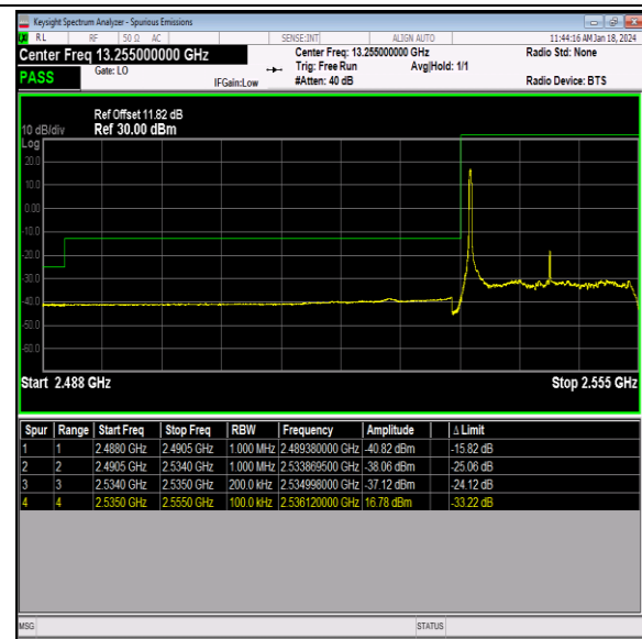
Band41_20MHz_16QAM_40140_1RB#0
