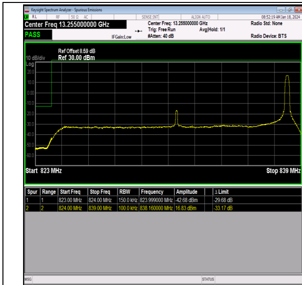
Band26_15MHz_64QAM_26865_1RB#74
