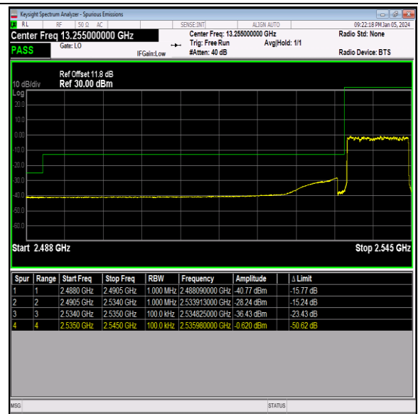
Band41_10MHz_64QAM_40090_50RB#0
