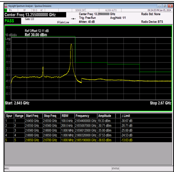
Band41_10MHz_16QAM_41190_1RB#49
