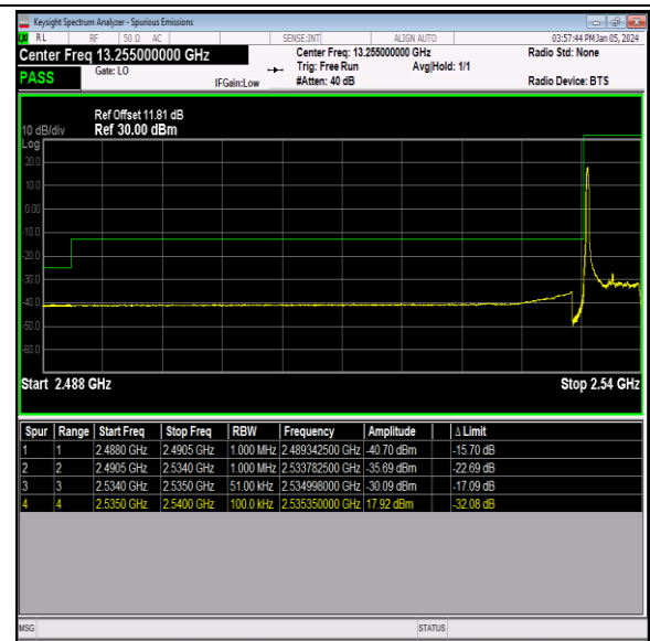
Band41_5MHz_64QAM_40065_1RB#0
