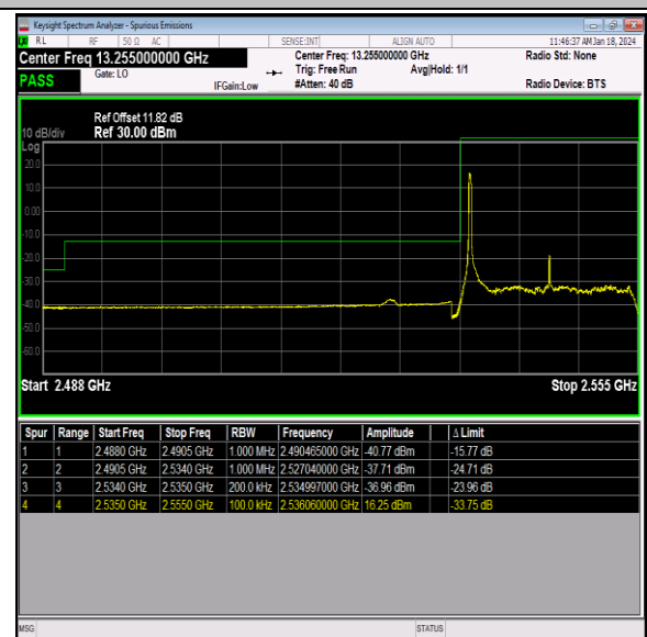
Band41_20MHz_64QAM_40140_1RB#0
