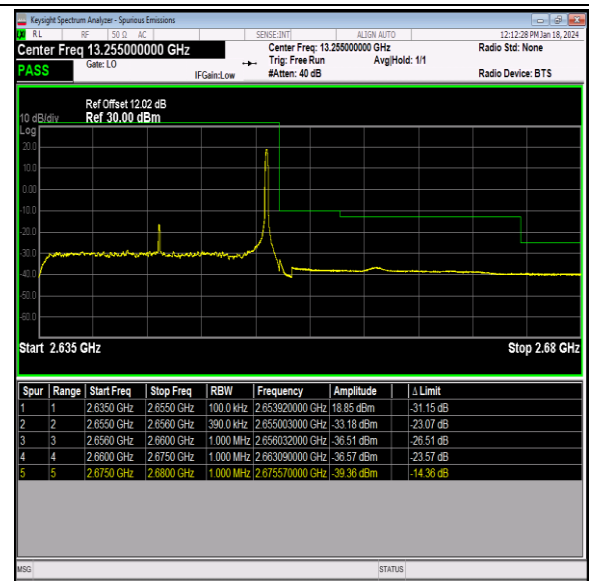
Band41_20MHz_16QAM_41140_1RB#99
