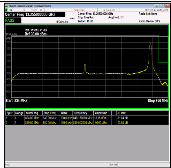
Band26_15MHz_16QAM_26965_1RB#74
