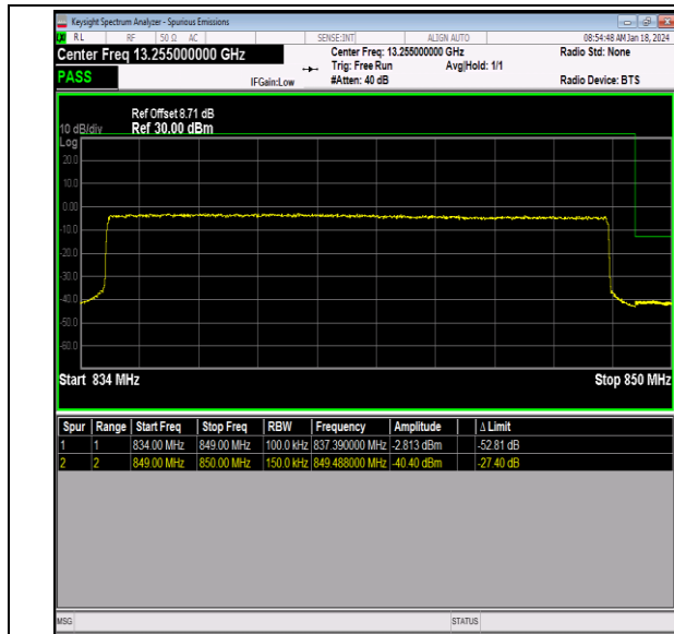
Band26_15MHz_64QAM_26965_75RB#0
