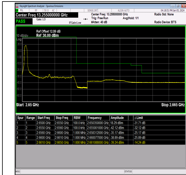
Band41_5MHz_64QAM_41215_1RB#0
