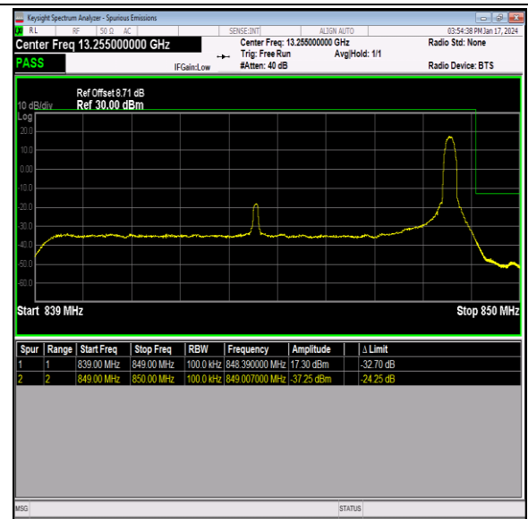
Band26_10MHz_64QAM_26990_1RB#49
