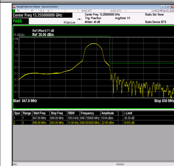
Band26_1.4MHz_64QAM_27033_1RB#5
