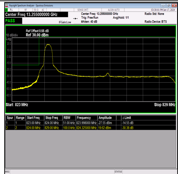
Band26_5MHz_QPSK_26815_1RB#0
