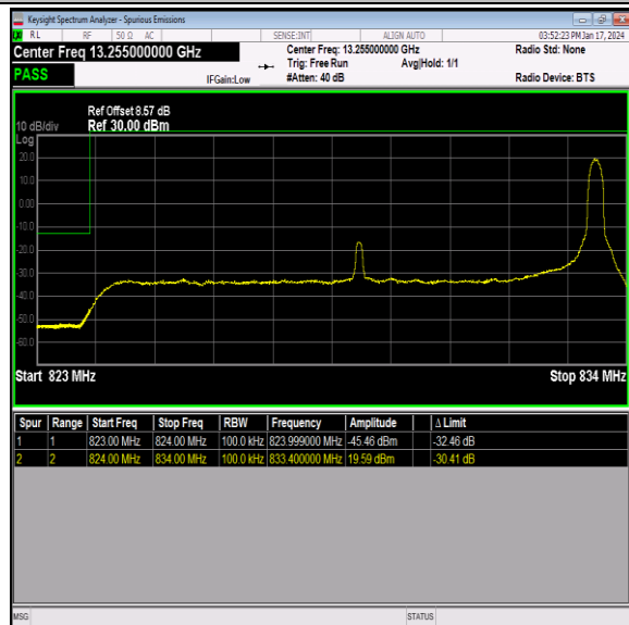
Band26_10MHz_QPSK_26840_1RB#49
