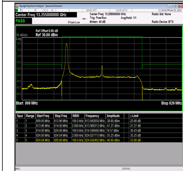
Band26_10MHz_QPSK_26740_1RB#0
