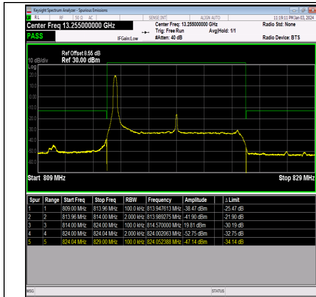
Band26_10MHz_64QAM_26740_1RB#0
