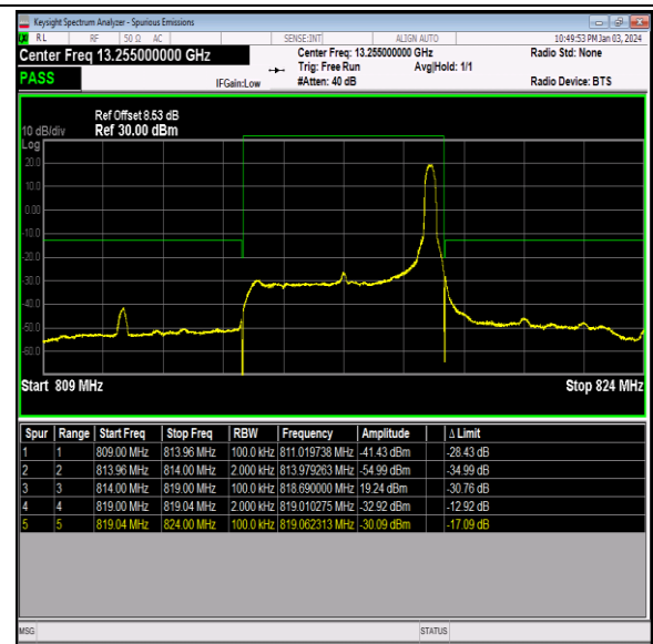
Band26_5MHz_64QAM_26715_1RB#24
