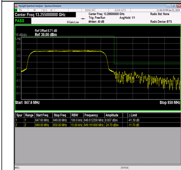
Band26_1.4MHz_16QAM_27033_6RB#0
