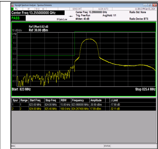
Band26_1.4MHz_16QAM_26797_1RB#0
