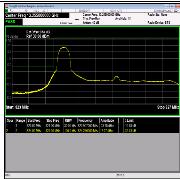
Band26_3MHz_64QAM_26805_1RB#0
