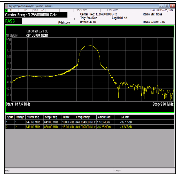
Band26_1.4MHz_16QAM_27033_1RB#5
