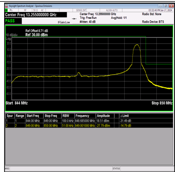
Band26_5MHz_16QAM_27015_1RB#24
