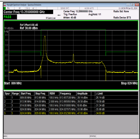
Band26_10MHz_16QAM_26740_1RB#0
