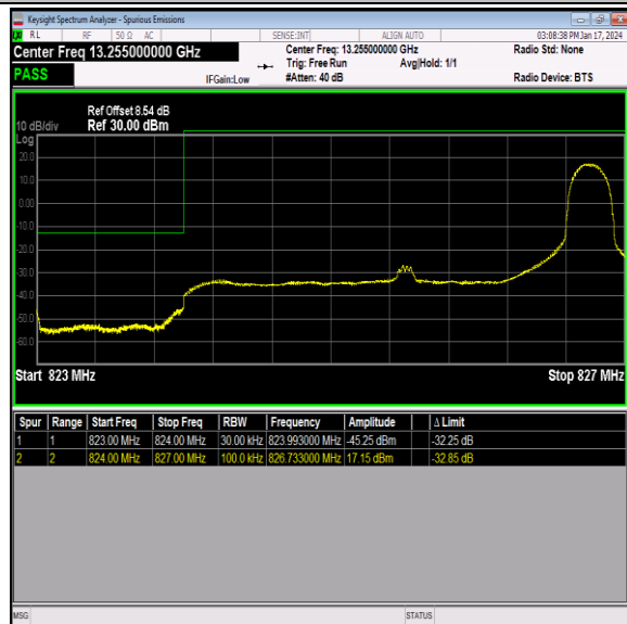
Band26_3MHz_64QAM_26805_1RB#14
