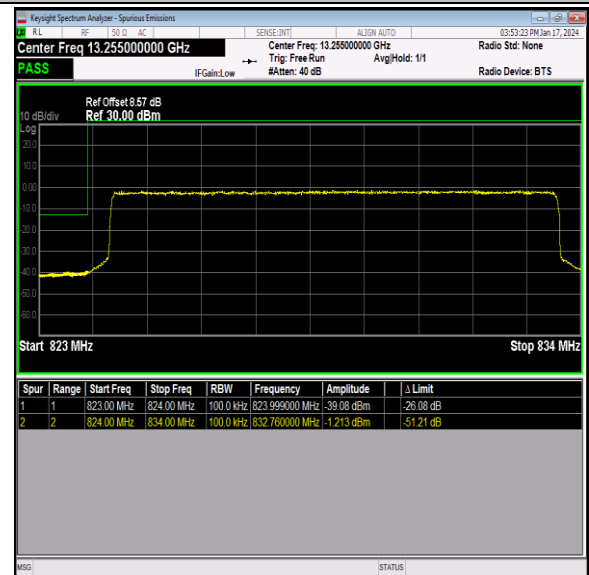
Band26_10MHz_64QAM_26840_50RB#0
