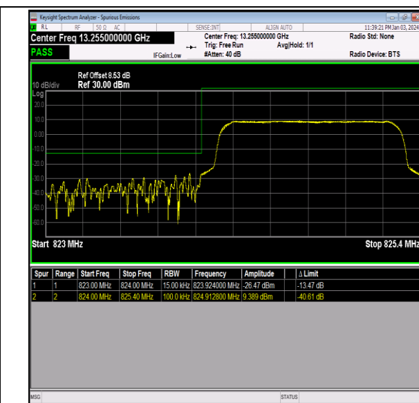
Band26_1.4MHz_64QAM_26797_6RB#0
