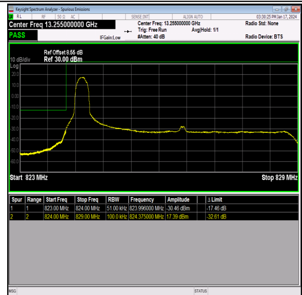
Band26_5MHz_64QAM_26815_1RB#0
