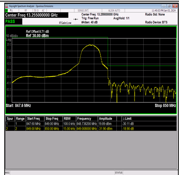
Band26_1.4MHz_QPSK_27033_1RB#5
