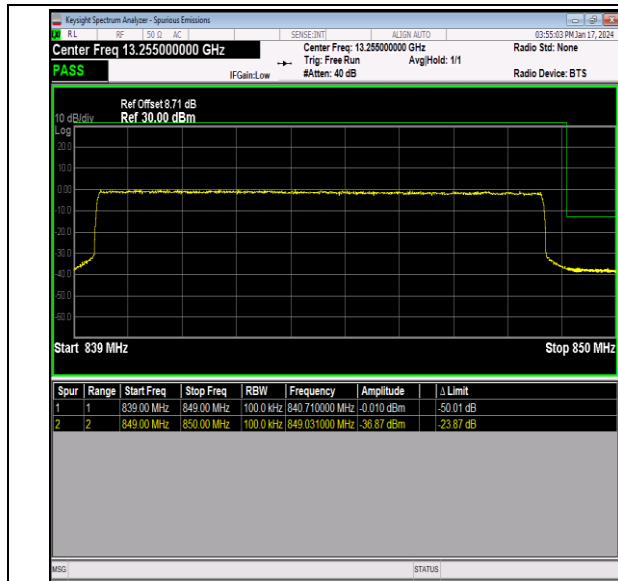
Band26_10MHz_16QAM_26990_50RB#0
