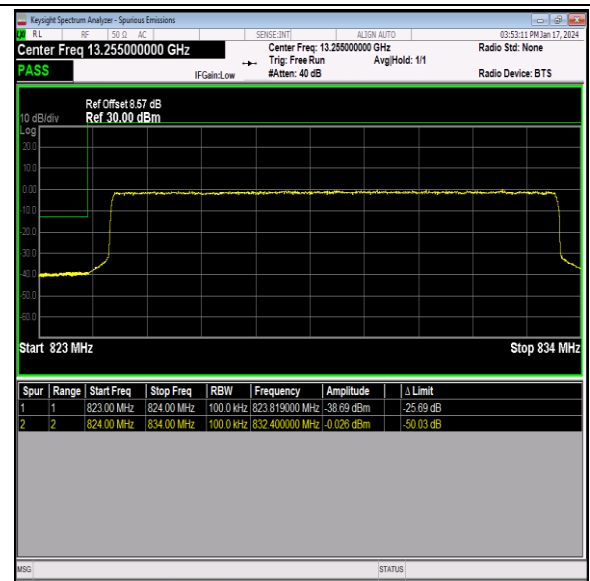
Band26_10MHz_16QAM_26840_50RB#0
