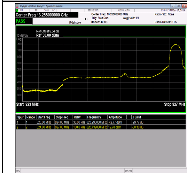
Band26_3MHz_QPSK_26805_1RB#14
