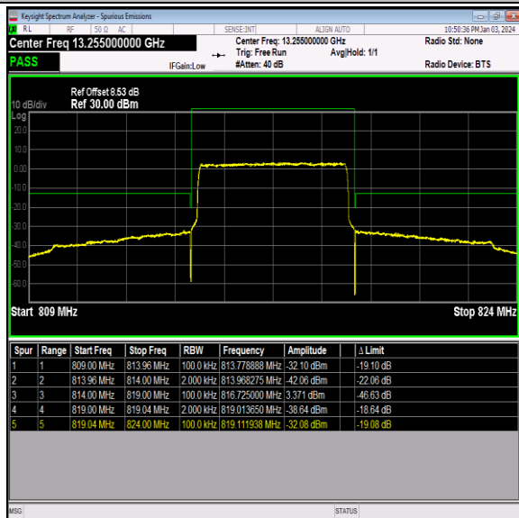
Band26_5MHz_64QAM_26715_25RB#0
