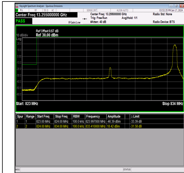
Band26_10MHz_16QAM_26840_1RB#49
