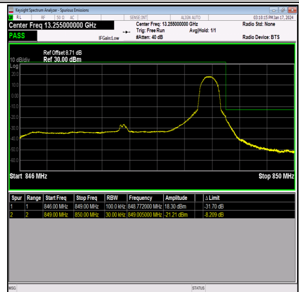
Band26_3MHz_16QAM_27025_1RB#14
