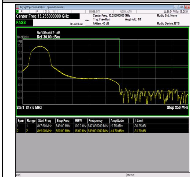
Band26_1.4MHz_64QAM_27033_1RB#0
