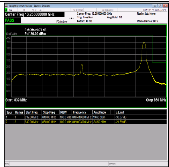
Band26_10MHz_QPSK_26990_1RB#49
