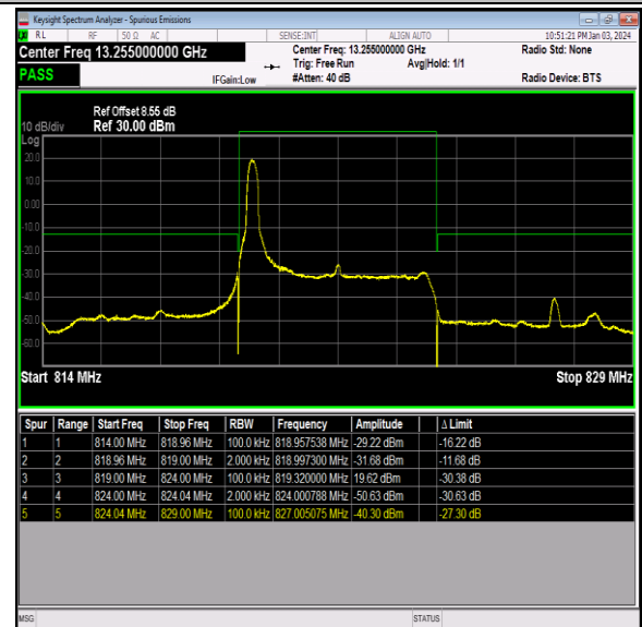
Band26_5MHz_64QAM_26765_1RB#0
