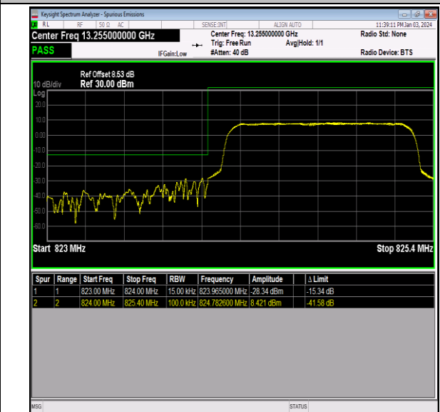
Band26_1.4MHz_16QAM_26797_6RB#0
