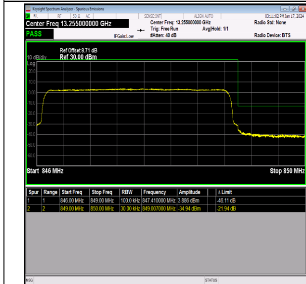
Band26_3MHz_64QAM_27025_15RB#0
