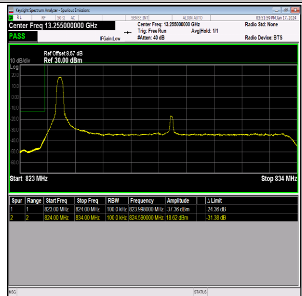
Band26_10MHz_16QAM_26840_1RB#0
