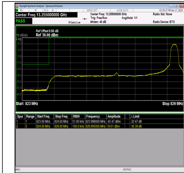
Band26_5MHz_QPSK_26815_1RB#24
