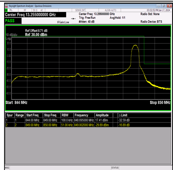
Band26_5MHz_64QAM_27015_1RB#24
