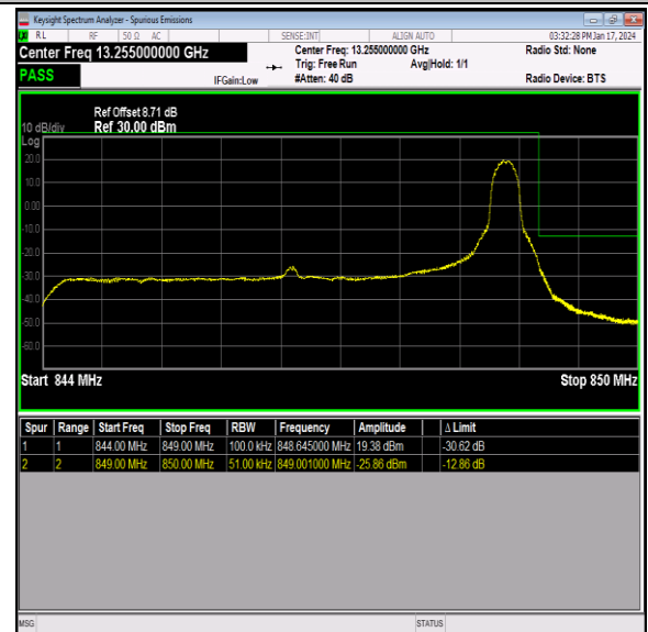
Band26_5MHz_QPSK_27015_1RB#24
