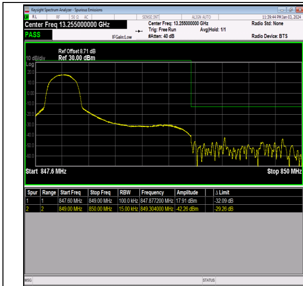
Band26_1.4MHz_16QAM_27033_1RB#0
