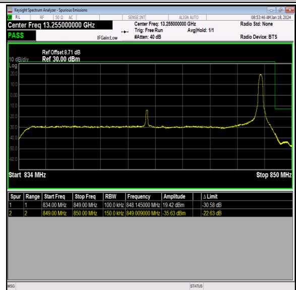
Band26_15MHz_QPSK_26965_1RB#74
