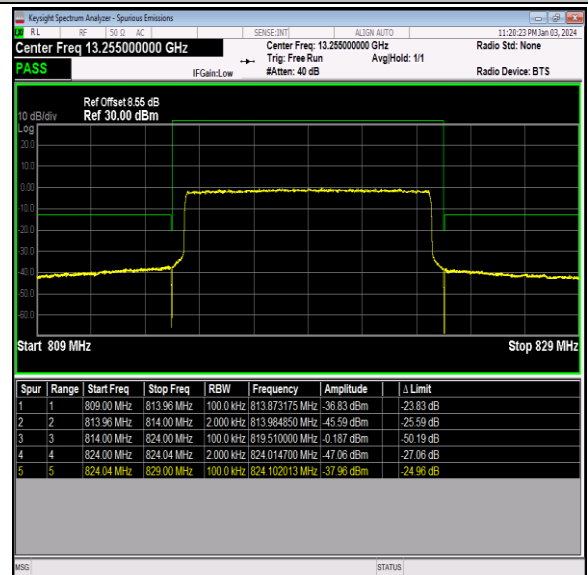
Band26_10MHz_16QAM_26740_50RB#0
