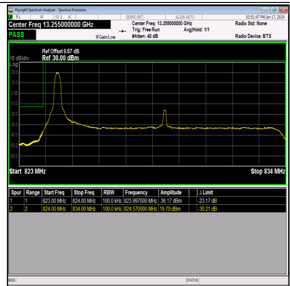
Band26_10MHz_QPSK_26840_1RB#0
