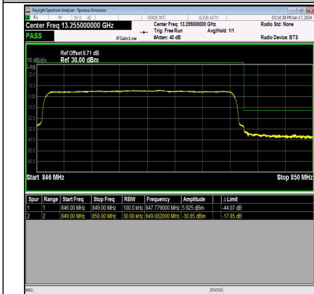
Band26_3MHz_QPSK_27025_15RB#0
