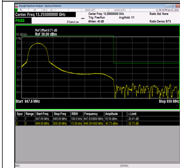
Band26_1.4MHz_QPSK_27033_1RB#0
