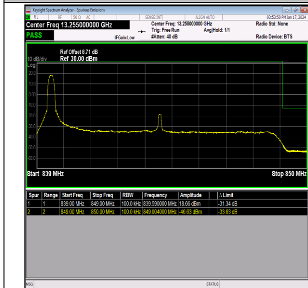
Band26_10MHz_16QAM_26990_1RB#0
