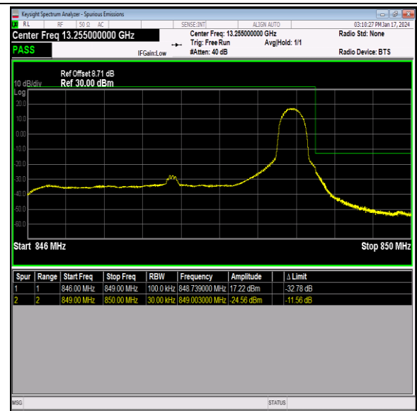
Band26_3MHz_64QAM_27025_1RB#14
