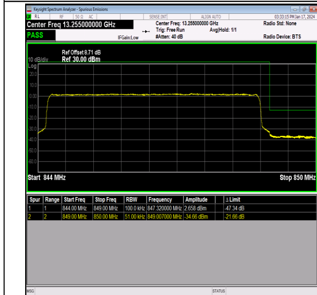
Band26_5MHz_16QAM_27015_25RB#0
