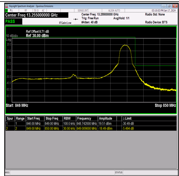
Band26_3MHz_QPSK_27025_1RB#14
