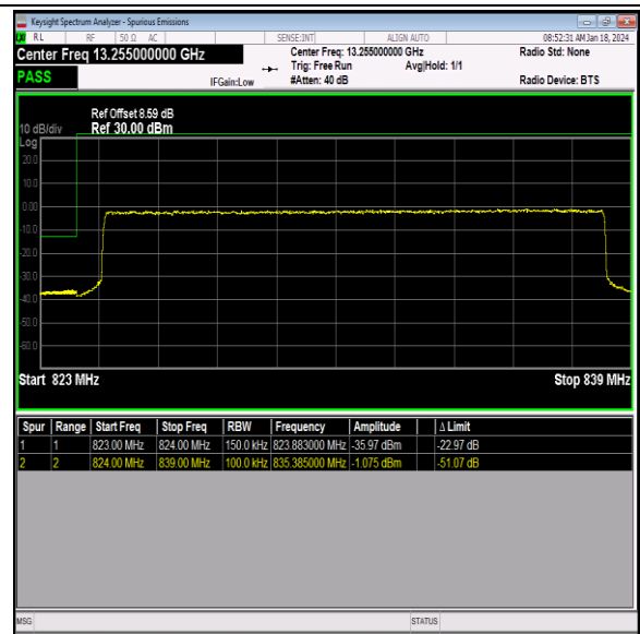
Band26_15MHz_QPSK_26865_75RB#0
