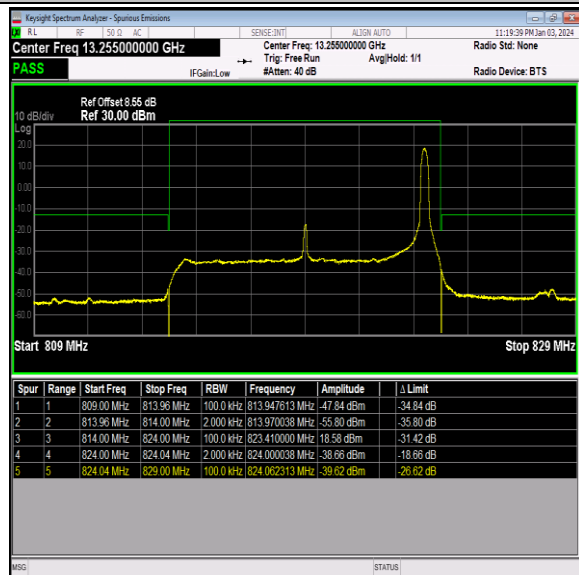
Band26_10MHz_16QAM_26740_1RB#49
