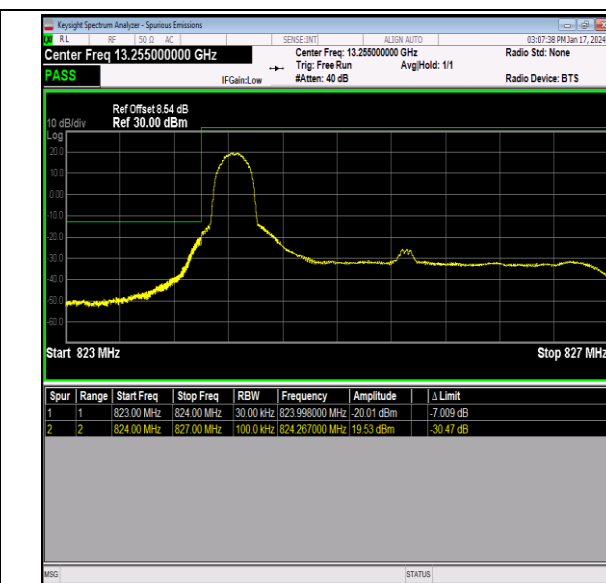
Band26_3MHz_QPSK_26805_1RB#0
