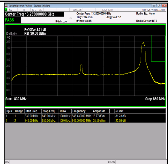
Band26_10MHz_16QAM_26990_1RB#49
