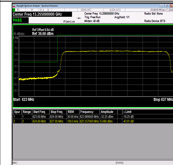
Band26_3MHz_QPSK_26805_15RB#0
