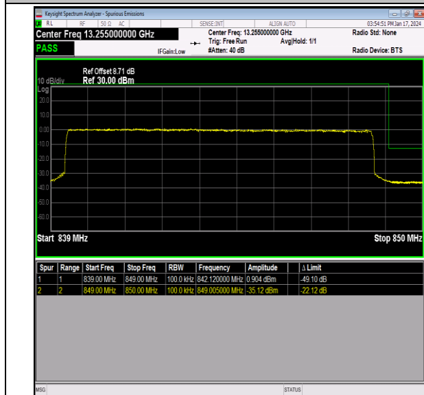
Band26_10MHz_QPSK_26990_50RB#0
