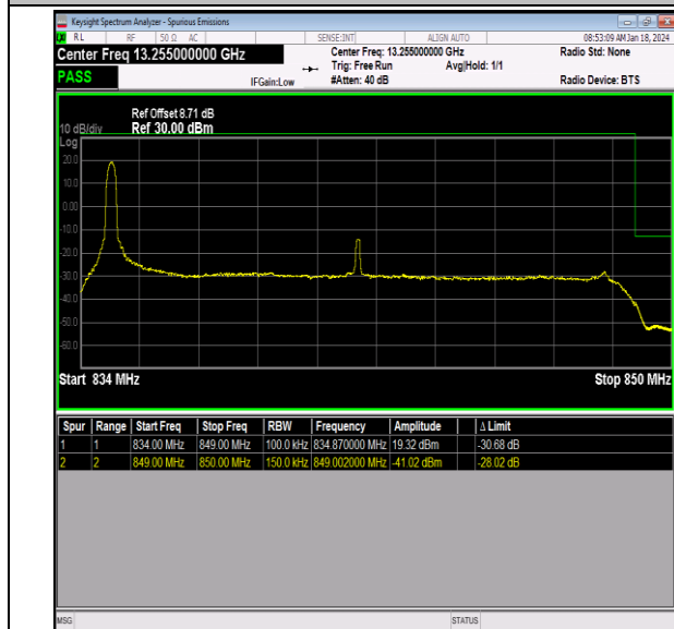
Band26_15MHz_QPSK_26965_1RB#0
