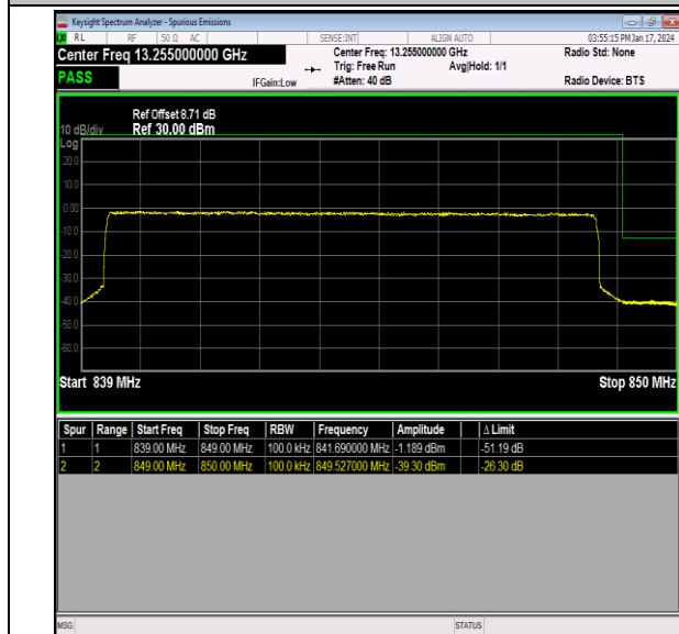
Band26_10MHz_64QAM_26990_50RB#0
