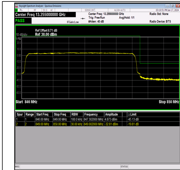
Band26_3MHz_16QAM_27025_15RB#0
