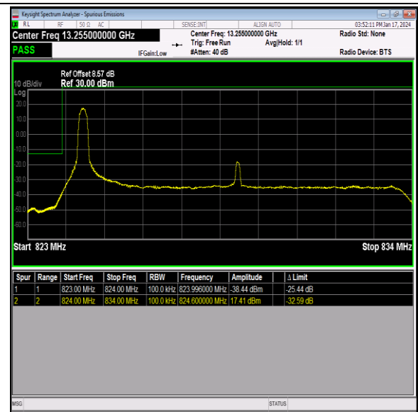
Band26_10MHz_64QAM_26840_1RB#0
