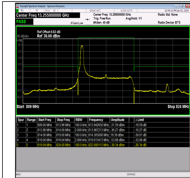
Band26_5MHz_64QAM_26715_1RB#0
