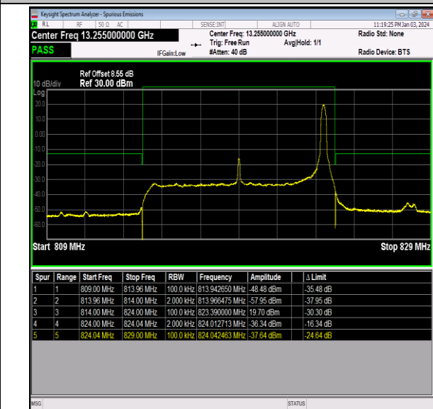
Band26_10MHz_QPSK_26740_1RB#49
