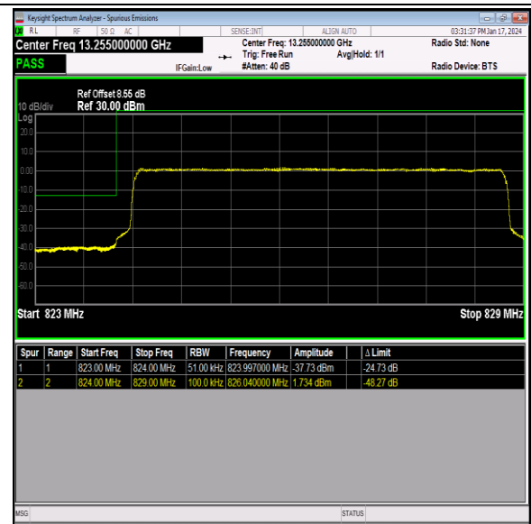
Band26_5MHz_64QAM_26815_25RB#0
