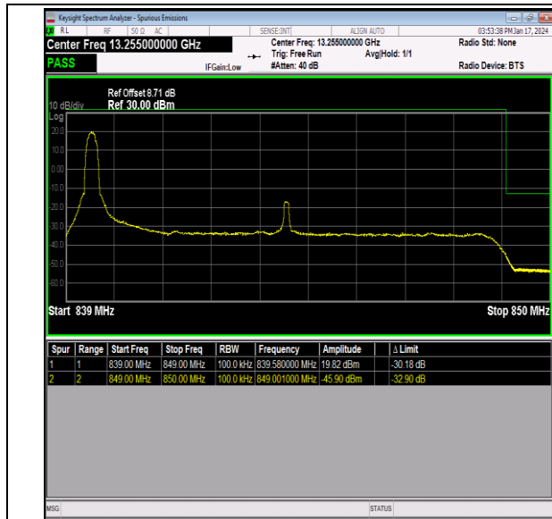
Band26_10MHz_QPSK_26990_1RB#0
