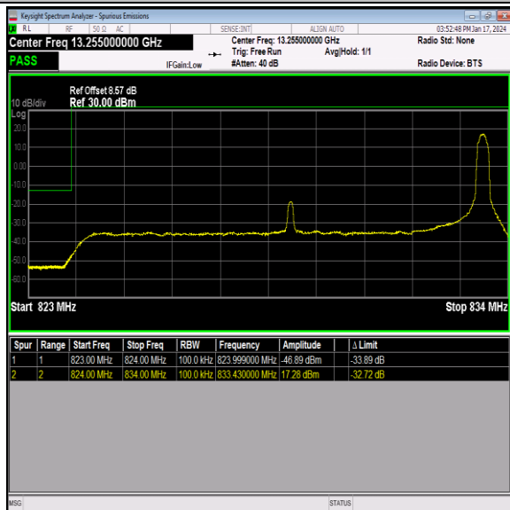
Band26_10MHz_64QAM_26840_1RB#49
