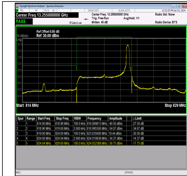
Band26_5MHz_64QAM_26765_1RB#24
