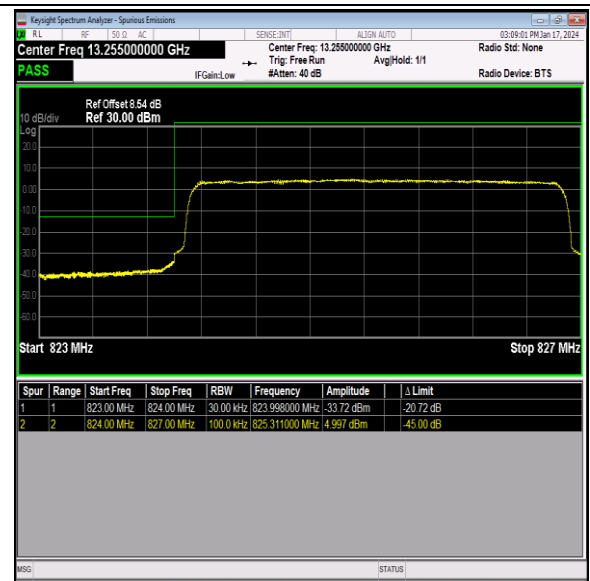
Band26_3MHz_16QAM_26805_15RB#0
