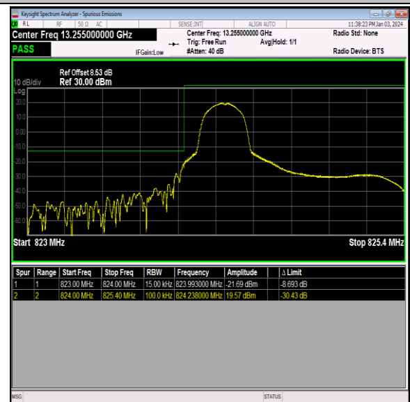
Band26_1.4MHz_64QAM_26797_1RB#0
