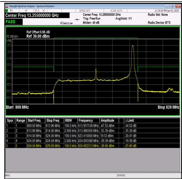
Band26_10MHz_64QAM_26740_1RB#49
