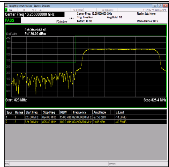
Band26_1.4MHz_QPSK_26797_6RB#0
