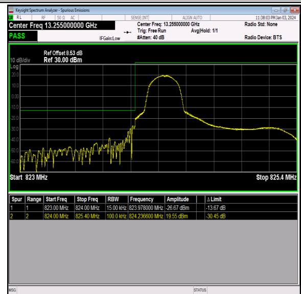
Band26_1.4MHz_QPSK_26797_1RB#0
