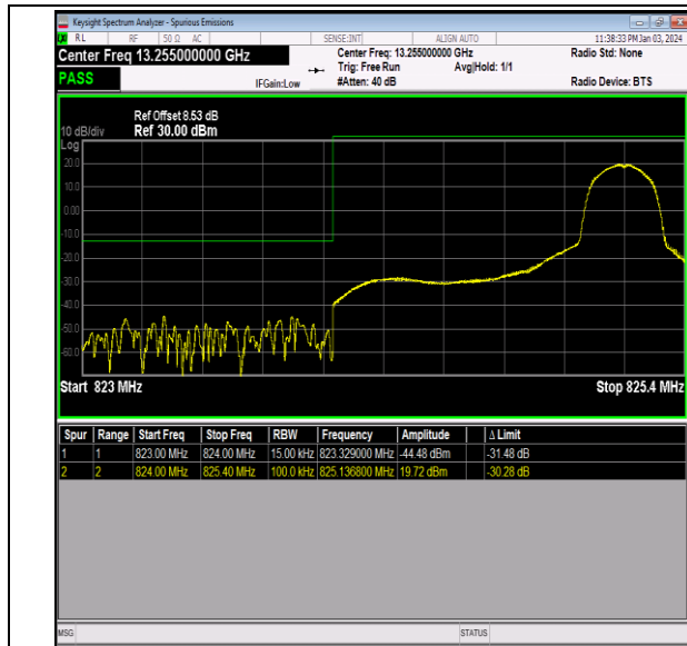
Band26_1.4MHz_QPSK_26797_1RB#5
