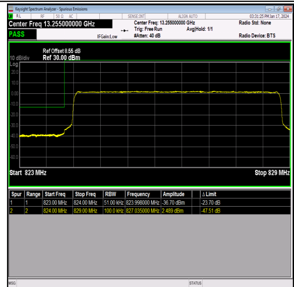
Band26_5MHz_16QAM_26815_25RB#0
