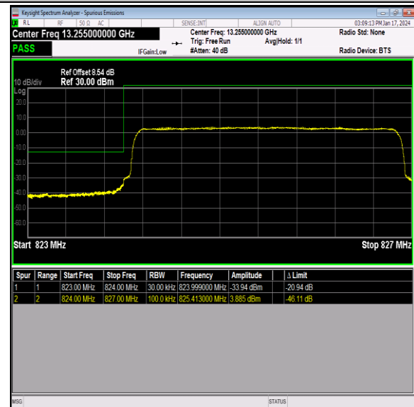
Band26_3MHz_64QAM_26805_15RB#0
