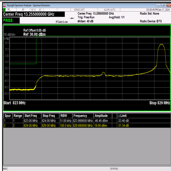
Band26_5MHz_16QAM_26815_1RB#24
