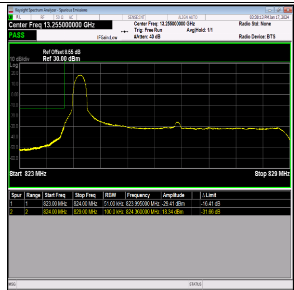
Band26_5MHz_16QAM_26815_1RB#0
