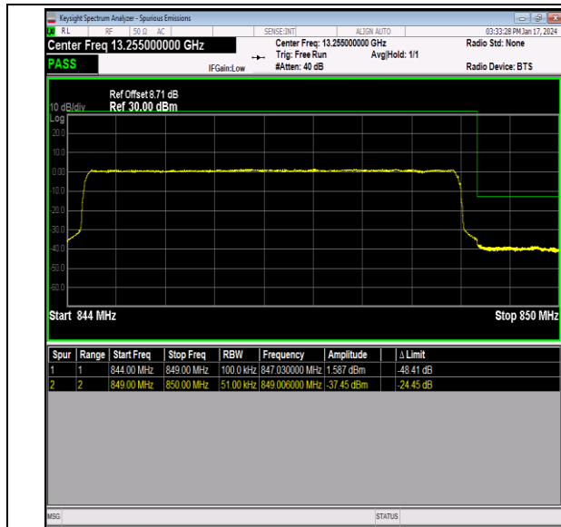
Band26_5MHz_64QAM_27015_25RB#0
