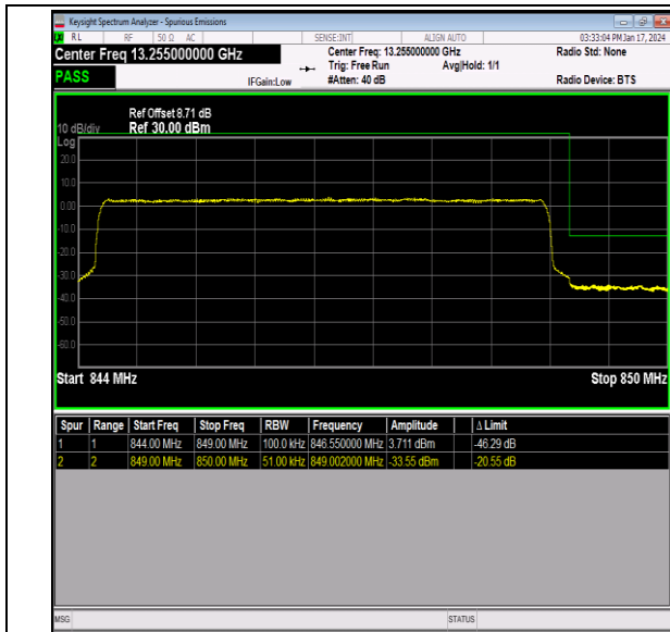
Band26_5MHz_QPSK_27015_25RB#0
