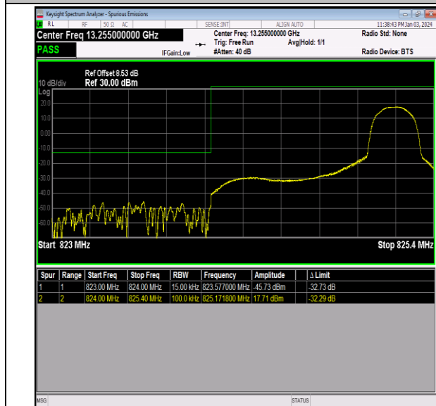
Band26_1.4MHz_16QAM_26797_1RB#5
