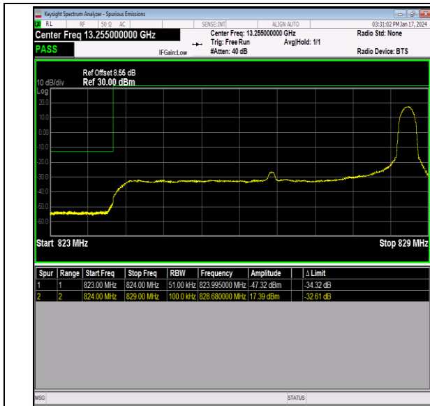
Band26_5MHz_64QAM_26815_1RB#24
