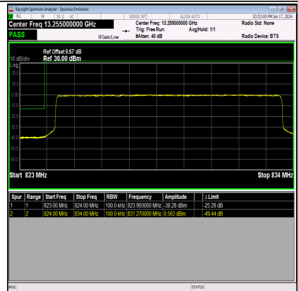
Band26_10MHz_QPSK_26840_50RB#0
