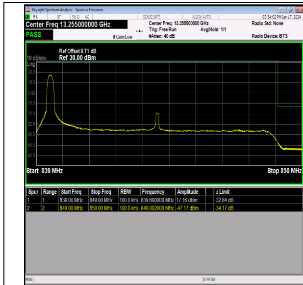
Band26_10MHz_64QAM_26990_1RB#0
