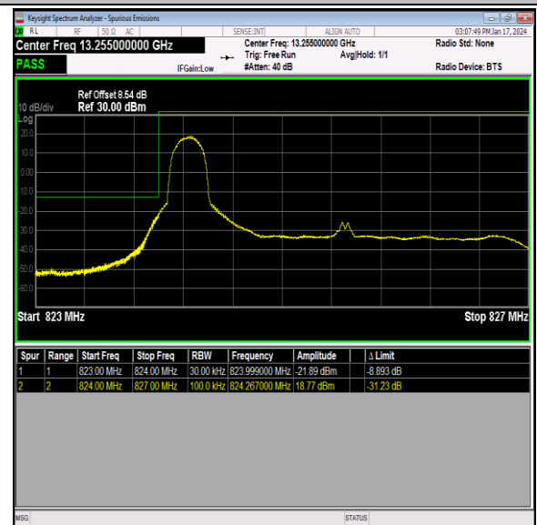
Band26_3MHz_16QAM_26805_1RB#0
