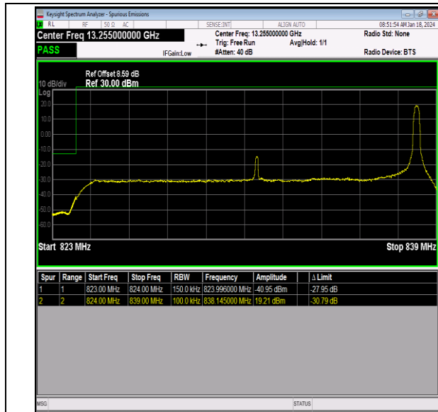
Band26_15MHz_QPSK_26865_1RB#74
