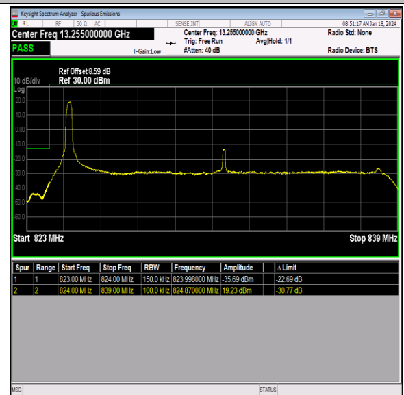
Band26_15MHz_QPSK_26865_1RB#0
