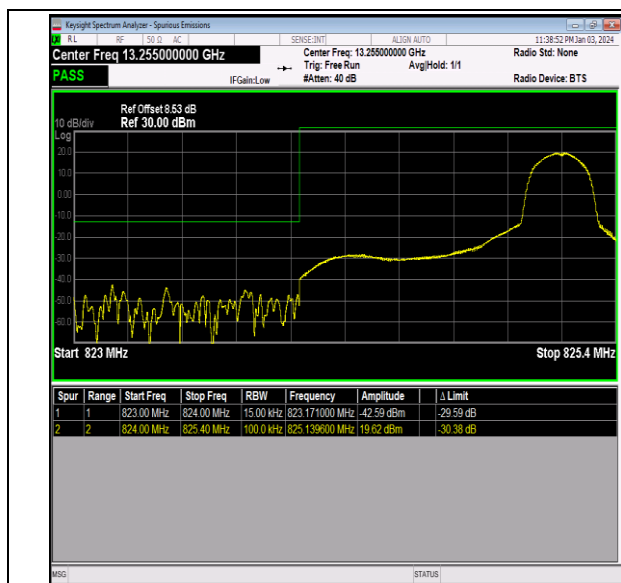
Band26_1.4MHz_64QAM_26797_1RB#5
