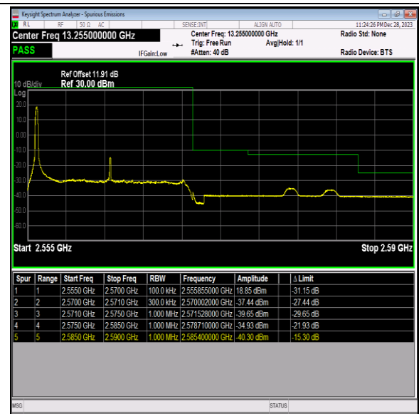
Band7_15MHz_16QAM_21375_1RB#0
