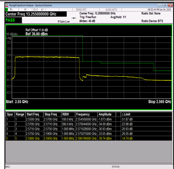
Band7_20MHz_64QAM_21350_100RB#0
