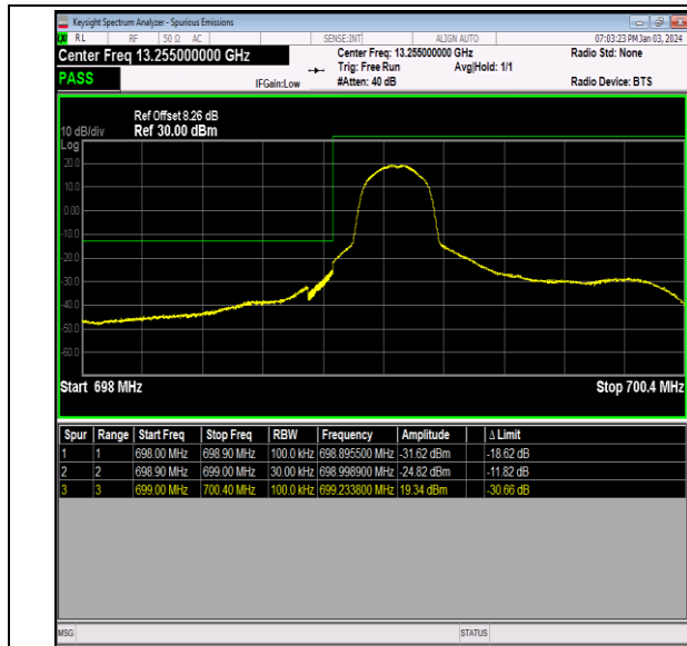
Band12_1.4MHz_64QAM_23017_1RB#0
