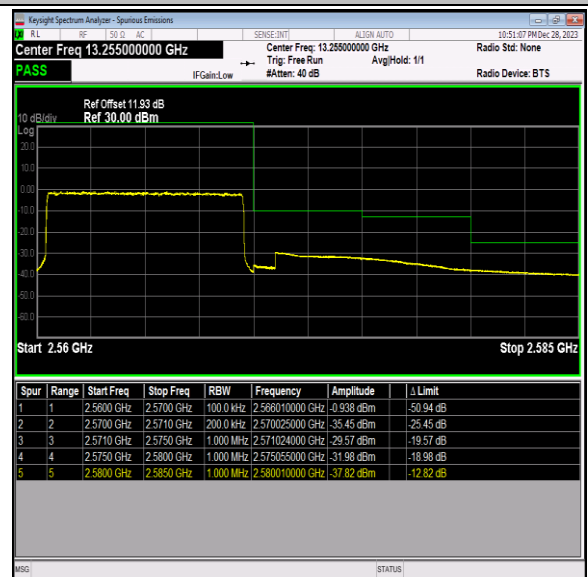
Band7_10MHz_64QAM_21400_50RB#0
