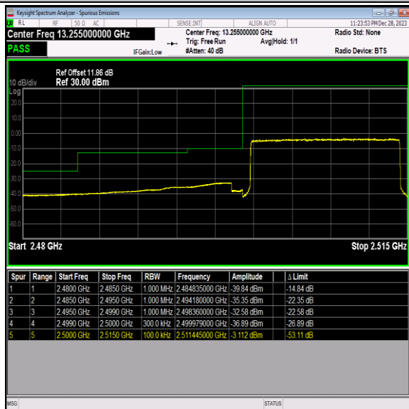
Band7_15MHz_64QAM_20825_75RB#0
