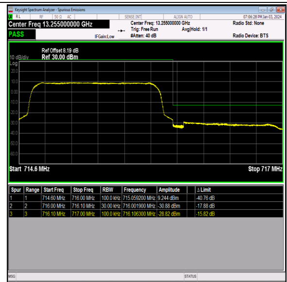
Band12_1.4MHz_QPSK_23173_6RB#0
