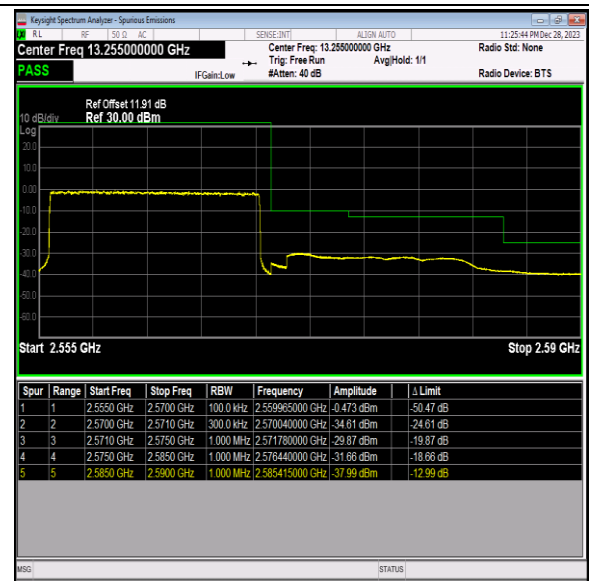
Band7_15MHz_QPSK_21375_75RB#0
