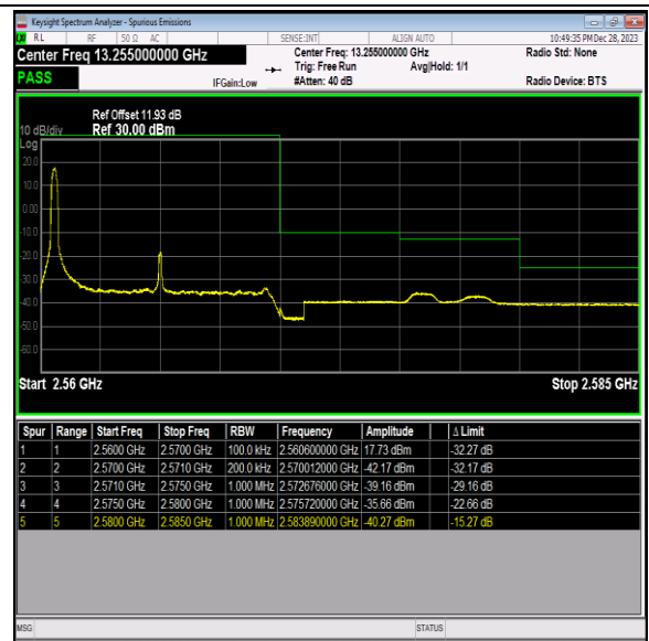
Band7_10MHz_64QAM_21400_1RB#0
