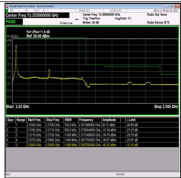
Band7_20MHz_64QAM_21350_1RB#0
