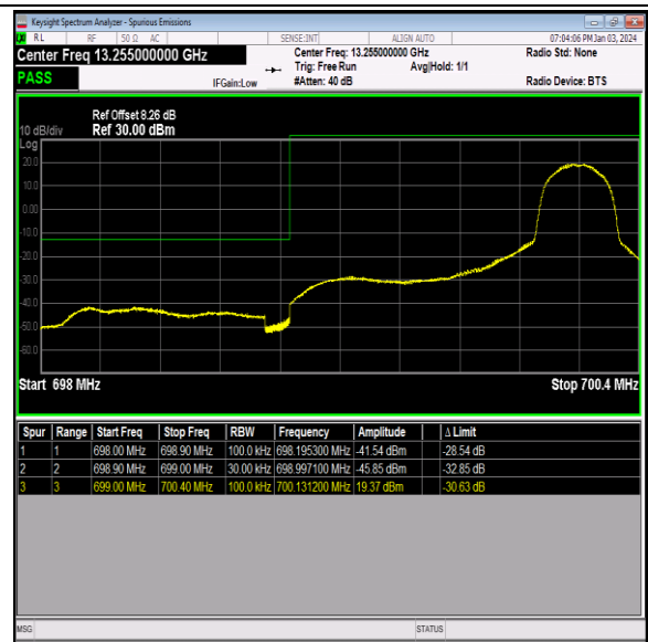
Band12_1.4MHz_64QAM_23017_1RB#5
