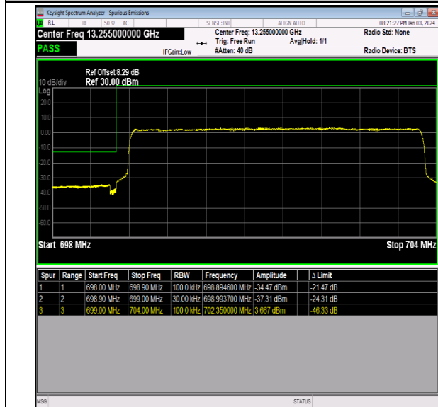
Band12_5MHz_QPSK_23035_25RB#0
