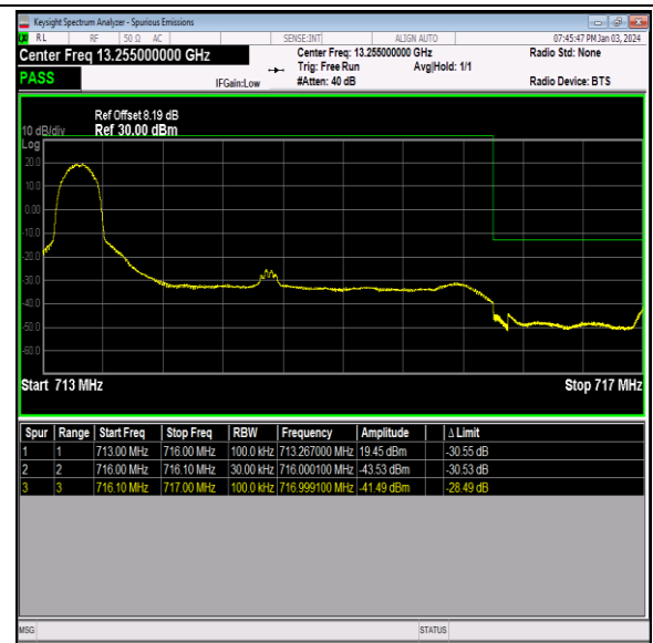
Band12_3MHz_64QAM_23165_1RB#0
