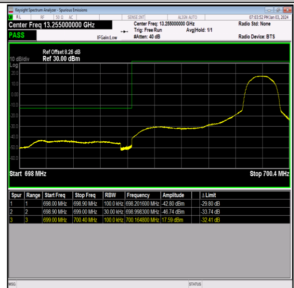
Band12_1.4MHz_16QAM_23017_1RB#5
