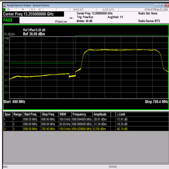
Band12_1.4MHz_64QAM_23017_6RB#0
