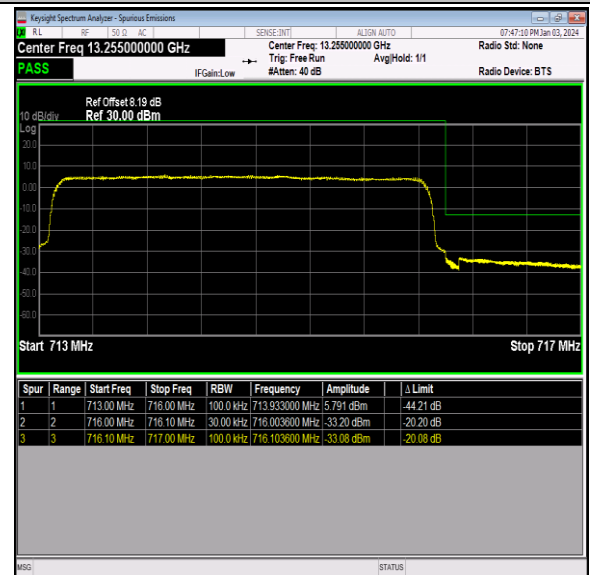
Band12_3MHz_64QAM_23165_15RB#0
