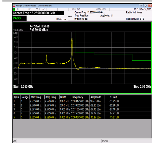
Band7_15MHz_16QAM_21375_1RB#74
