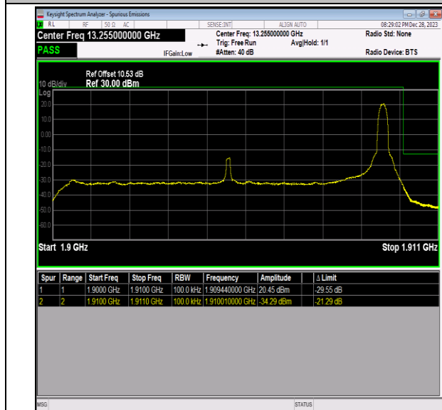
Band2_10MHz_QPSK_19150_1RB#49
