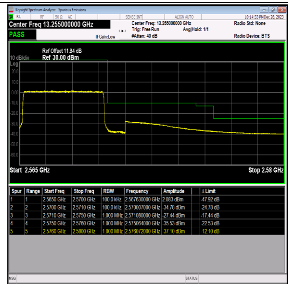
Band7_5MHz_64QAM_21425_25RB#0
