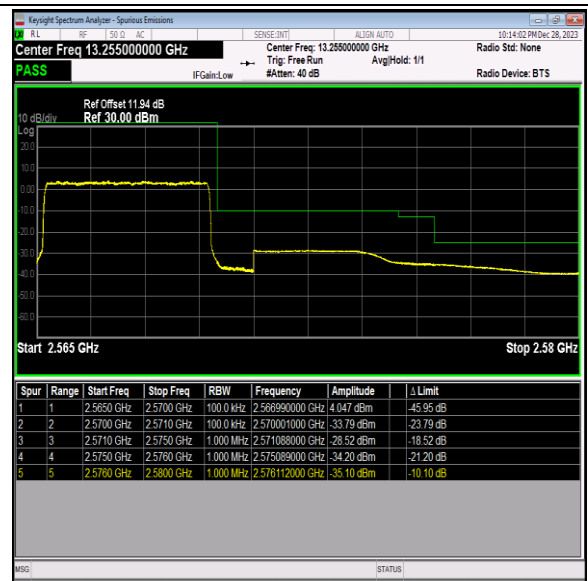
Band7_5MHz_QPSK_21425_25RB#0
