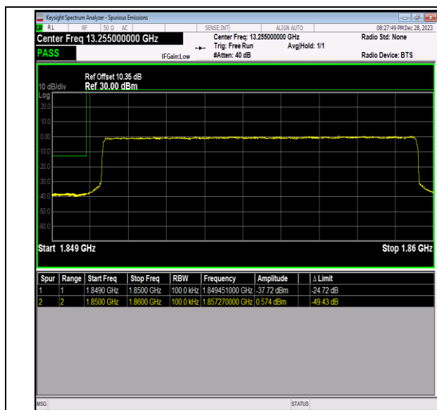
Band2_10MHz_QPSK_18650_50RB#0
