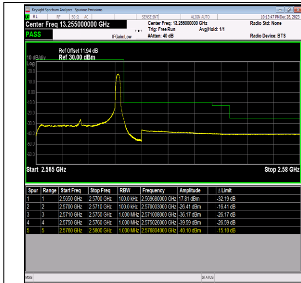
Band7_5MHz_64QAM_21425_1RB#24
