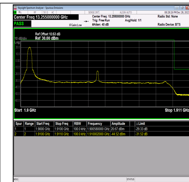
Band2_10MHz_QPSK_19150_1RB#0
