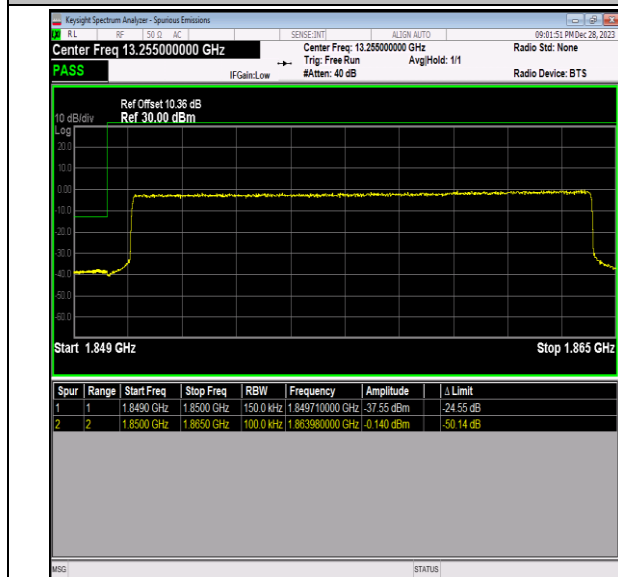
Band2_15MHz_QPSK_18675_75RB#0
