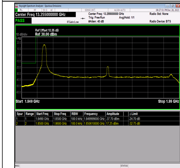
Band2_10MHz_64QAM_18650_1RB#0
