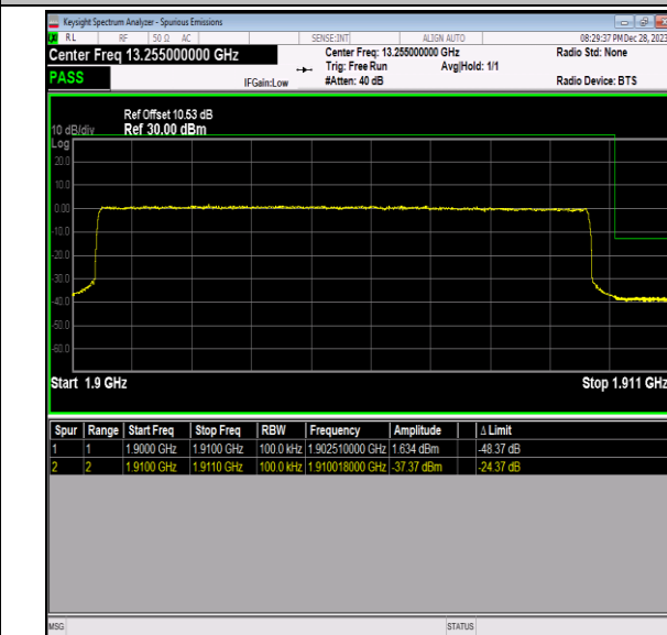
Band2_10MHz_QPSK_19150_50RB#0
