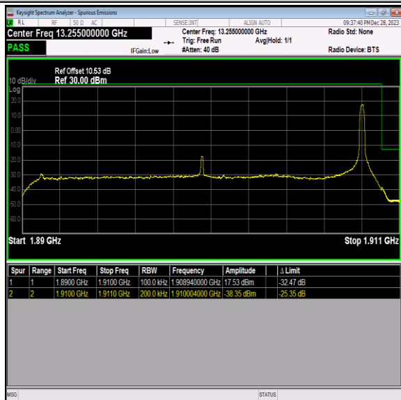
Band2_20MHz_64QAM_19100_1RB#99
