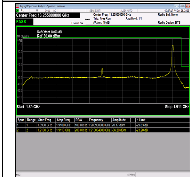
Band2_20MHz_QPSK_19100_1RB#99
