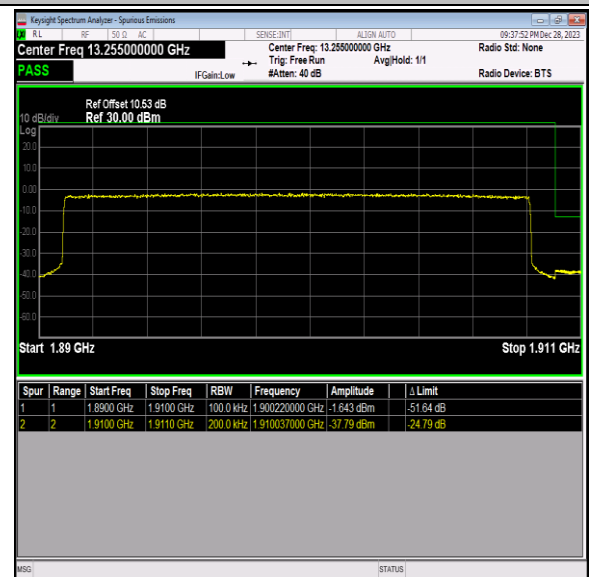
Band2_20MHz_QPSK_19100_100RB#0
