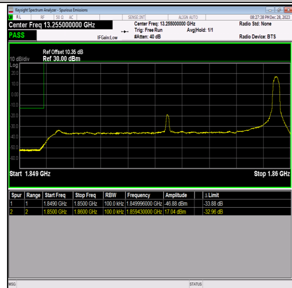
Band2_10MHz_64QAM_18650_1RB#49
