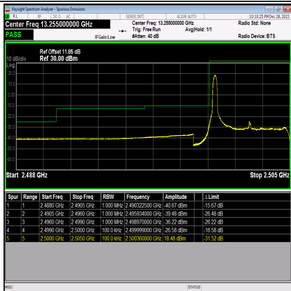
Band7_5MHz_16QAM_20775_1RB#0
