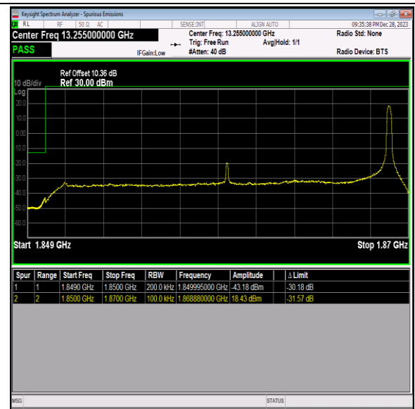
Band2_20MHz_16QAM_18700_1RB#99
