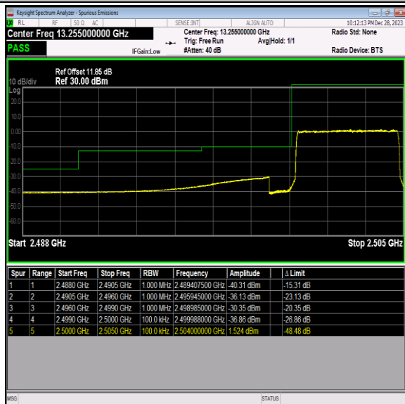
Band7_5MHz_64QAM_20775_25RB#0
