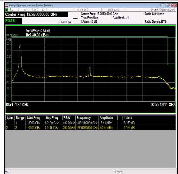
Band2_20MHz_16QAM_19100_1RB#0
