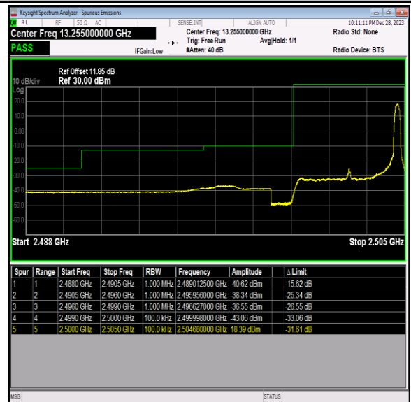
Band7_5MHz_16QAM_20775_1RB#24
