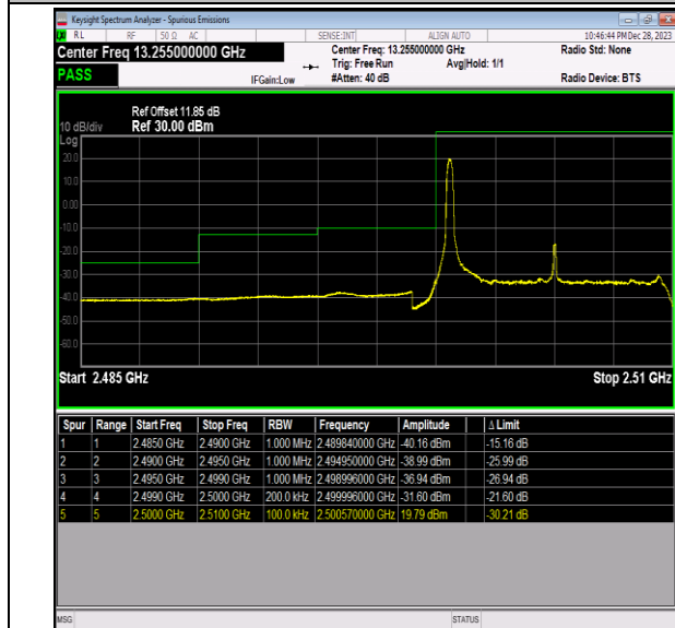
Band7_10MHz_QPSK_20800_1RB#0
