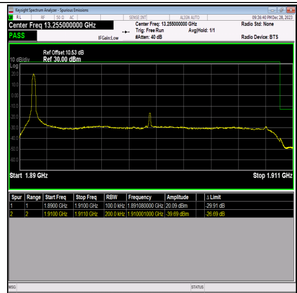
Band2_20MHz_QPSK_19100_1RB#0
