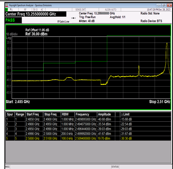
Band7_10MHz_QPSK_20800_1RB#49
