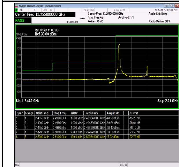
Band7_10MHz_64QAM_20800_1RB#0
