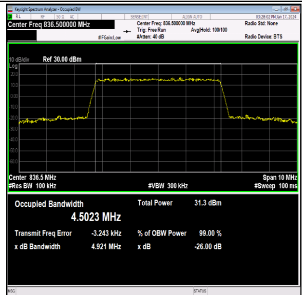
26(824-849)-5MHz-QPSK-26915-25RB#0-PASS
