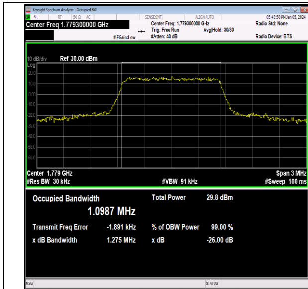
Band66-1.4MHz-16QAM-132665-6RB#0-PASS
