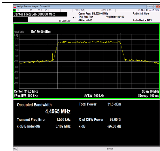
26(824-849)-5MHz-QPSK-27015-25RB#0-PASS
