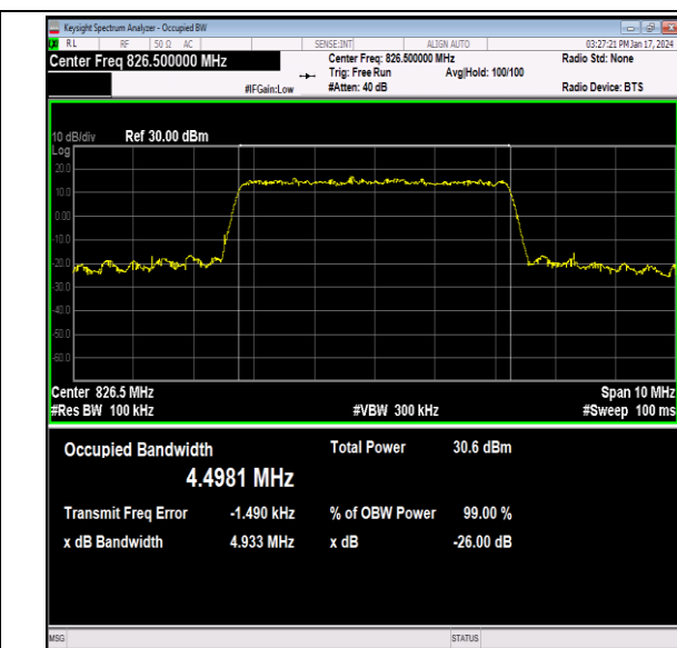
26(824-849)-5MHz-16QAM-26815-25RB#0-PASS
