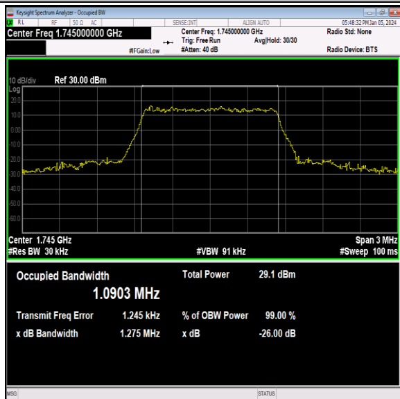
Band66-1.4MHz-64QAM-132322-6RB#0-PASS
