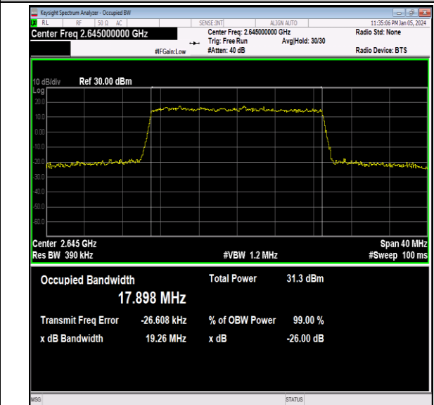
41(2535-2655)-20MHz-16QAM-41140-100RB#0-PASS
