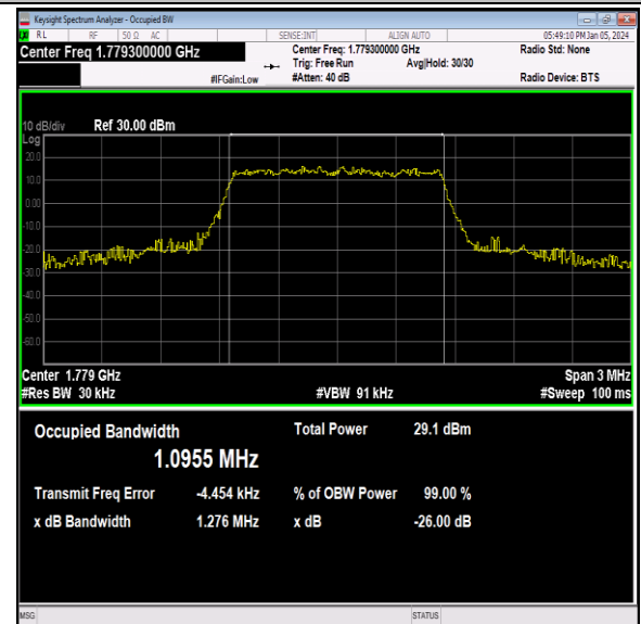
Band66-1.4MHz-64QAM-132665-6RB#0-PASS
