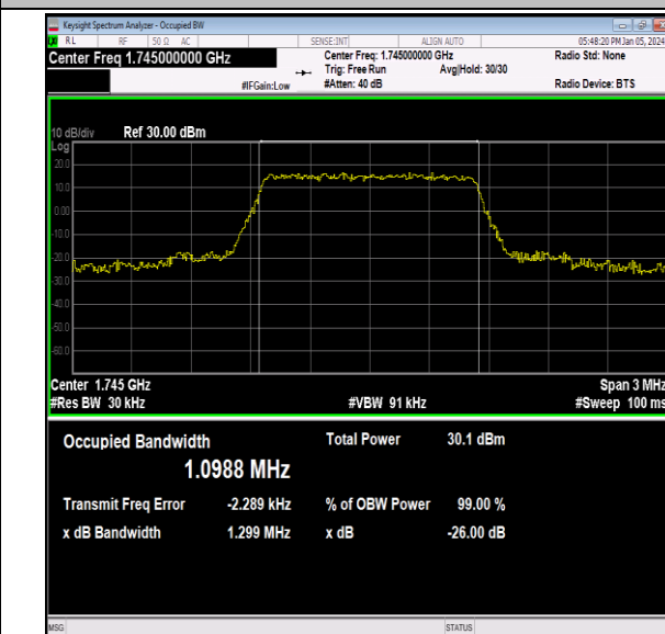
Band66-1.4MHz-16QAM-132322-6RB#0-PASS
