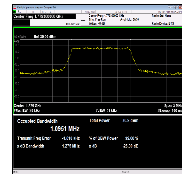
Band66-1.4MHz-QPSK-132665-6RB#0-PASS
