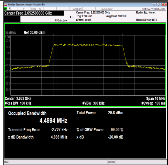
41(2535-2655)-5MHz-64QAM-41215-25RB#0-PASS
