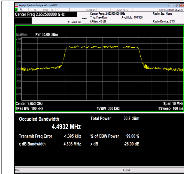
41(2535-2655)-5MHz-16QAM-41215-25RB#0-PASS
