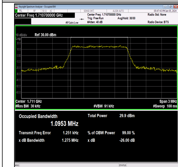
Band66-1.4MHz-16QAM-131979-6RB#0-PASS
