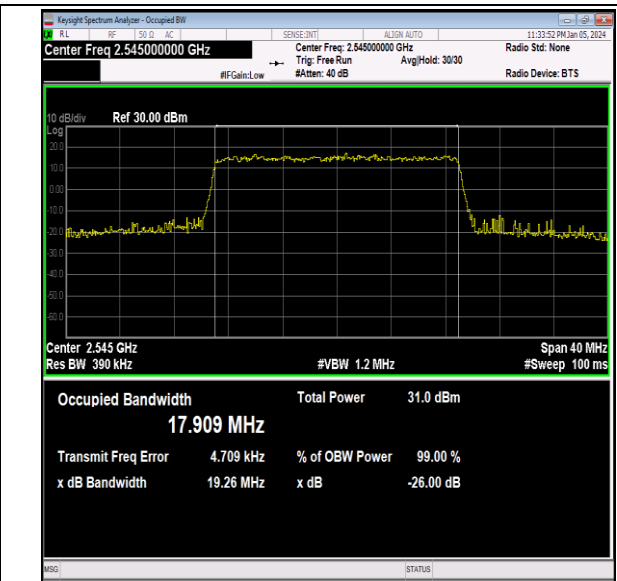
41(2535-2655)-20MHz-16QAM-40140-100RB#0-PASS
