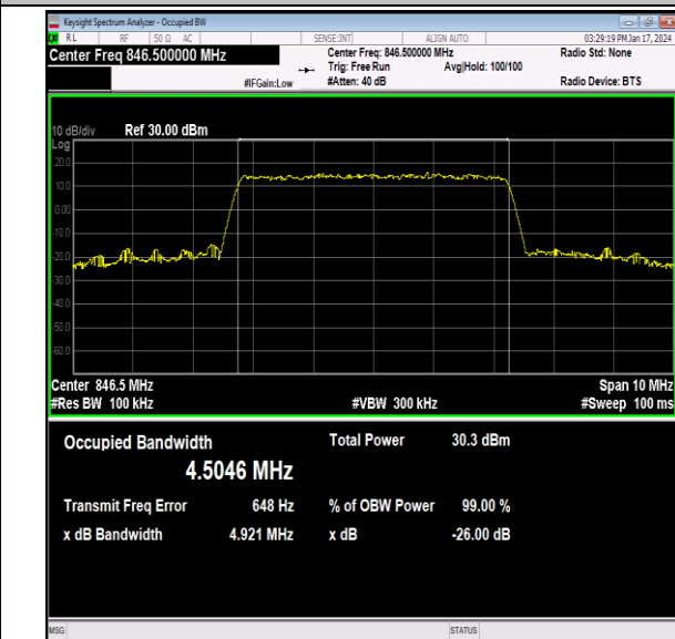
26(824-849)-5MHz-16QAM-27015-25RB#0-PASS
