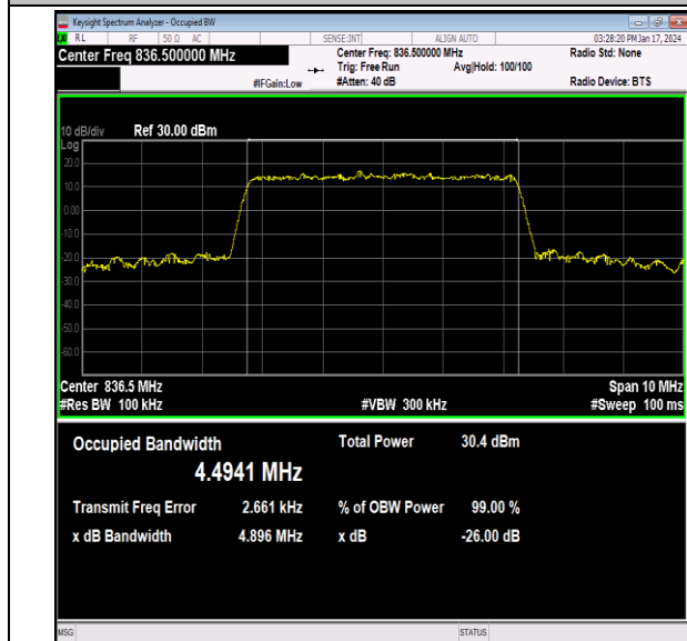
26(824-849)-5MHz-16QAM-26915-25RB#0-PASS
