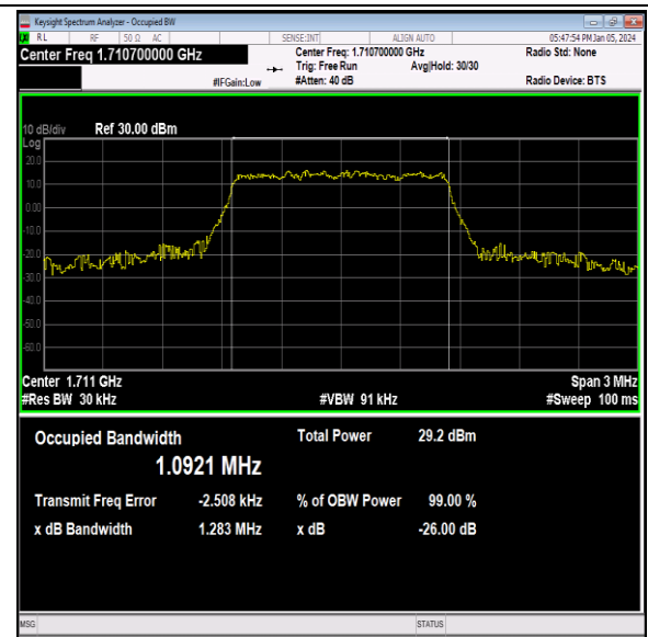
Band66-1.4MHz-64QAM-131979-6RB#0-PASS
