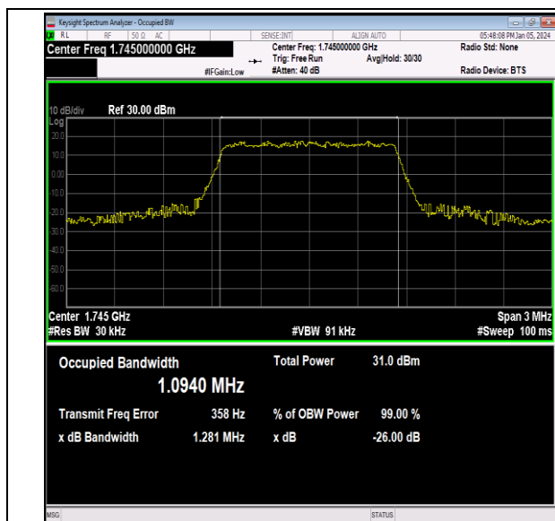
Band66-1.4MHz-QPSK-132322-6RB#0-PASS
