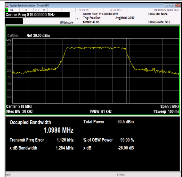
26(814-824)-1.4MHz-QPSK-26740-6RB#0-PASS
