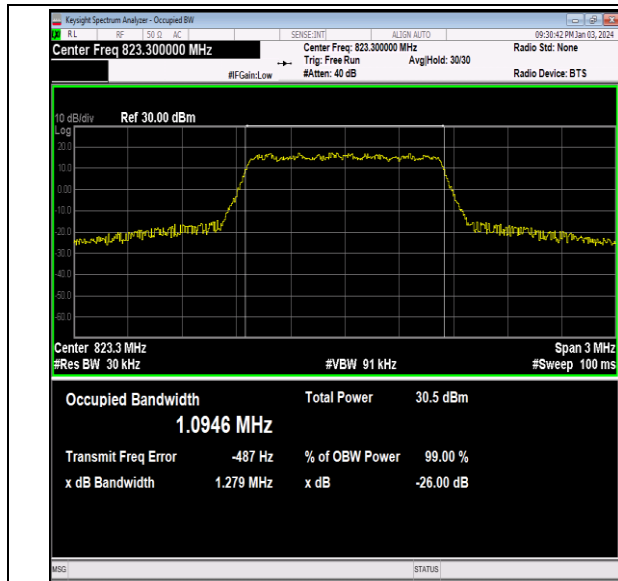
26(814-824)-1.4MHz-QPSK-26783-6RB#0-PASS
