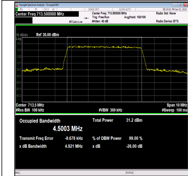
Band12-5MHz-QPSK-23155-25RB#0-PASS
