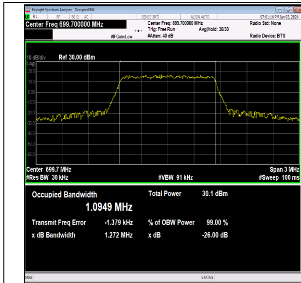
Band12-1.4MHz-64QAM-23017-6RB#0-PASS
