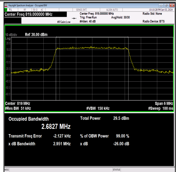
26(814-824)-3MHz-16QAM-26740-15RB#0-PASS
