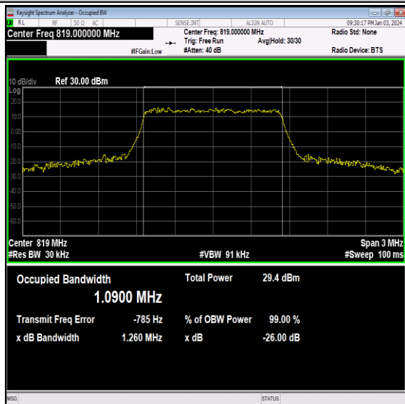
26(814-824)-1.4MHz-16QAM-26740-6RB#0-PASS
