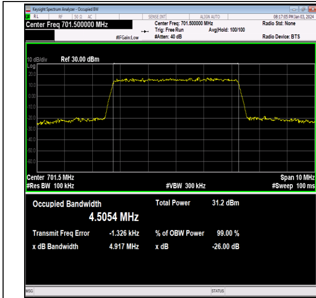
Band12-5MHz-QPSK-23035-25RB#0-PASS
