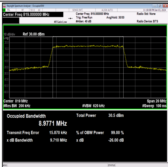
26(814-824)-10MHz-16QAM-26740-50RB#0-PASS
