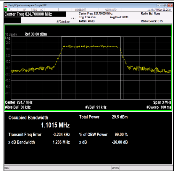
26(824-849)-1.4MHz-16QAM-26797-6RB#0-PASS
