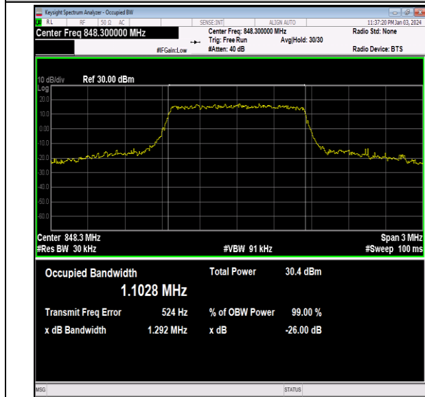
26(824-849)-1.4MHz-QPSK-27033-6RB#0-PASS
