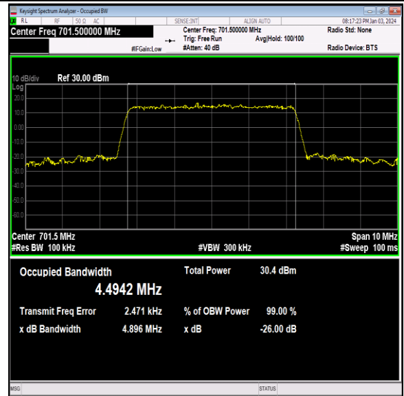
Band12-5MHz-16QAM-23035-25RB#0-PASS
