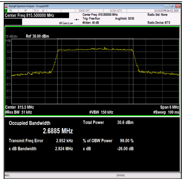
26(814-824)-3MHz-64QAM-26705-15RB#0-PASS
