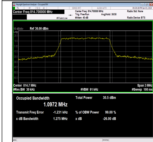
26(814-824)-1.4MHz-QPSK-26697-6RB#0-PASS
