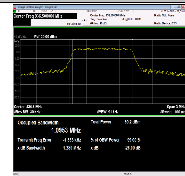
26(824-849)-1.4MHz-64QAM-26915-6RB#0-PASS
