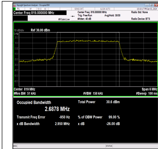
26(814-824)-3MHz-QPSK-26740-15RB#0-PASS
