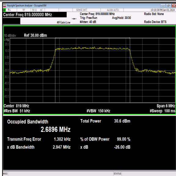
26(814-824)-3MHz-64QAM-26740-15RB#0-PASS
