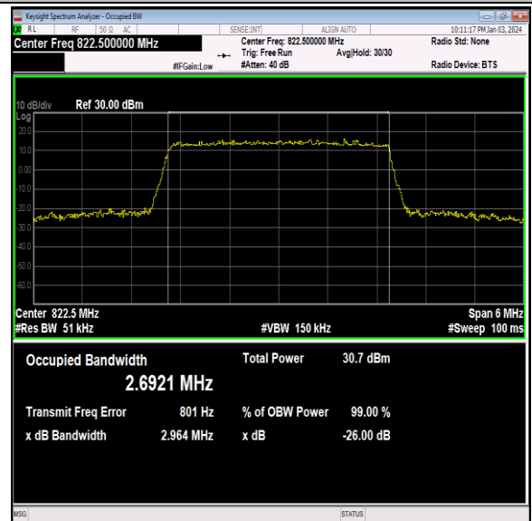
26(814-824)-3MHz-64QAM-26775-15RB#0-PASS
