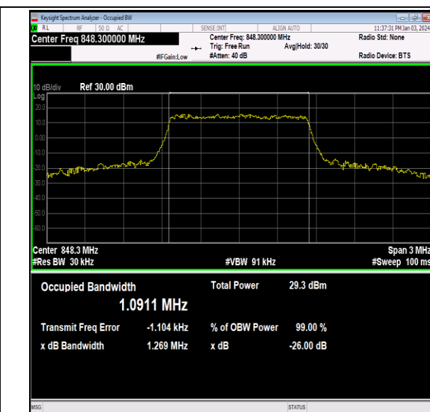
26(824-849)-1.4MHz-16QAM-27033-6RB#0-PASS
