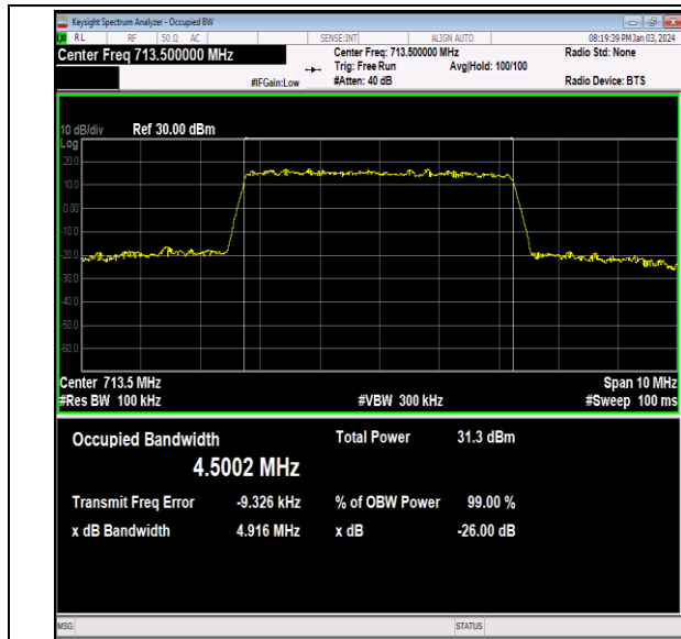
Band12-5MHz-64QAM-23155-25RB#0-PASS
