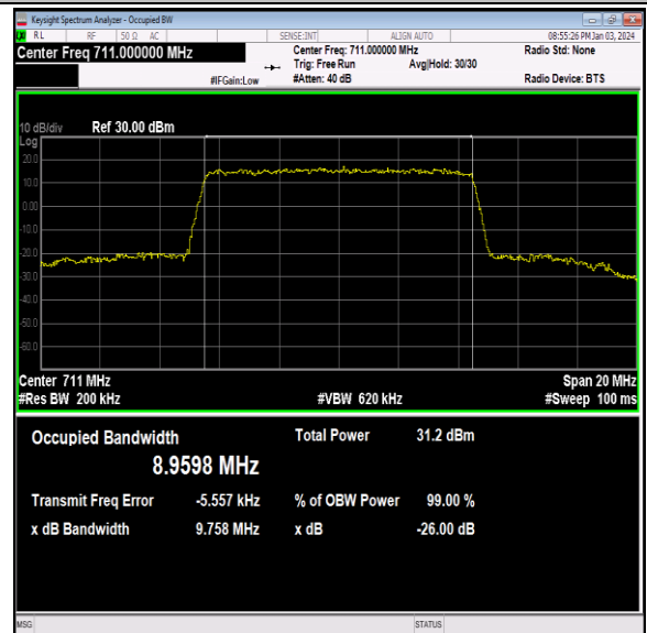
Band12-10MHz-QPSK-23130-50RB#0-PASS
