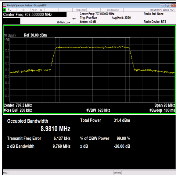
Band12-10MHz-QPSK-23095-50RB#0-PASS
