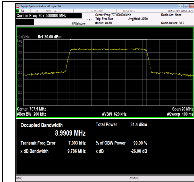
Band12-10MHz-64QAM-23095-50RB#0-PASS
