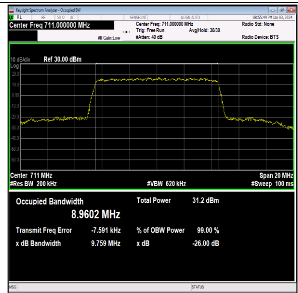
Band12-10MHz-64QAM-23130-50RB#0-PASS
