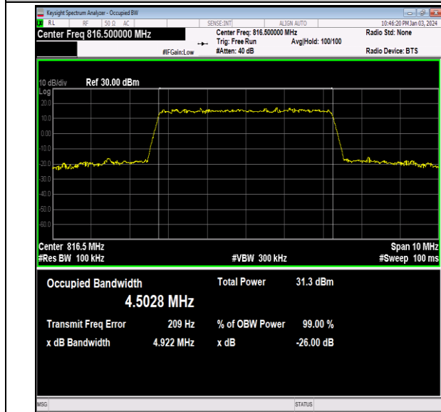
26(814-824)-5MHz-64QAM-26715-25RB#0-PASS
