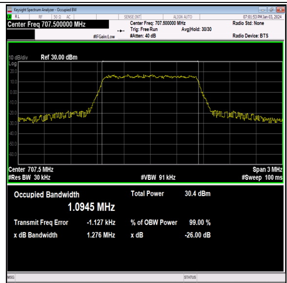
Band12-1.4MHz-64QAM-23095-6RB#0-PASS
