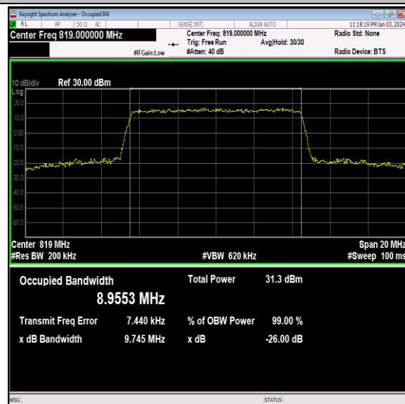
26(814-824)-10MHz-64QAM-26740-50RB#0-PASS
