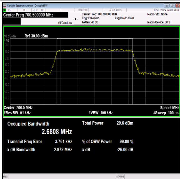
Band12-3MHz-16QAM-23025-15RB#0-PASS
