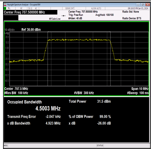
Band12-5MHz-QPSK-23095-25RB#0-PASS
