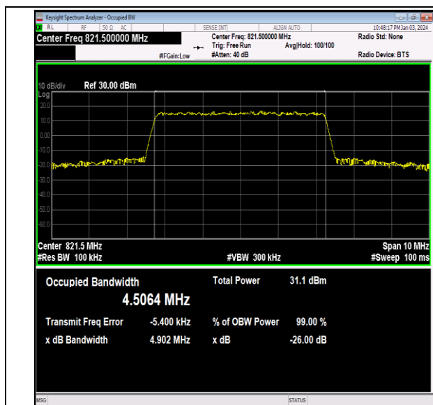
26(814-824)-5MHz-64QAM-26765-25RB#0-PASS
