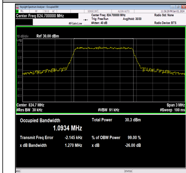
26(824-849)-1.4MHz-64QAM-26797-6RB#0-PASS
