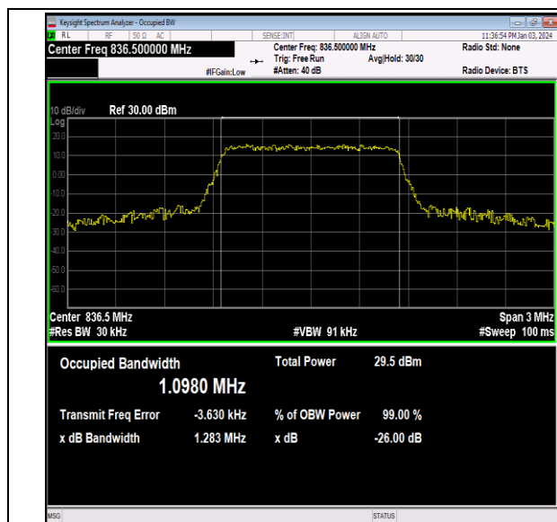
26(824-849)-1.4MHz-16QAM-26915-6RB#0-PASS
