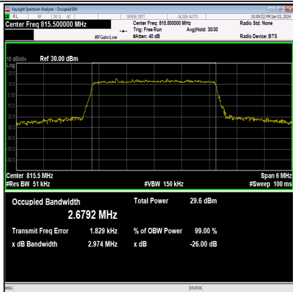
26(814-824)-3MHz-16QAM-26705-15RB#0-PASS
