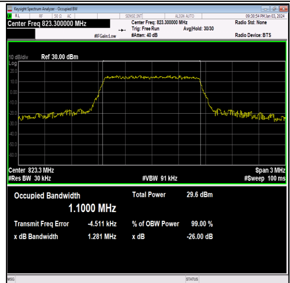
26(814-824)-1.4MHz-16QAM-26783-6RB#0-PASS
