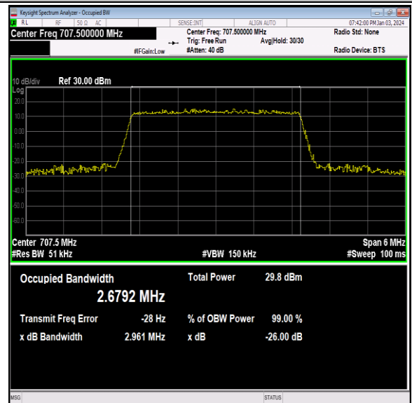
Band12-3MHz-16QAM-23095-15RB#0-PASS
