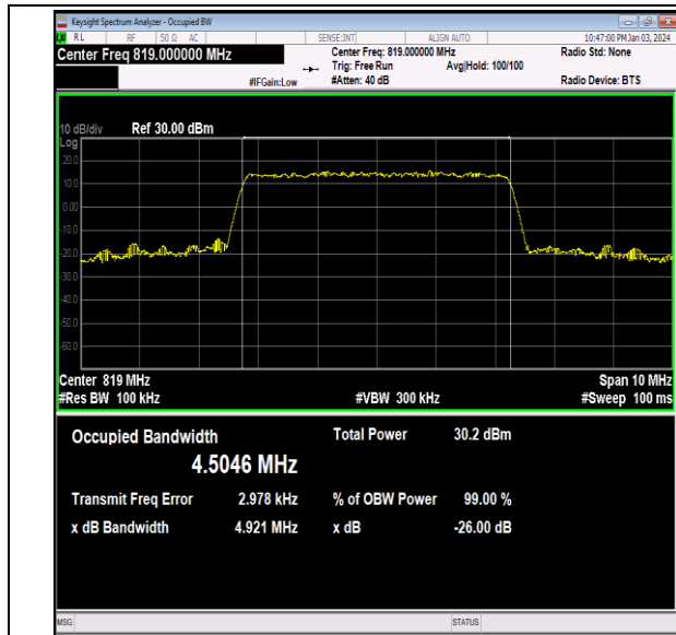
26(814-824)-5MHz-16QAM-26740-25RB#0-PASS
