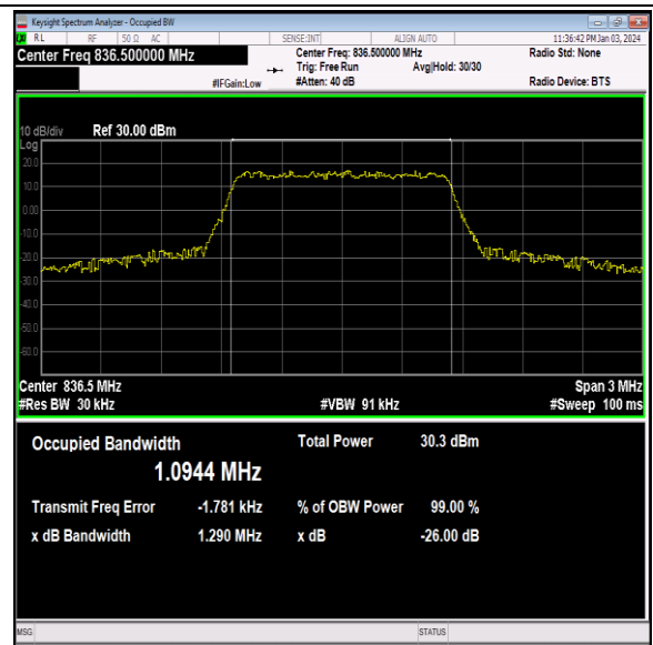
26(824-849)-1.4MHz-QPSK-26915-6RB#0-PASS
