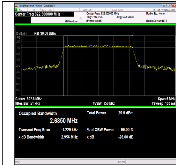
26(814-824)-3MHz-16QAM-26775-15RB#0-PASS
