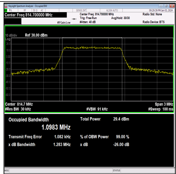
26(814-824)-1.4MHz-16QAM-26697-6RB#0-PASS
