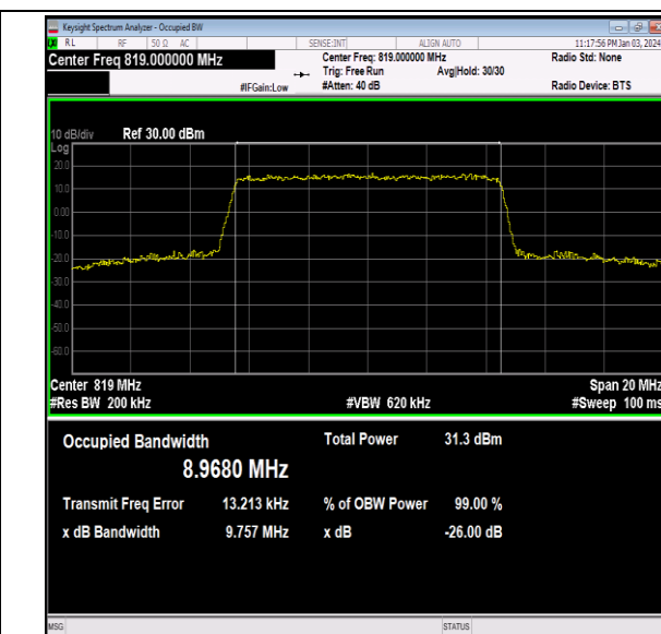
26(814-824)-10MHz-QPSK-26740-50RB#0-PASS
