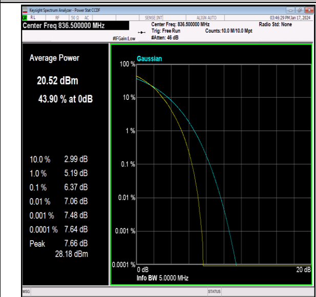
26(824-849)-5MHz-64QAM-26915-25RB#0-PASS
