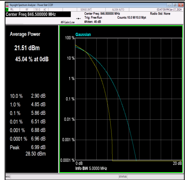
26(824-849)-5MHz-16QAM-27015-25RB#0-PASS
