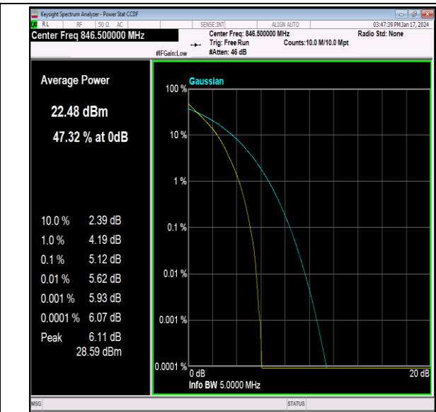
26(824-849)-5MHz-QPSK-27015-25RB#0-PASS
