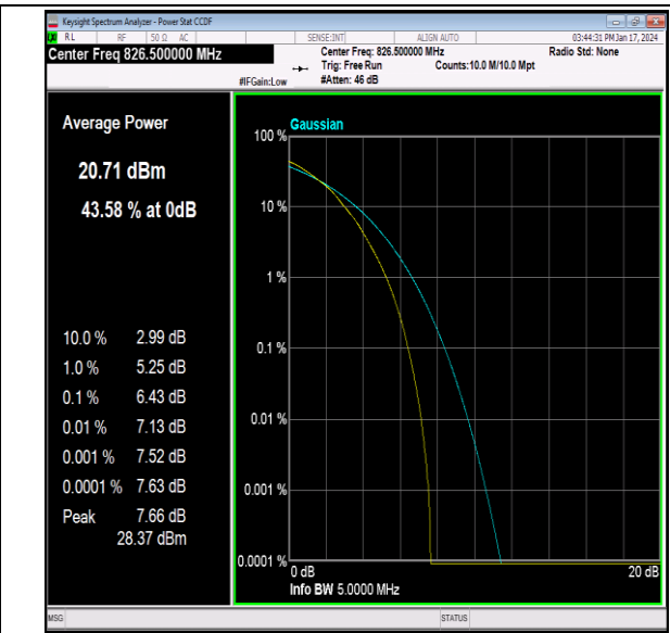
26(824-849)-5MHz-64QAM-26815-25RB#0-PASS
