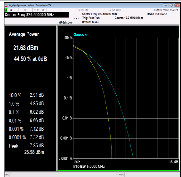
26(824-849)-5MHz-16QAM-26815-25RB#0-PASS
