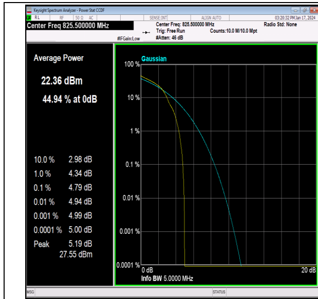
26(824-849)-3MHz-16QAM-26805-1RB#0-PASS
