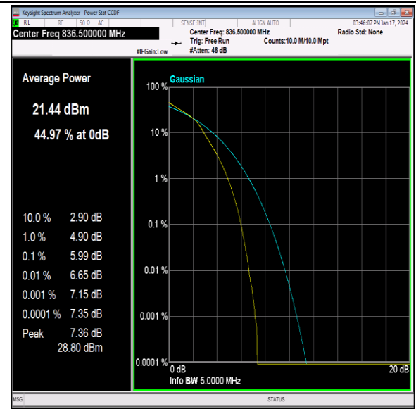
26(824-849)-5MHz-16QAM-26915-25RB#0-PASS
