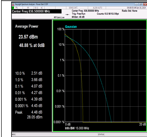
26(824-849)-15MHz-QPSK-26915-1RB#0-PASS
