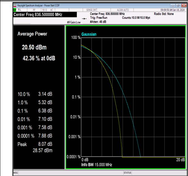
26(824-849)-15MHz-64QAM-26915-75RB#0-PASS
