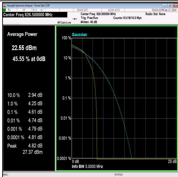
26(824-849)-5MHz-16QAM-26815-1RB#0-PASS
