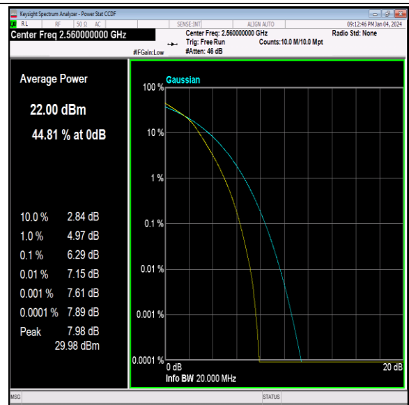
Band7-20MHz-16QAM-21350-100RB#0-PASS
