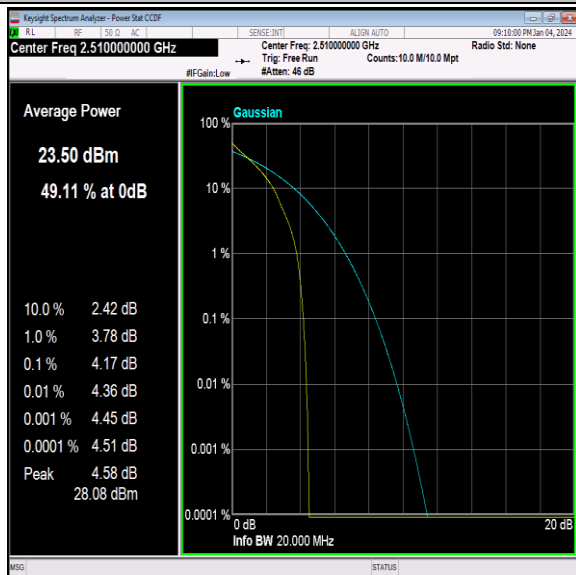
Band7-20MHz-64QAM-20850-1RB#0-PASS
