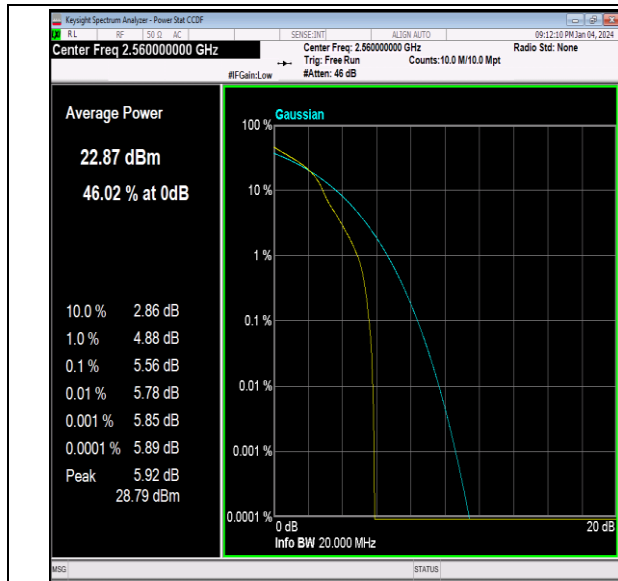
Band7-20MHz-16QAM-21350-1RB#0-PASS
