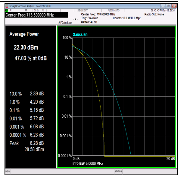
Band12-5MHz-QPSK-23155-25RB#0-PASS
