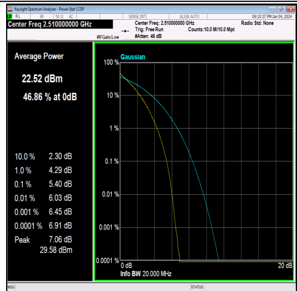
Band7-20MHz-64QAM-20850-100RB#0-PASS
