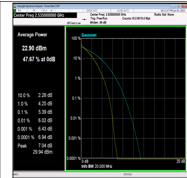
Band7-20MHz-64QAM-21100-100RB#0-PASS
