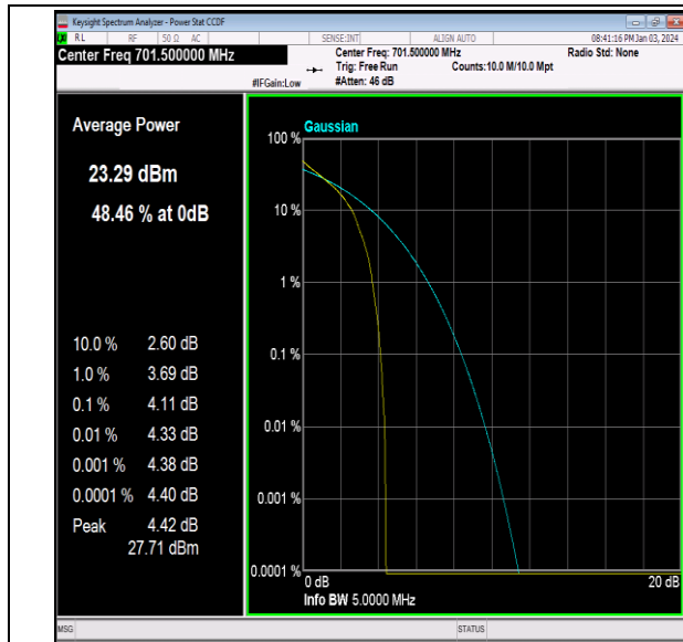
Band12-5MHz-64QAM-23035-1RB#0-PASS
