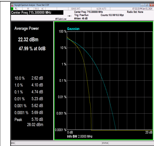
Band12-1.4MHz-QPSK-23173-6RB#0-PASS
