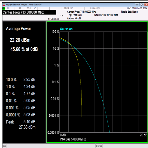
Band12-5MHz-16QAM-23155-1RB#0-PASS
