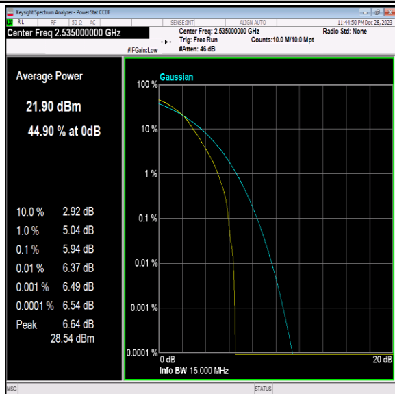
Band7-15MHz-64QAM-21100-1RB#0-PASS
