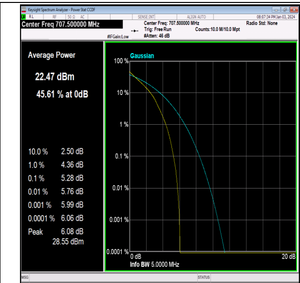
Band12-3MHz-64QAM-23095-15RB#0-PASS
