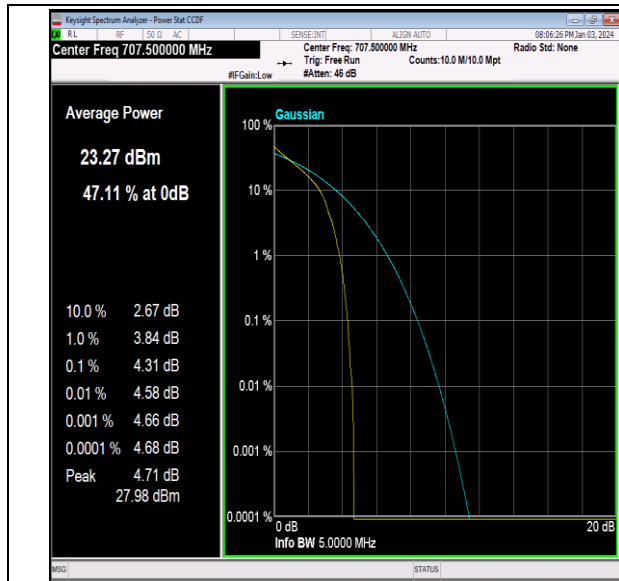
Band12-3MHz-64QAM-23095-1RB#0-PASS
