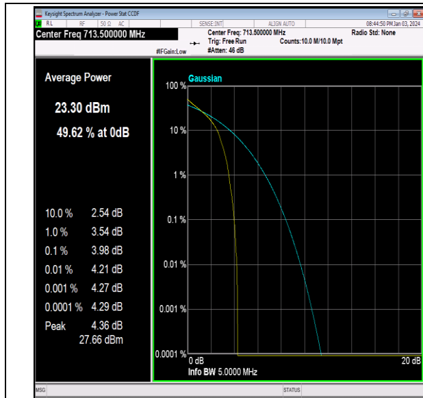
Band12-5MHz-QPSK-23155-1RB#0-PASS
