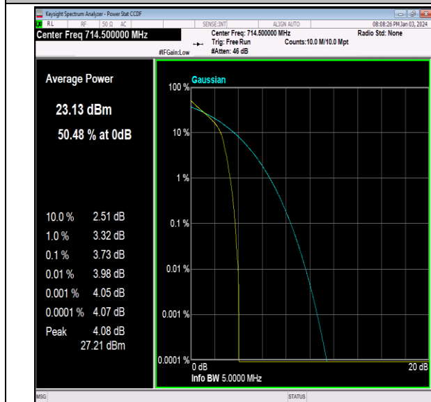
Band12-3MHz-64QAM-23165-1RB#0-PASS
