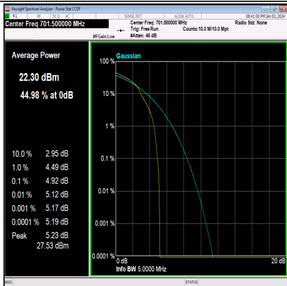
Band12-5MHz-16QAM-23035-1RB#0-PASS
