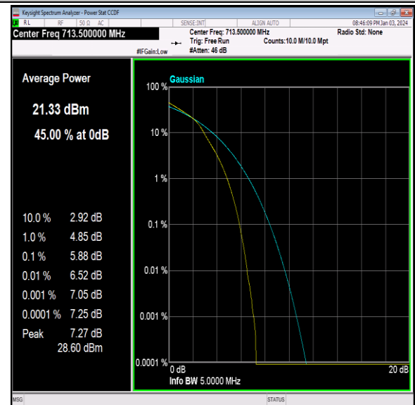
Band12-5MHz-16QAM-23155-25RB#0-PASS
