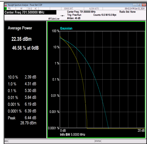
Band12-5MHz-64QAM-23035-25RB#0-PASS
