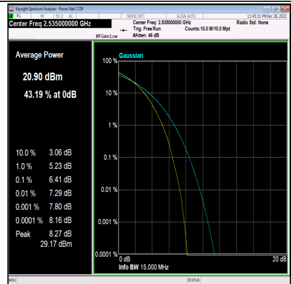
Band7-15MHz-64QAM-21100-75RB#0-PASS
