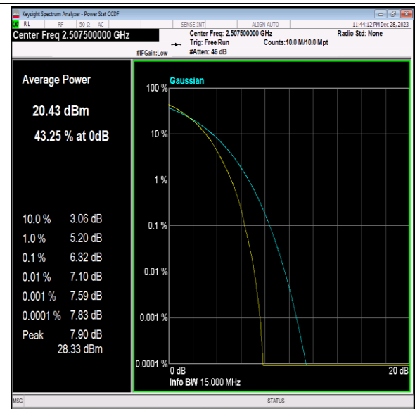
Band7-15MHz-64QAM-20825-75RB#0-PASS
