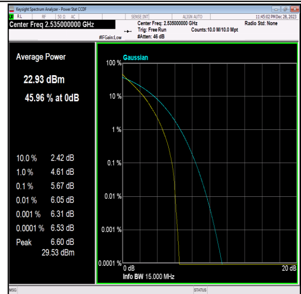
Band7-15MHz-QPSK-21100-75RB#0-PASS
