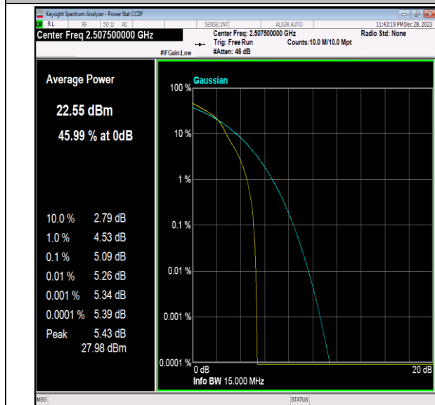
Band7-15MHz-16QAM-20825-1RB#0-PASS
