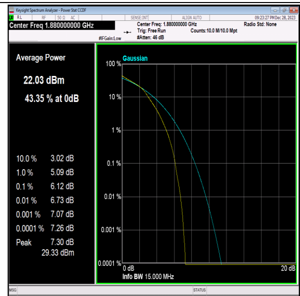
Band2-15MHz-16QAM-18900-75RB#0-PASS
