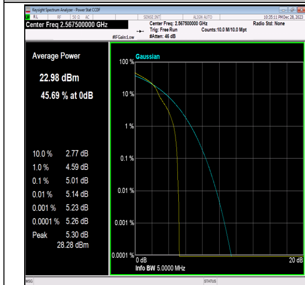
Band7-5MHz-16QAM-21425-1RB#0-PASS
