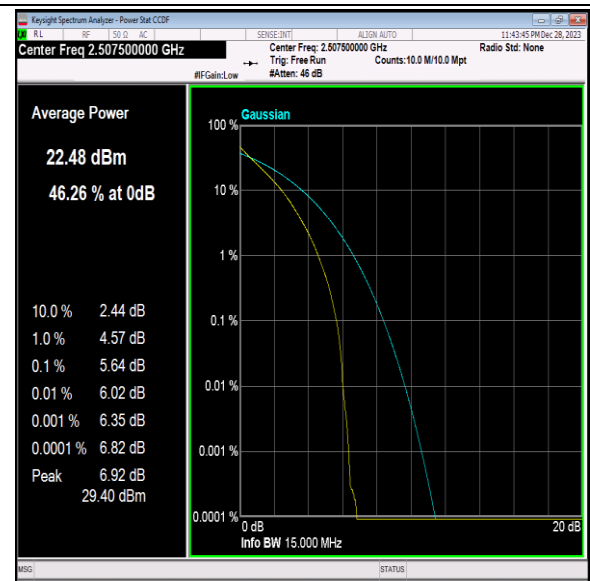
Band7-15MHz-QPSK-20825-75RB#0-PASS
