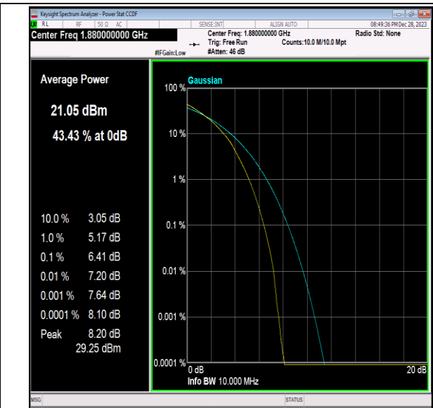
Band2-10MHz-64QAM-18900-50RB#0-PASS
