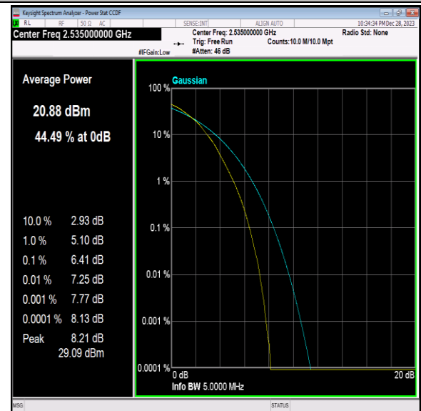
Band7-5MHz-64QAM-21100-25RB#0-PASS
