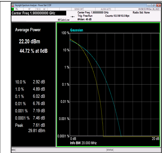
Band2-20MHz-16QAM-19100-100RB#0-PASS
