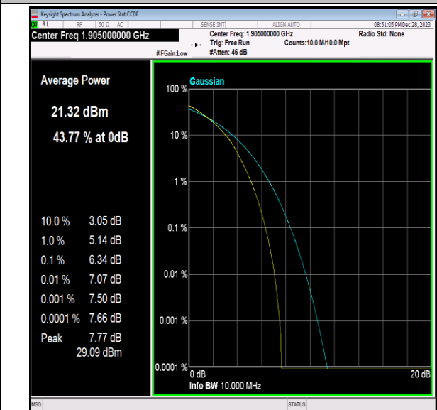
Band2-10MHz-64QAM-19150-50RB#0-PASS
