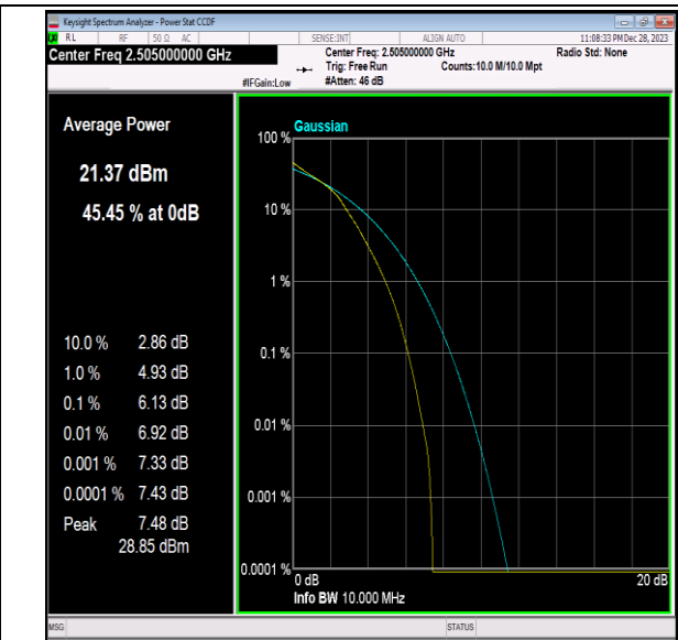
Band7-10MHz-16QAM-20800-50RB#0-PASS
