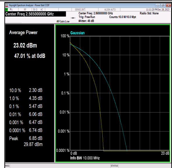
Band7-10MHz-QPSK-21400-50RB#0-PASS
