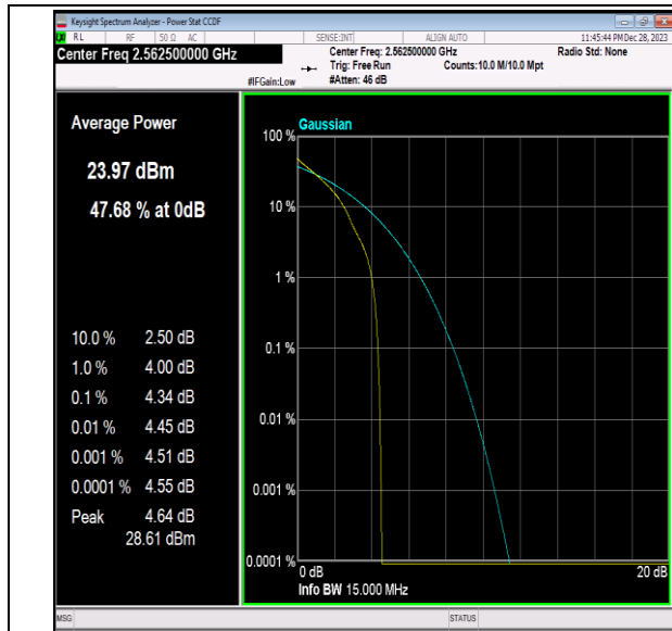
Band7-15MHz-QPSK-21375-1RB#0-PASS
