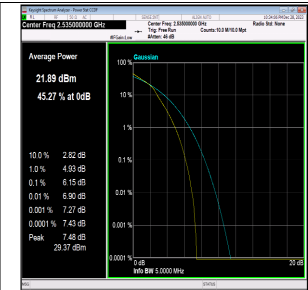
Band7-5MHz-16QAM-21100-25RB#0-PASS
