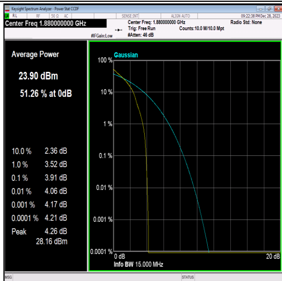
Band2-15MHz-QPSK-18900-1RB#0-PASS
