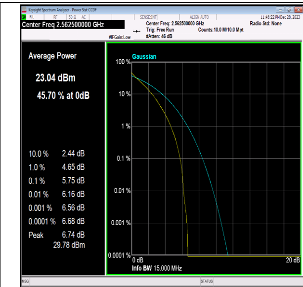
Band7-15MHz-QPSK-21375-75RB#0-PASS
