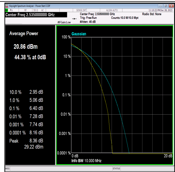
Band7-10MHz-64QAM-21100-50RB#0-PASS
