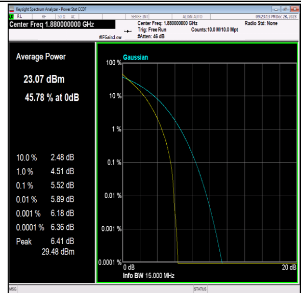
Band2-15MHz-QPSK-18900-75RB#0-PASS
