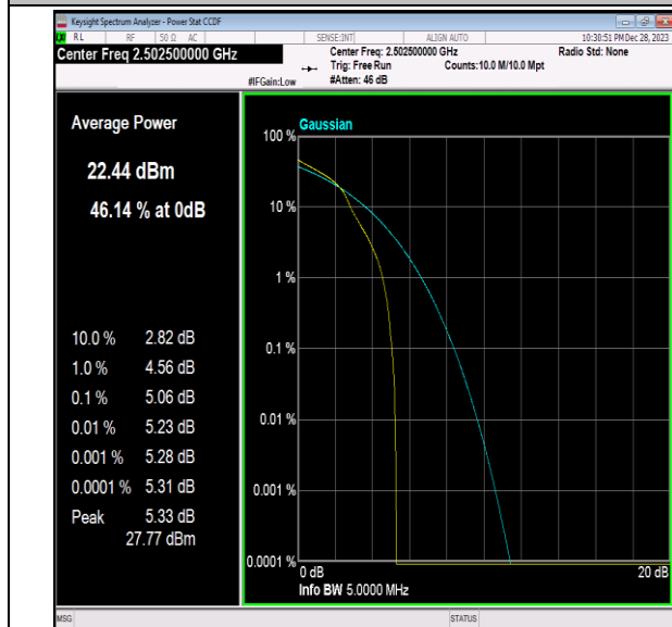
Band7-5MHz-16QAM-20775-1RB#0-PASS
