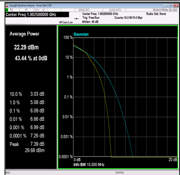
Band2-15MHz-16QAM-19125-75RB#0-PASS
