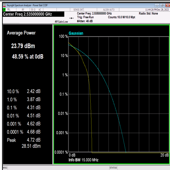
Band7-15MHz-QPSK-21100-1RB#0-PASS
