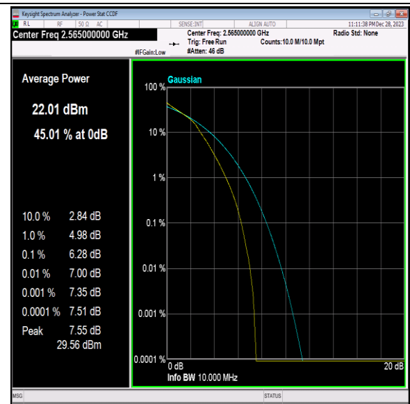
Band7-10MHz-16QAM-21400-50RB#0-PASS
