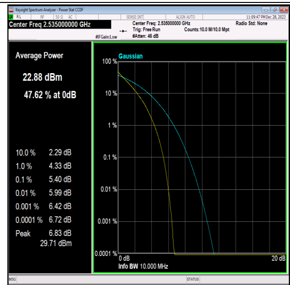
Band7-10MHz-QPSK-21100-50RB#0-PASS
