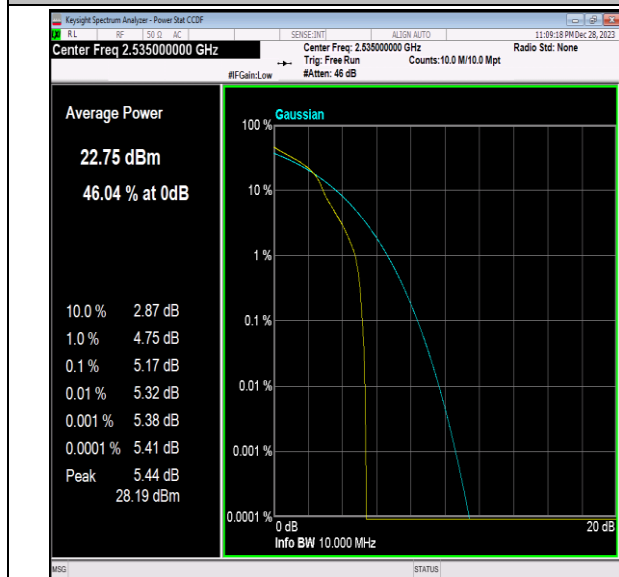
Band7-10MHz-16QAM-21100-1RB#0-PASS
