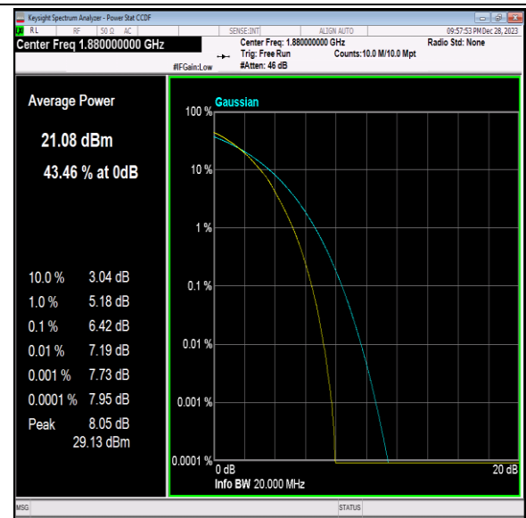
Band2-20MHz-64QAM-18900-100RB#0-PASS
