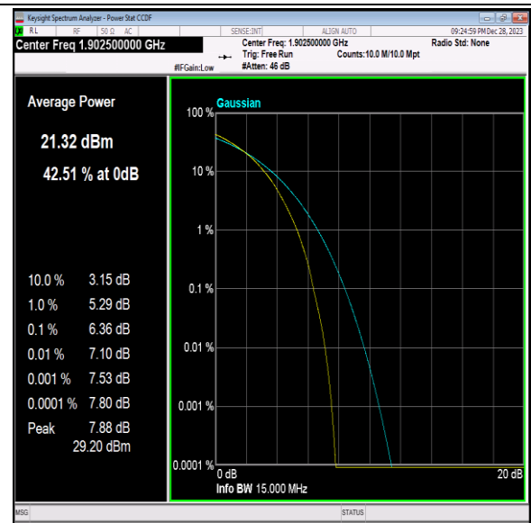
Band2-15MHz-64QAM-19125-75RB#0-PASS
