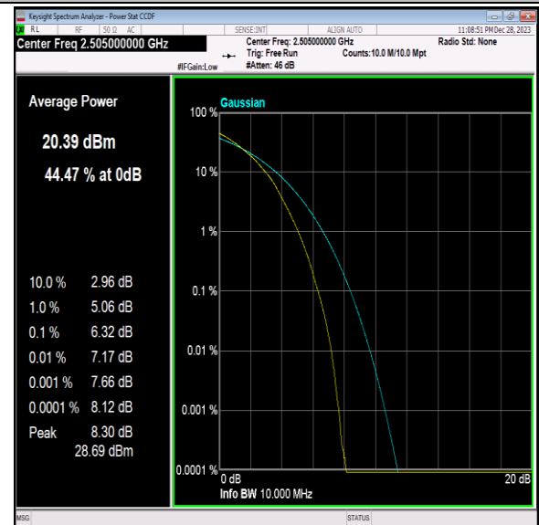
Band7-10MHz-64QAM-20800-50RB#0-PASS
