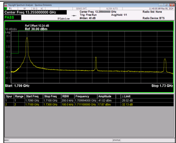
Band66_20MHz_64QAM_132072_1RB#0
