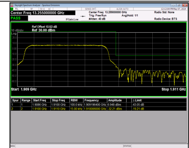
Band2_1.4MHz_64QAM_19193_6RB#0
