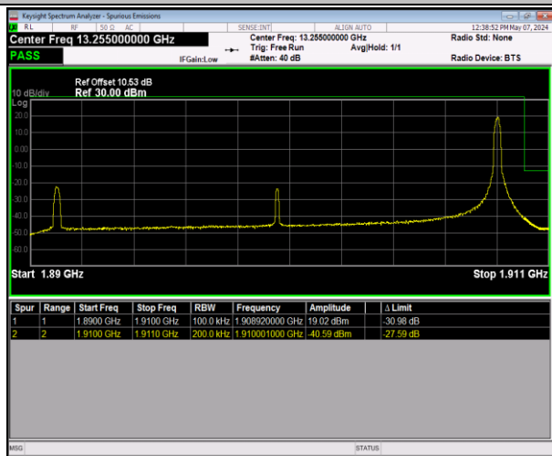
Band2_20MHz_16QAM_19100_1RB#99
