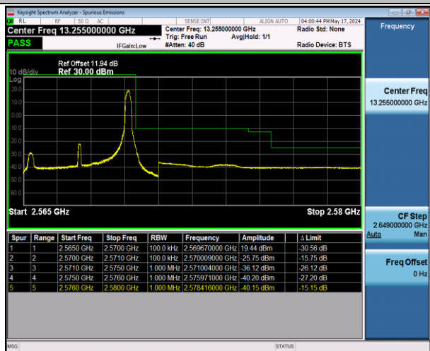
Band7_5MHz_16QAM_21425_1RB#24
